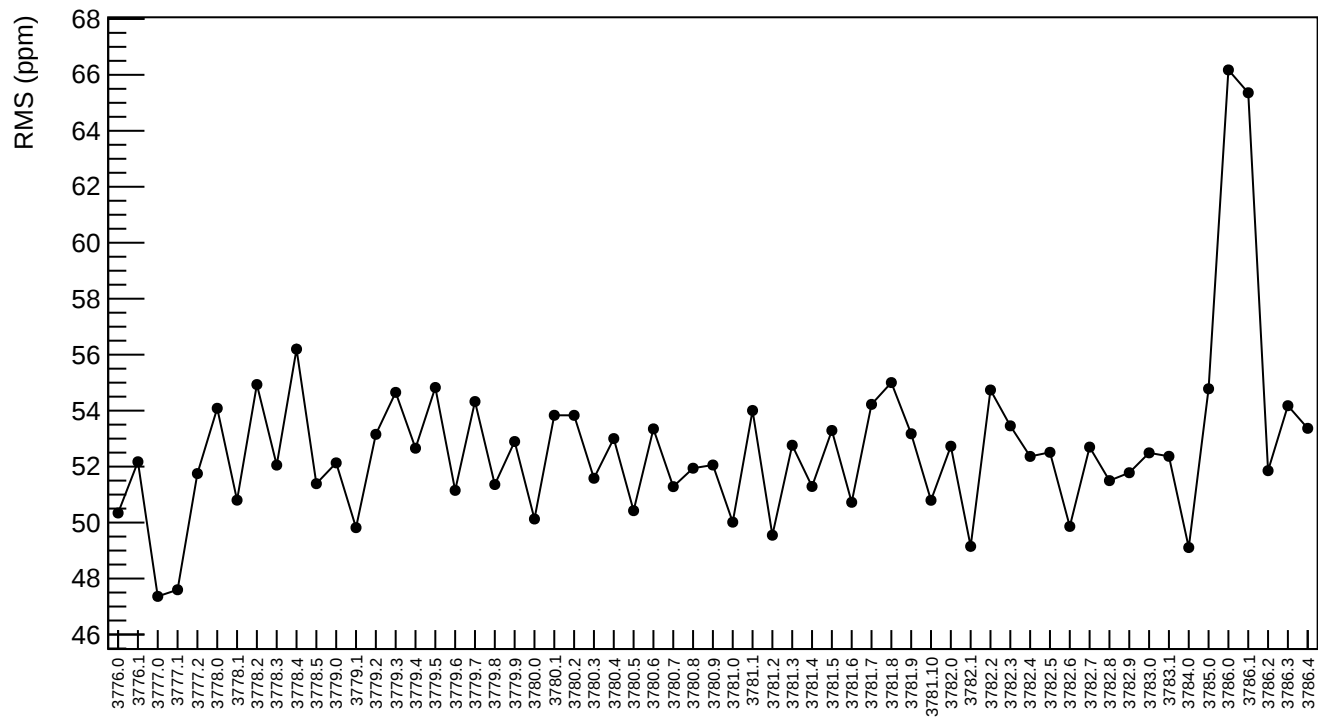
corr_usr_evMon4 RMS (ppm)
