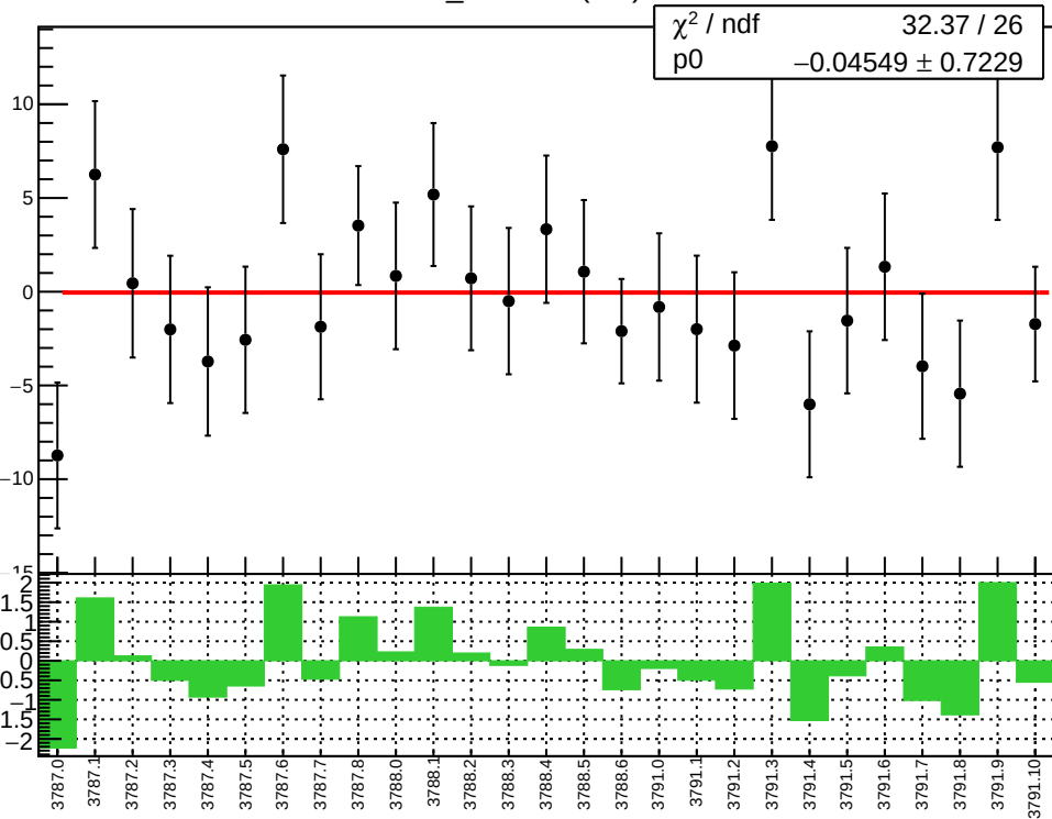
diff_evMon9 (nm)
