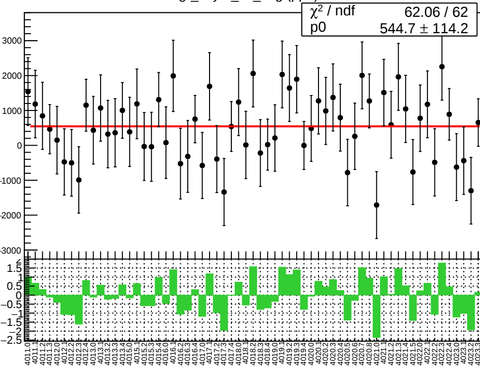
lagr_asym_us_avg (ppb)
