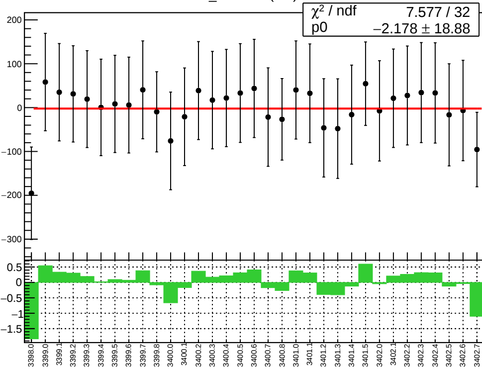
diff_evMon1 (nm)
