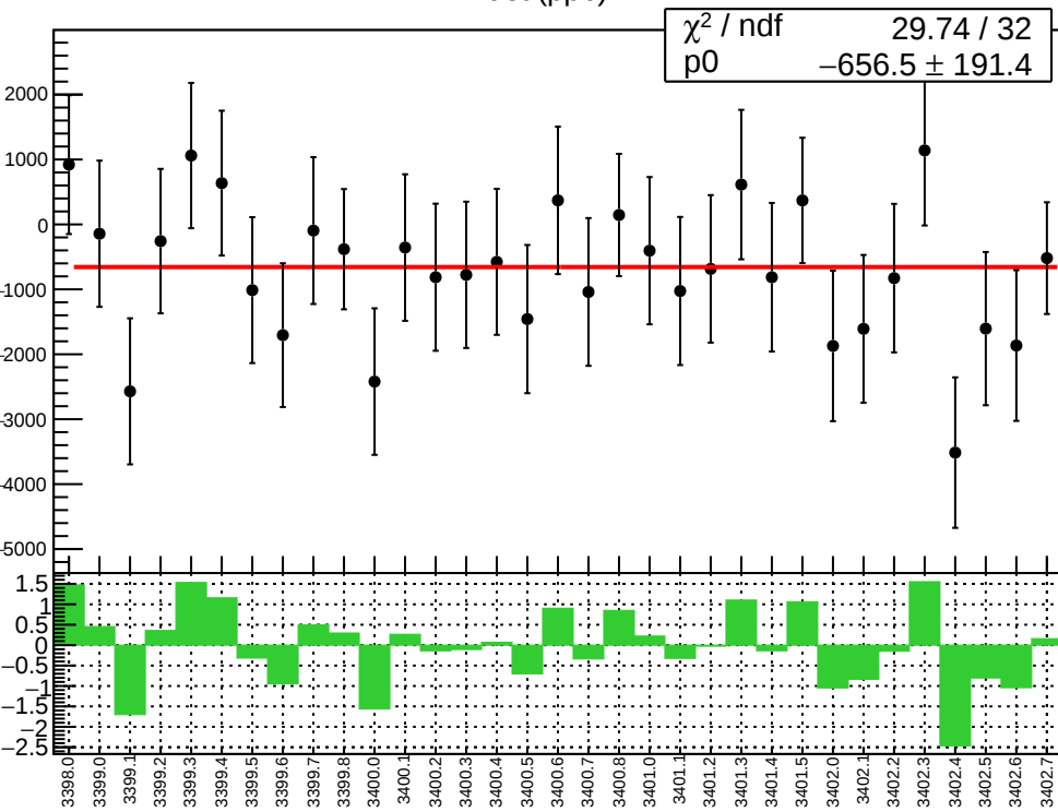
Adet (ppb)
