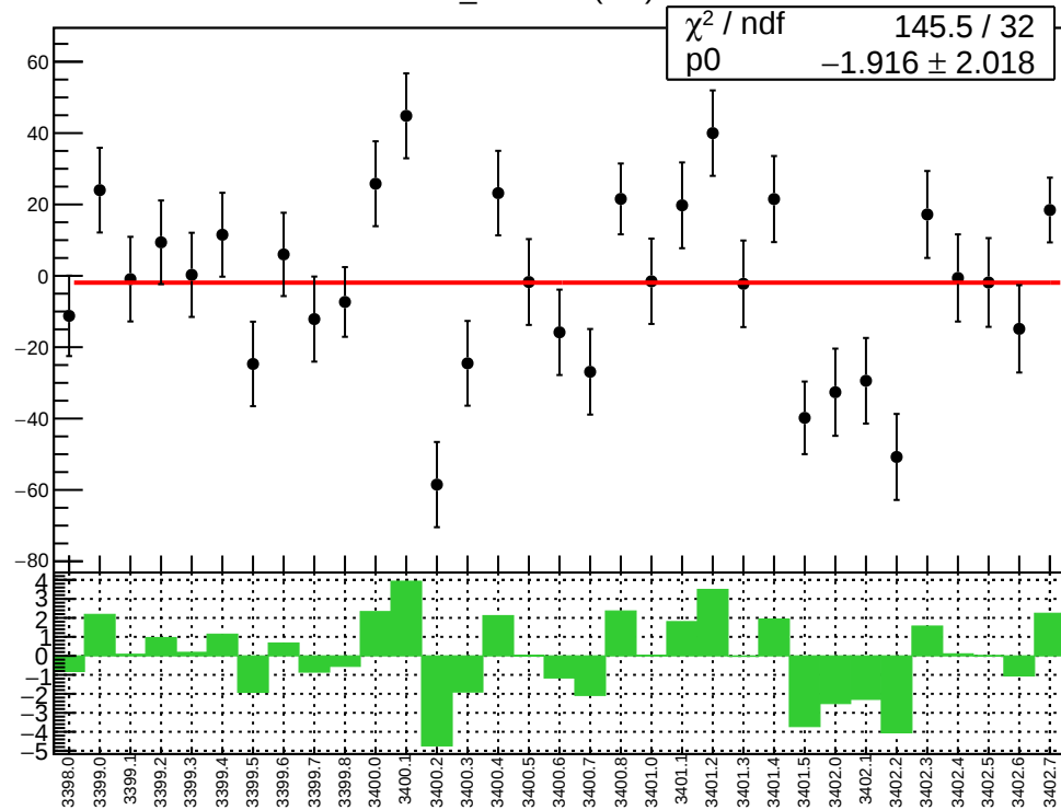
diff_evMon6 (nm)
