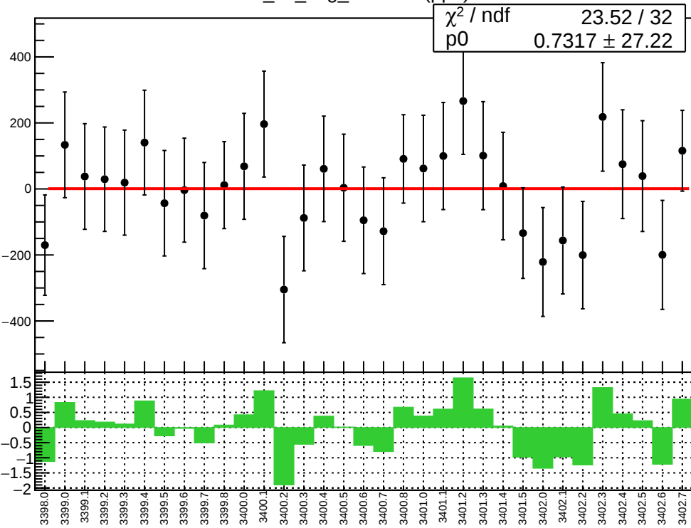
corr_us_avg_evMon7 (ppb)
