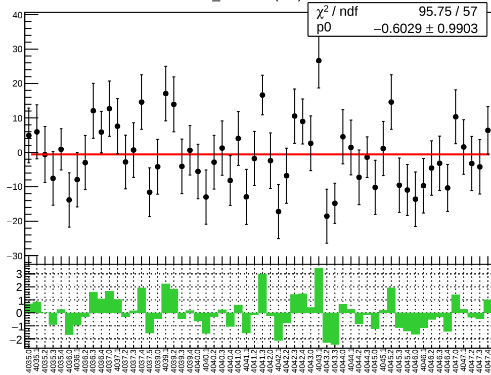
diff_evMon7 (nm)
