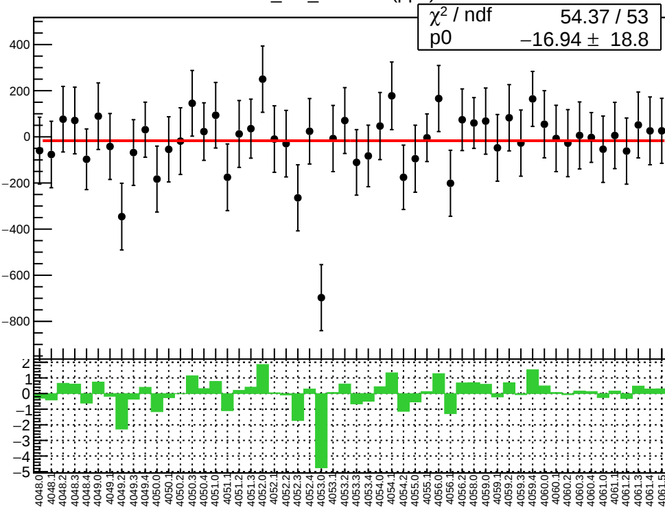
corr_usr_evMon6 (ppb)
