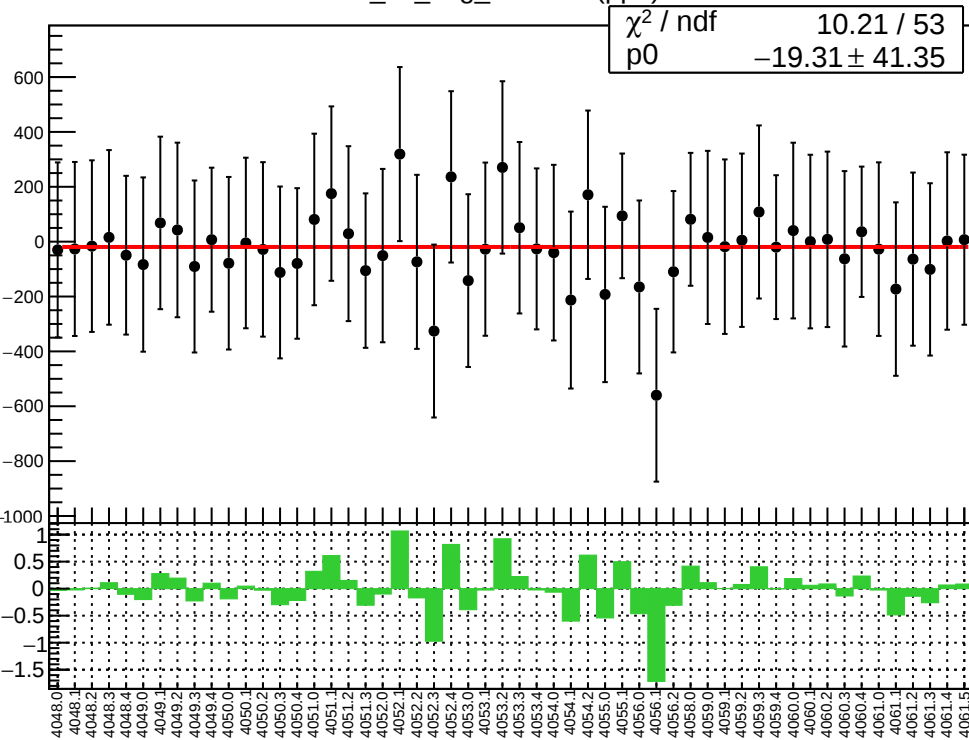
corr_us_avg_evMon3 (ppb)
