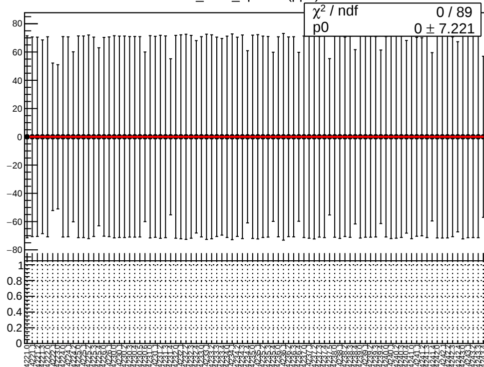
corr_Adet_bpm8Y (ppb)
