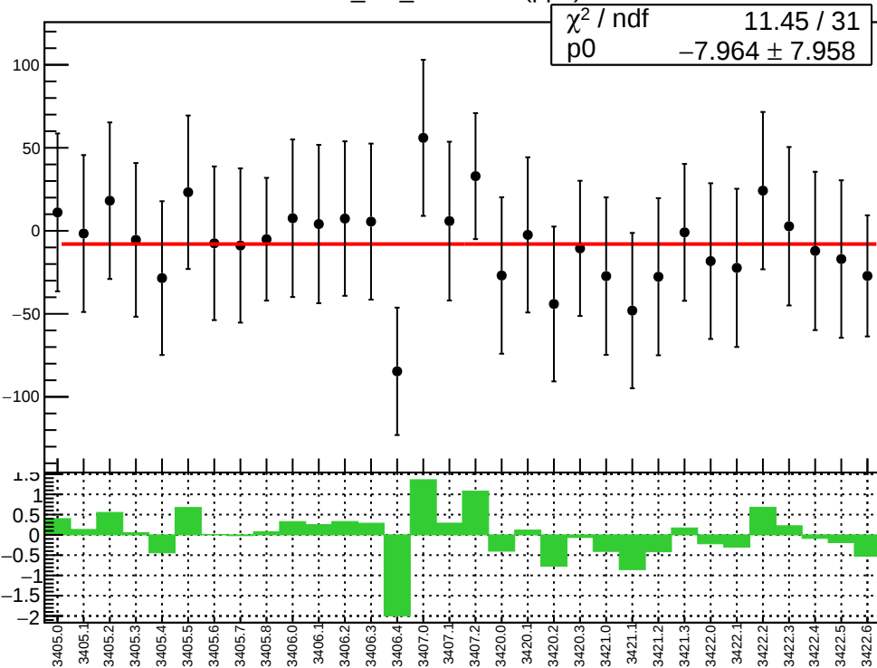
corr_usr_evMon11 (ppb)
