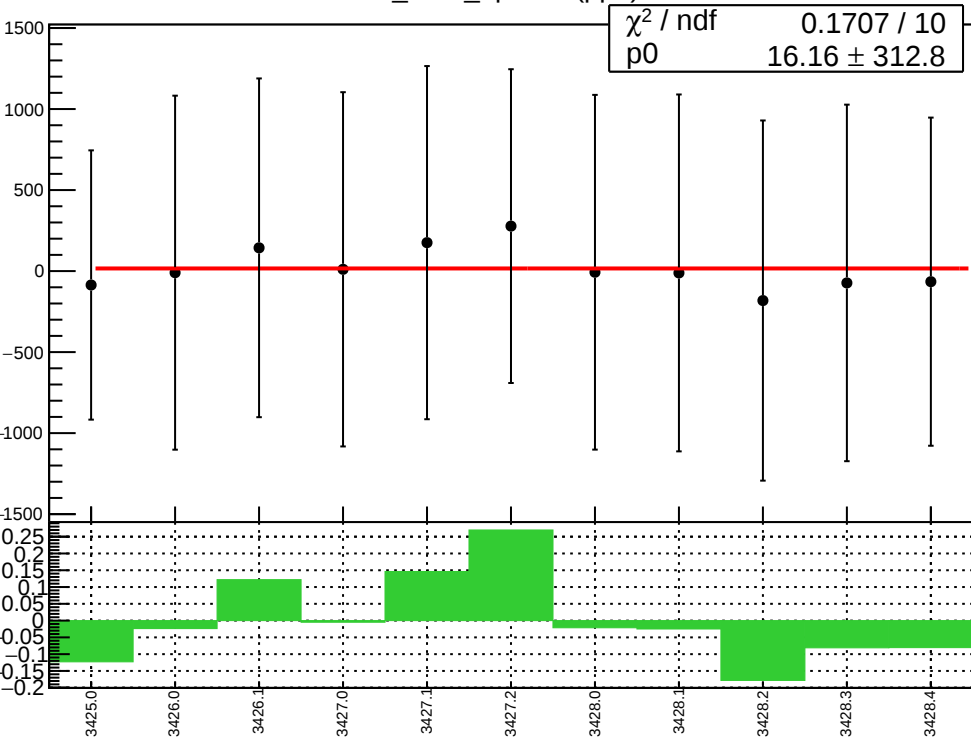
corr_Adet_bpm1X (ppb)
