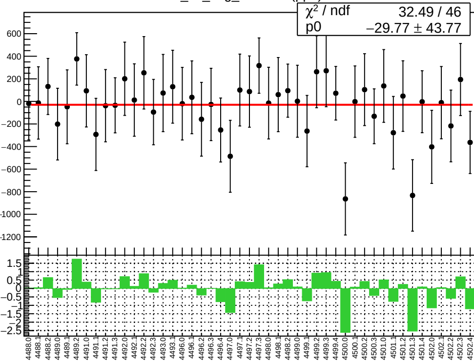
corr_us_avg_evMon3 (ppb)
