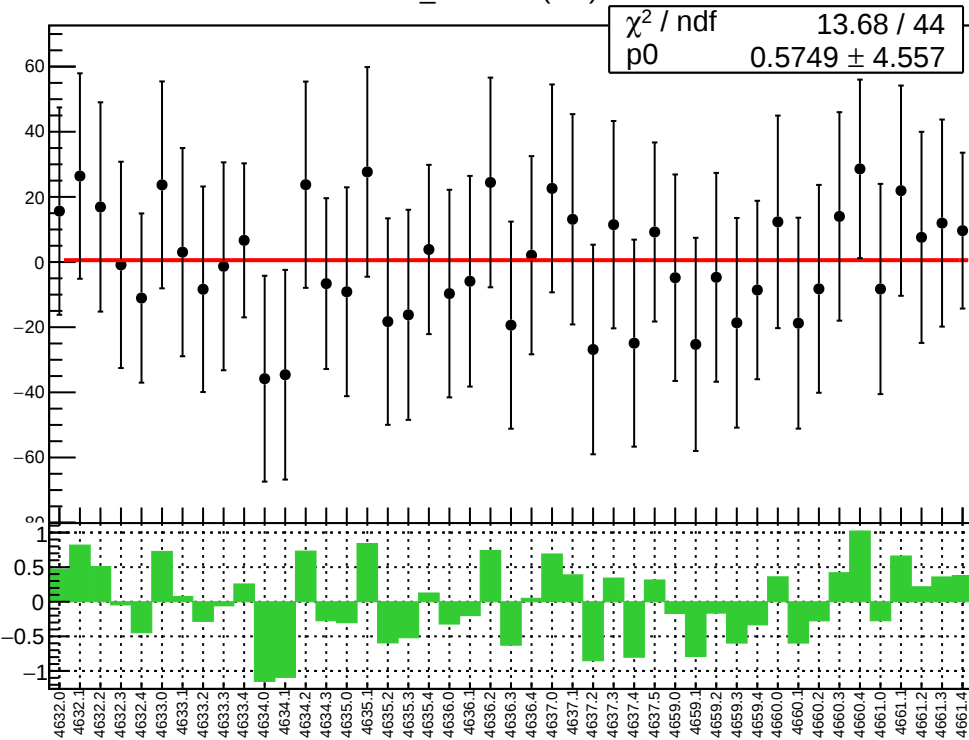
diff_evMon4 (nm)
