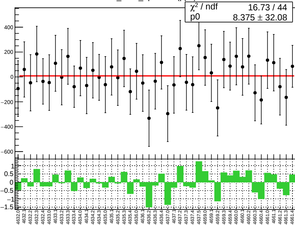
corr_Adet_bpm16Y (ppb)
