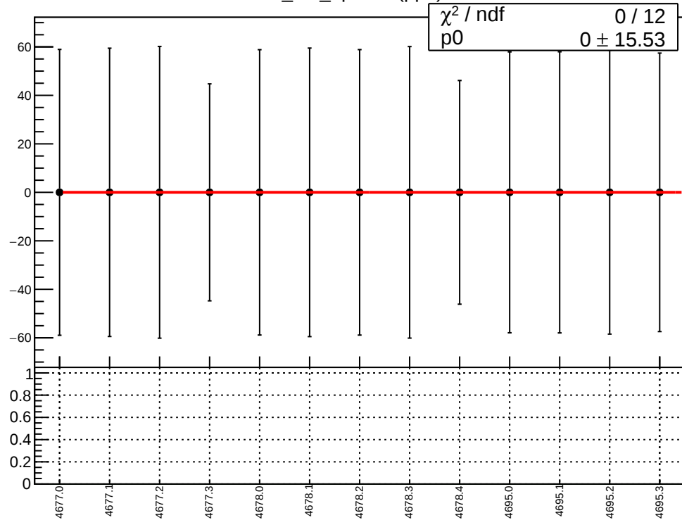
corr_usr_bpm8X (ppb)
