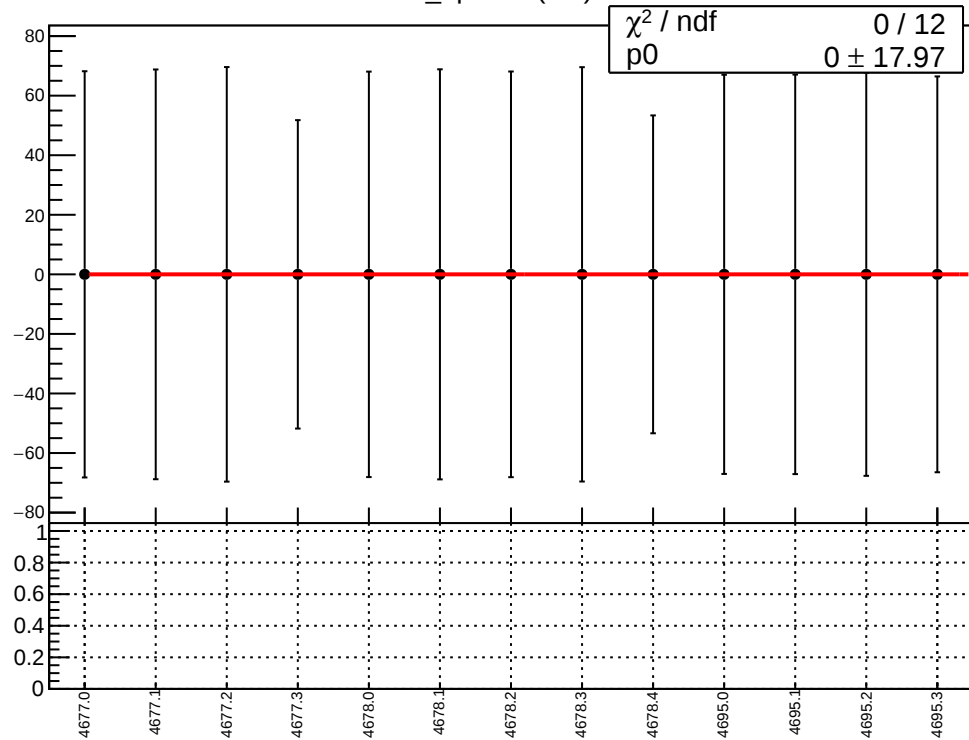
diff_bpm8X (nm)
