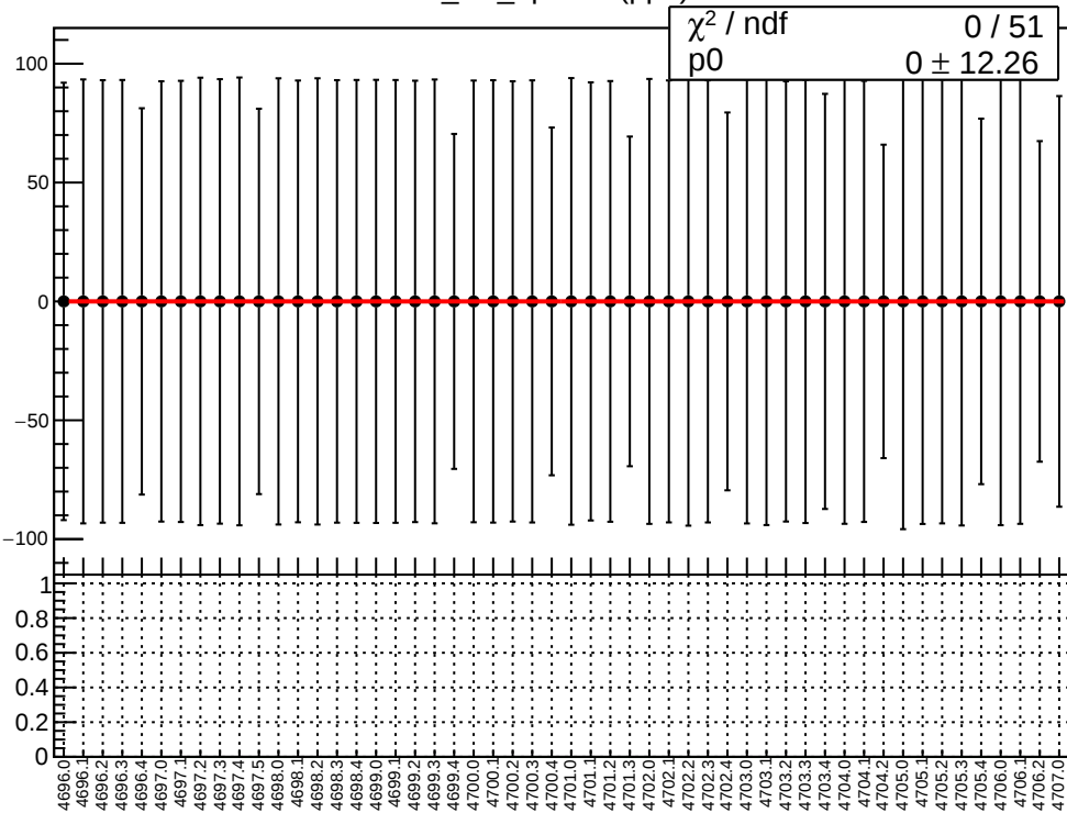
corr_usl_bpm8X (ppb)
