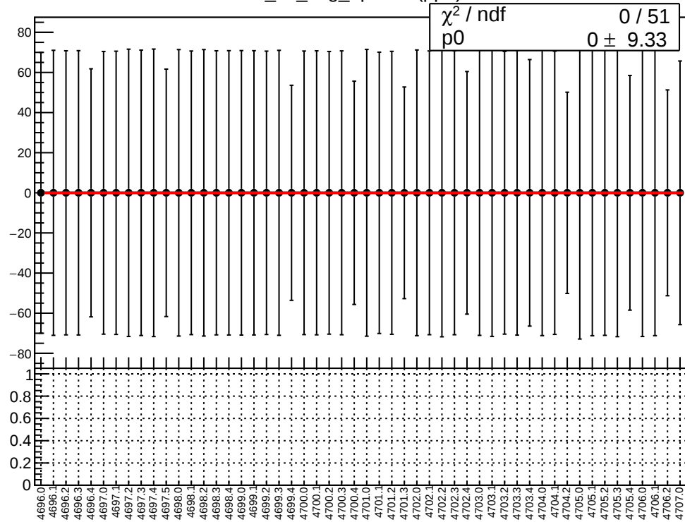
corr_us_avg_bpm8Y (ppb)
