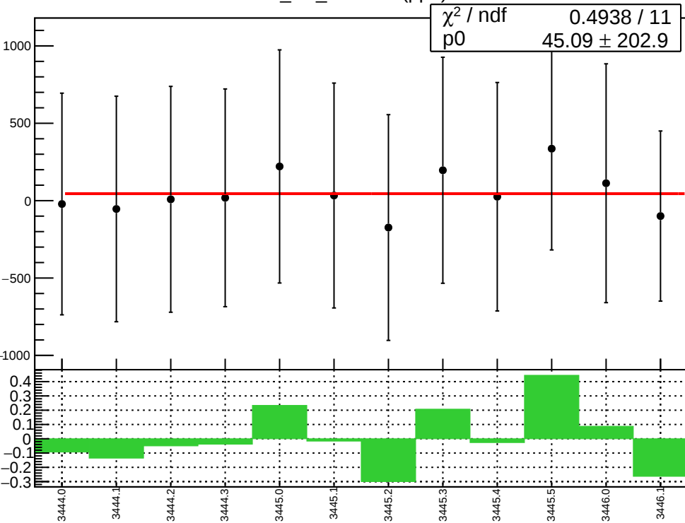
corr_usl_evMon1 (ppb)
