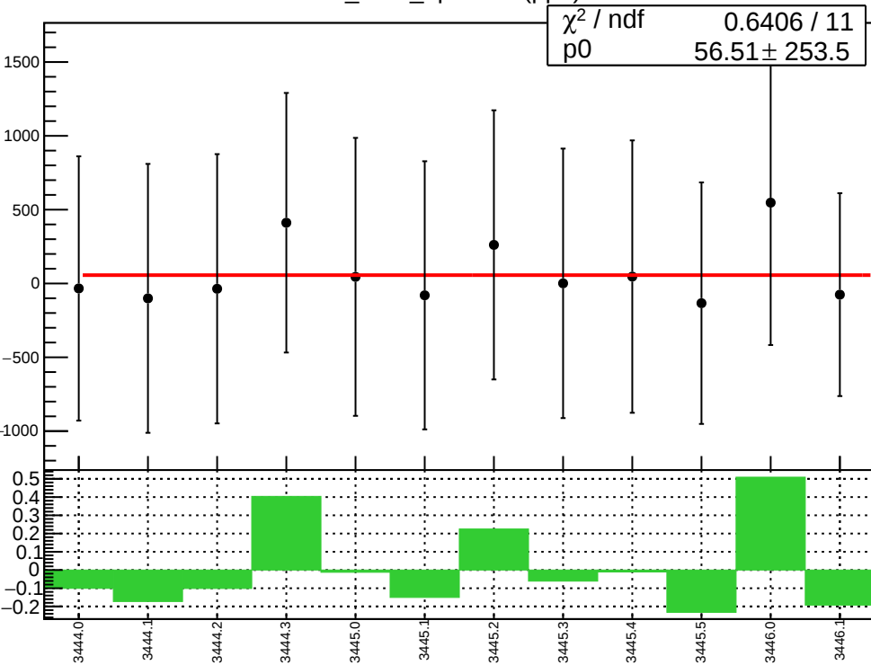
corr_Adet_bpm4eX (ppb)
