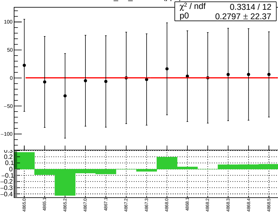
corr_usl_evMon8 (ppb)
