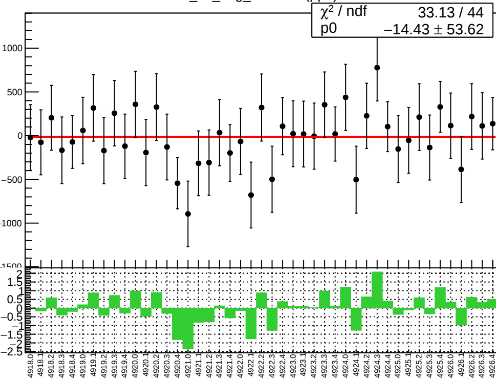
corr_us_avg_evMon4 (ppb)
