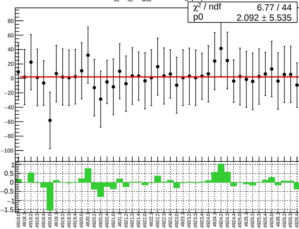
corr_us_avg_evMon8 (ppb)
