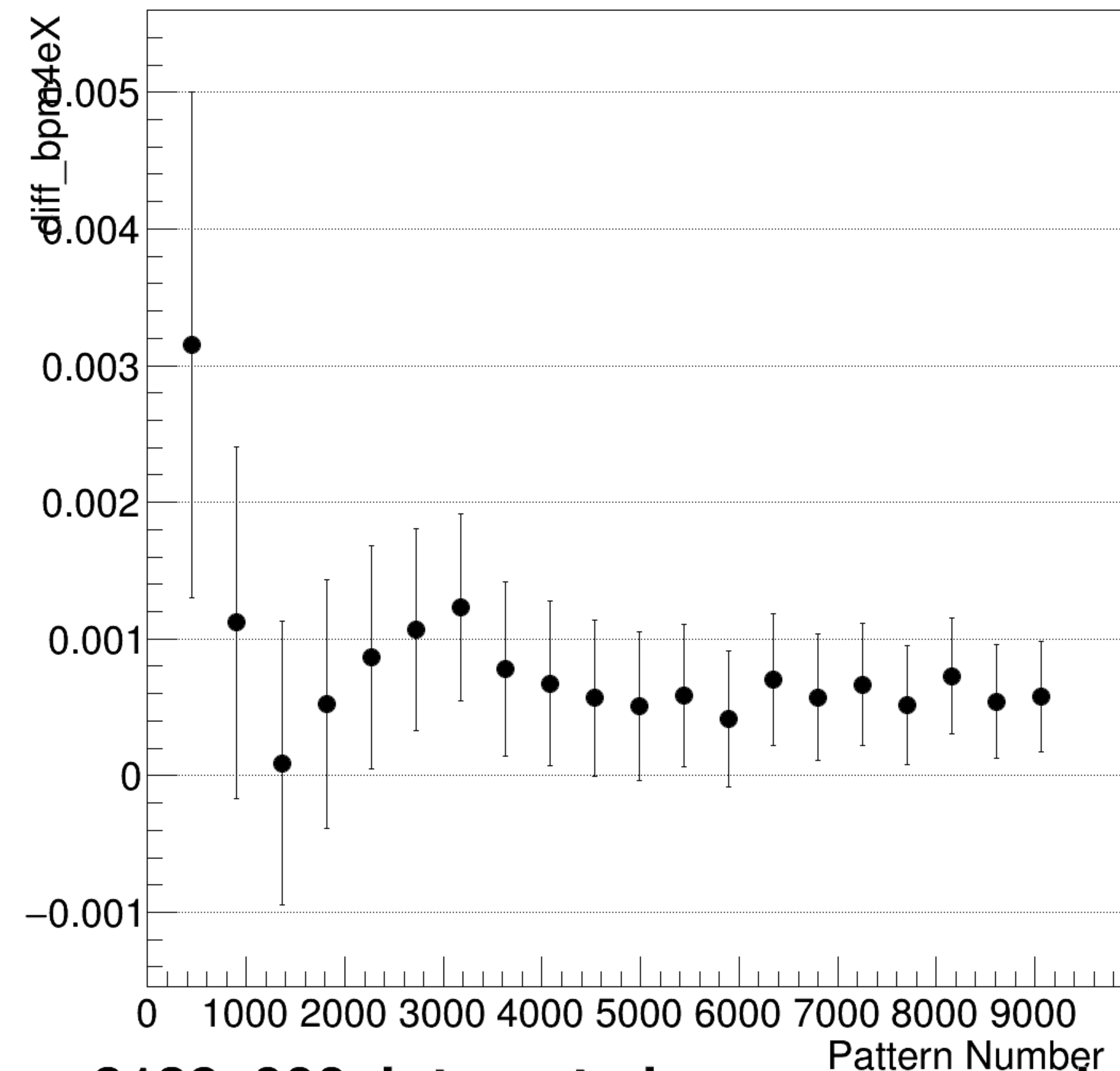
diff_bpm4eX Integrated Convergence
