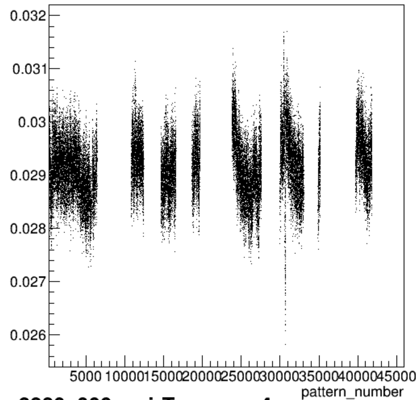
yield_sam4:pattern_number {ErrorFlag==0}
