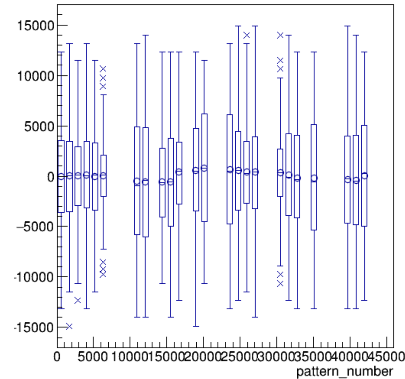
asym_sam6/ppm:pattern_number {ErrorFlag==0}
