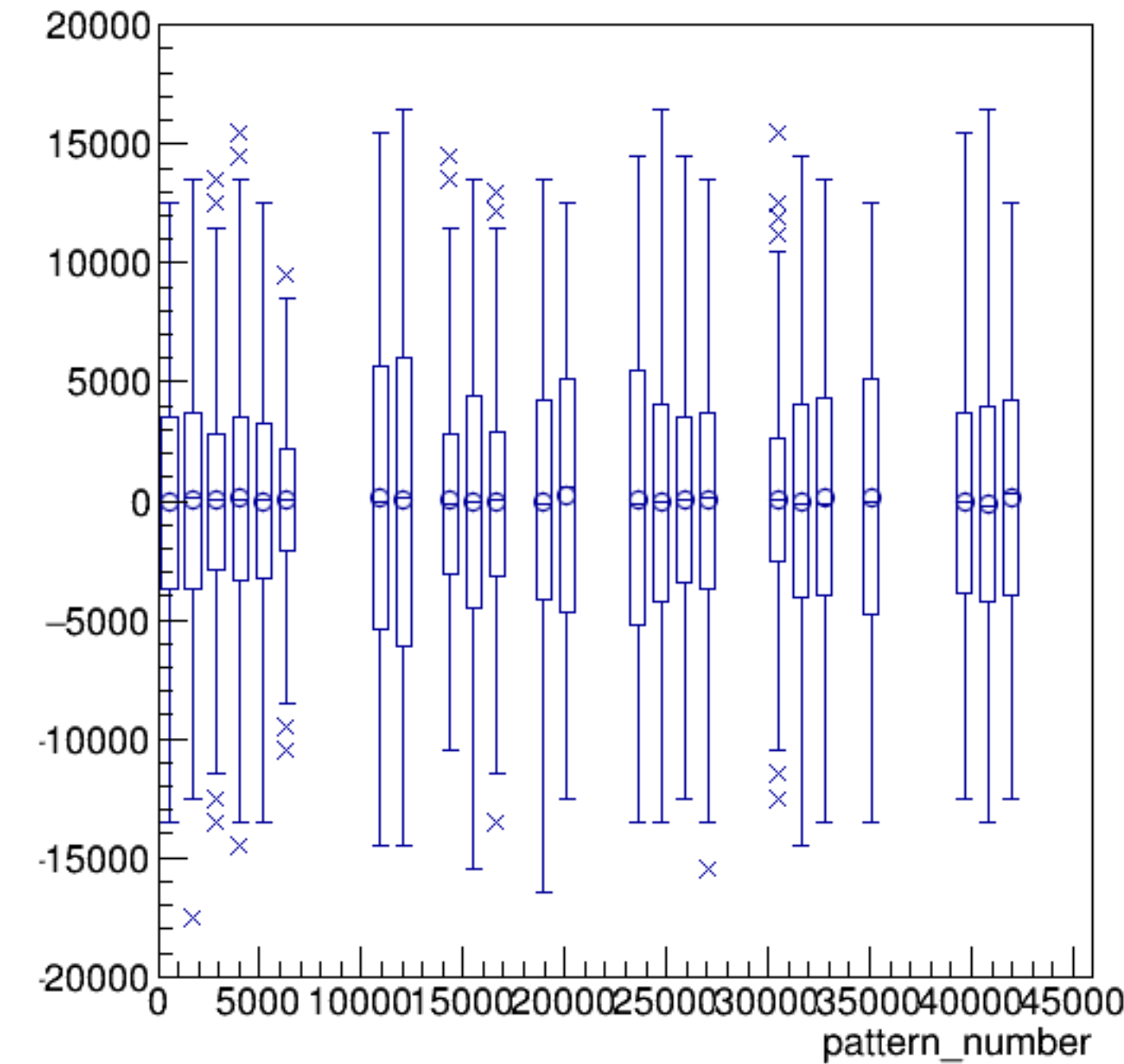
asym_sam7/ppm:pattern_number {ErrorFlag==0}
