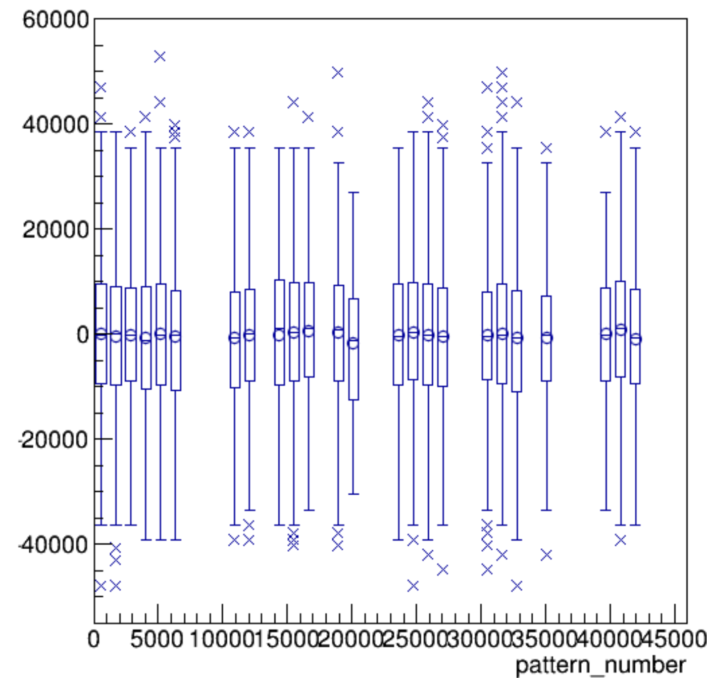
asym_sam3/ppm:pattern_number {ErrorFlag==0}
