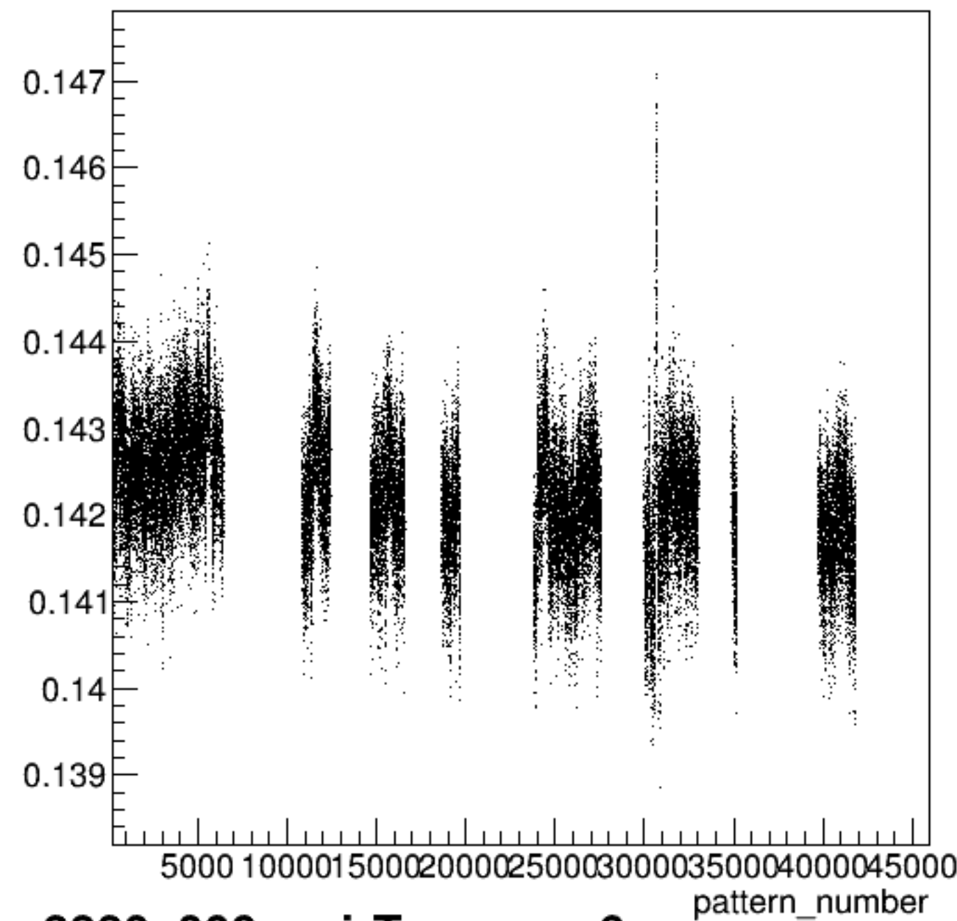
yield_sam6:pattern_number {ErrorFlag==0}
