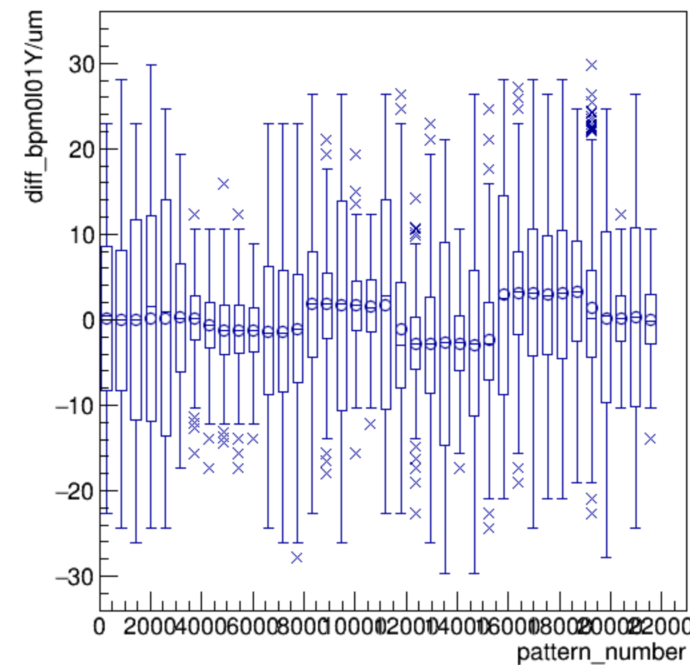
diff_bpm0l01Y/um:pattern_number {ErrorFlag==0}
