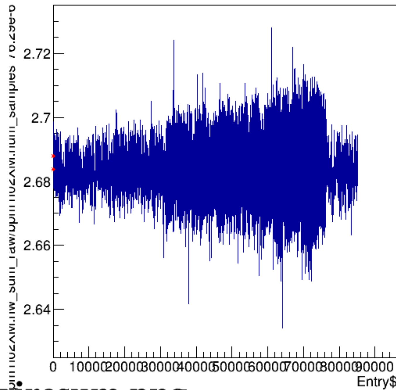
bpm1i02XM.hw_sum_raw/bpm1i02XM.num_samples*76.29e-6:Entry$
