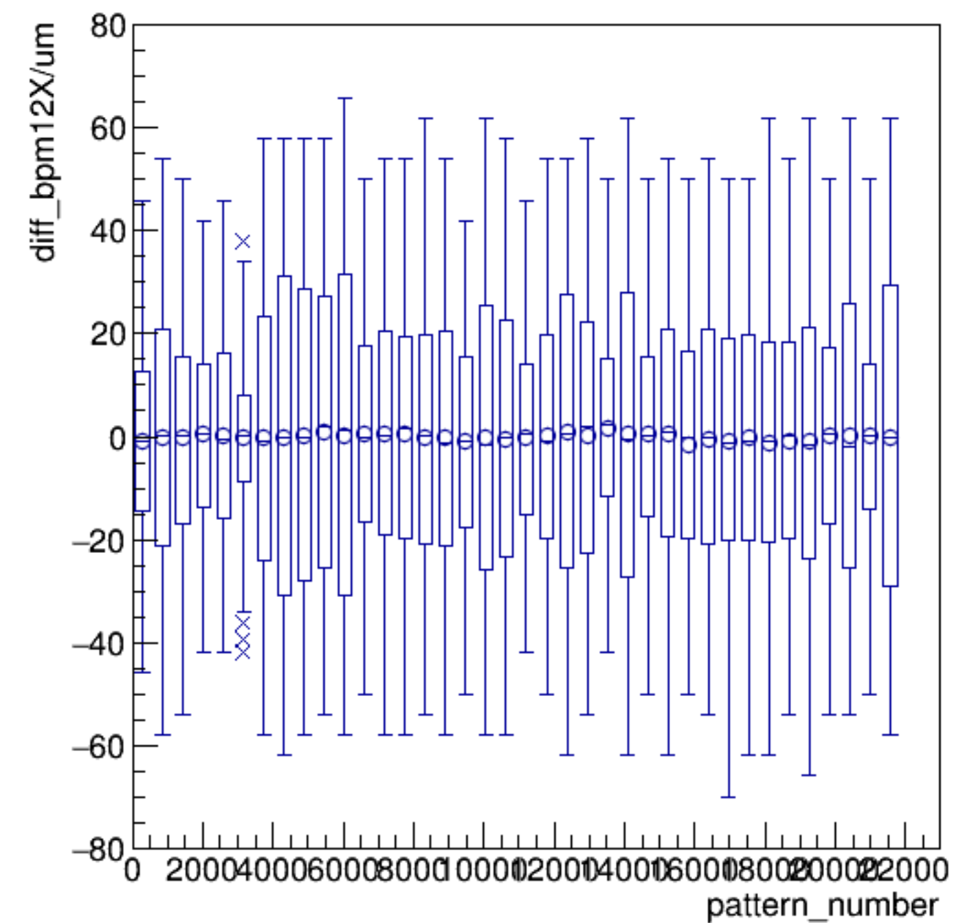
diff_bpm12X/um:pattern_number {ErrorFlag==0}
