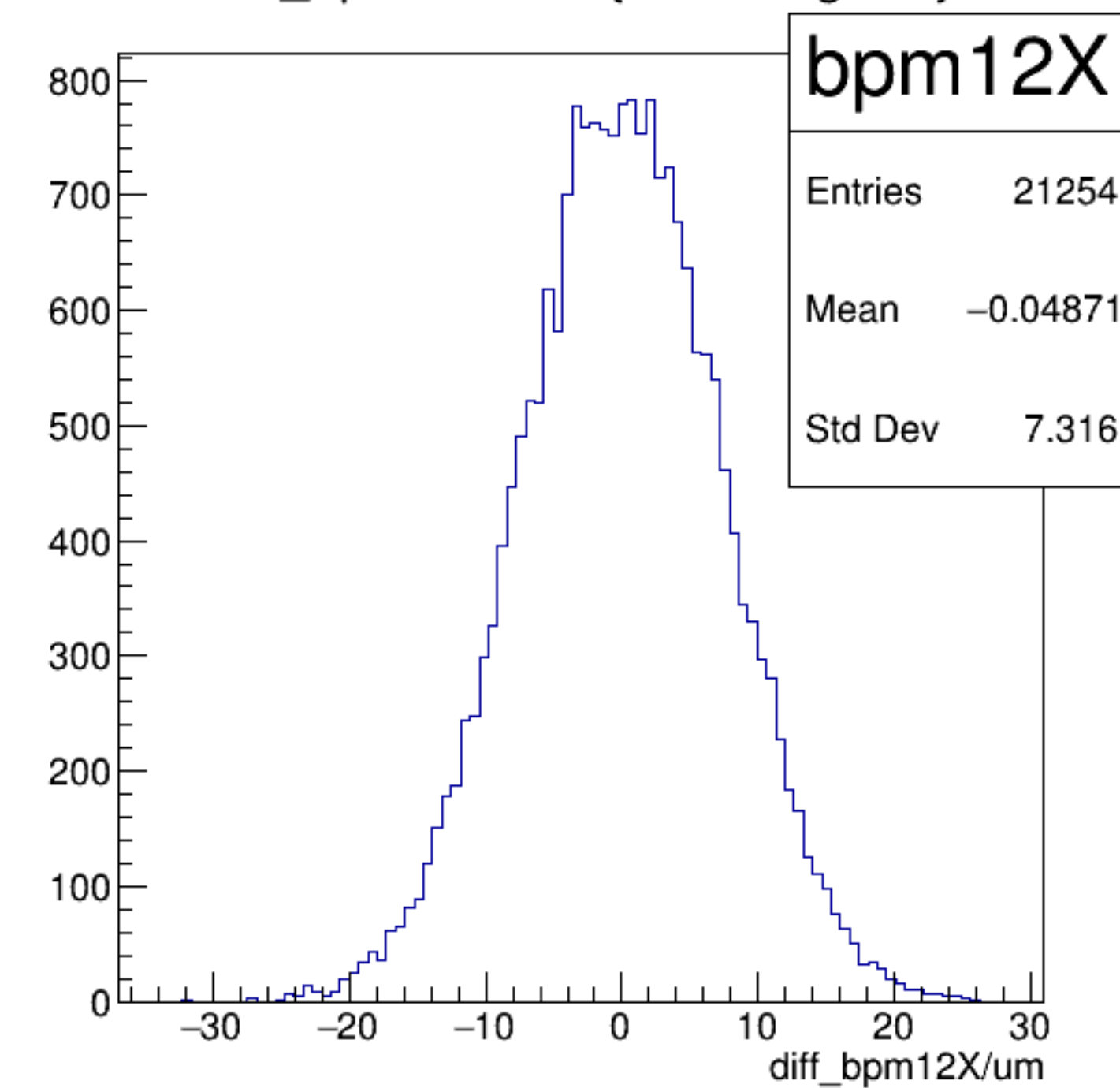
diff_bpm12X/um {ErrorFlag==0}
