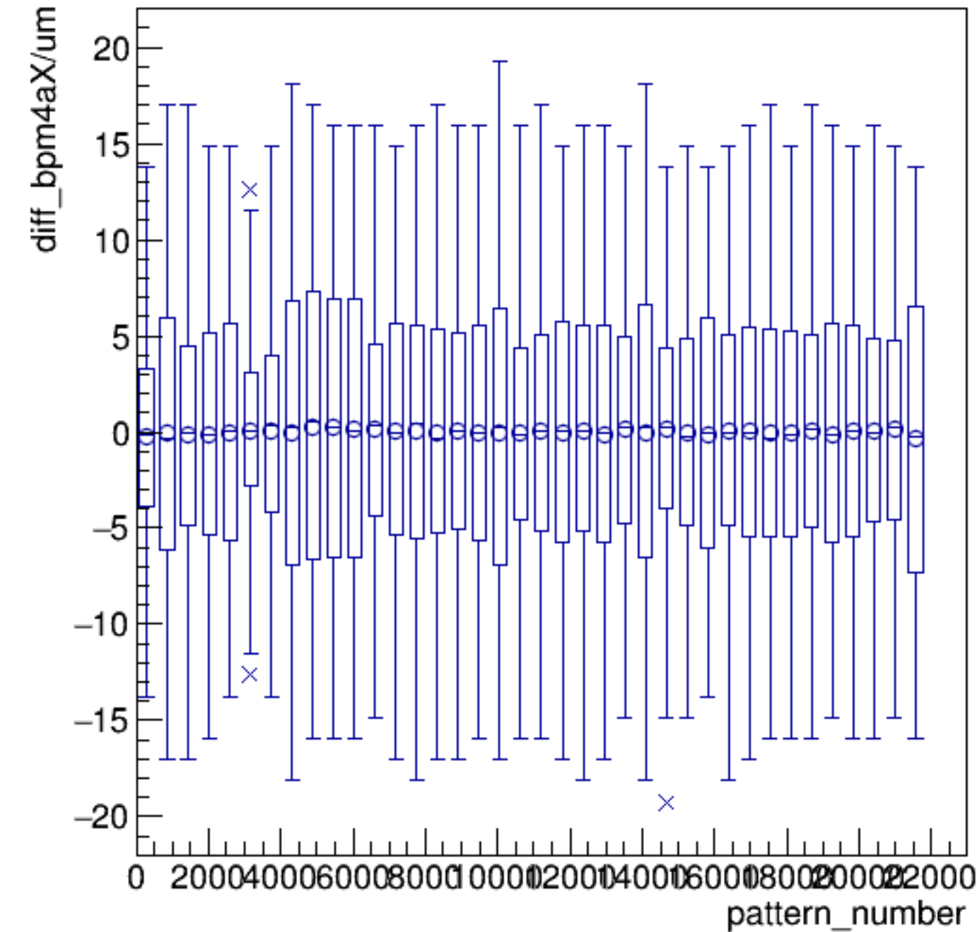
diff_bpm4aX/um:pattern_number {ErrorFlag==0}
