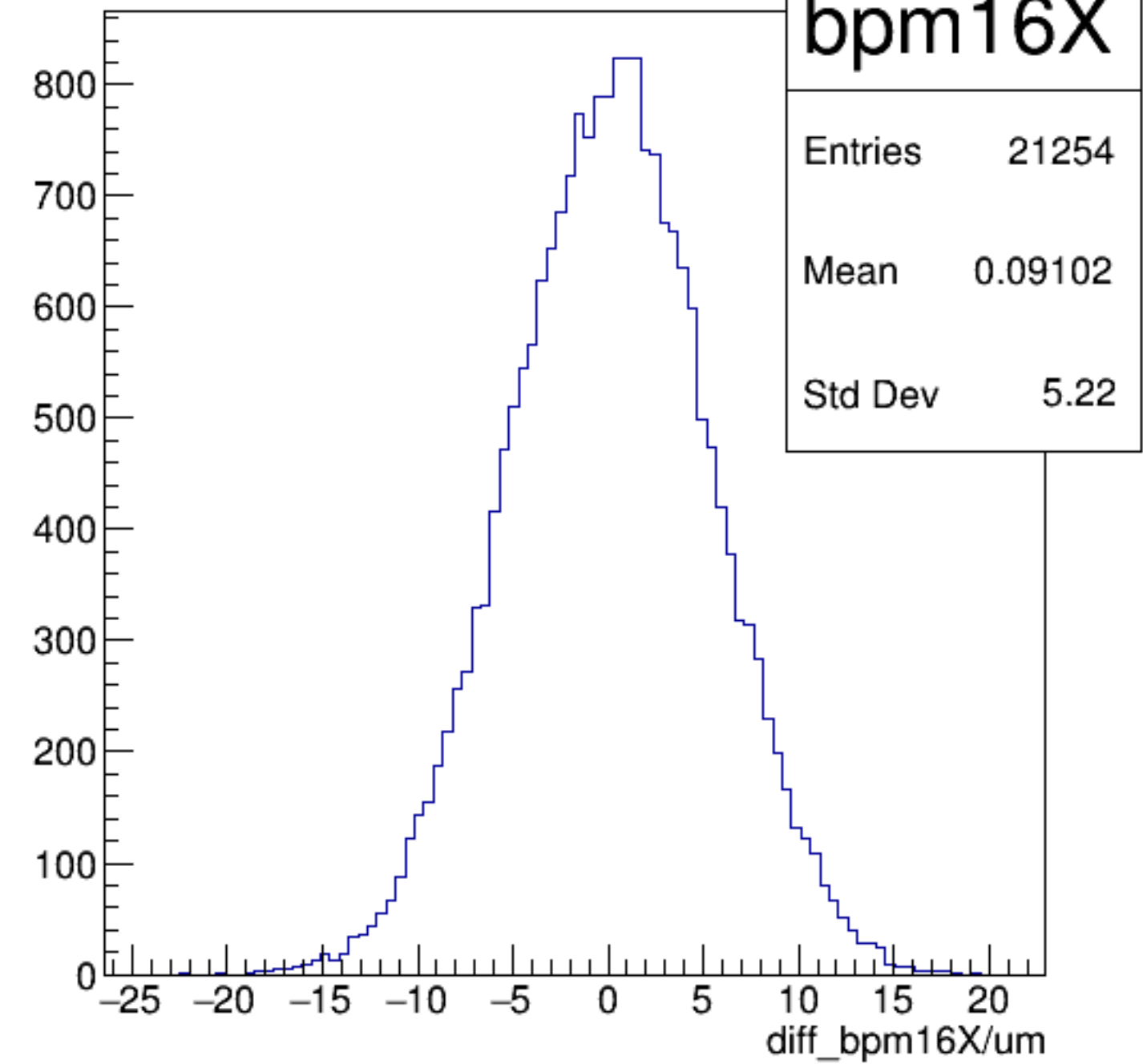
diff_bpm16X/um {ErrorFlag==0}
