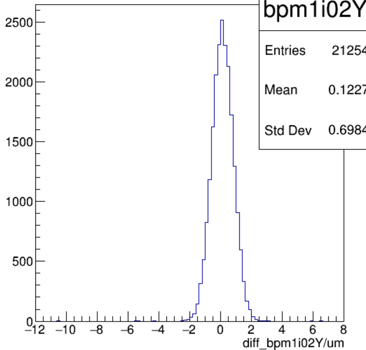
diff_bpm1i02Y/um {ErrorFlag==0}
