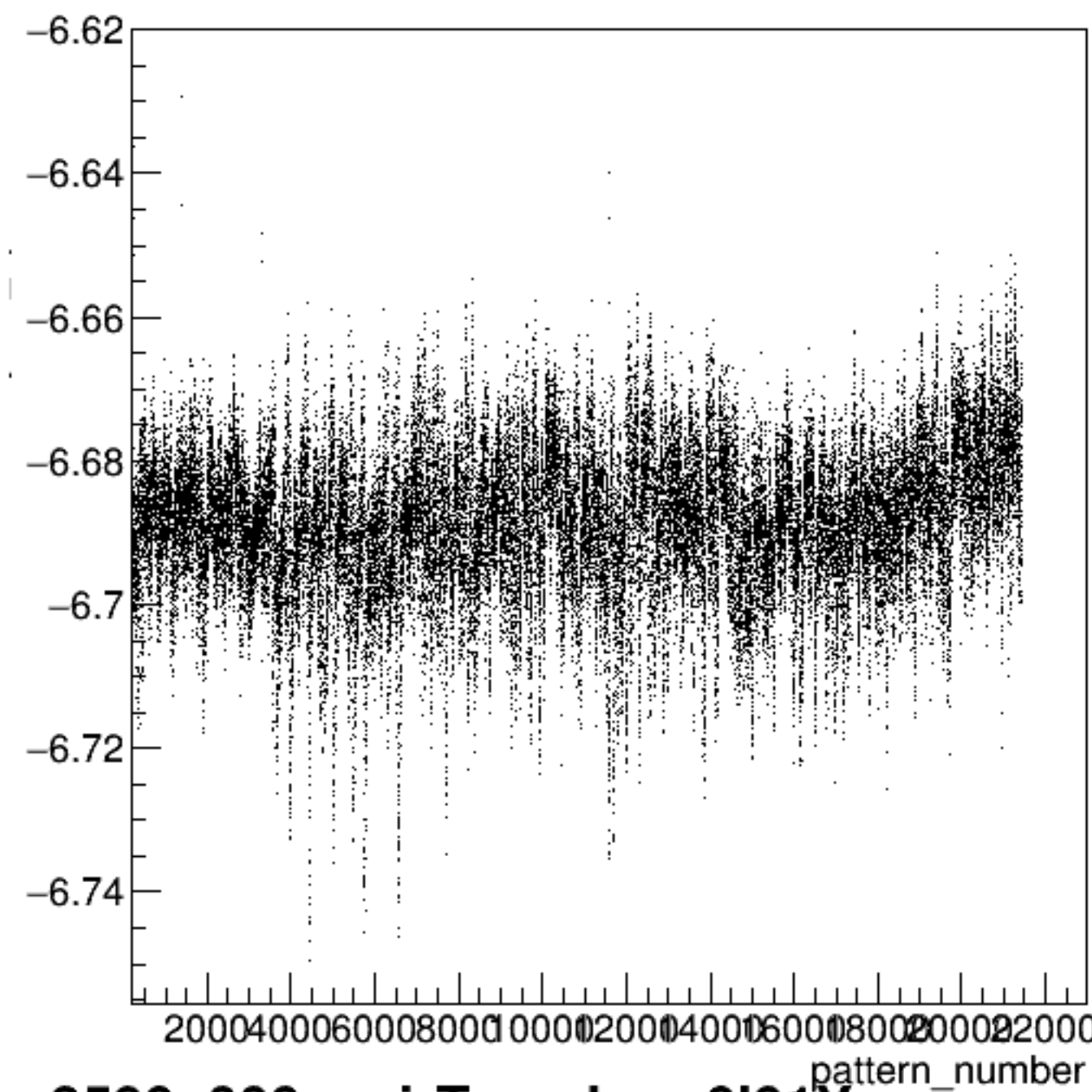
yield_bpm0l01Y/mm:pattern_number {ErrorFlag==0}
