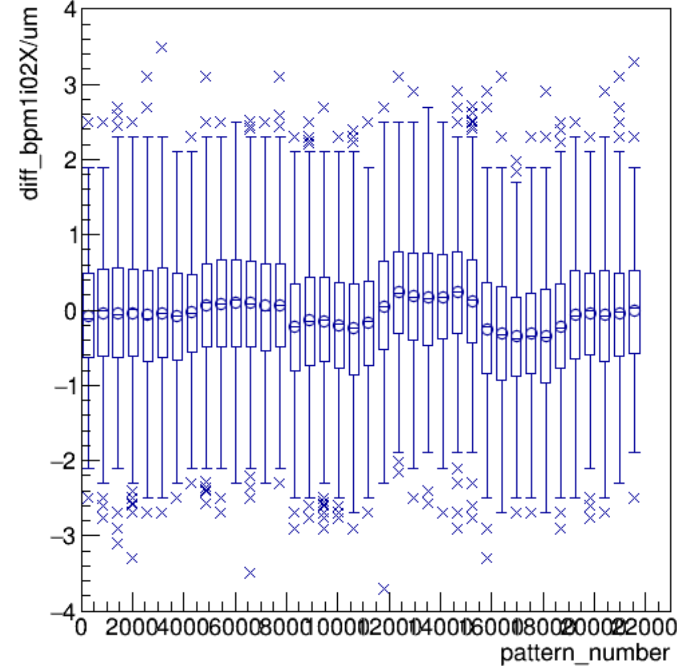
diff_bpm1i02X/um:pattern_number {ErrorFlag==0}
