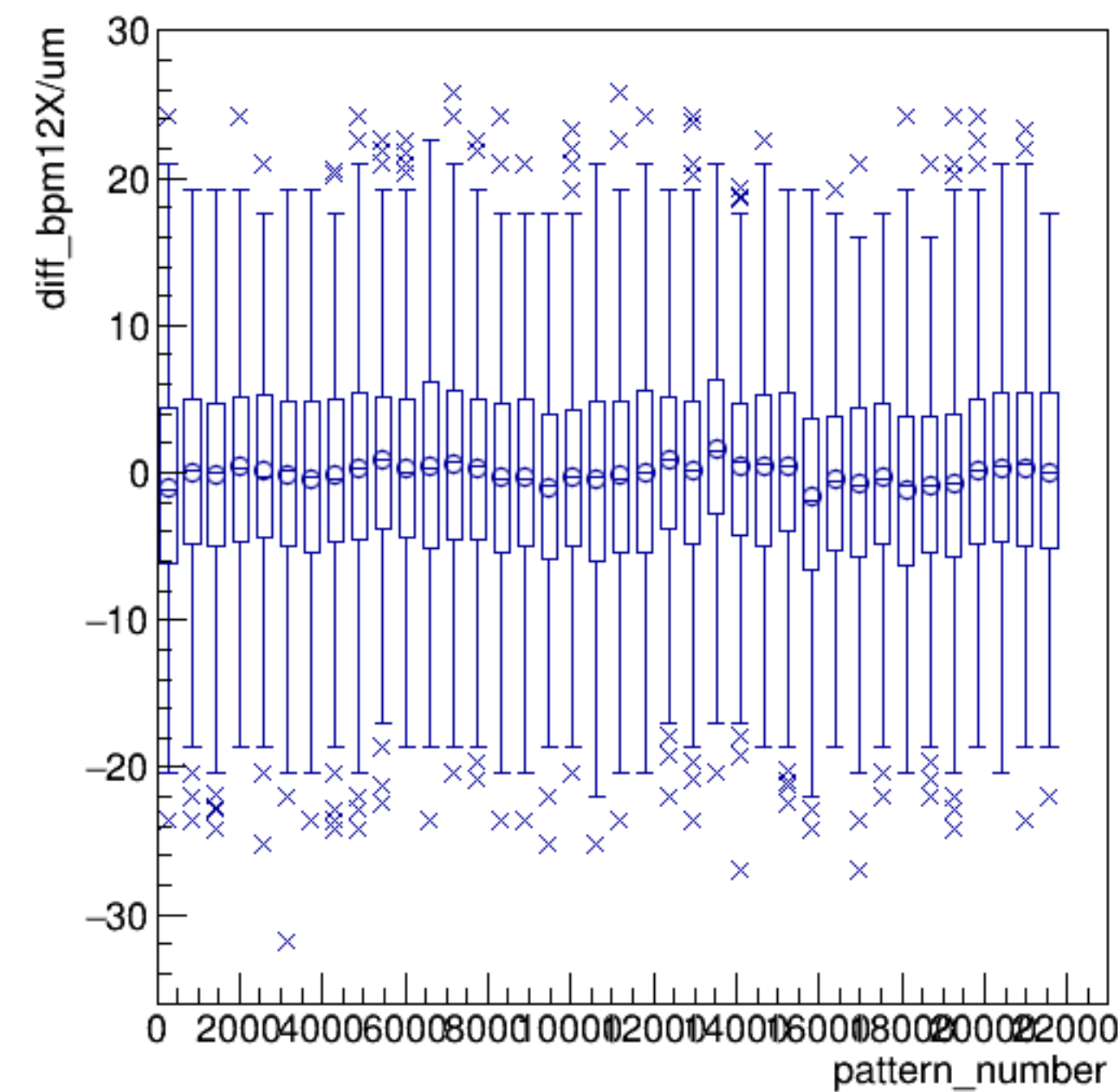
diff_bpm12X/um:pattern_number {ErrorFlag==0}
