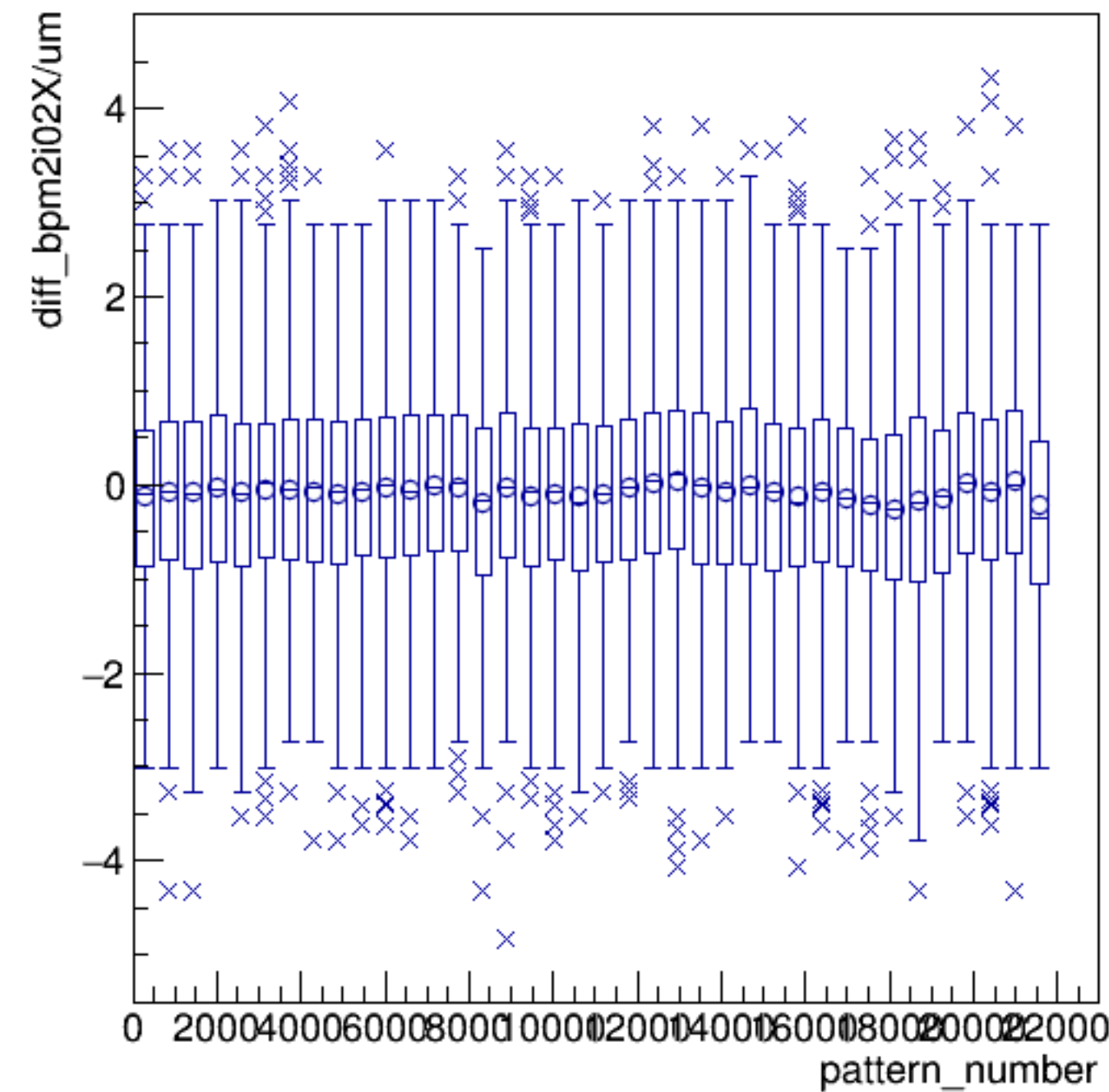
diff_bpm2i02X/um:pattern_number {ErrorFlag==0}
