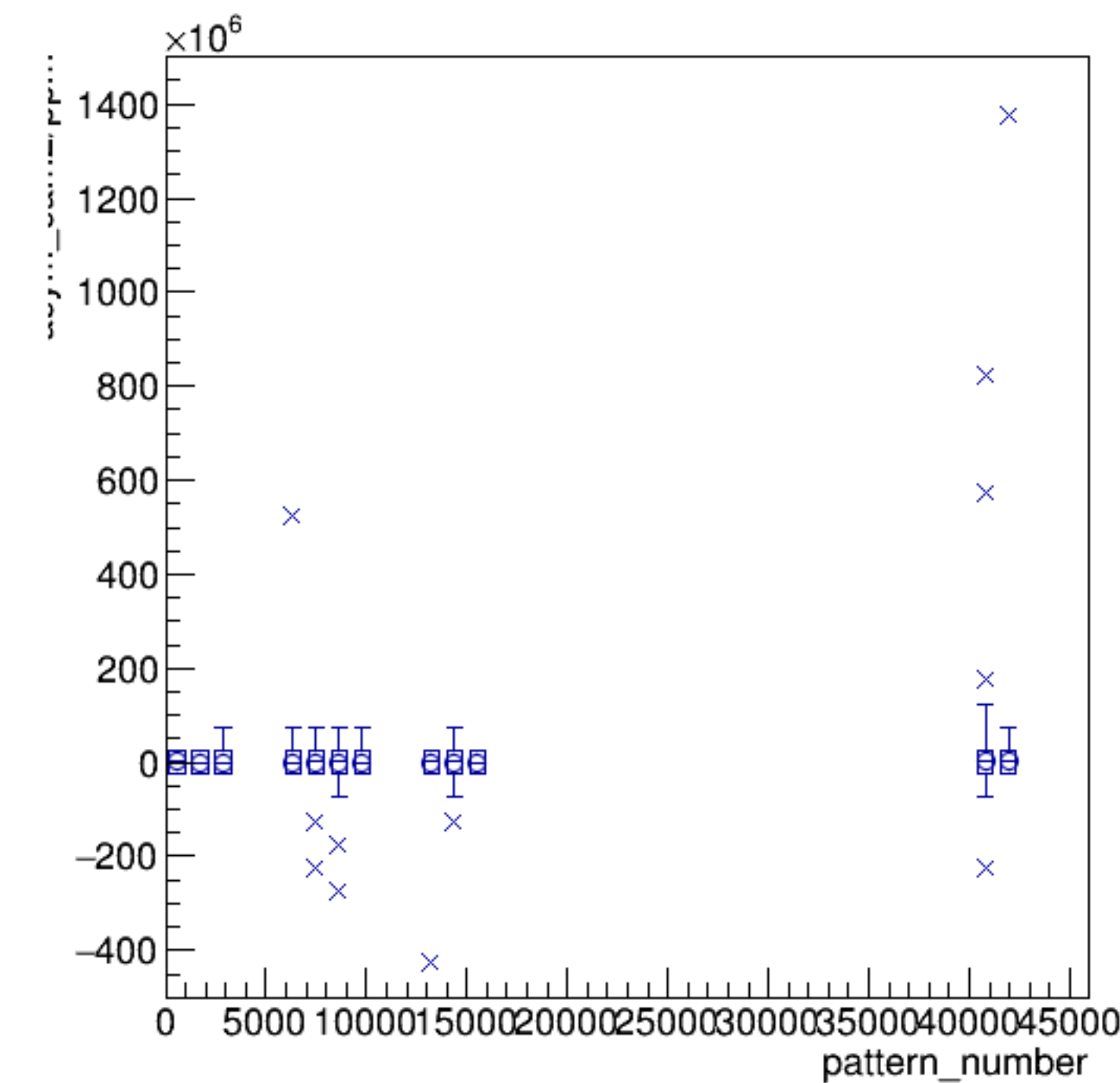
asym_sam2/ppm:pattern_number {ErrorFlag==0}
