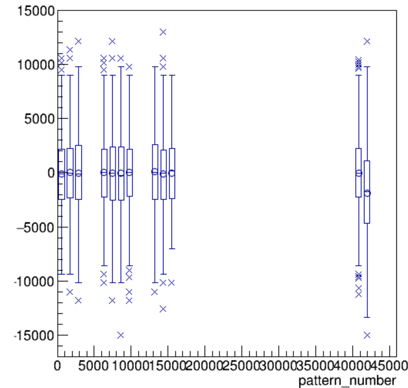
asym_sam5/ppm:pattern_number {ErrorFlag==0}
