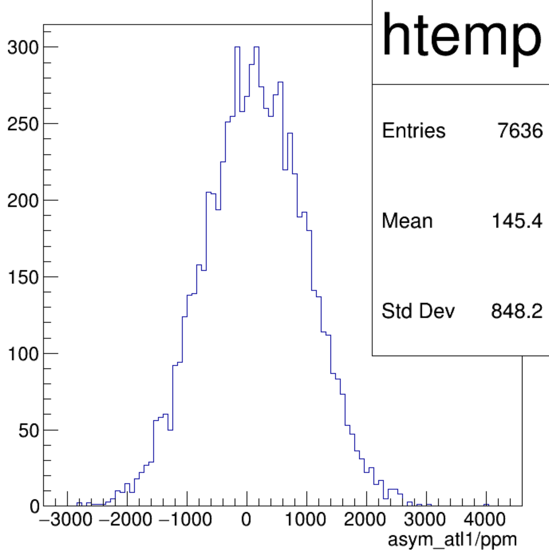
asym_atl1/ppm {ok_cut}
