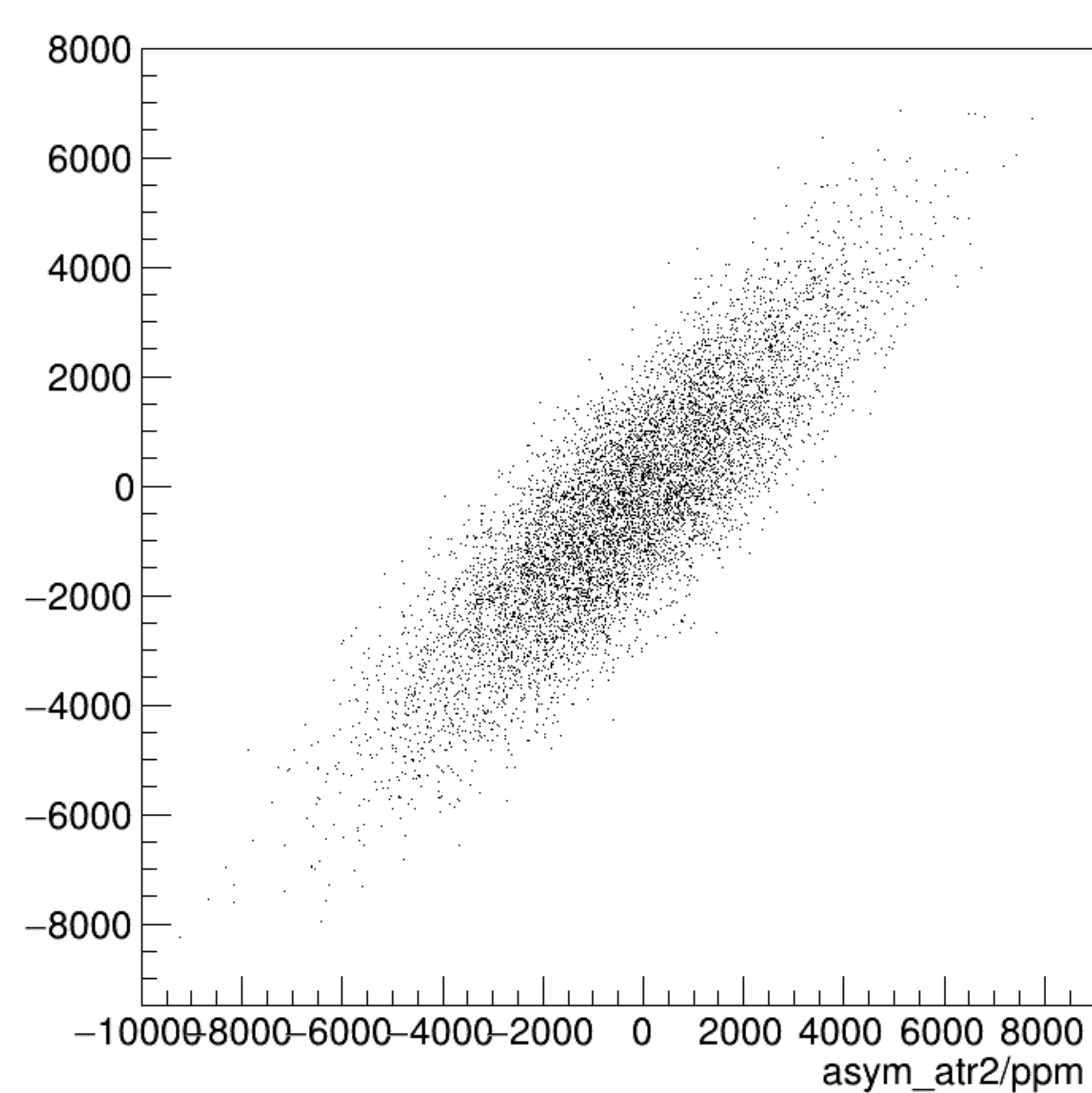
asym_atl2/ppm:asym_atr2/ppm {ok_cut}
