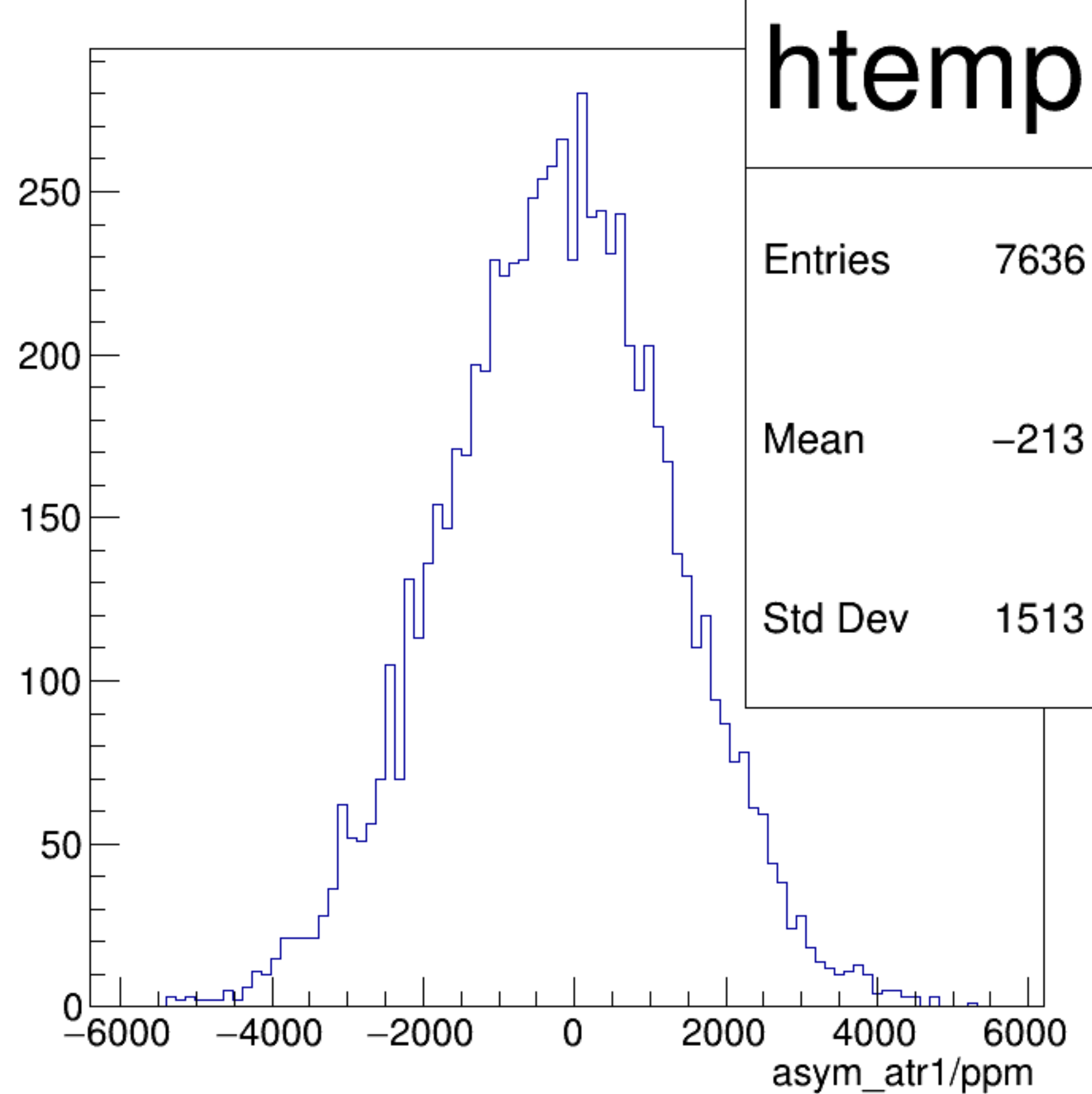
asym_atr1/ppm {ok_cut}
