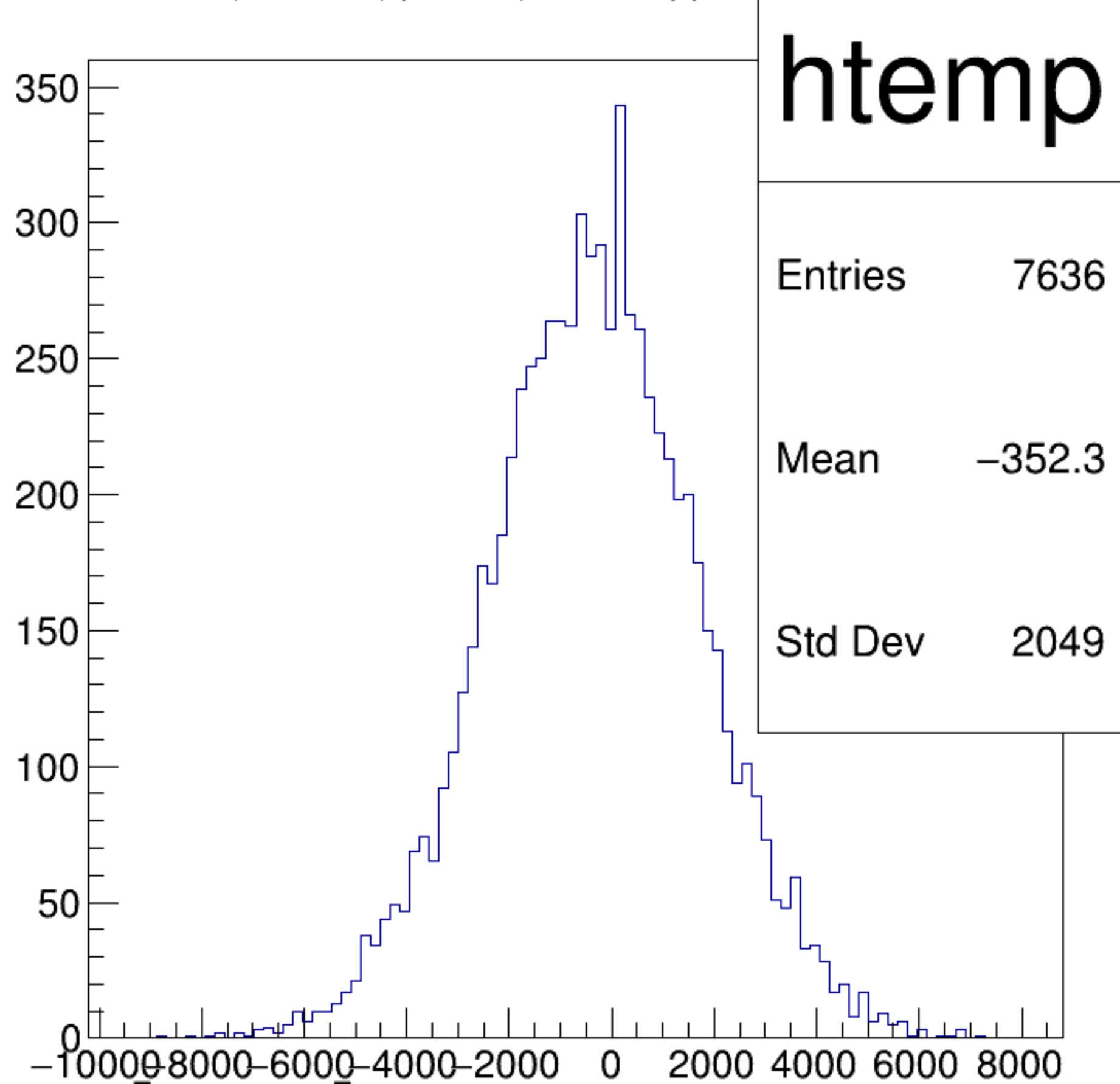
(asym_atl2/ppm+asym_atr2/ppm)/2 {ok_cut}
