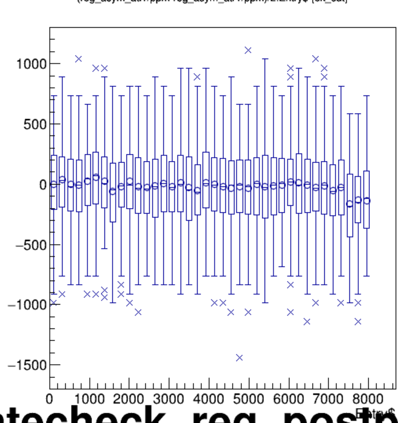
(reg_asym_atl1/ppm-reg_asym_atr1/ppm)/2:Entry$ {ok_cut}
