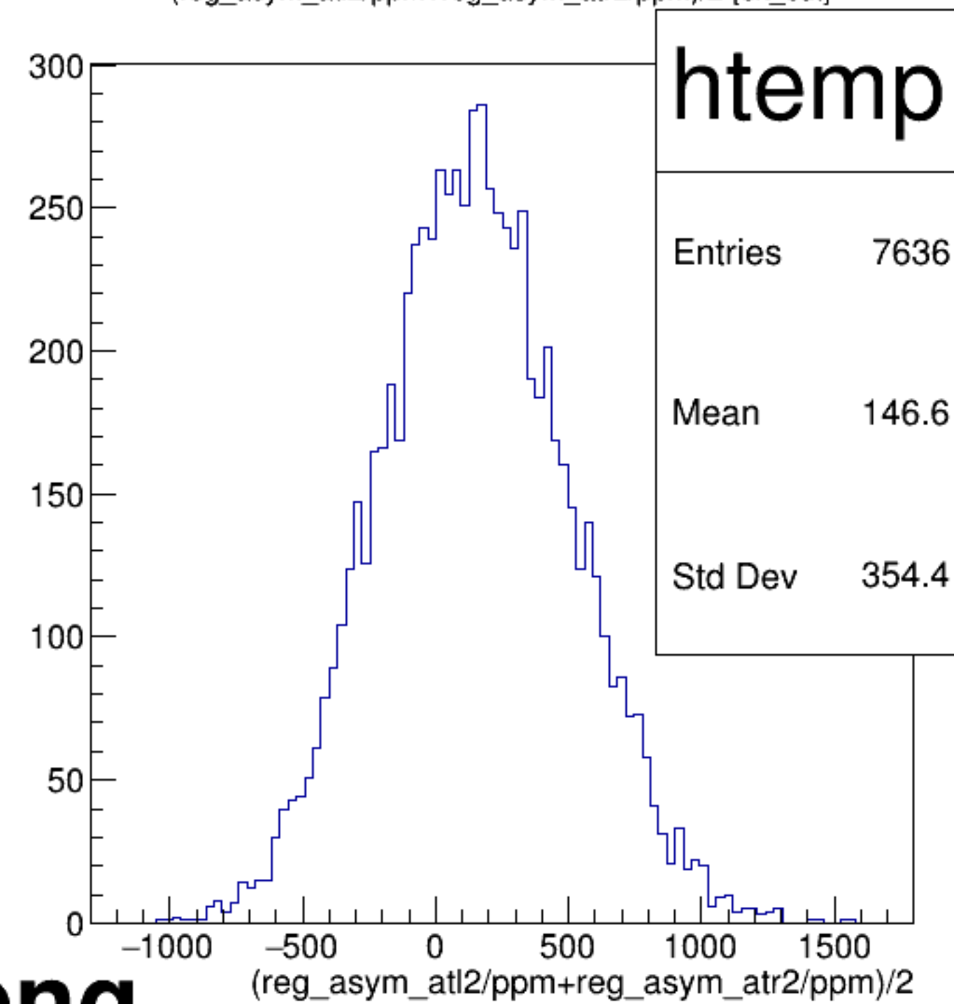
(reg_asym_atl2/ppm+reg_asym_atr2/ppm)/2 {ok_cut}
