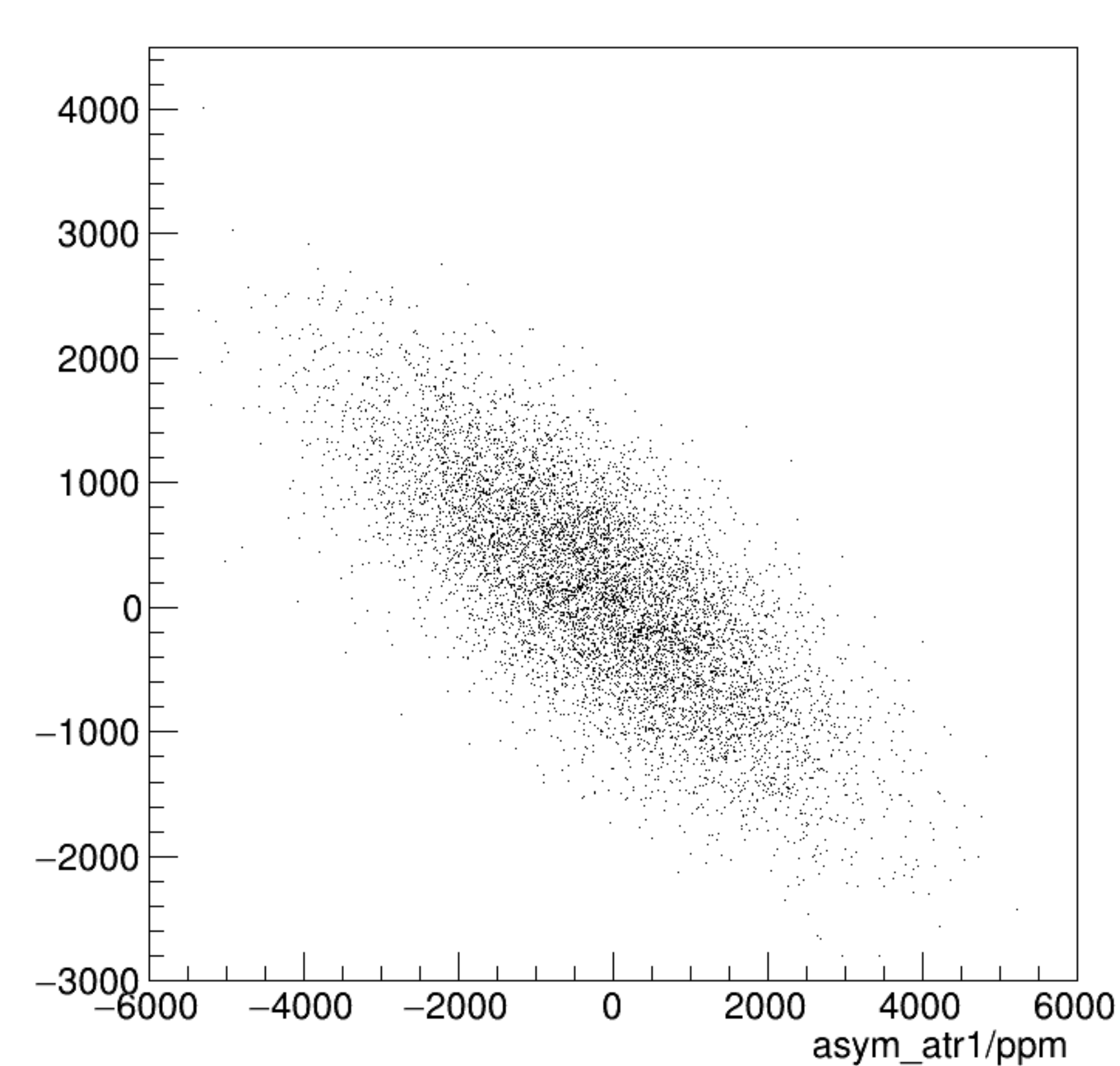
asym_atl1/ppm:asym_atr1/ppm {ok_cut}
