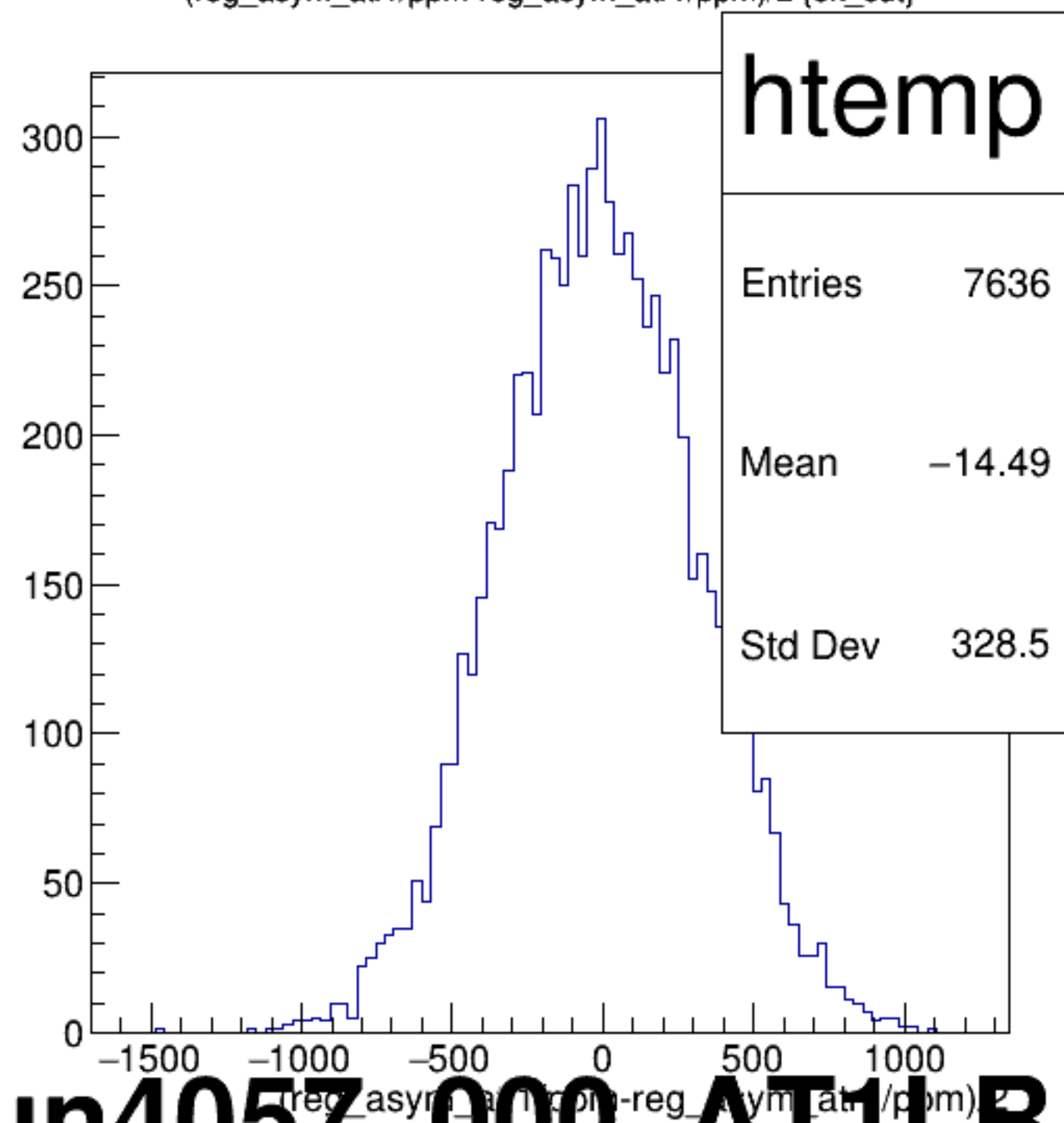
(reg_asym_atl1/ppm-reg_asym_atr1/ppm)/2 {ok_cut}
