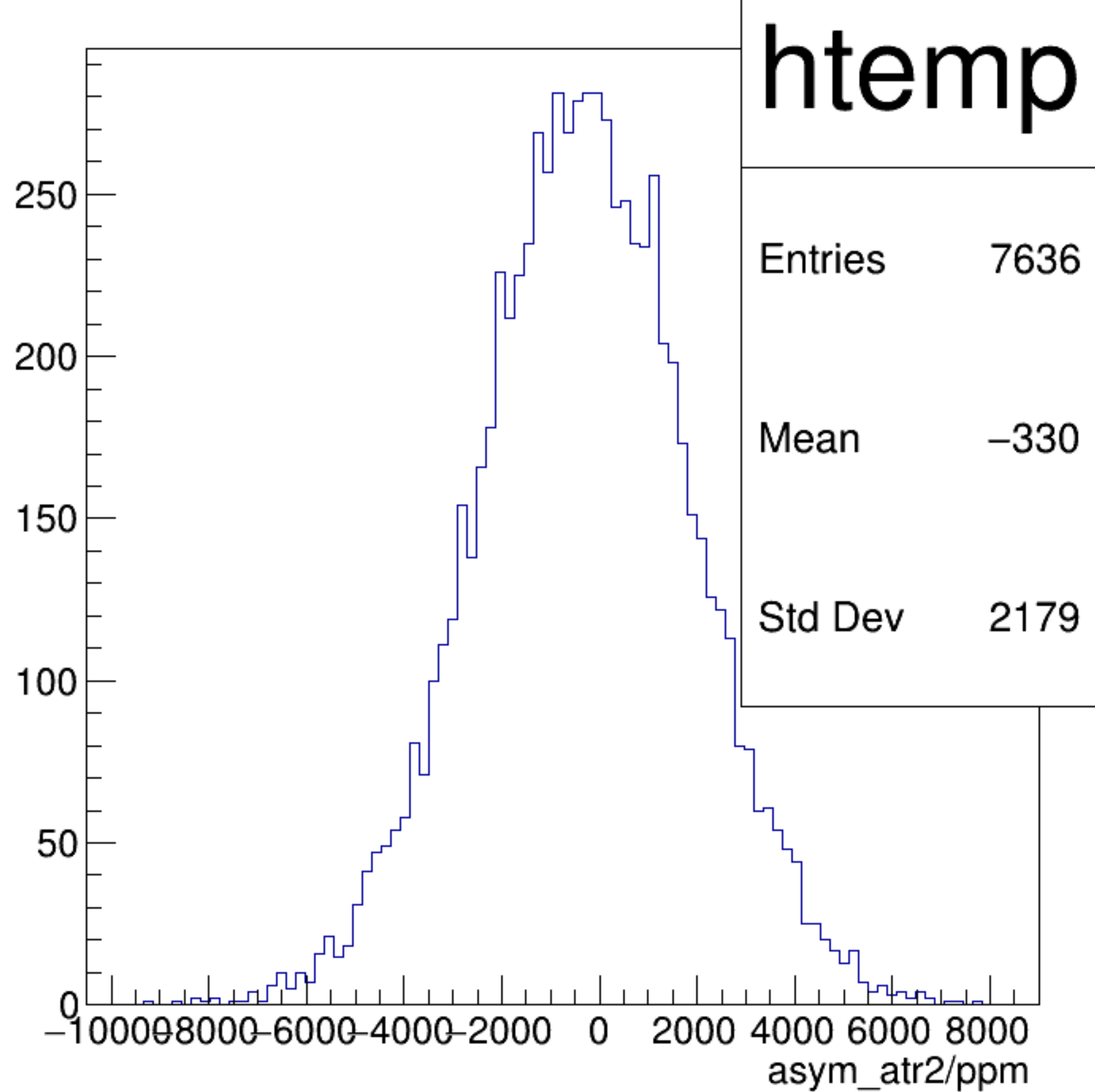
asym_atr2/ppm {ok_cut}
