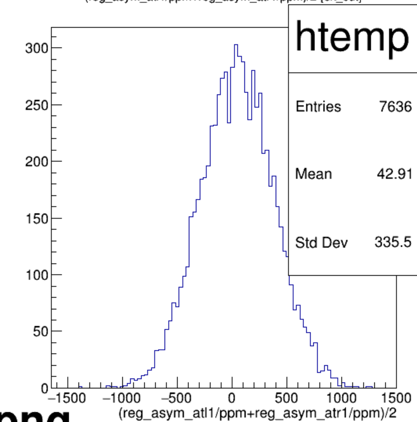
(reg_asym_atl1/ppm+reg_asym_atr1/ppm)/2 {ok_cut}
