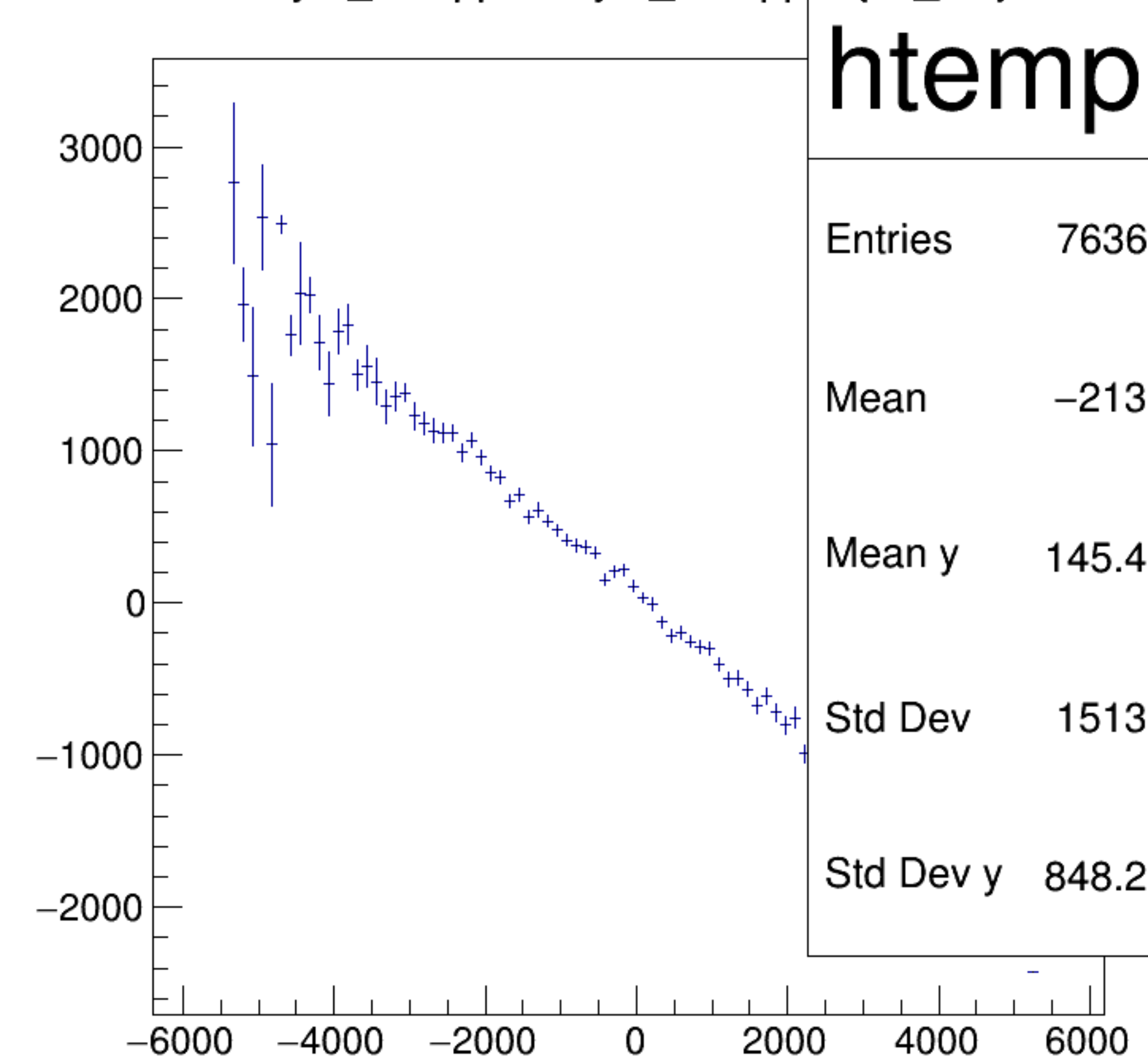
asym_atl1/ppm:asym_atr1/ppm {ok_cut}
