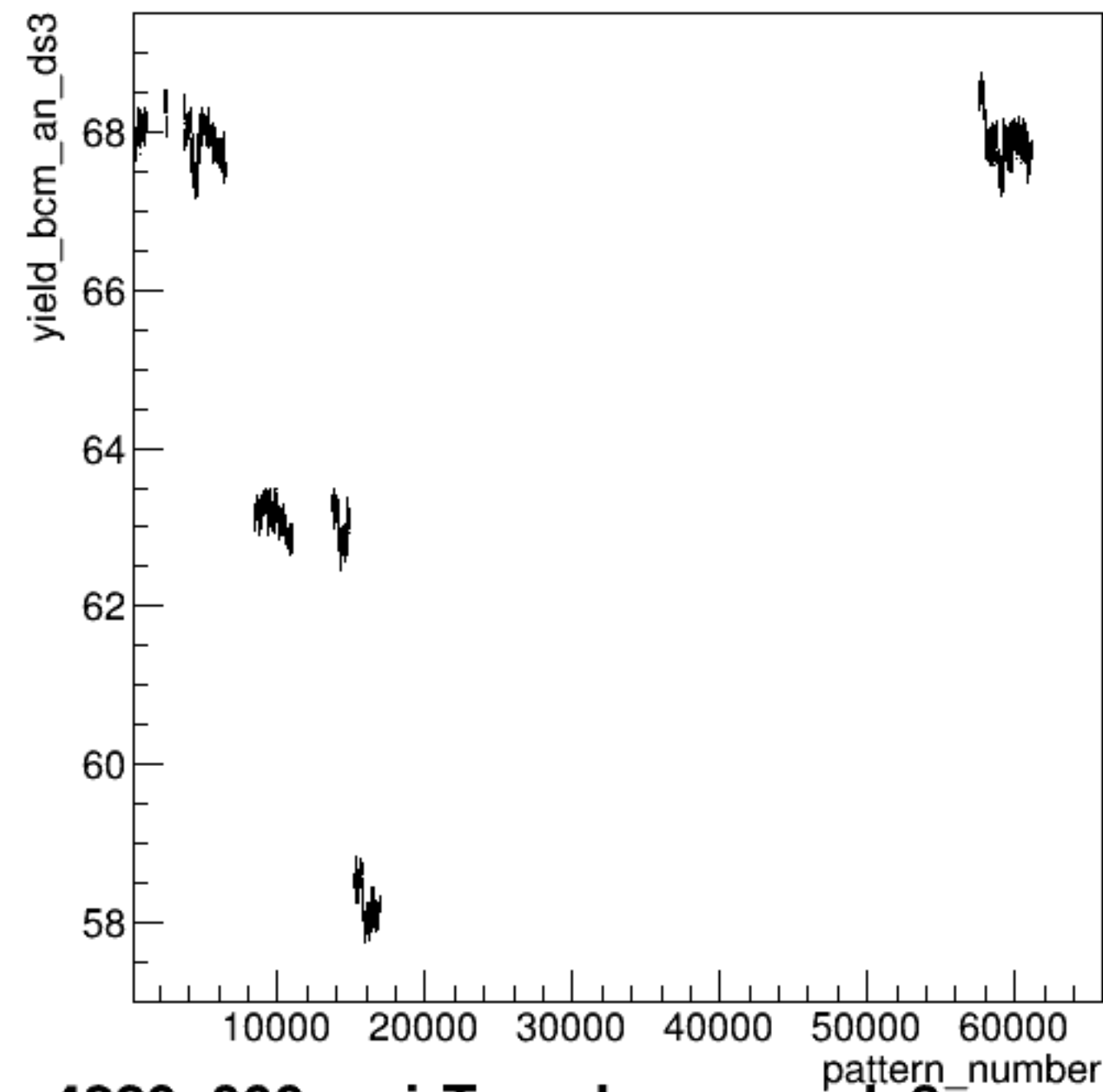
yield_bcm_an_ds3:pattern_number {ErrorFlag==0}
