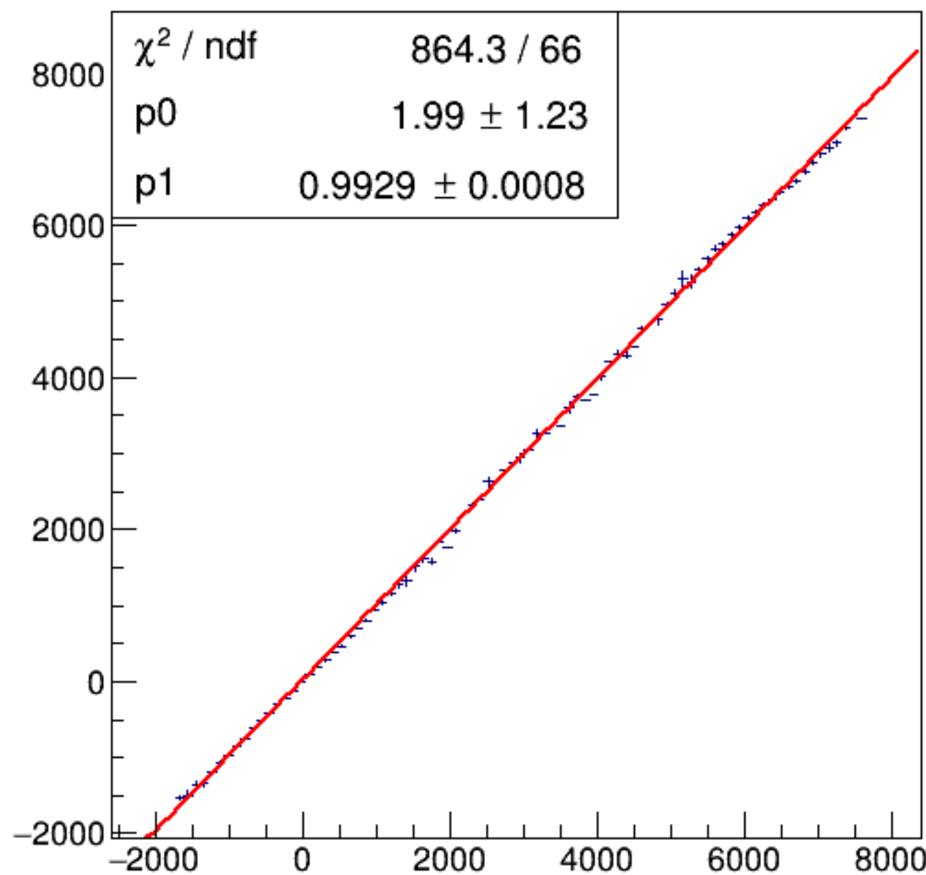
run4229_000_asym_bcm_dg_us_vs_asym_bcm_dg_ds_pr.png
