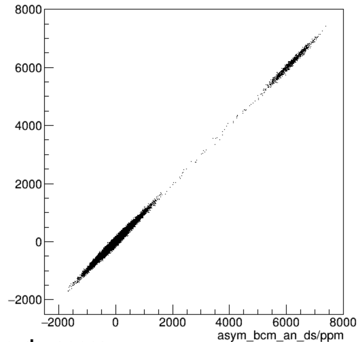
run4229_000_asym_bcm_an_us_vs_asym_bcm_an_ds_pr.png
