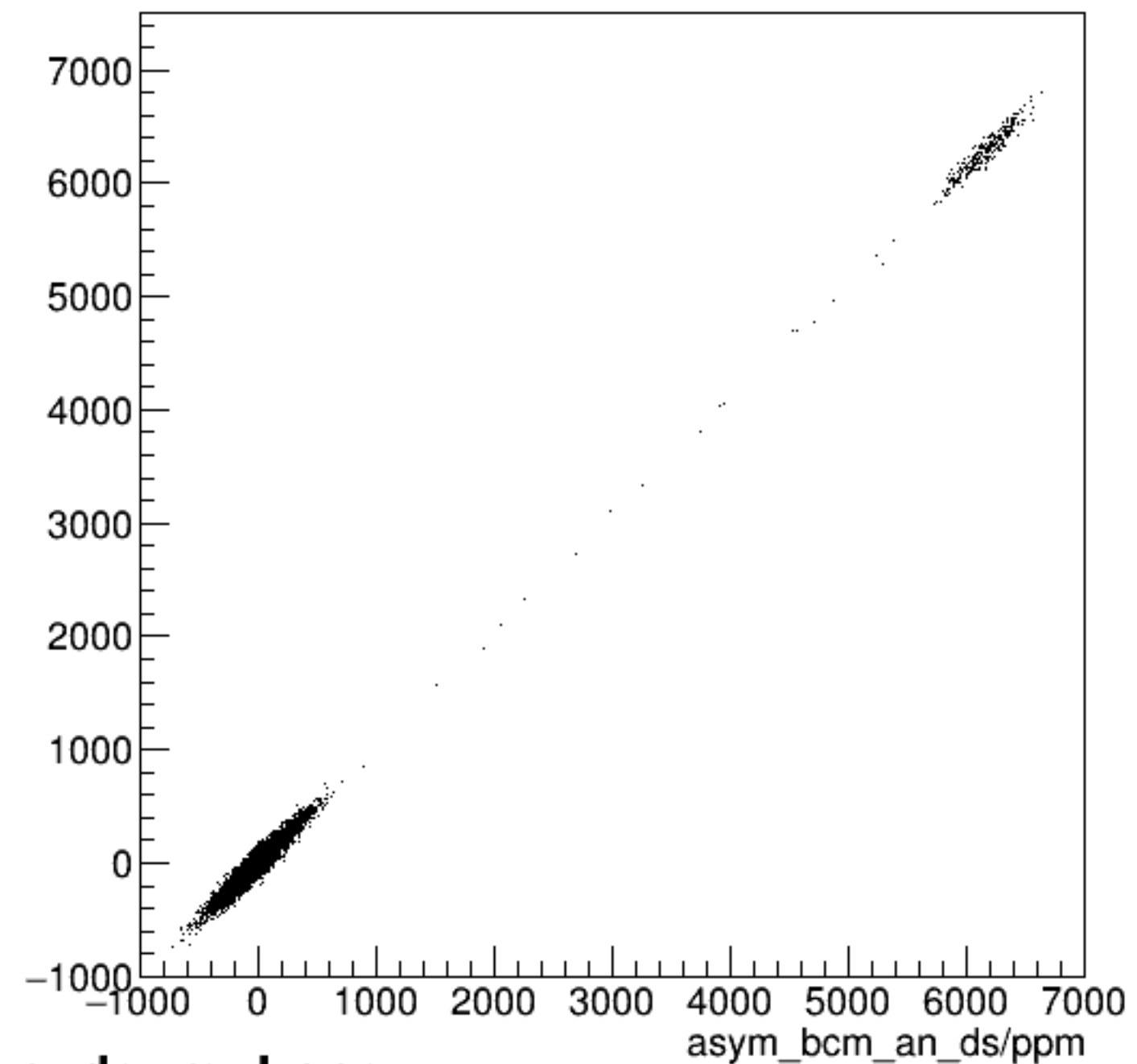
run4229_000_asym_bcm_dg_us_vs_asym_bcm_an_ds_mul.png
