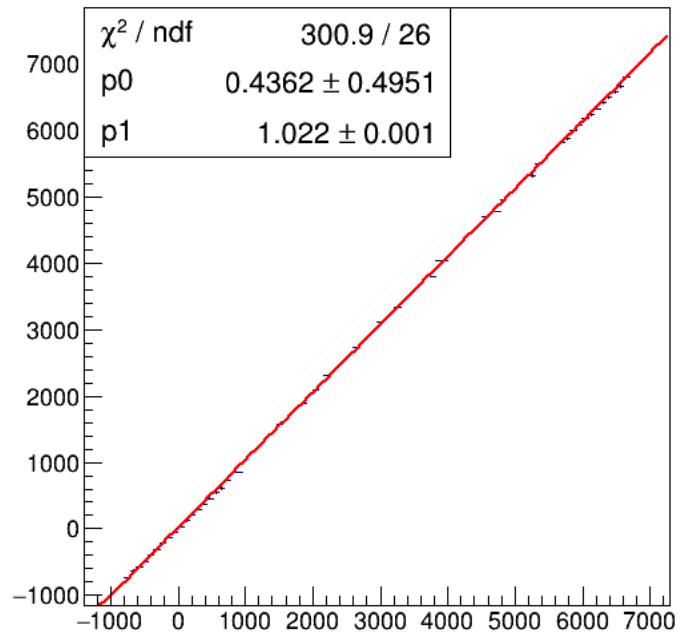
run4229_000_asym_bcm_dg_us_vs_asym_bcm_an_ds_mul.png
