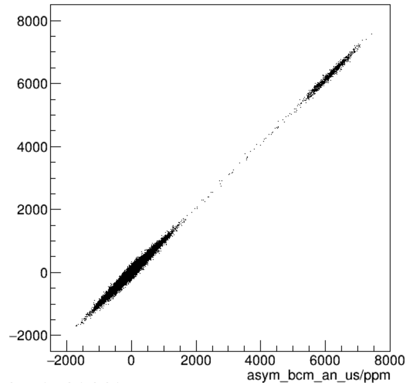
run4229_000_asym_bcm_dg_ds_vs_asym_bcm_an_us_pr.png
