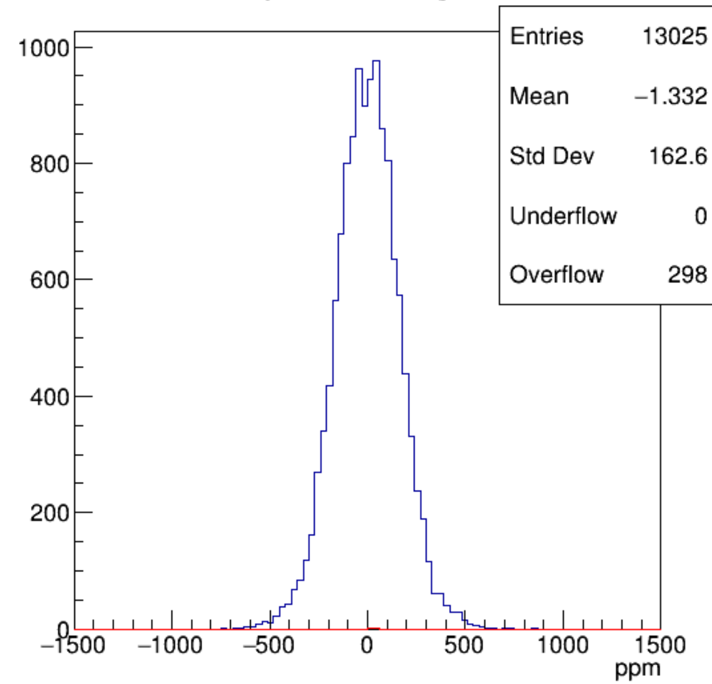
asym_bcm_dg_us
