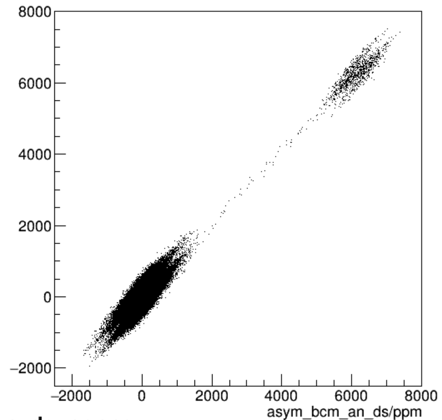
run4229_000_asym_bcm_dg_us_vs_asym_bcm_an_ds_pr.png
