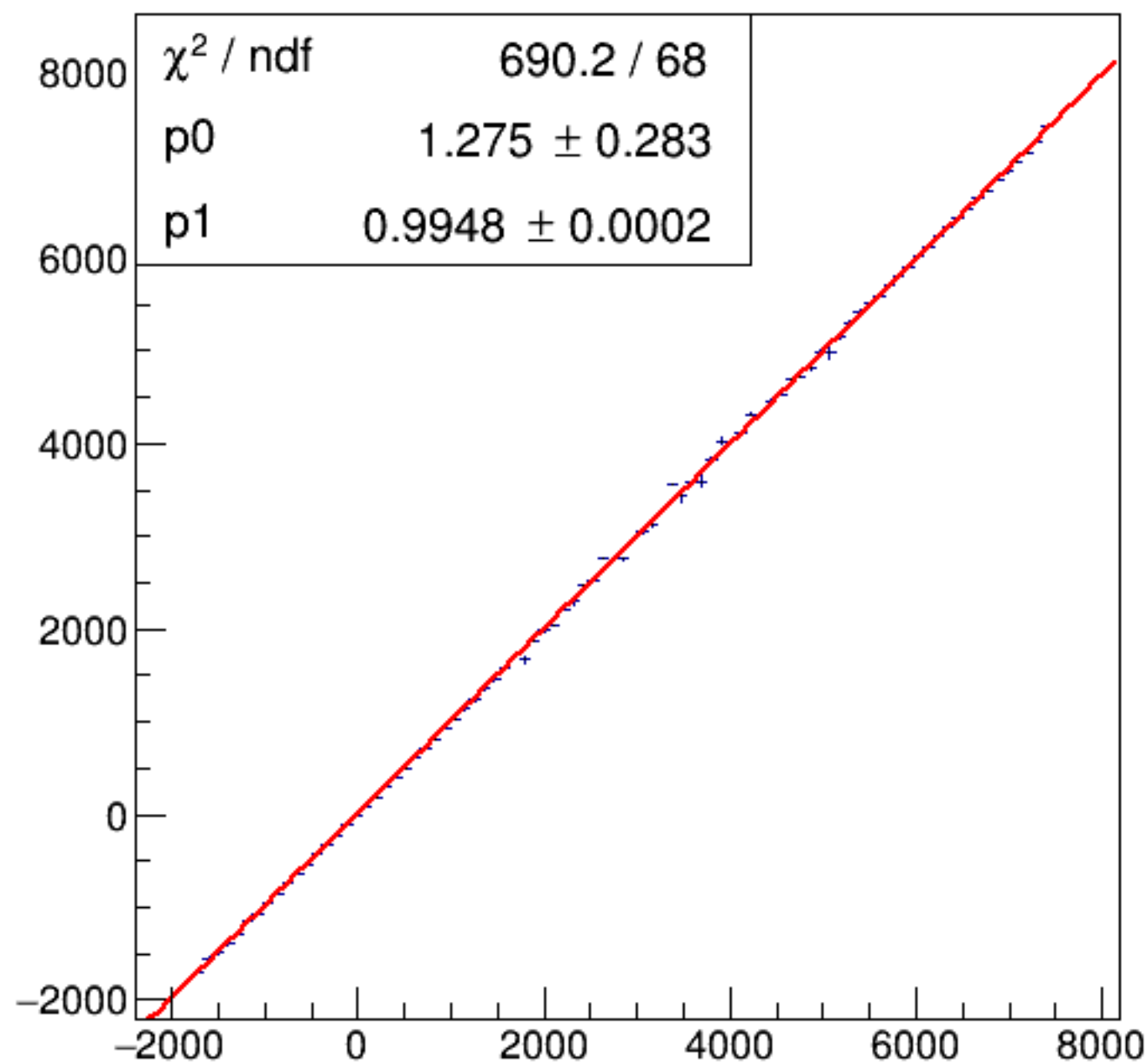
run4229_000_asym_bcm_an_us_vs_asym_bcm_an_ds_pr.png
