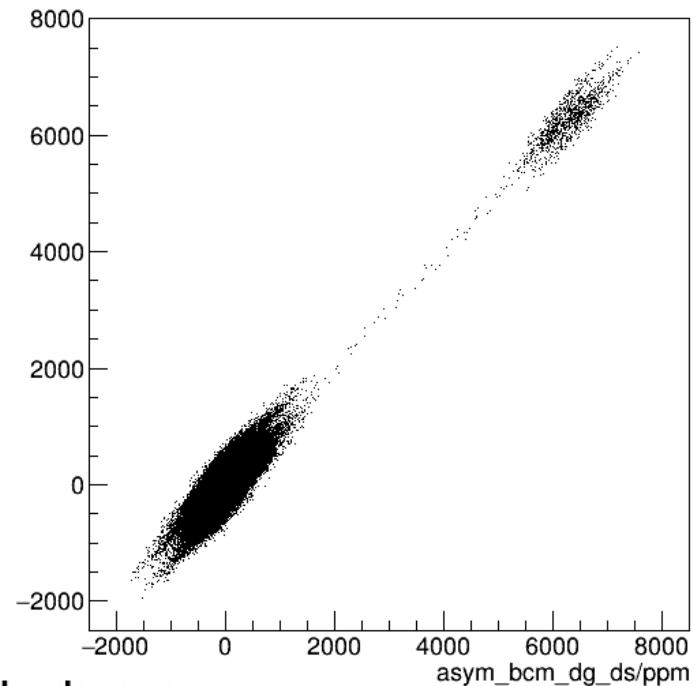
run4229_000_asym_bcm_dg_us_vs_asym_bcm_dg_ds_pr.png
