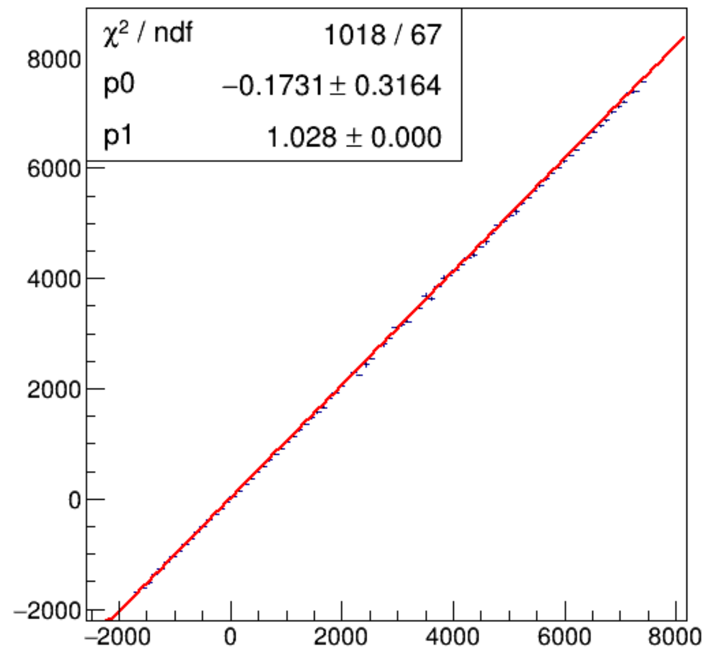
run4229_000_asym_bcm_dg_ds_vs_asym_bcm_an_us_pr.png
