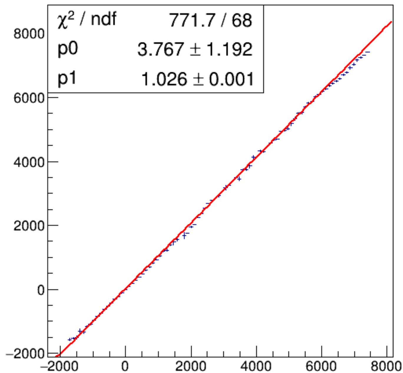
run4229_000_asym_bcm_dg_us_vs_asym_bcm_an_ds_pr.png
