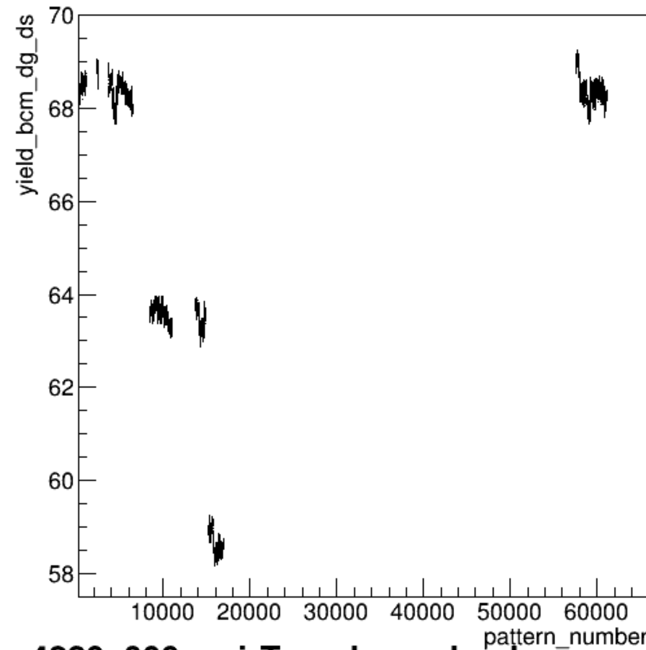
yield_bcm_dg_ds:pattern_number {ErrorFlag==0}
