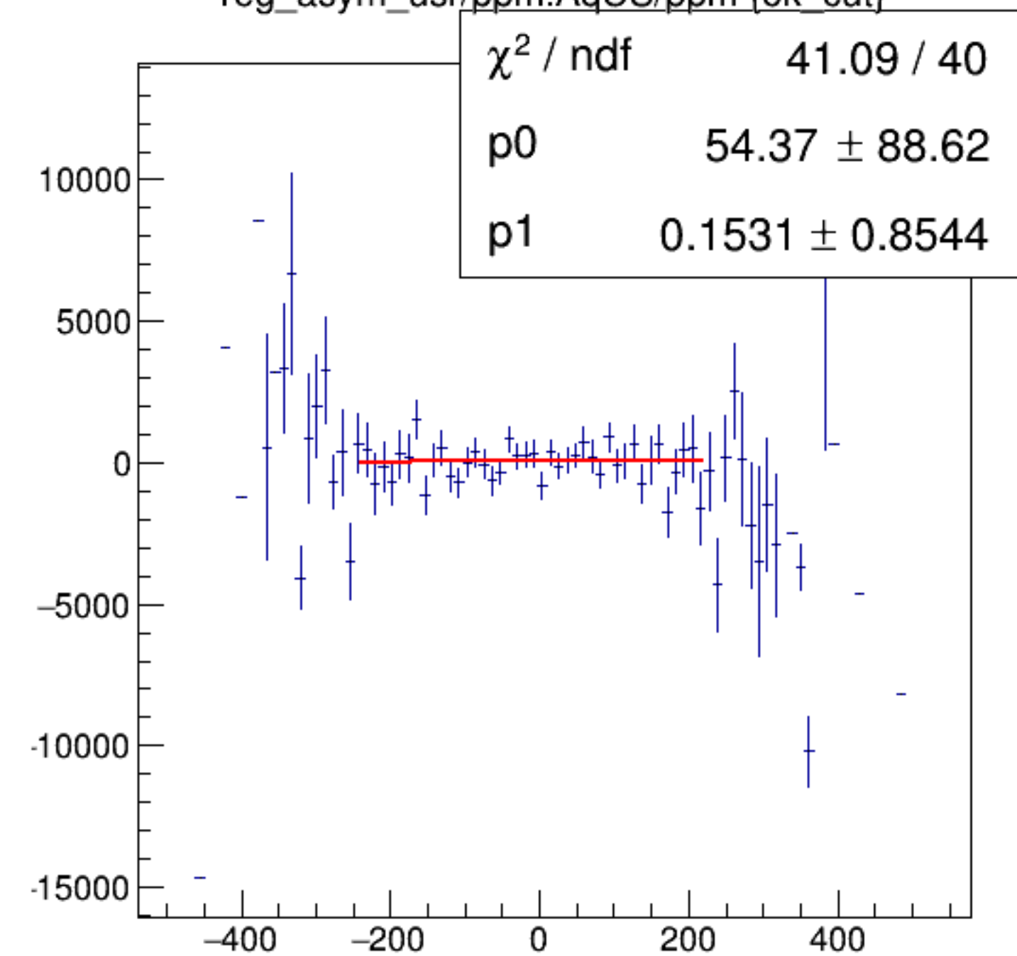
reg_asym_usr/ppm:AqUS/ppm {ok_cut}
