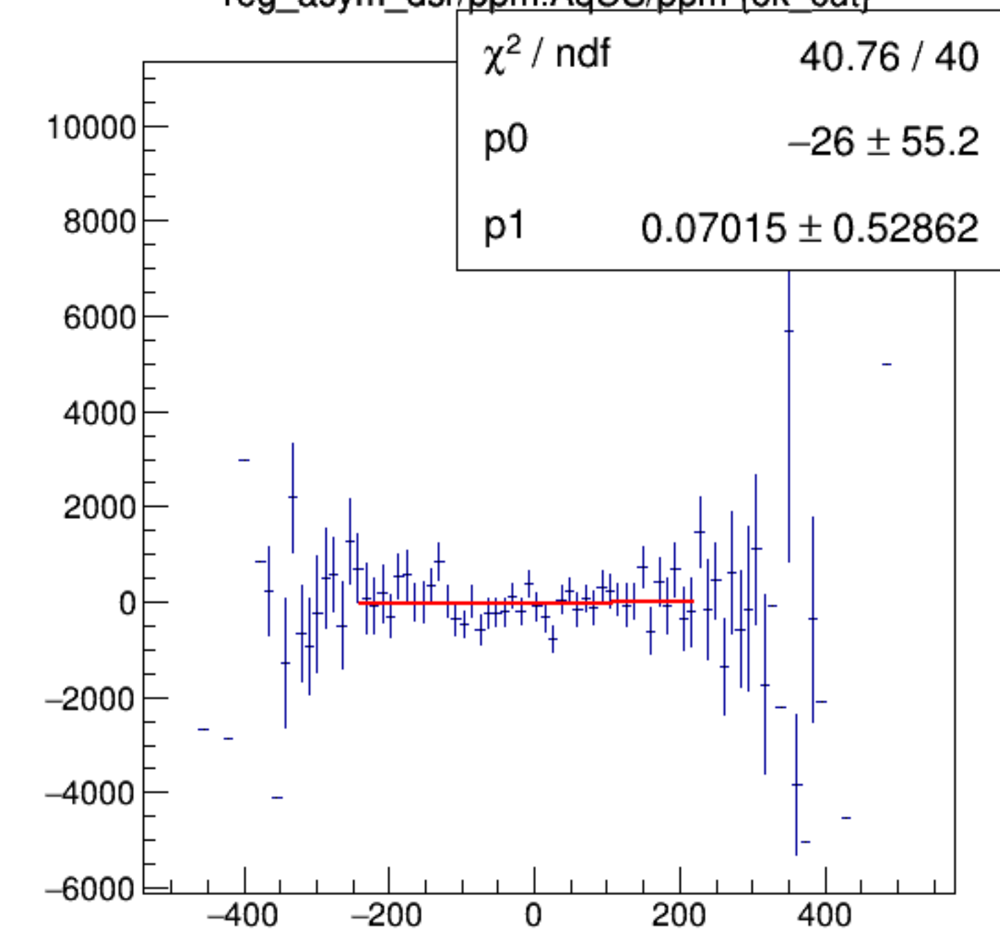
reg_asym_dsr/ppm:AqUS/ppm {ok_cut}
