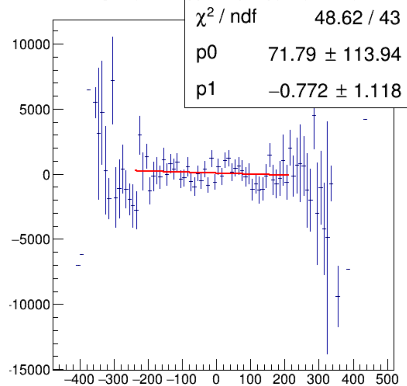
reg_asym_dsl/ppm:AqDS/ppm {ok_cut}
