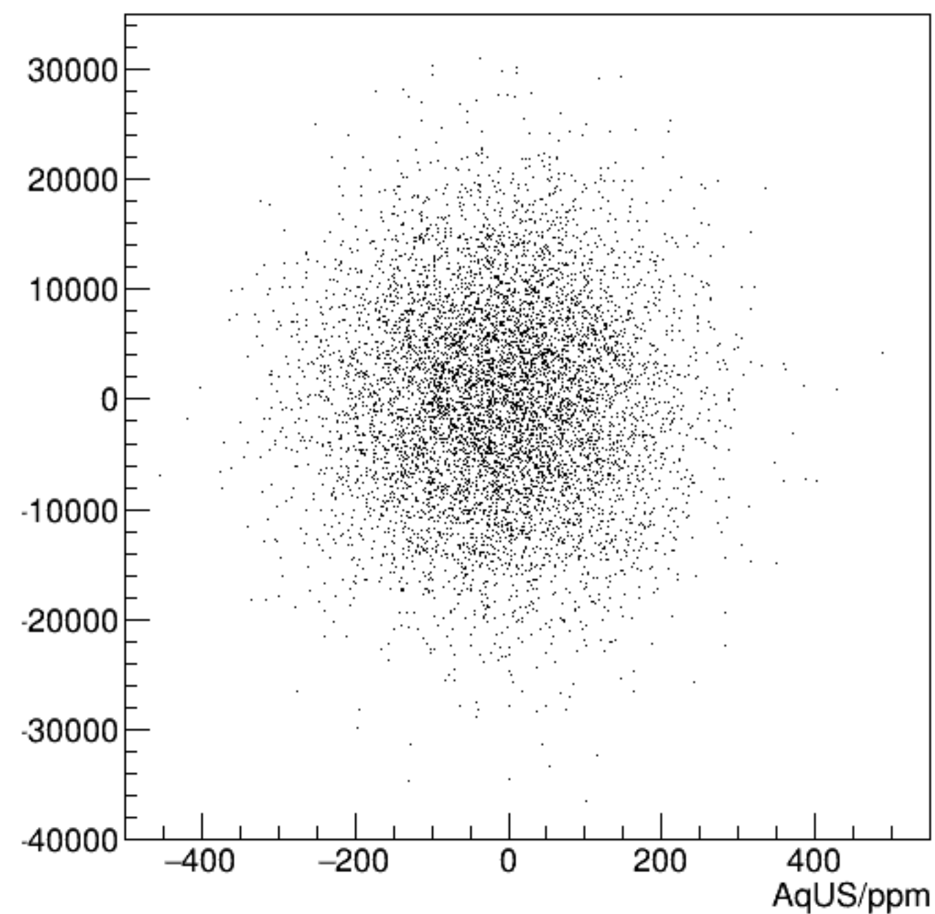
reg_asym_dsl/ppm:AqUS/ppm {ok_cut}
