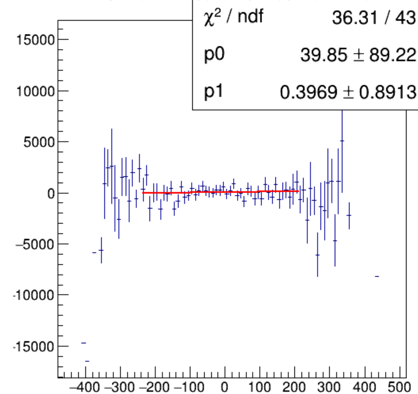
reg_asym_usr/ppm:AqDS/ppm {ok_cut}
