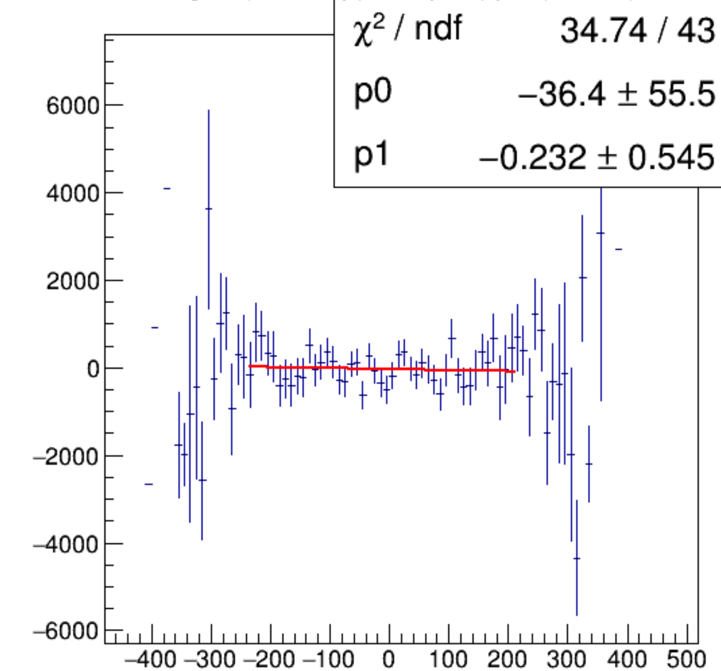
reg_asym_dsr/ppm:AqDS/ppm {ok_cut}
