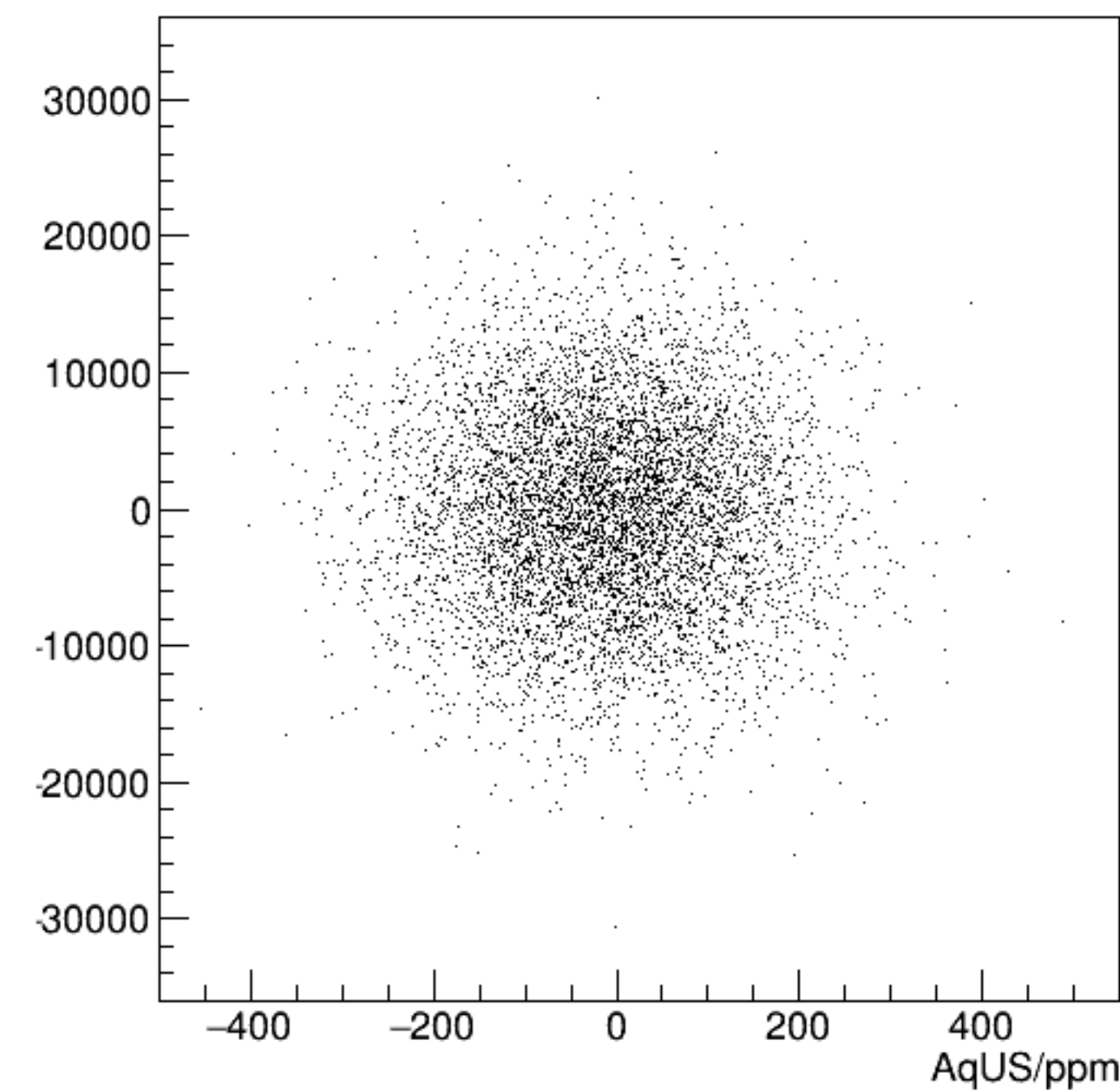
reg_asym_usr/ppm:AqUS/ppm {ok_cut}
