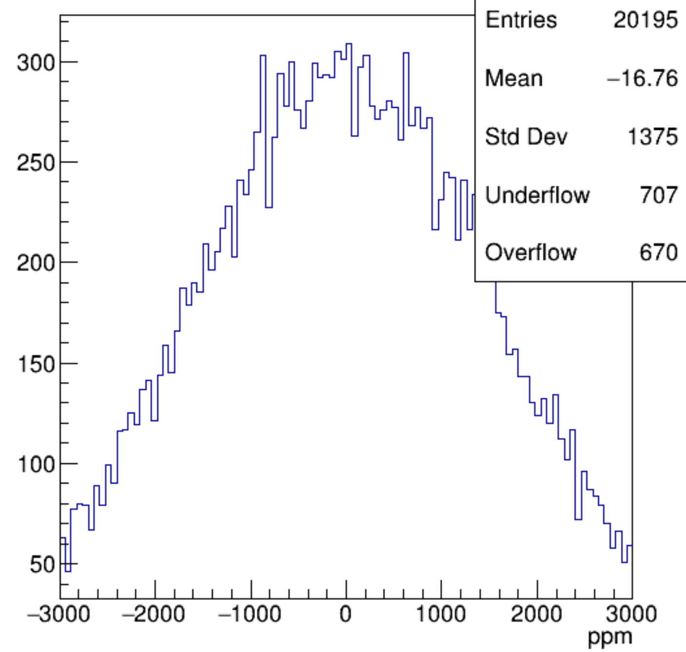
asym_dsl
