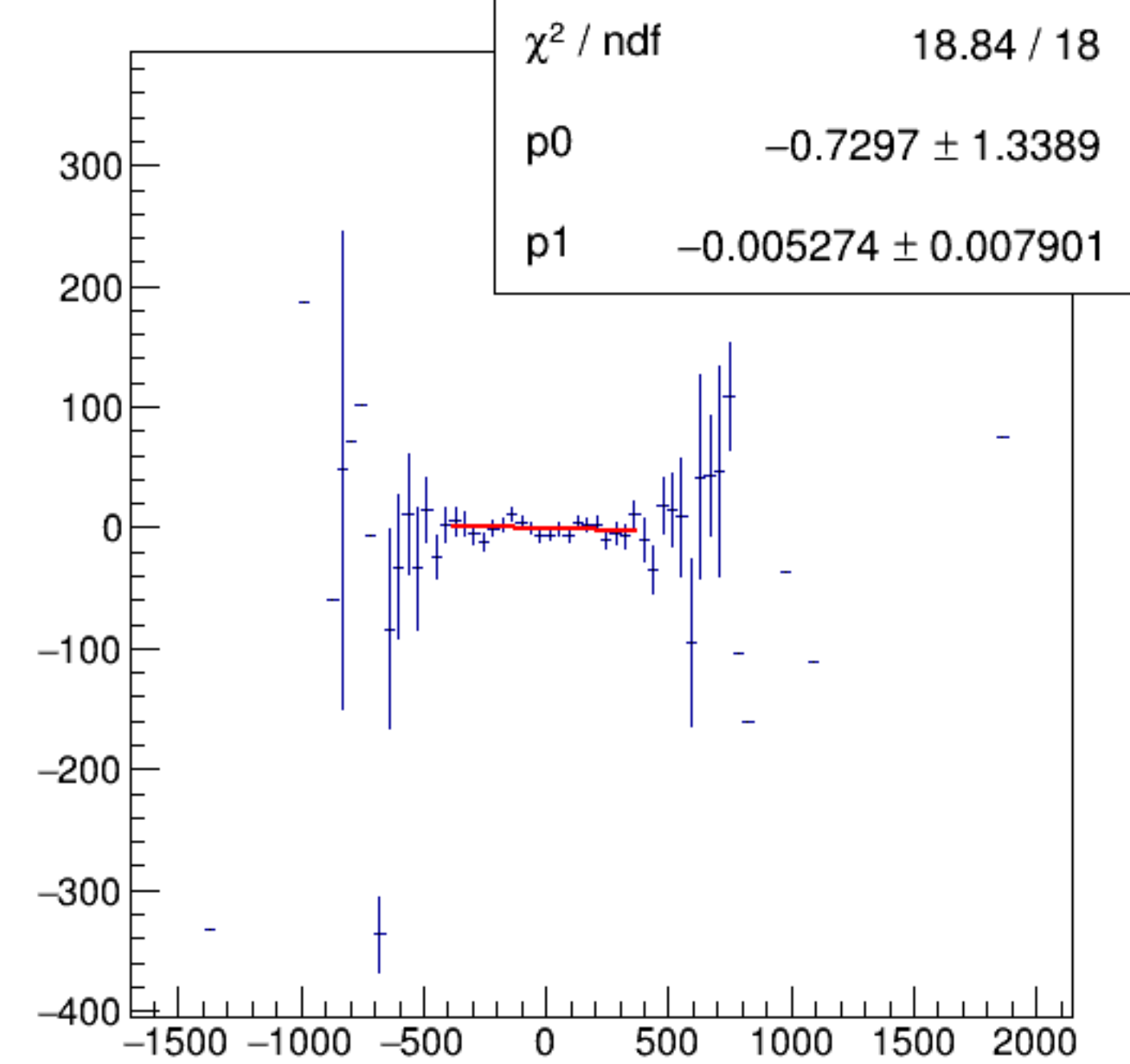
cor_usr/ppm:AqDS/ppm {ErrorFlag==0}
