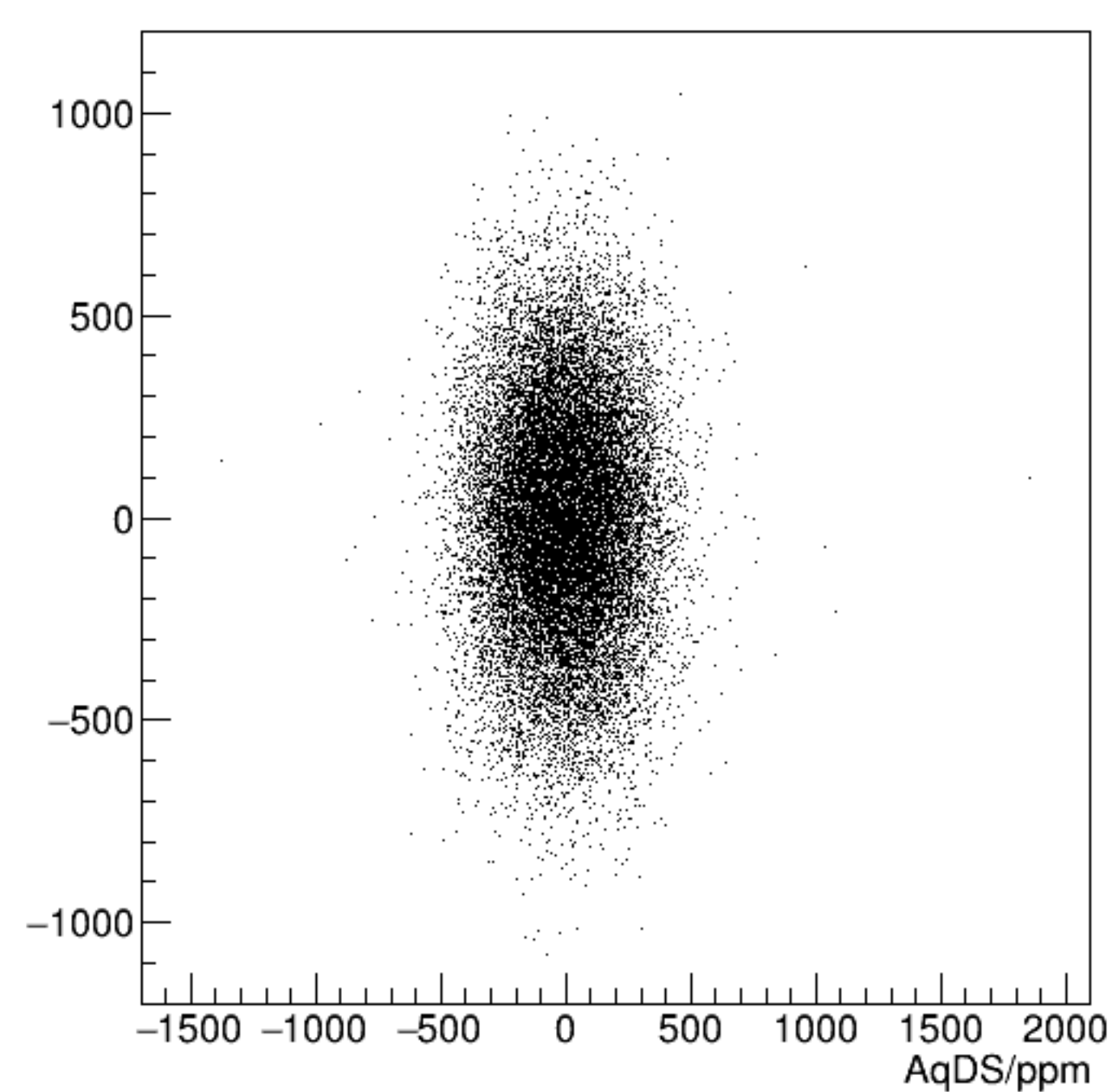
cor_dsl/ppm:AqDS/ppm {ErrorFlag==0}
