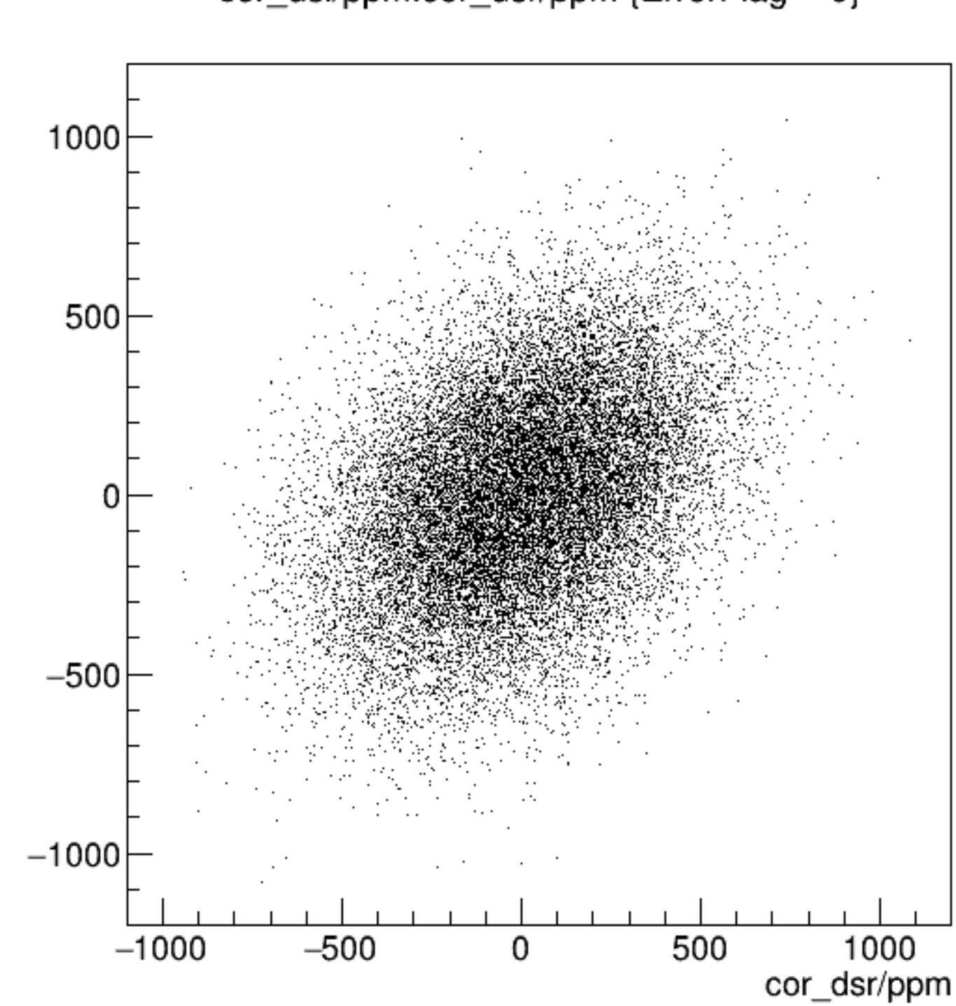
cor_dsl/ppm:cor_dsr/ppm {ErrorFlag==0}
