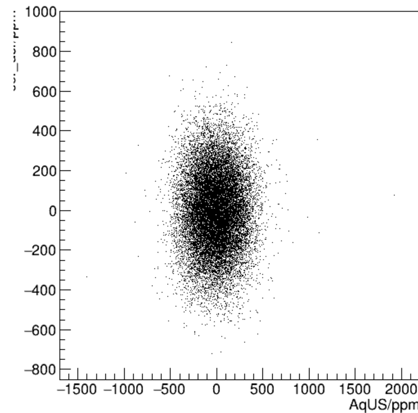
cor_usr/ppm:AqUS/ppm {ErrorFlag==0}
