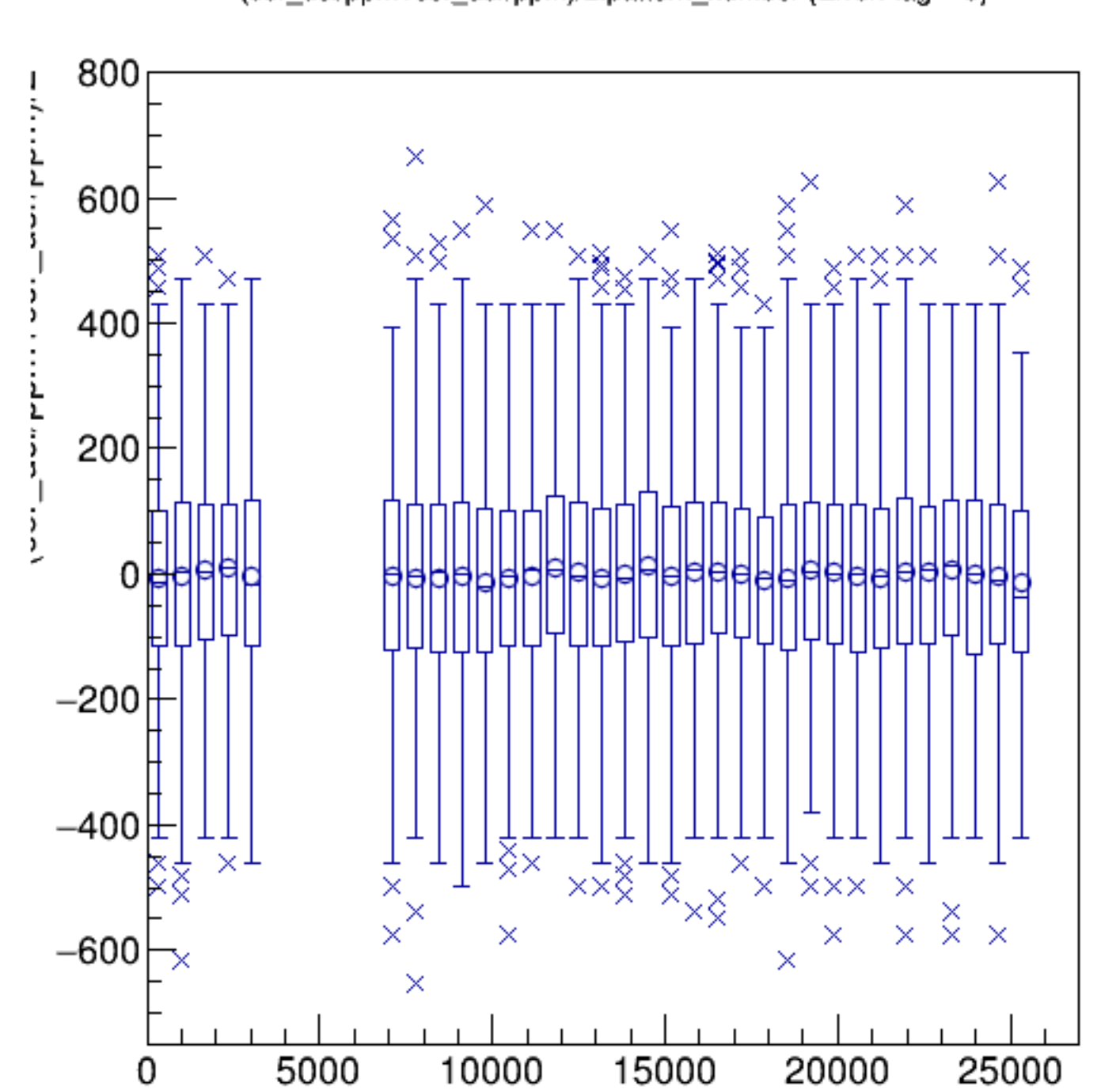
(cor_usl/ppm+cor_usr/ppm)/2:pattern_number {ErrorFlag==0}
