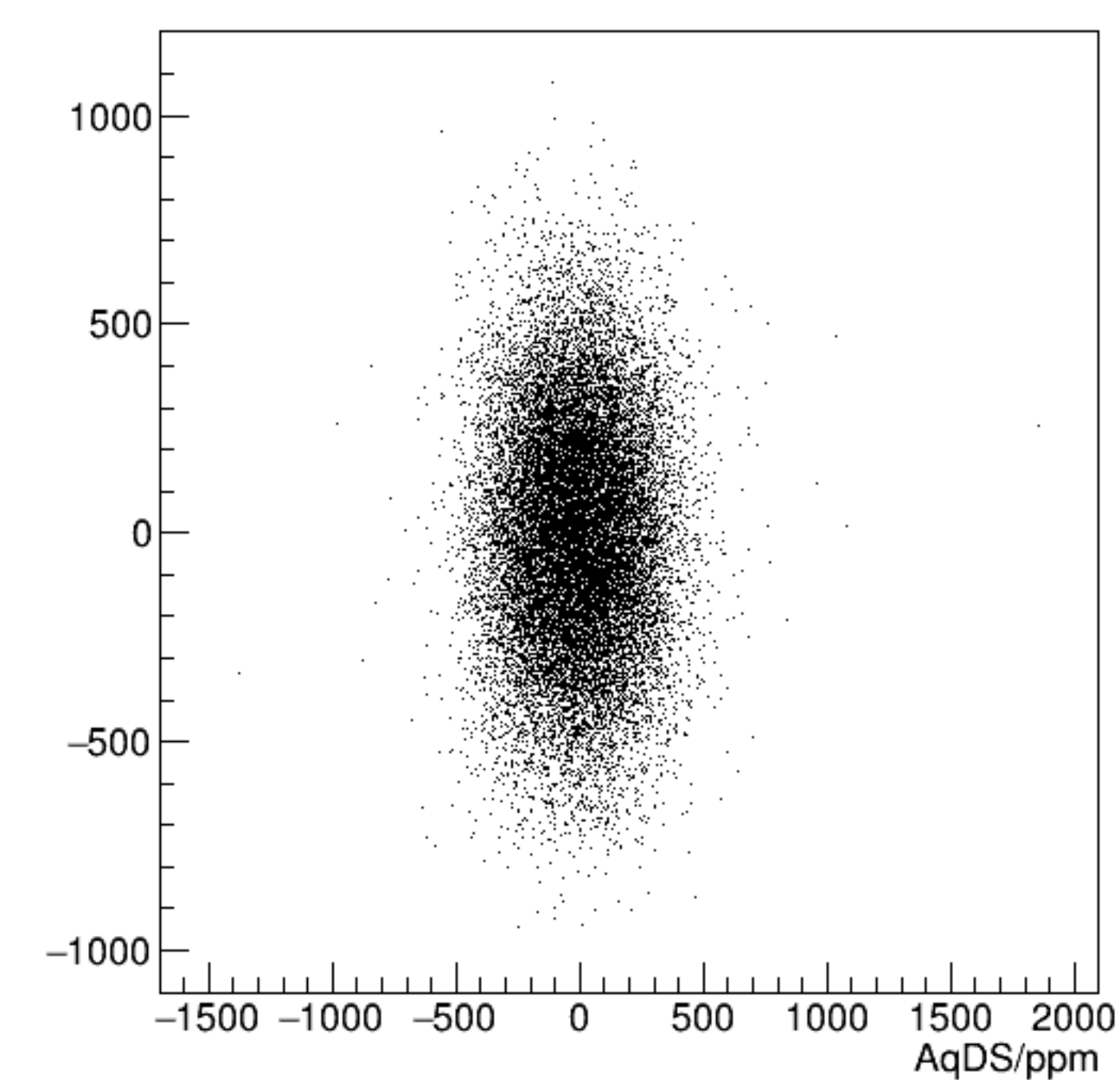
cor_dsr/ppm:AqDS/ppm {ErrorFlag==0}
