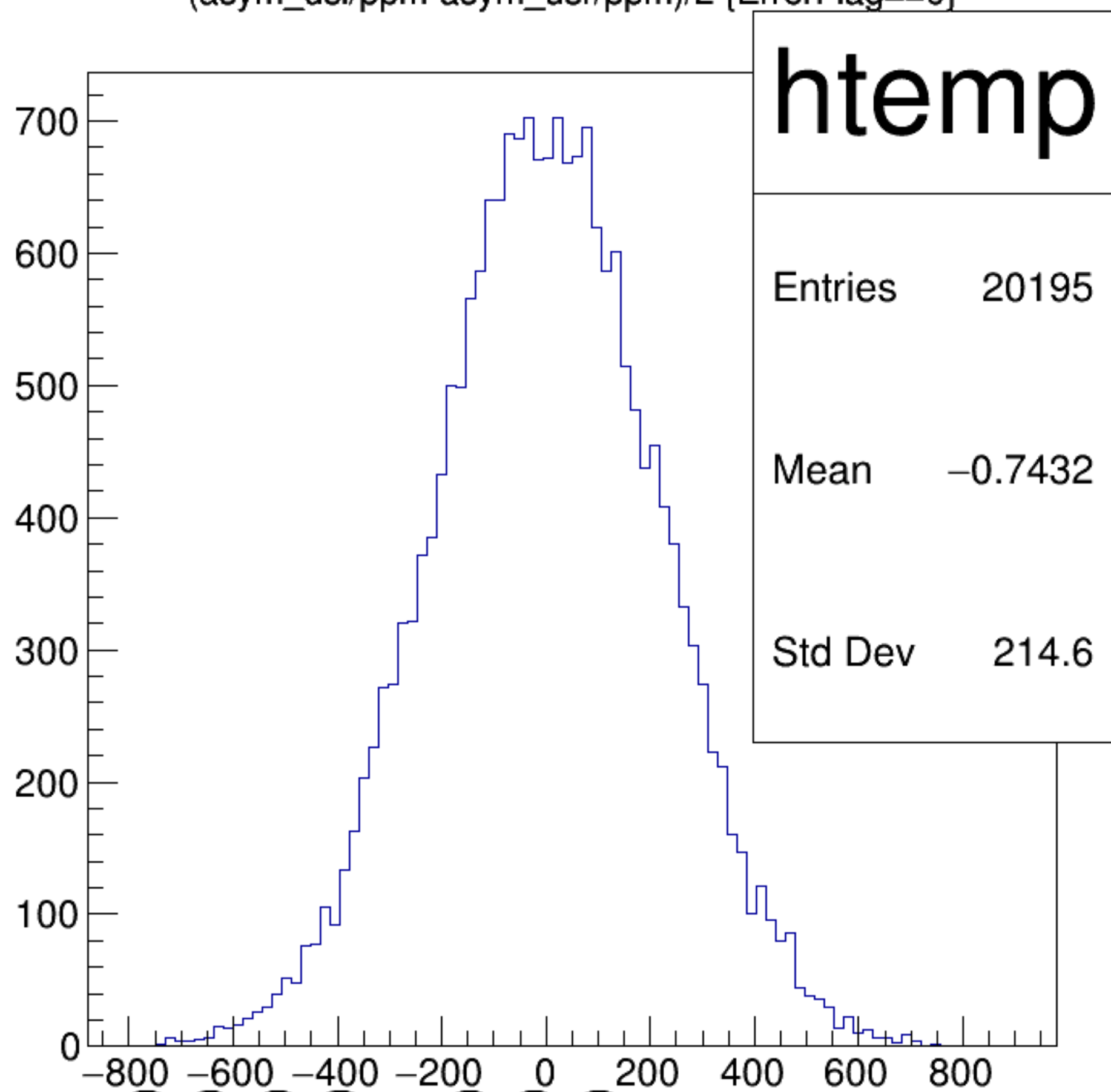
(asym_usl/ppm-asym_usr/ppm)/2 {ErrorFlag==0}
