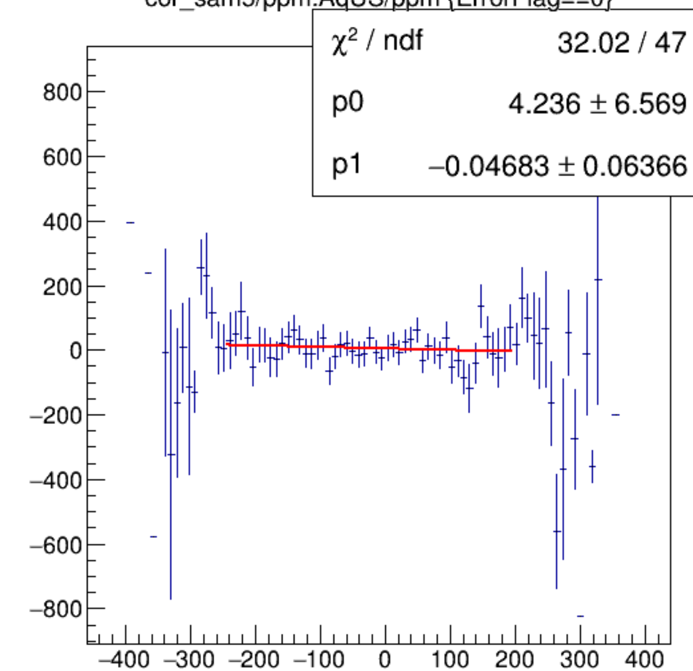
cor_sam5/ppm:AqUS/ppm {ErrorFlag==0}
