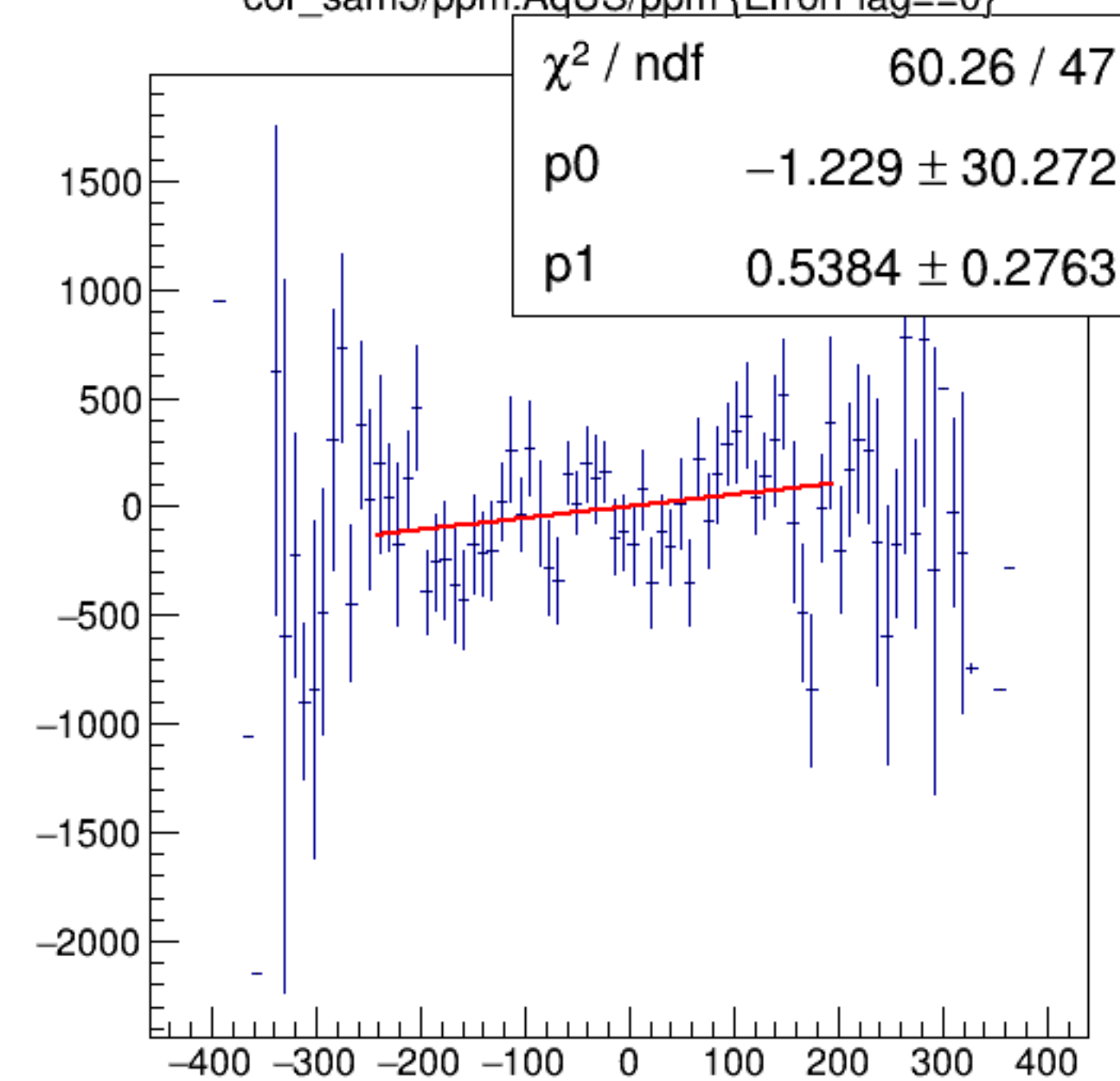
cor_sam3/ppm:AqUS/ppm {ErrorFlag==0}
