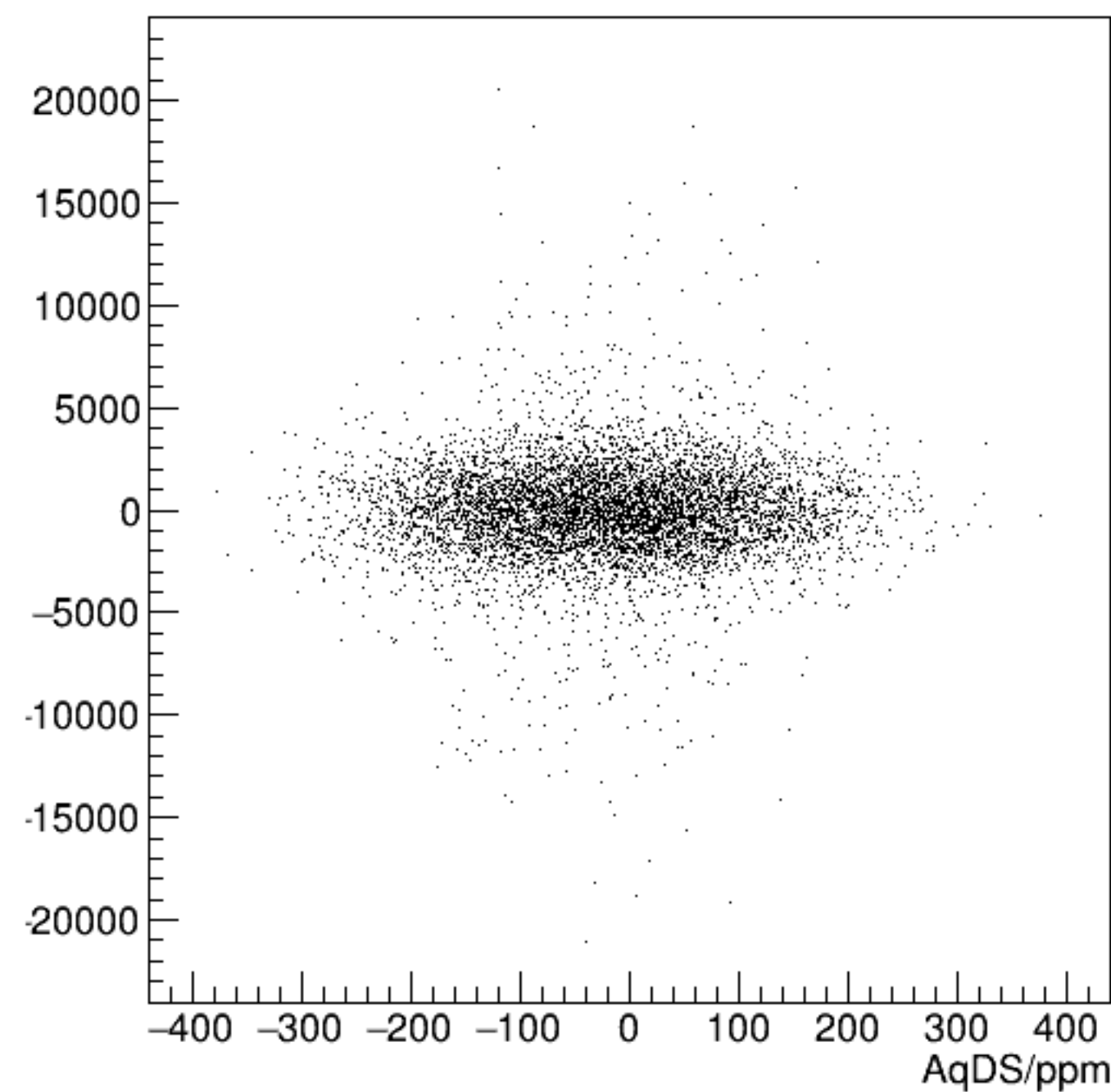
cor_sam3/ppm:AqDS/ppm {ErrorFlag==0}
