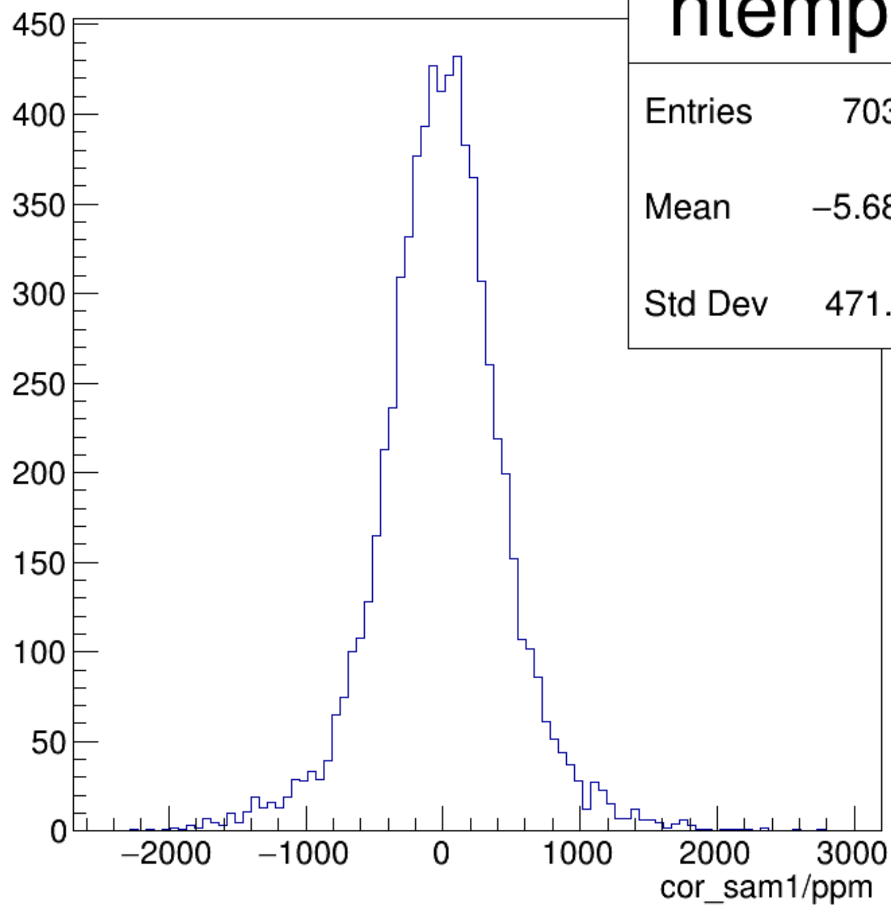
cor_sam1/ppm {ErrorFlag==0}
