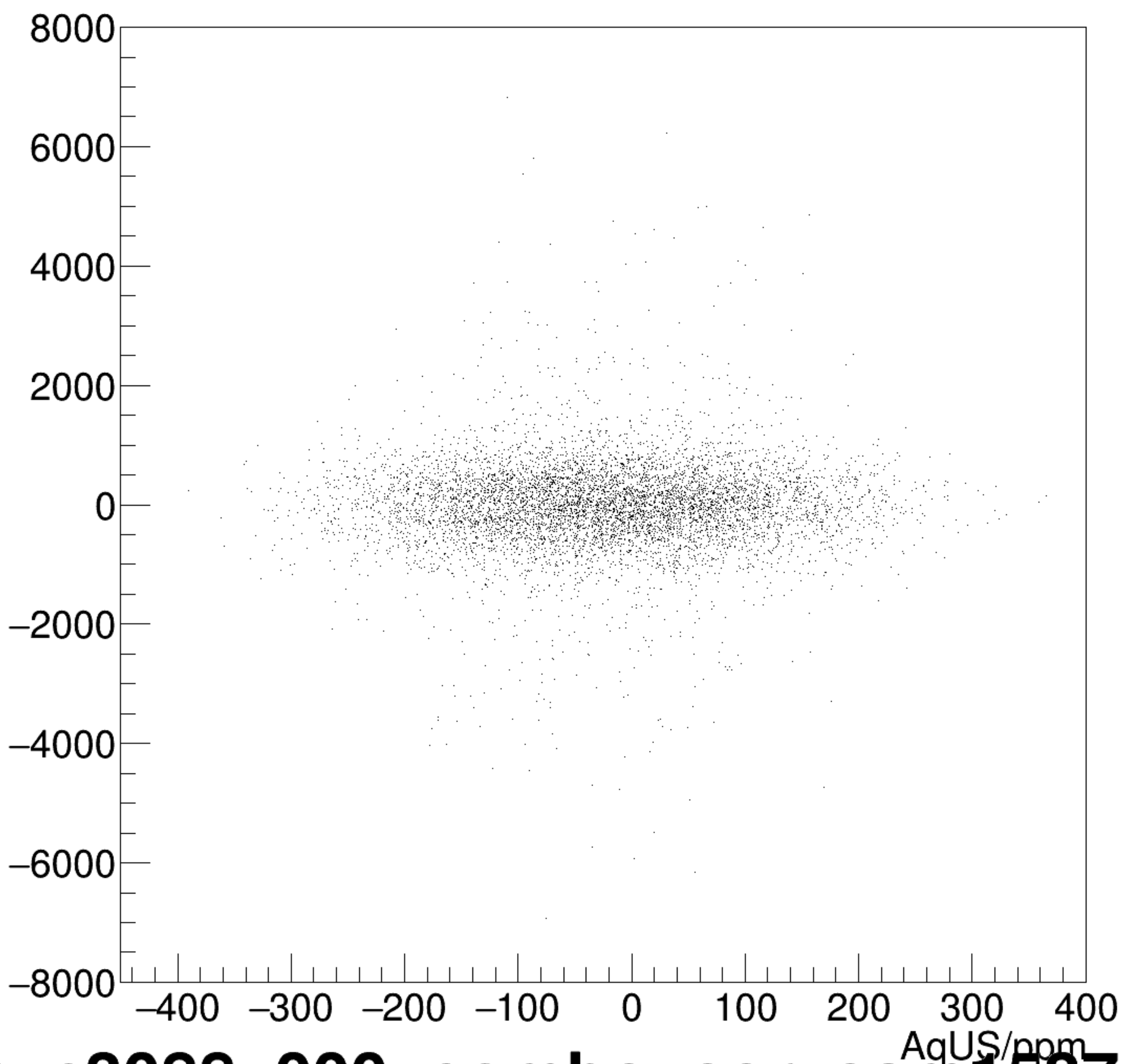
AverageLumi/ppm:AqUS/ppm {ErrorFlag==0}
