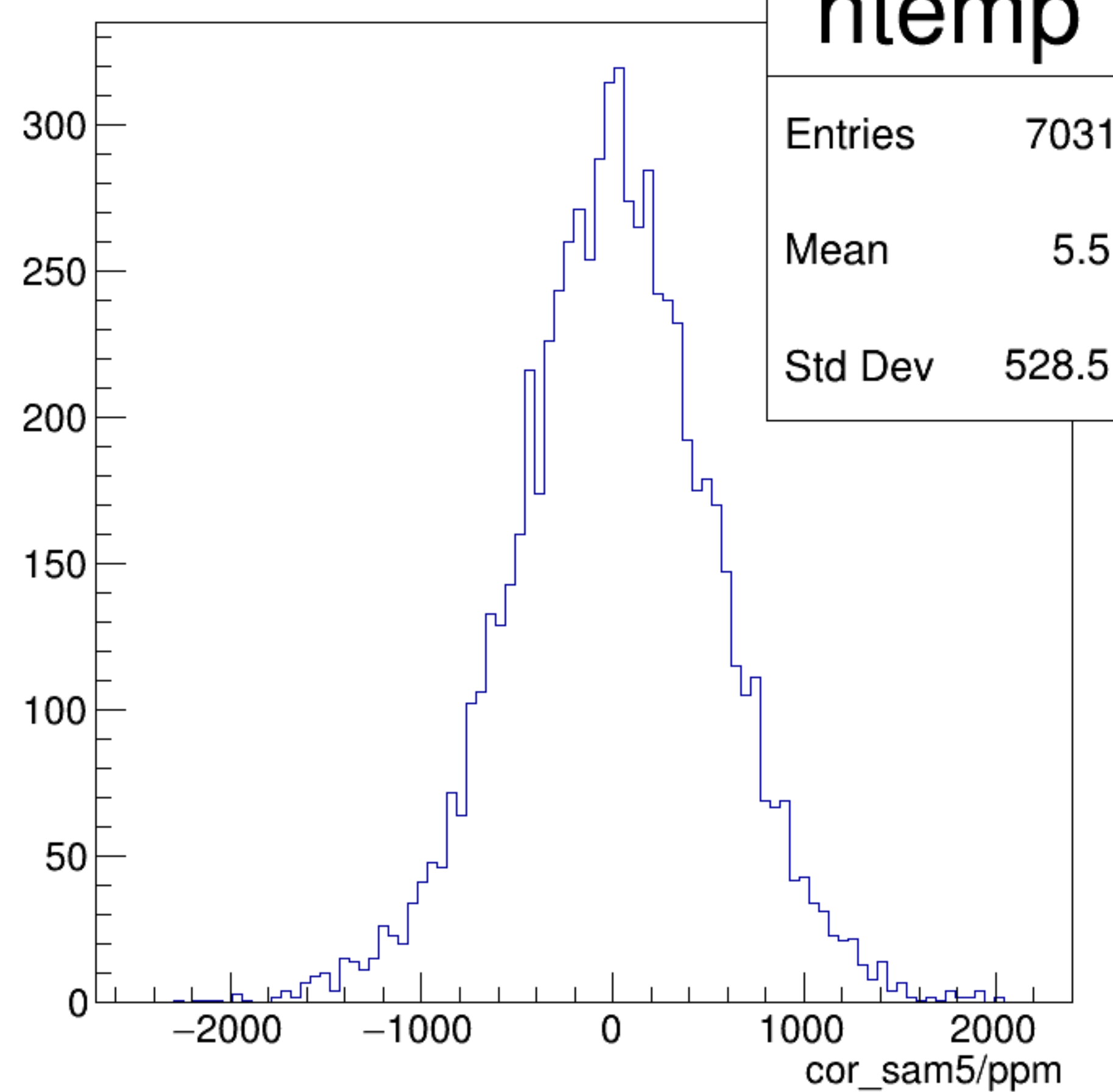
cor_sam5/ppm {ErrorFlag==0}
