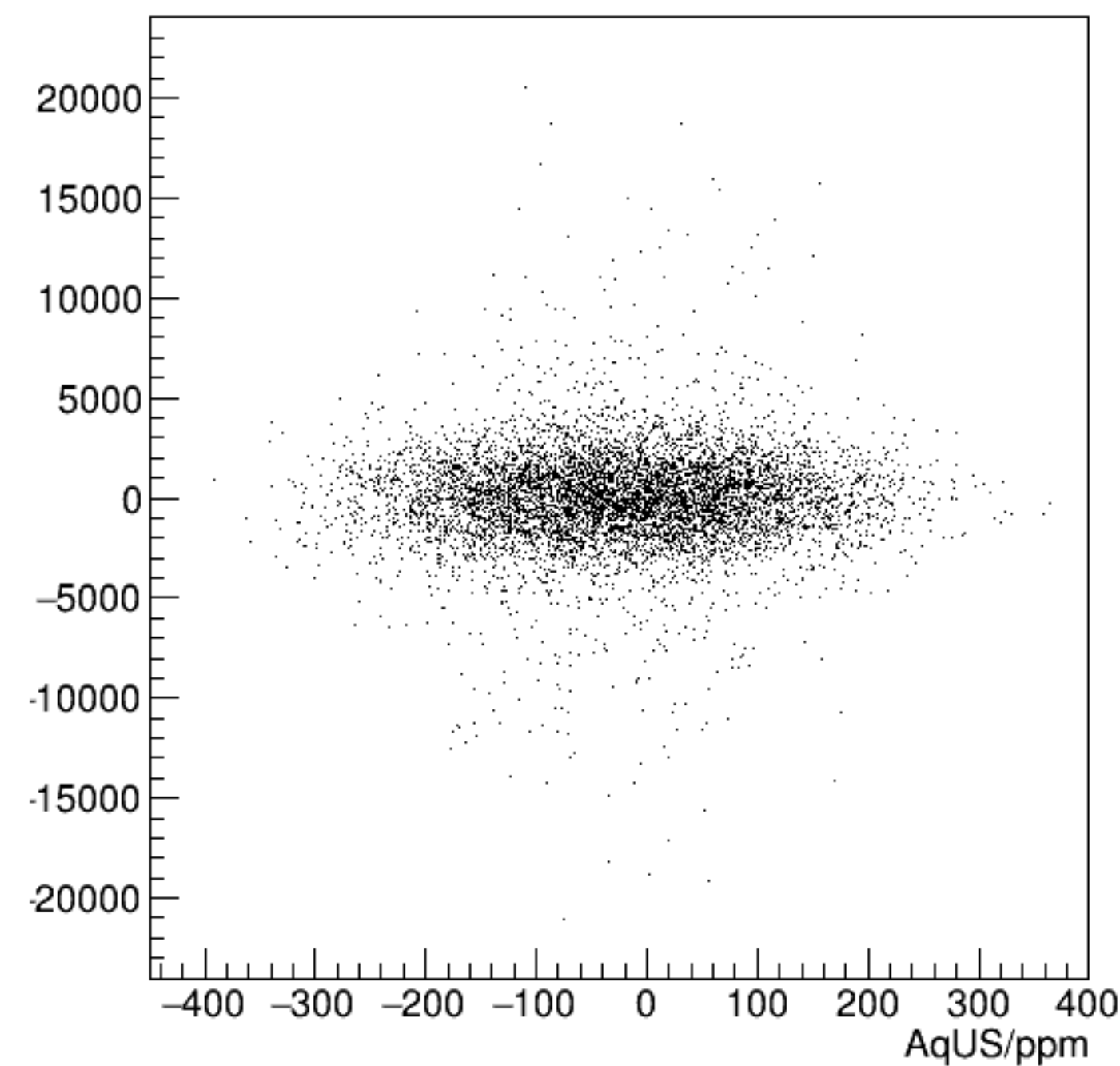
cor_sam3/ppm:AqUS/ppm {ErrorFlag==0}
