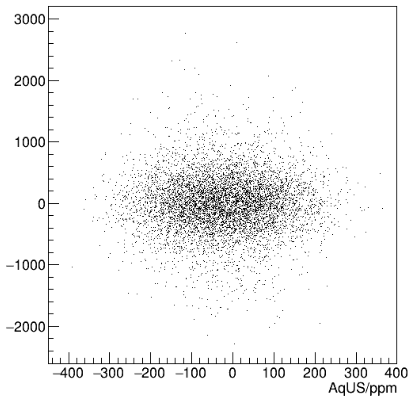
cor_sam1/ppm:AqUS/ppm {ErrorFlag==0}
