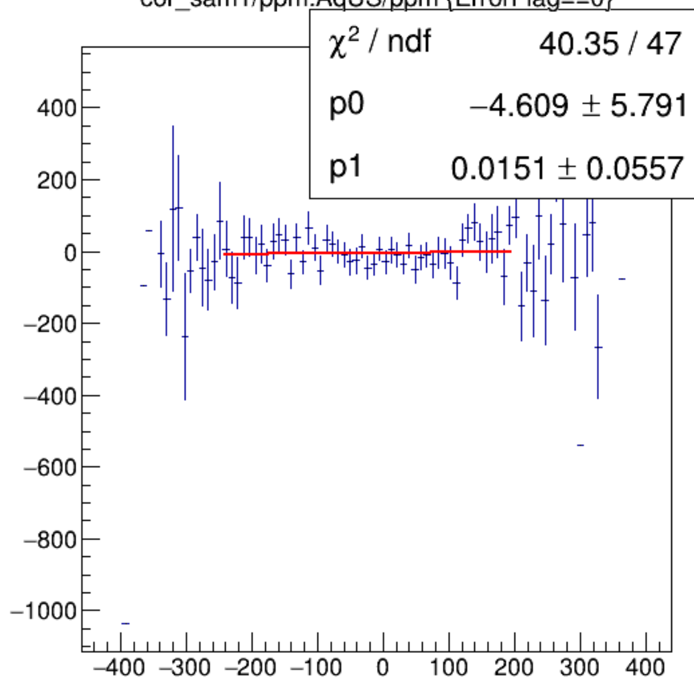
cor_sam1/ppm:AqUS/ppm {ErrorFlag==0}
