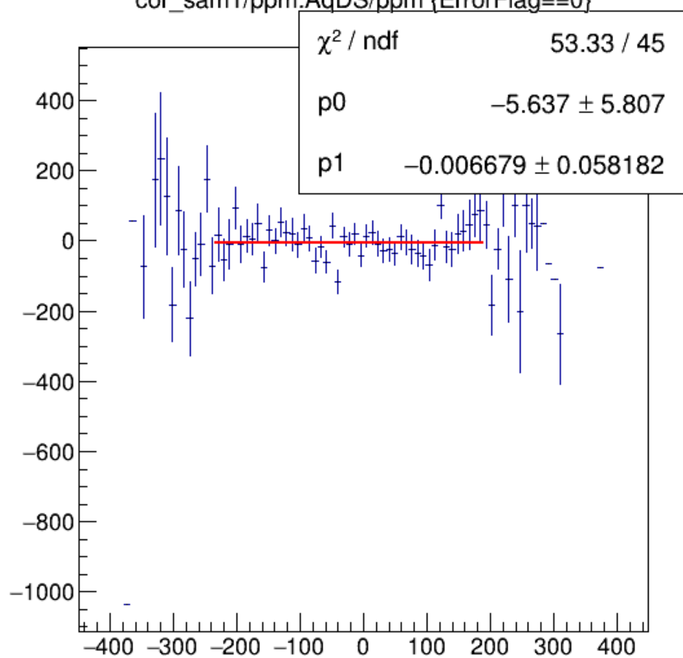
cor_sam1/ppm:AqDS/ppm {ErrorFlag==0}
