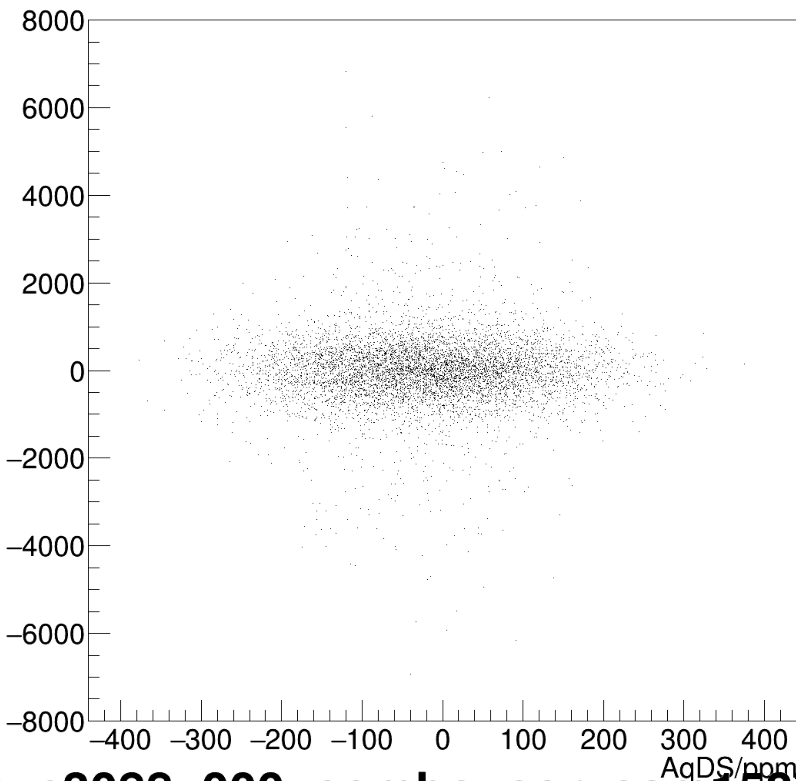
AverageLumi/ppm:AqDS/ppm {ErrorFlag==0}
