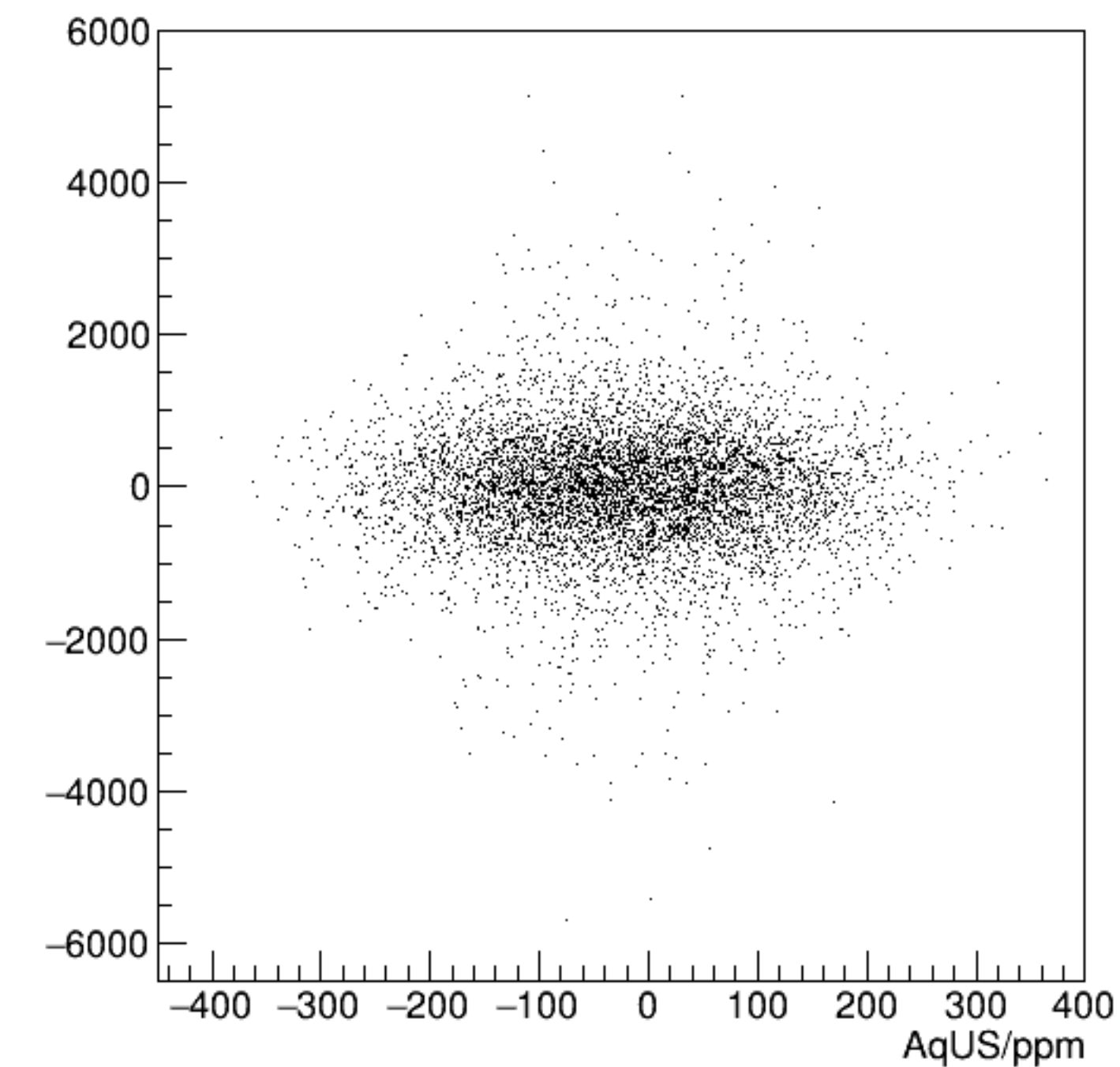
cor_sam7/ppm:AqUS/ppm {ErrorFlag==0}
