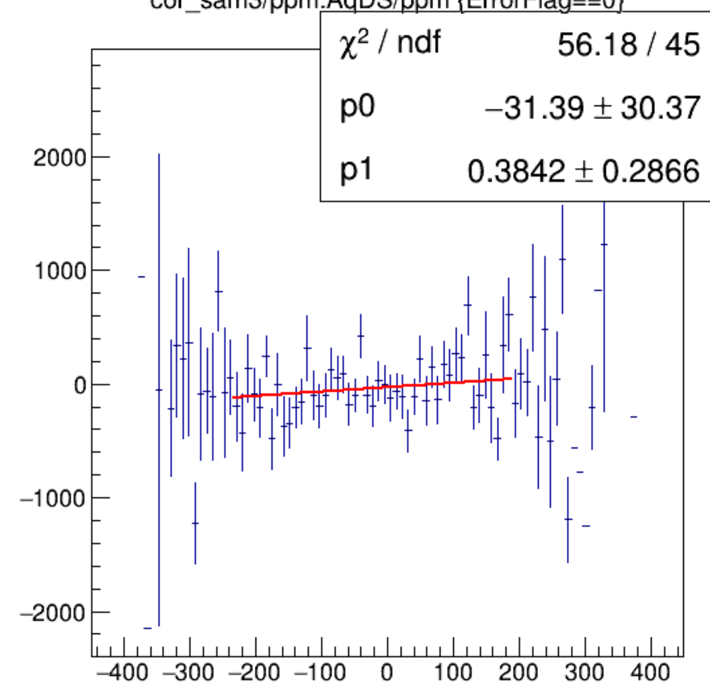
cor_sam3/ppm:AqDS/ppm {ErrorFlag==0}
