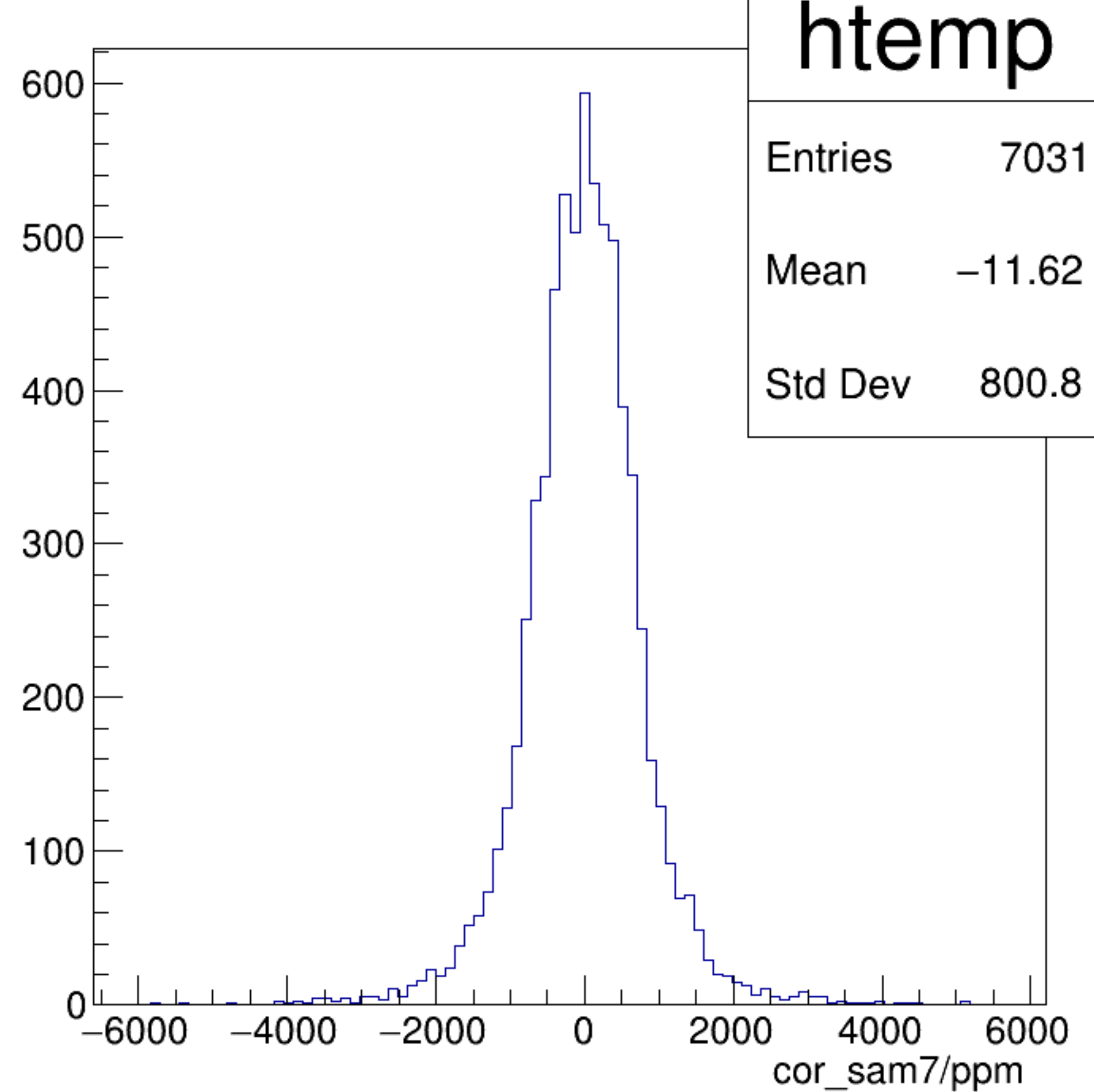
cor_sam7/ppm {ErrorFlag==0}
