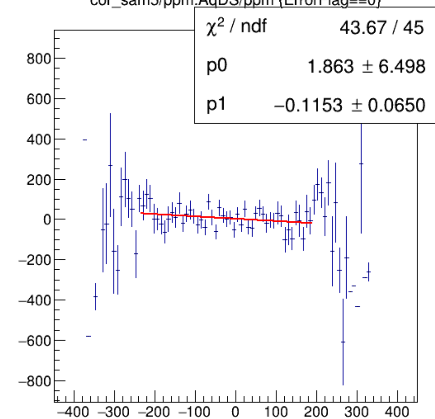
cor_sam5/ppm:AqDS/ppm {ErrorFlag==0}
