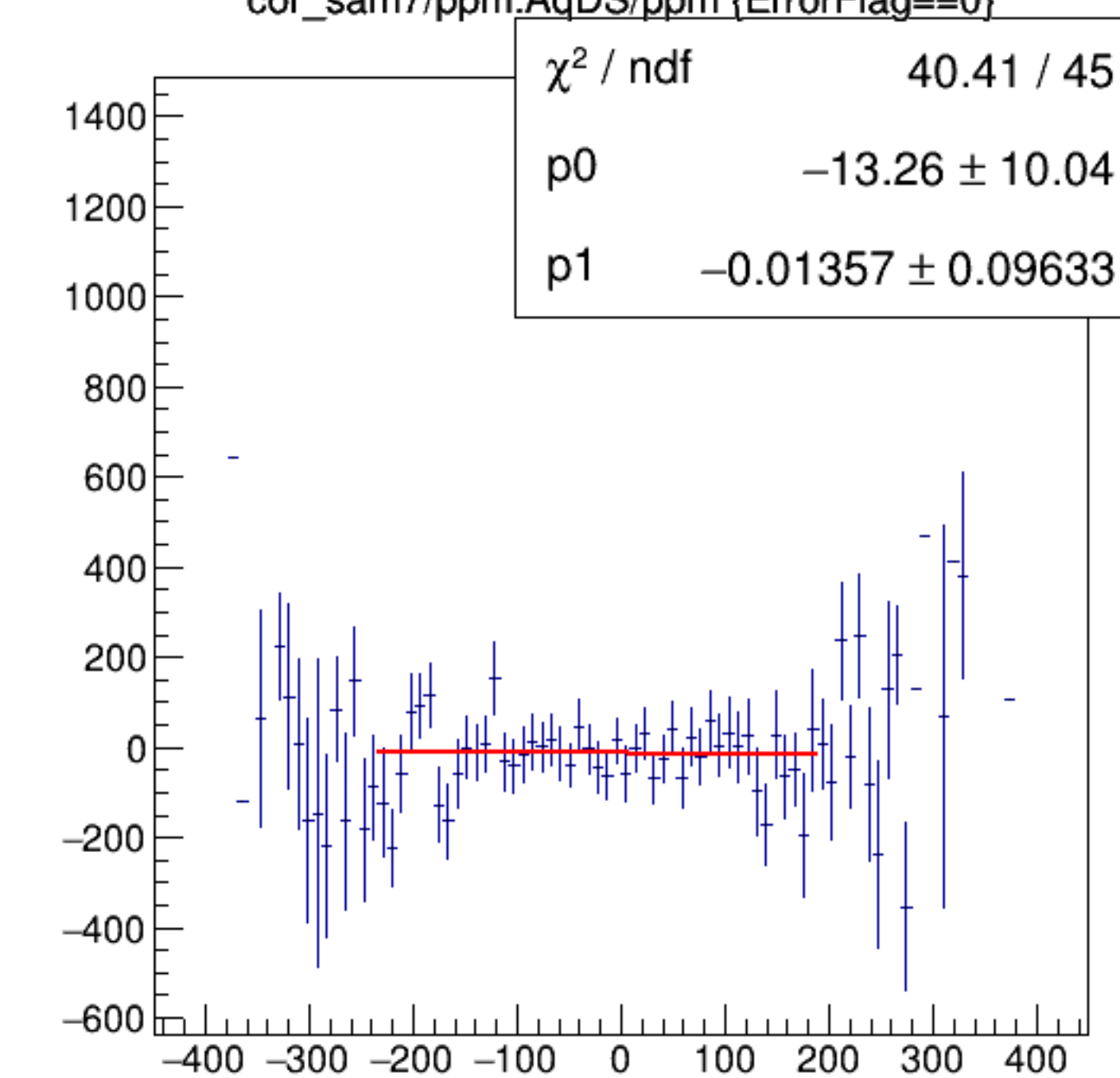
cor_sam7/ppm:AqDS/ppm {ErrorFlag==0}
