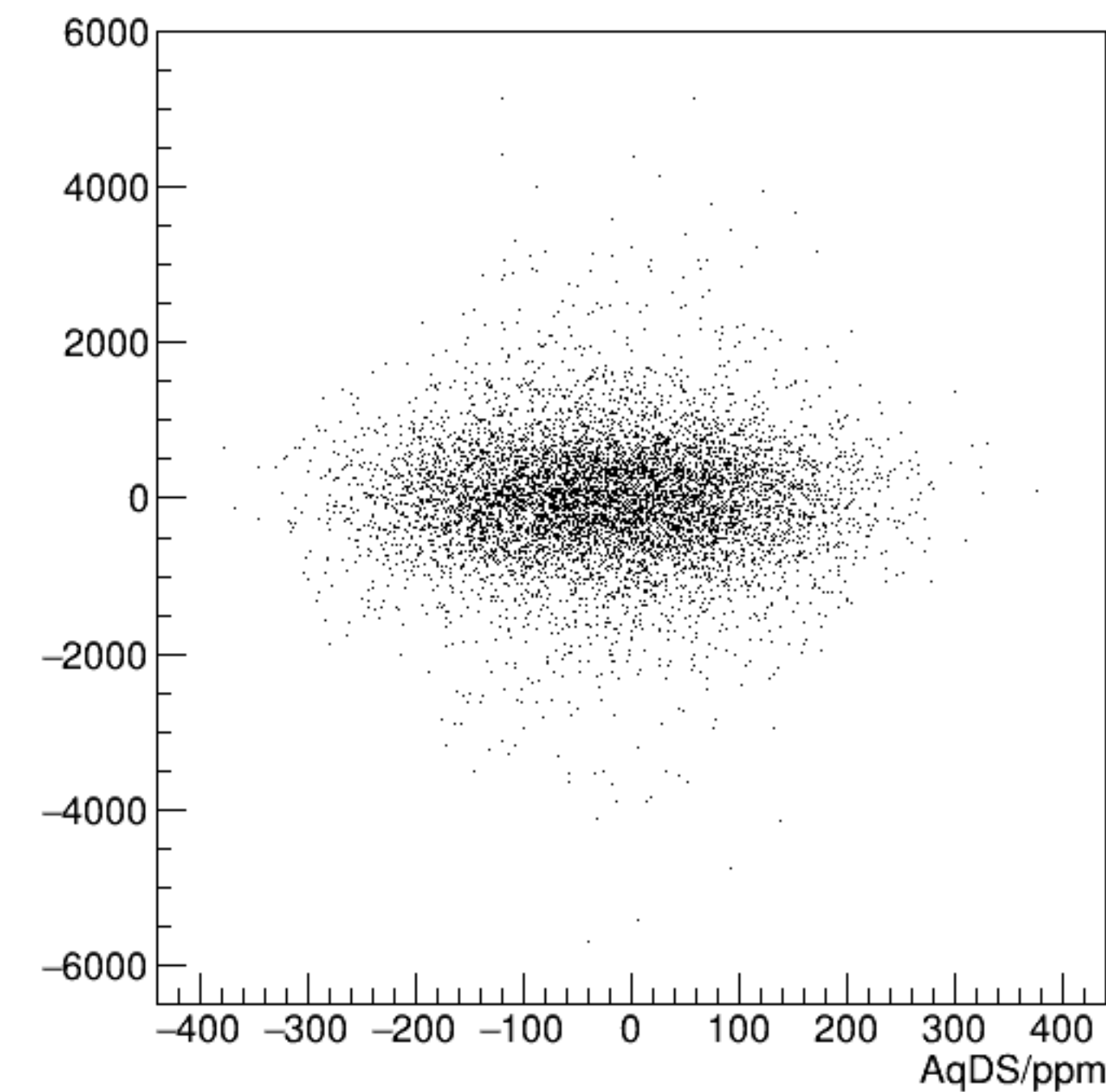
cor_sam7/ppm:AqDS/ppm {ErrorFlag==0}
