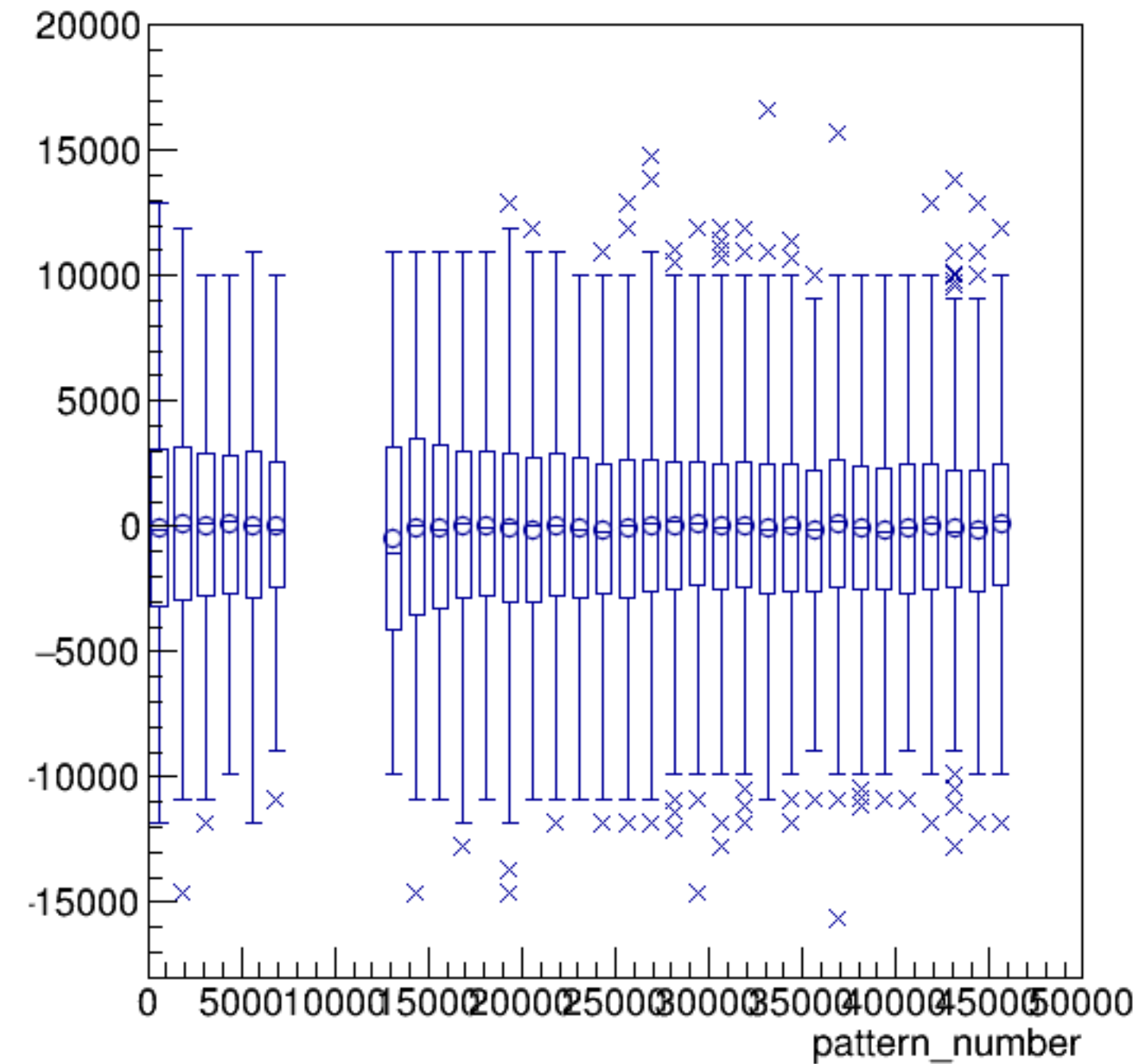
asym_usl/ppm:pattern_number {ErrorFlag==0}
