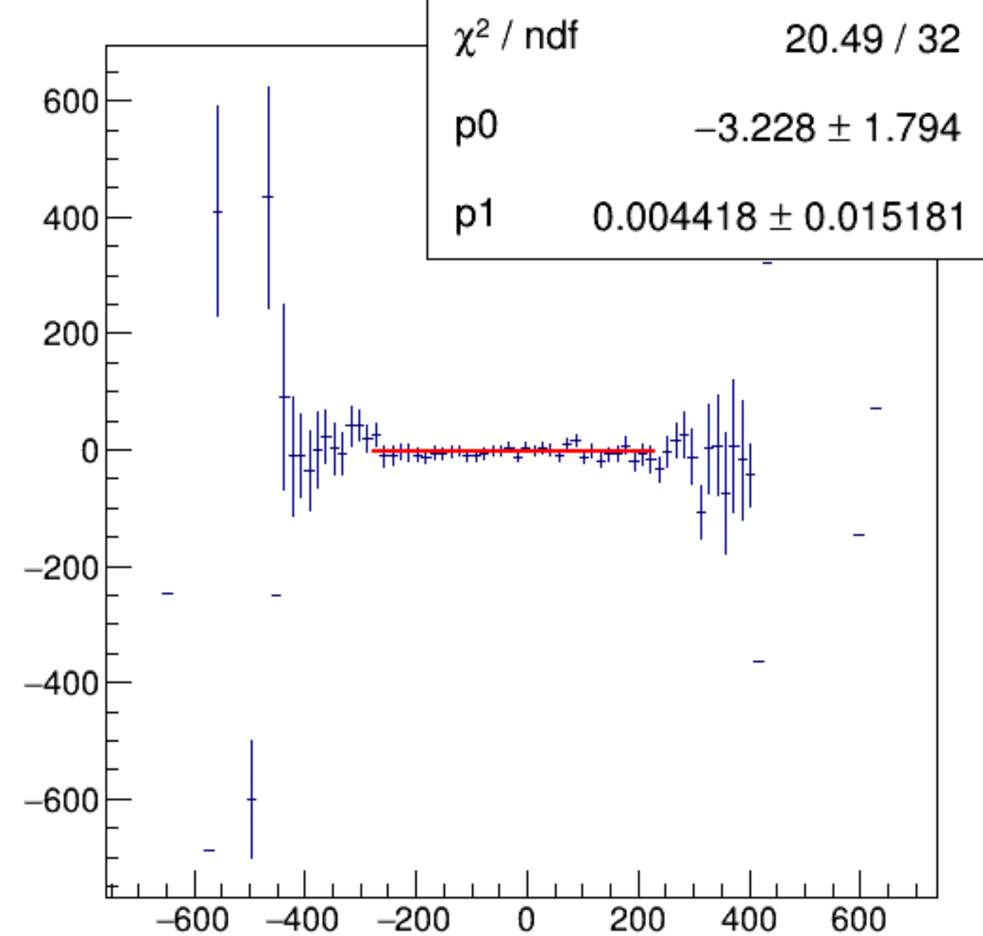
cor_usr/ppm:AqDS/ppm {ErrorFlag==0}
