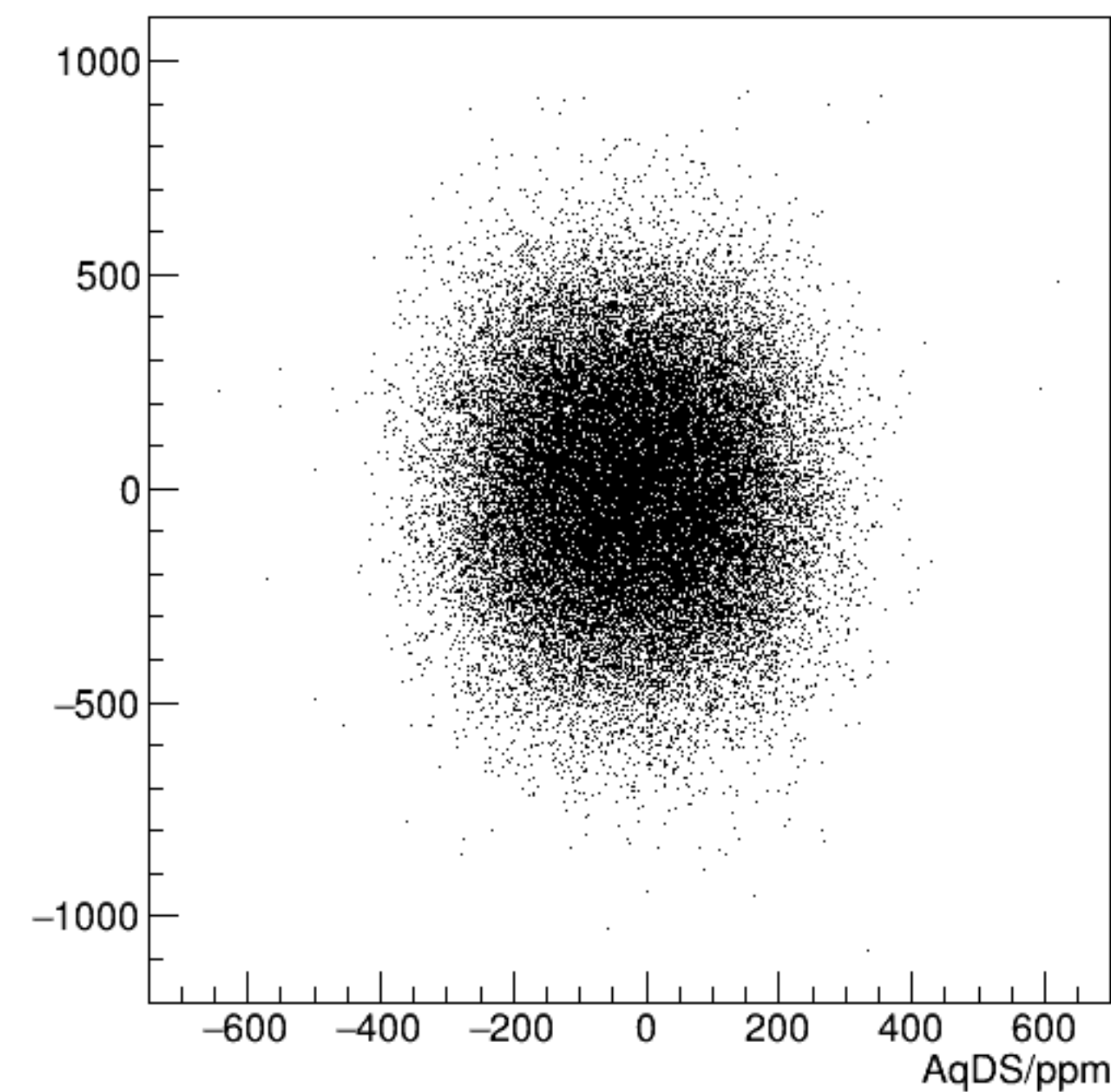
cor_usr/ppm:AqDS/ppm {ErrorFlag==0}
