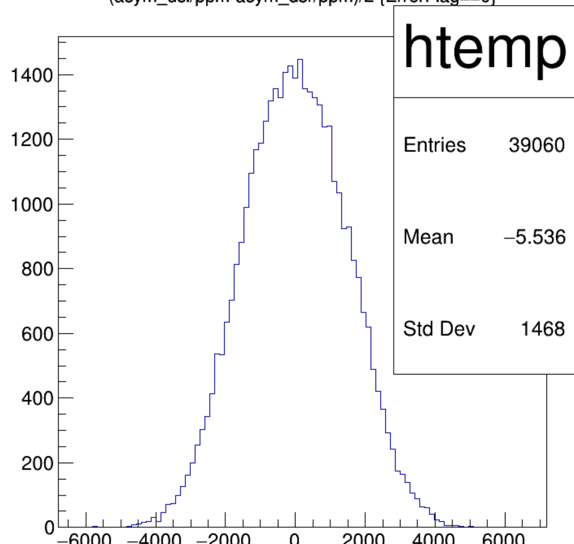
(asym_dsl/ppm-asym_dsr/ppm)/2 {ErrorFlag==0}
