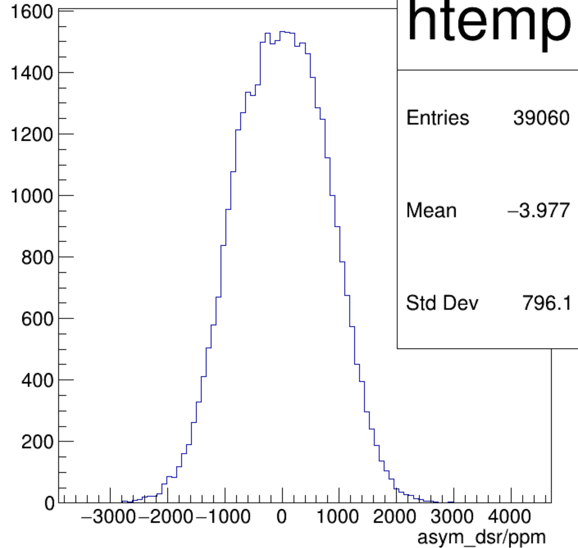
asym_dsr/ppm {ErrorFlag==0}
