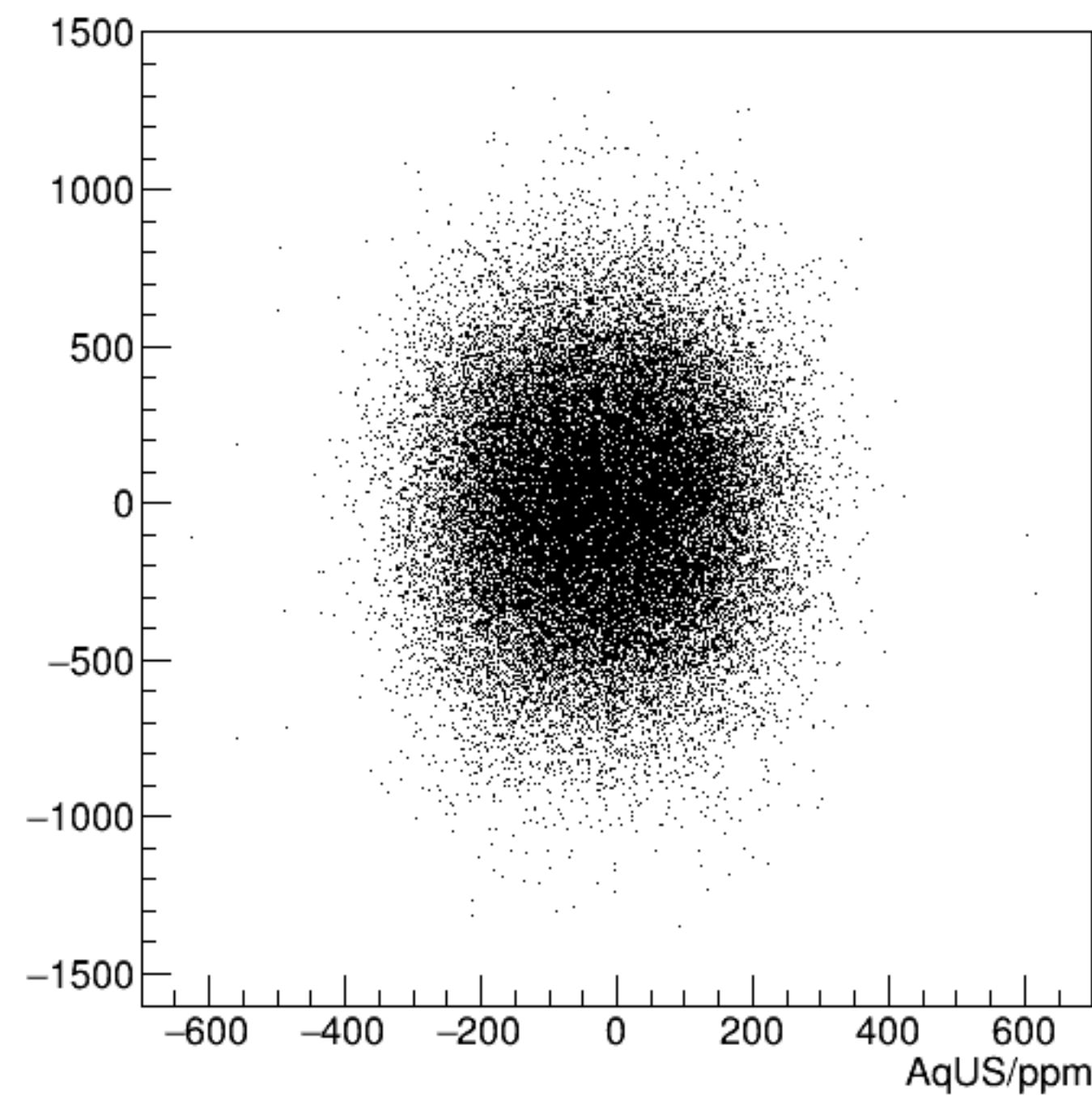
cor_dsl/ppm:AqUS/ppm {ErrorFlag==0}
