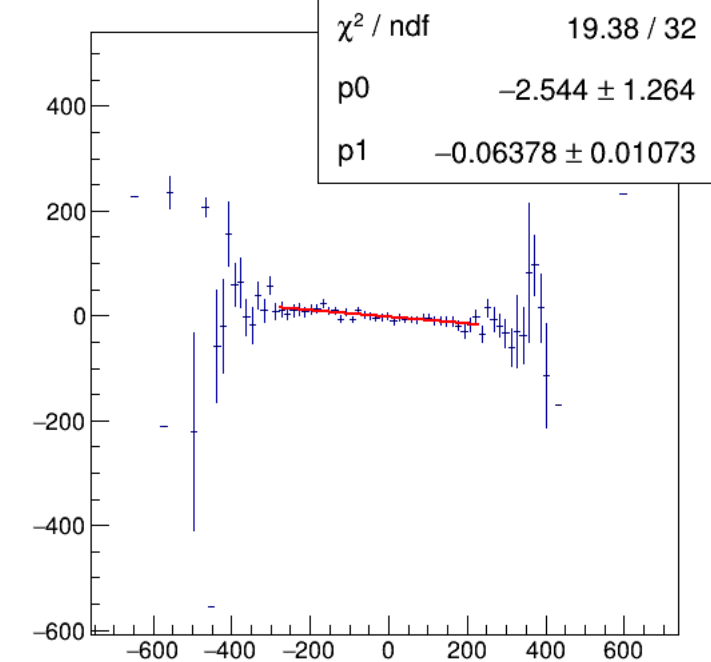
cor_usr/ppm:AqDS/ppm {ErrorFlag==0}
