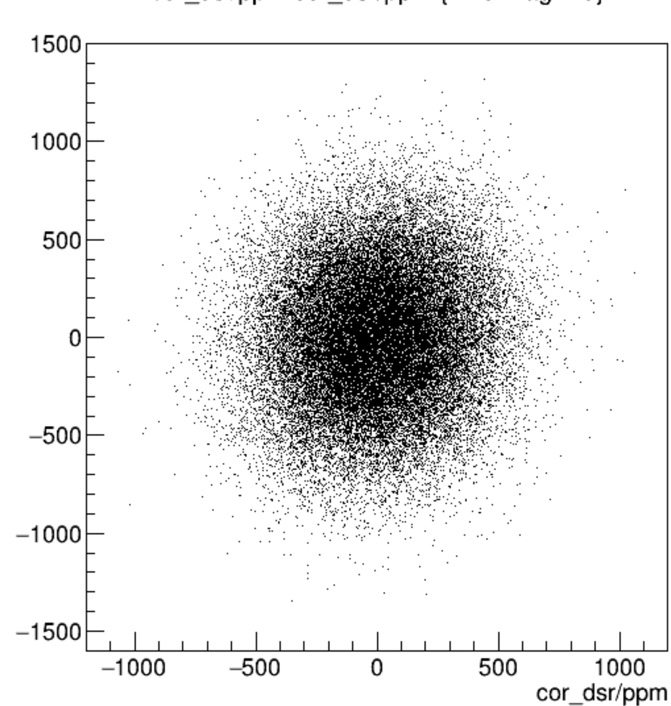
cor_dsl/ppm:cor_dsr/ppm {ErrorFlag==0}
