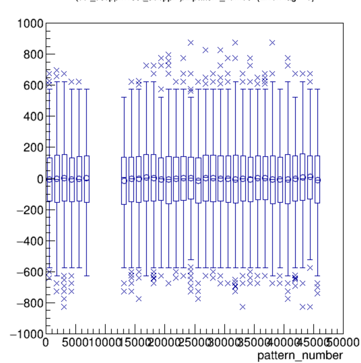
(cor_usl/ppm+cor_usr/ppm)/2:pattern_number {ErrorFlag==0}
