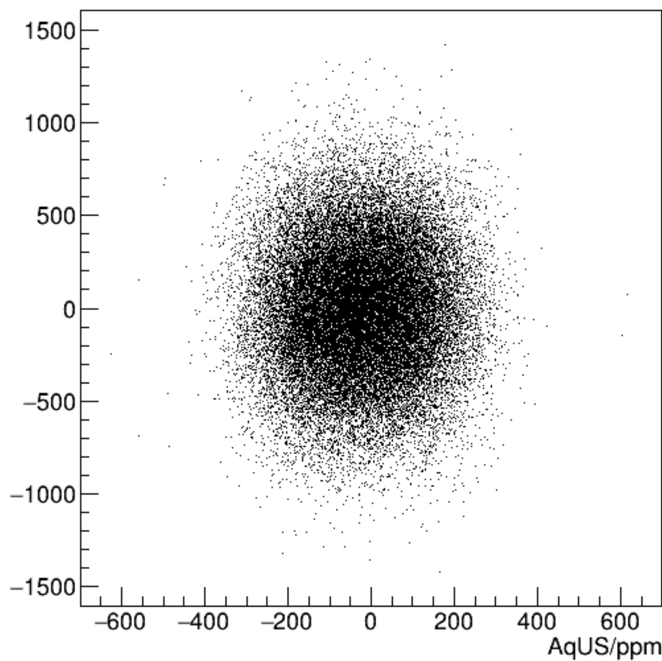
cor_usl/ppm:AqUS/ppm {ErrorFlag==0}
