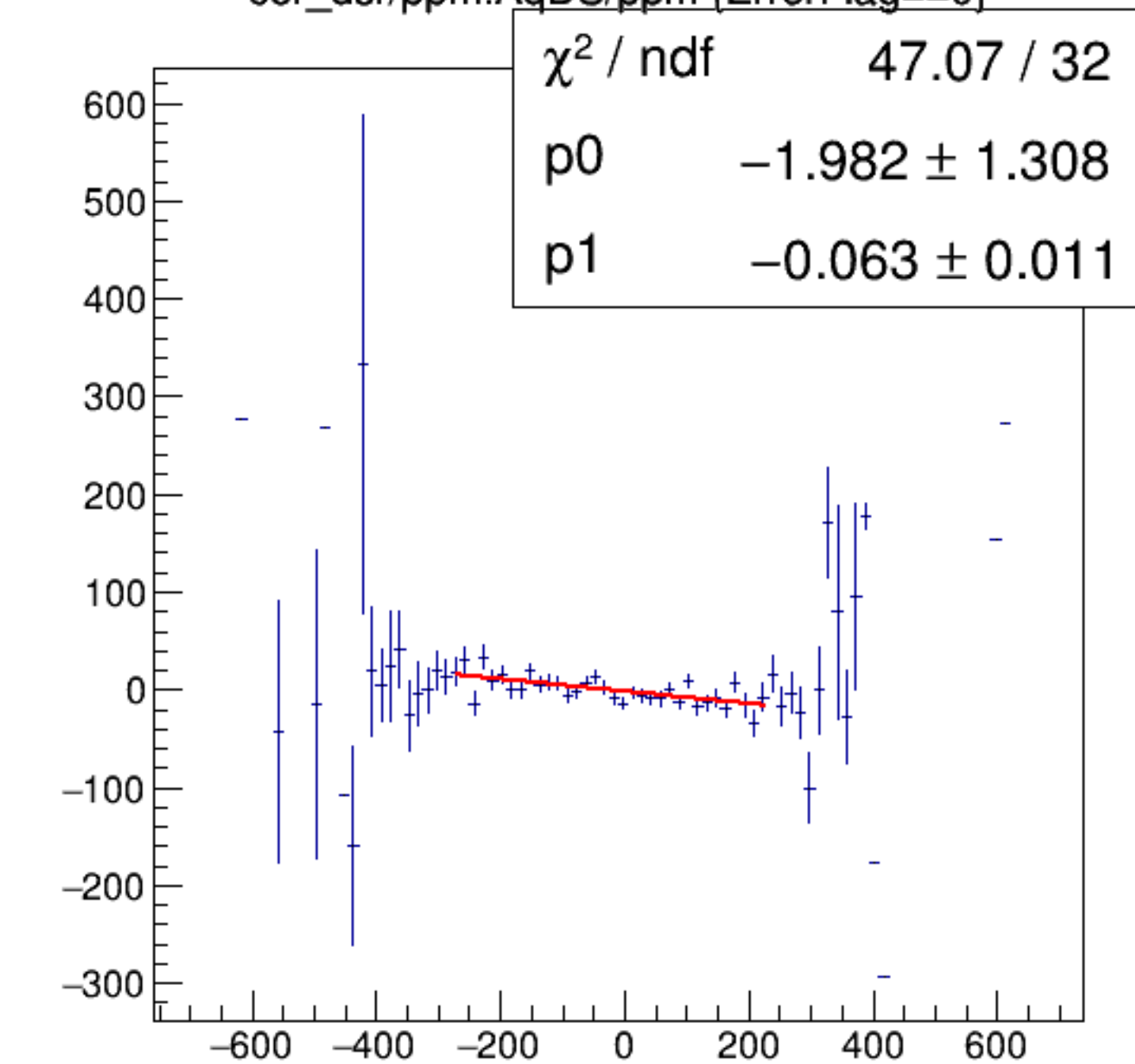
cor_dsr/ppm:AqDS/ppm {ErrorFlag==0}
