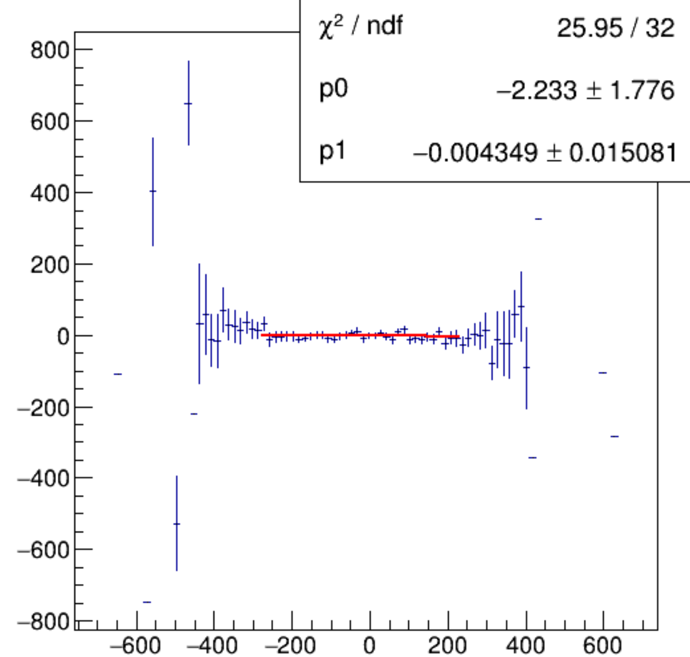
cor_dsl/ppm:AqDS/ppm {ErrorFlag==0}
