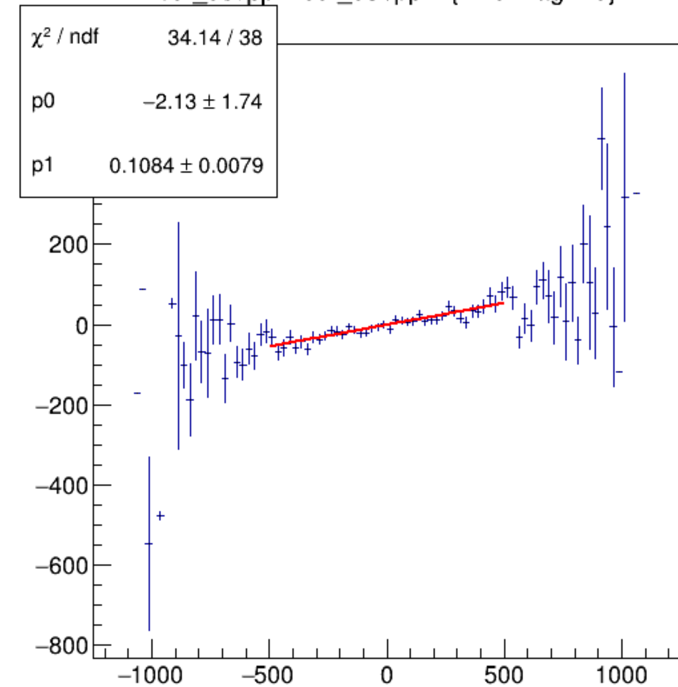
cor_dsl/ppm:cor_dsr/ppm {ErrorFlag==0}
