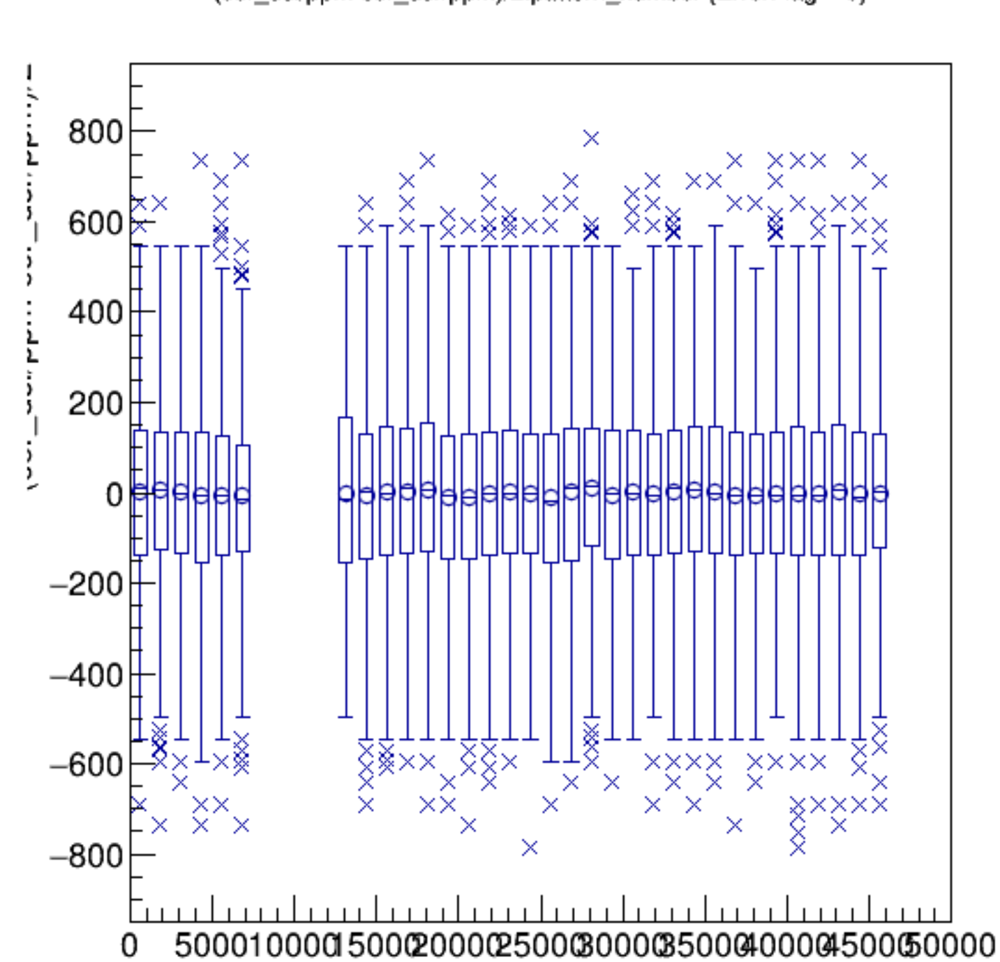
(cor_dsl/ppm-cor_dsr/ppm)/2:pattern_number {ErrorFlag==0}
