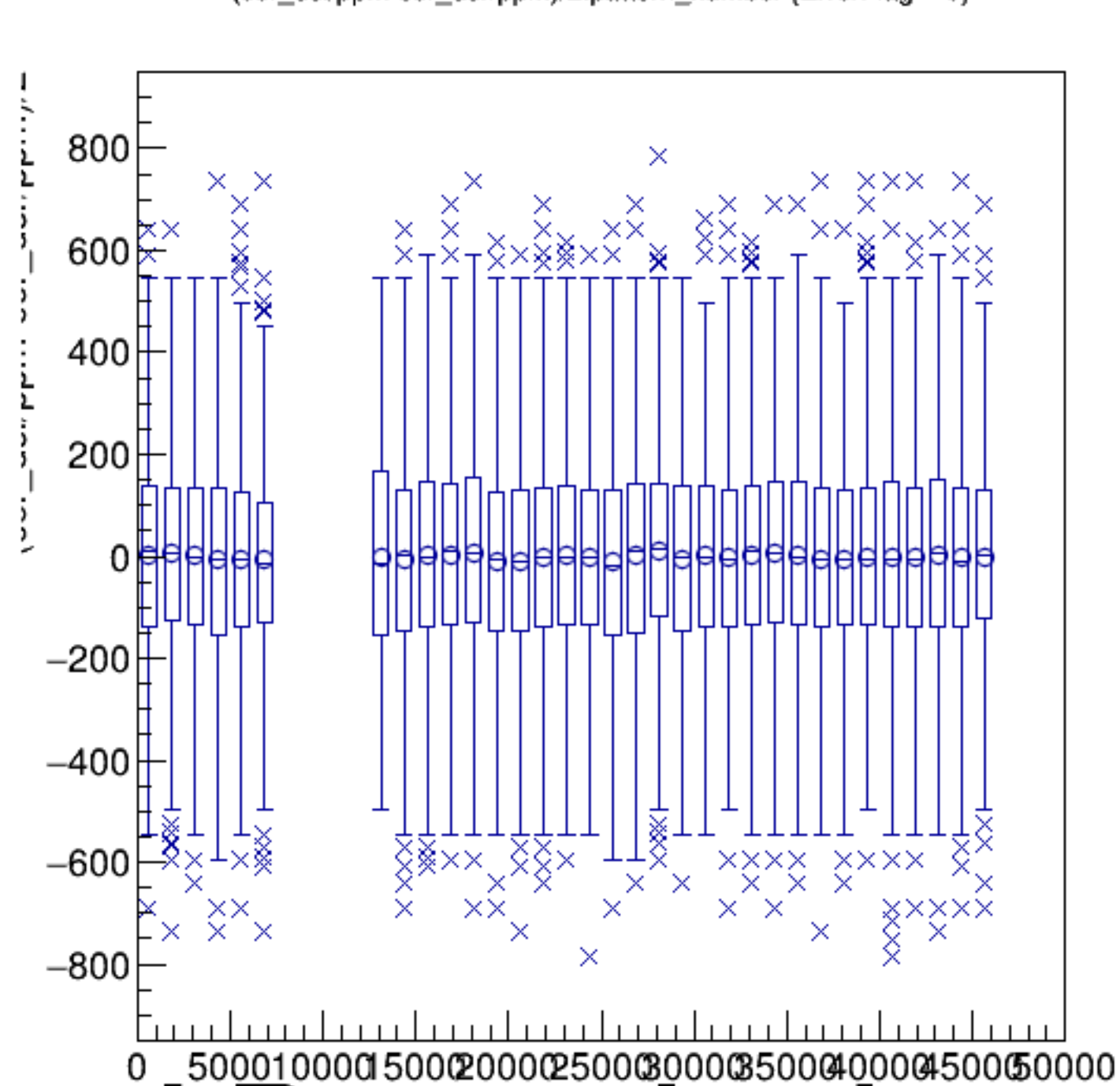
(cor_dsl/ppm-cor_dsr/ppm)/2:pattern_number {ErrorFlag==0}
