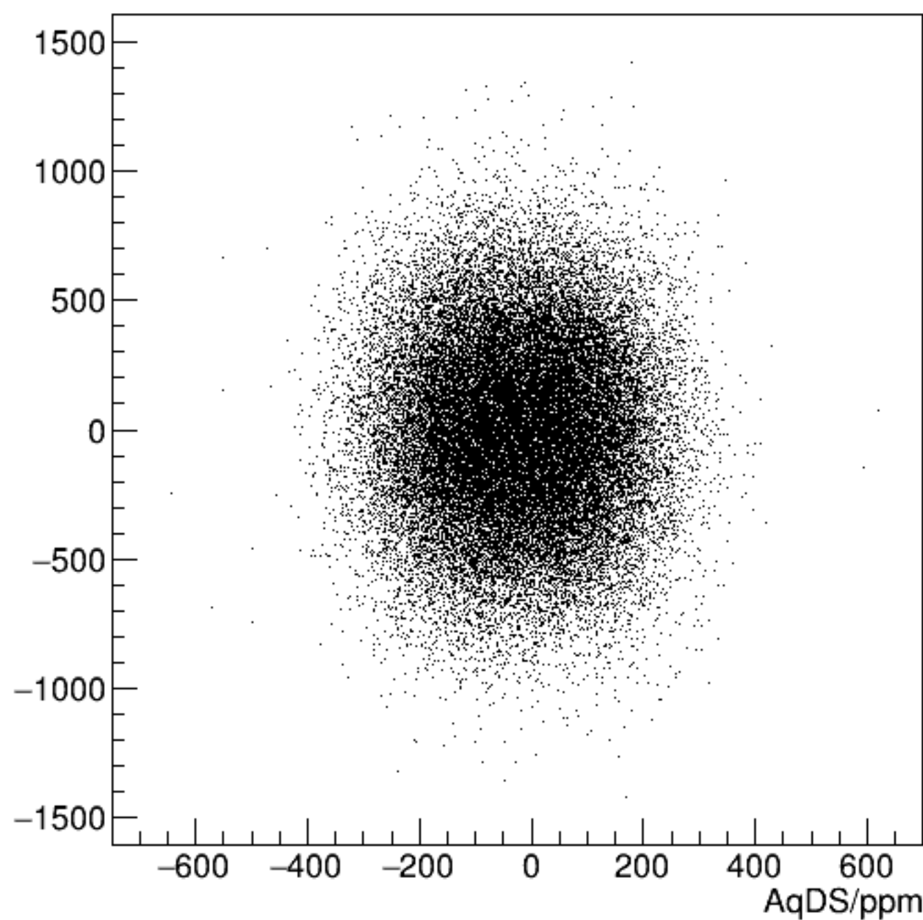
cor_usr/ppm:AqDS/ppm {ErrorFlag==0}
