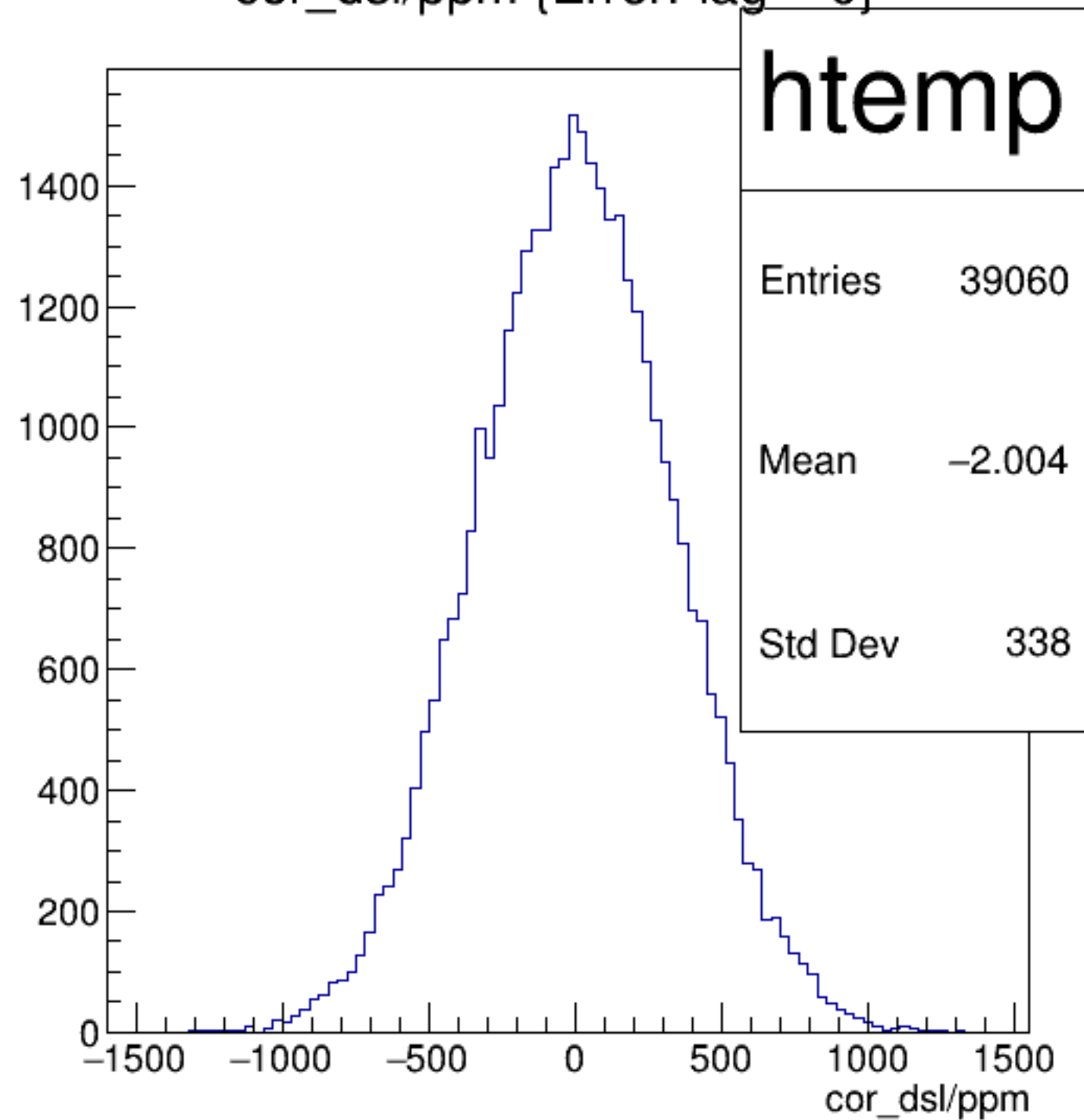
cor_dsl/ppm {ErrorFlag==0}
