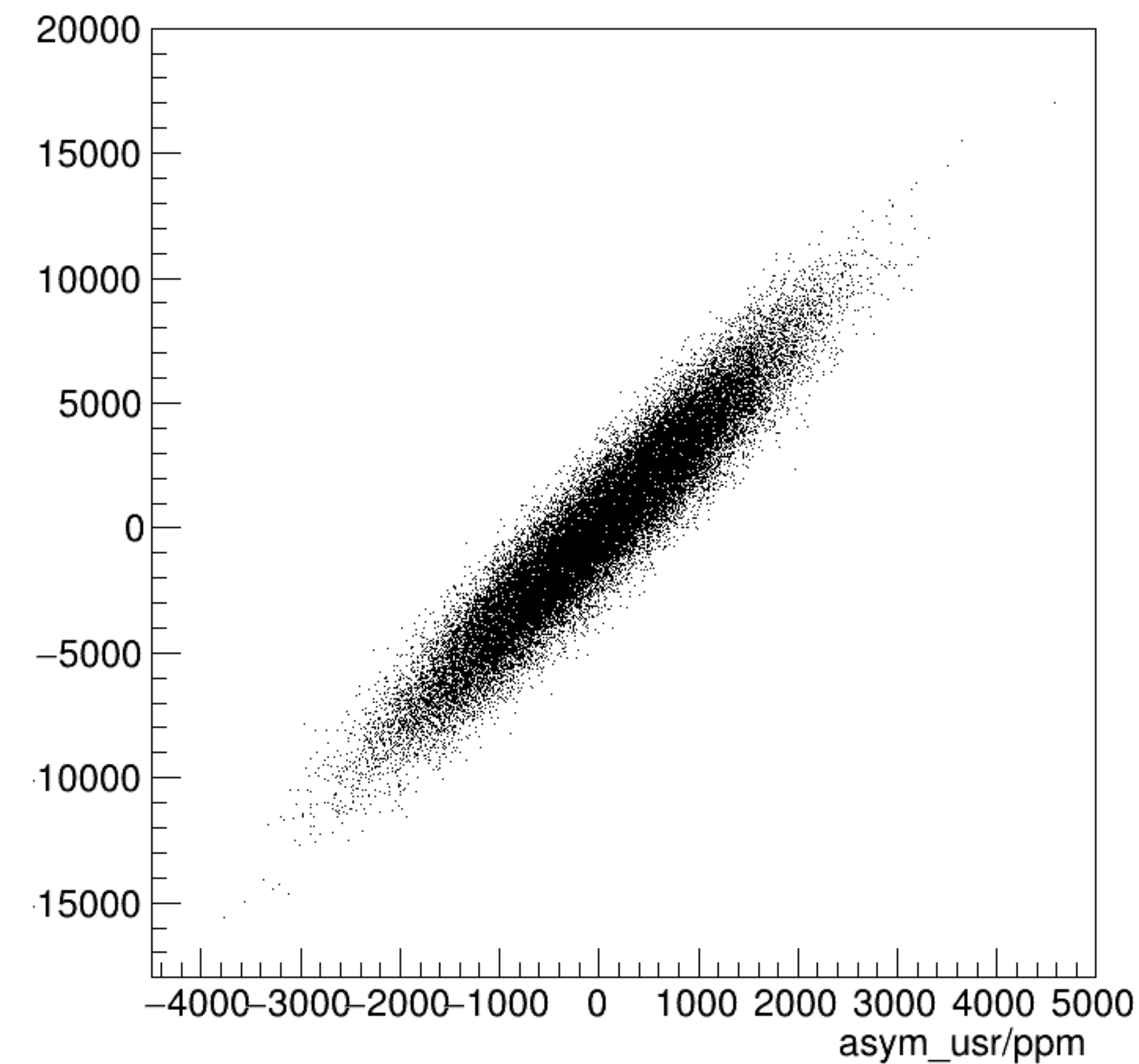
asym_usl/ppm:asym_usr/ppm {ErrorFlag==0}
