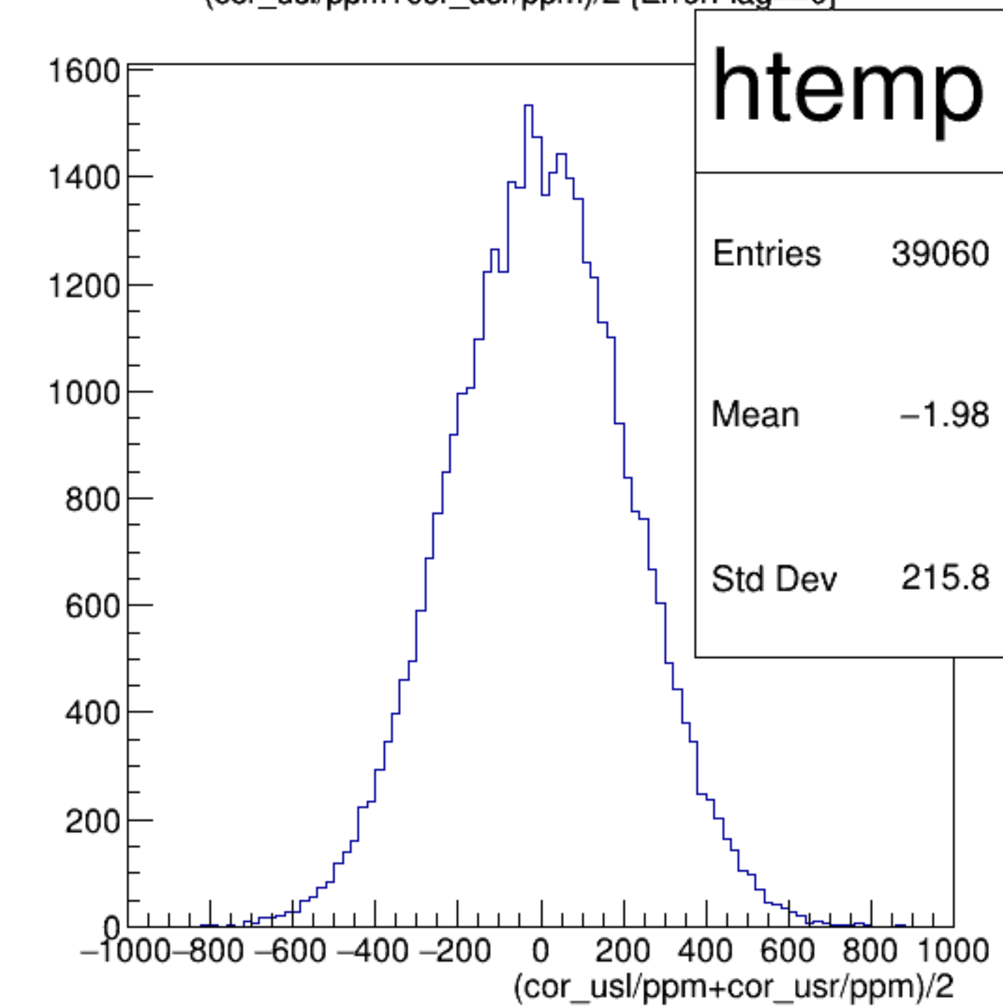
(cor_usl/ppm+cor_usr/ppm)/2 {ErrorFlag==0}
