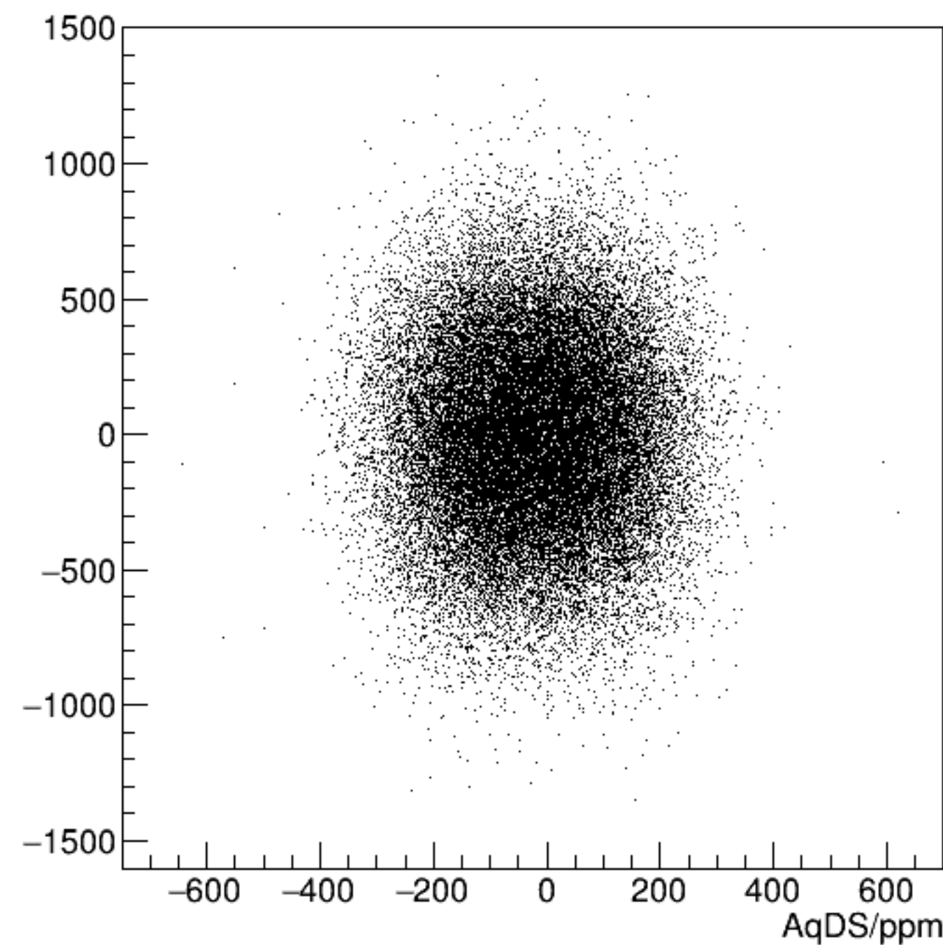
cor_dsl/ppm:AqDS/ppm {ErrorFlag==0}
