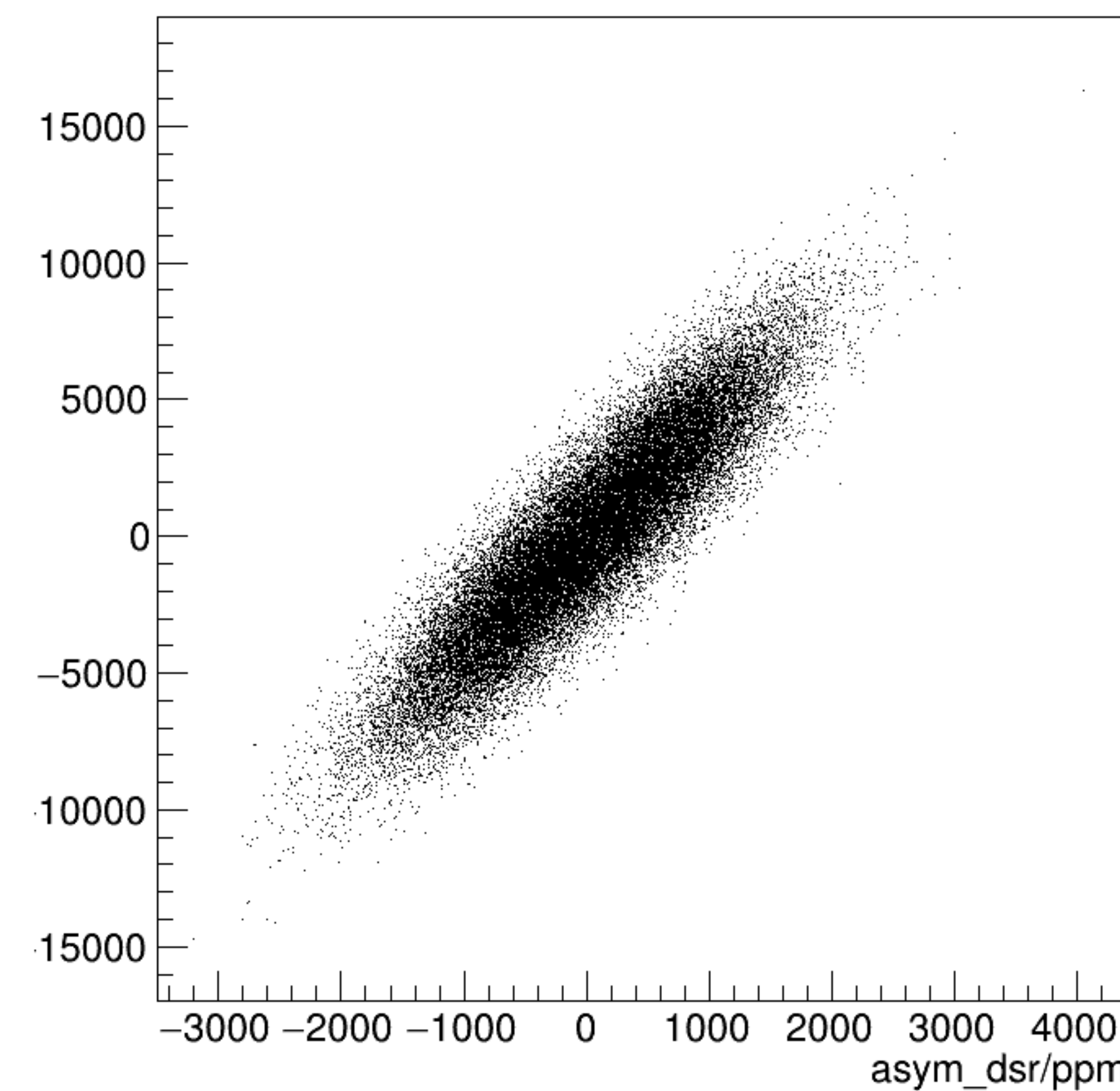
asym_dsl/ppm:asym_dsr/ppm {ErrorFlag==0}
