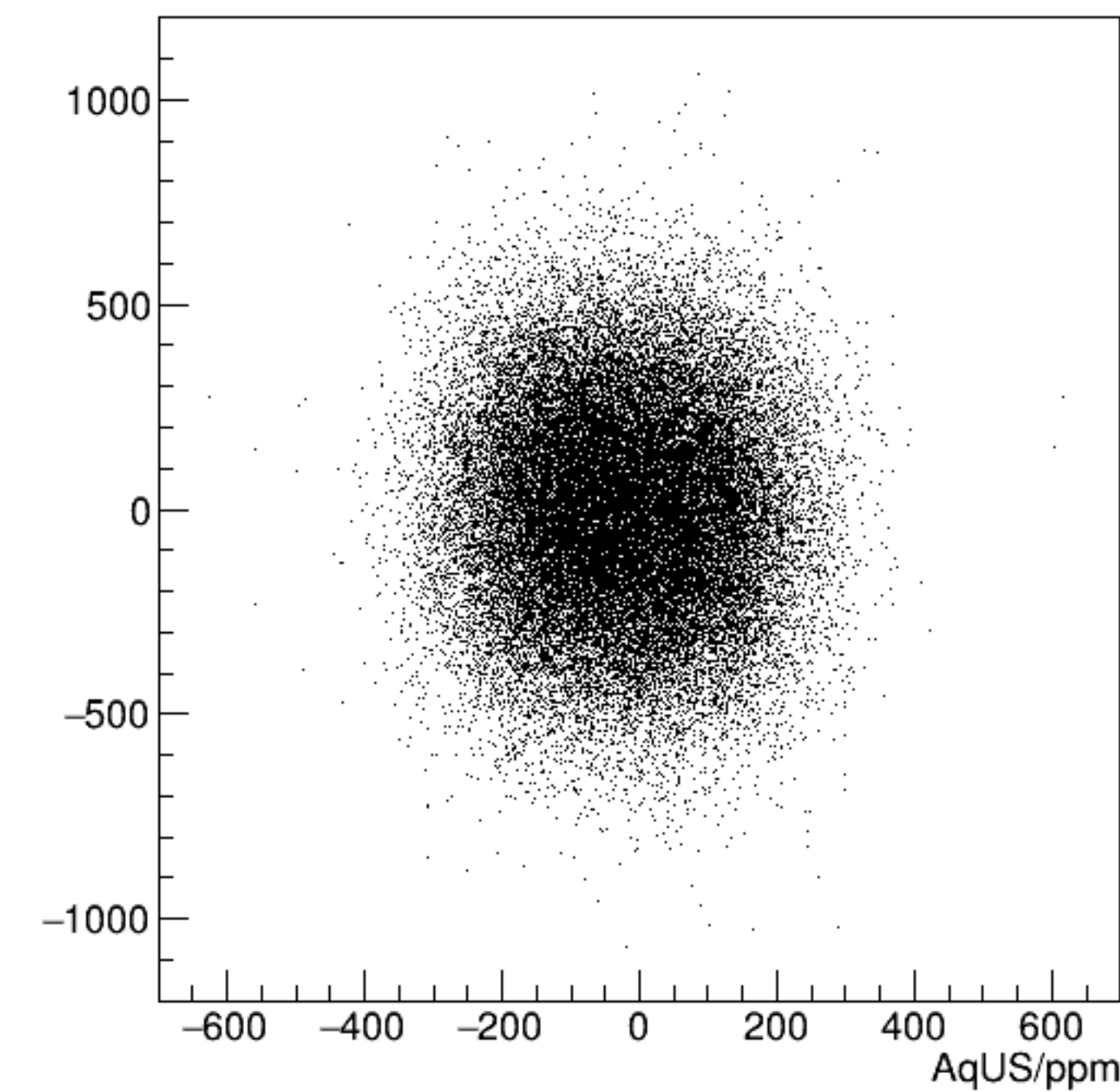
cor_dsr/ppm:AqUS/ppm {ErrorFlag==0}
