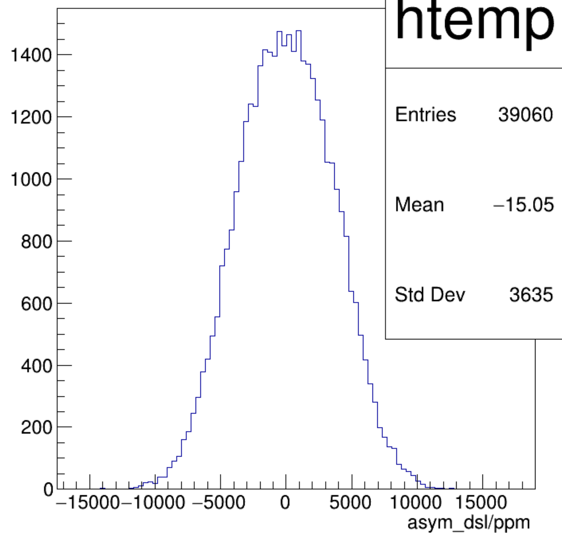
asym_dsl/ppm {ErrorFlag==0}
