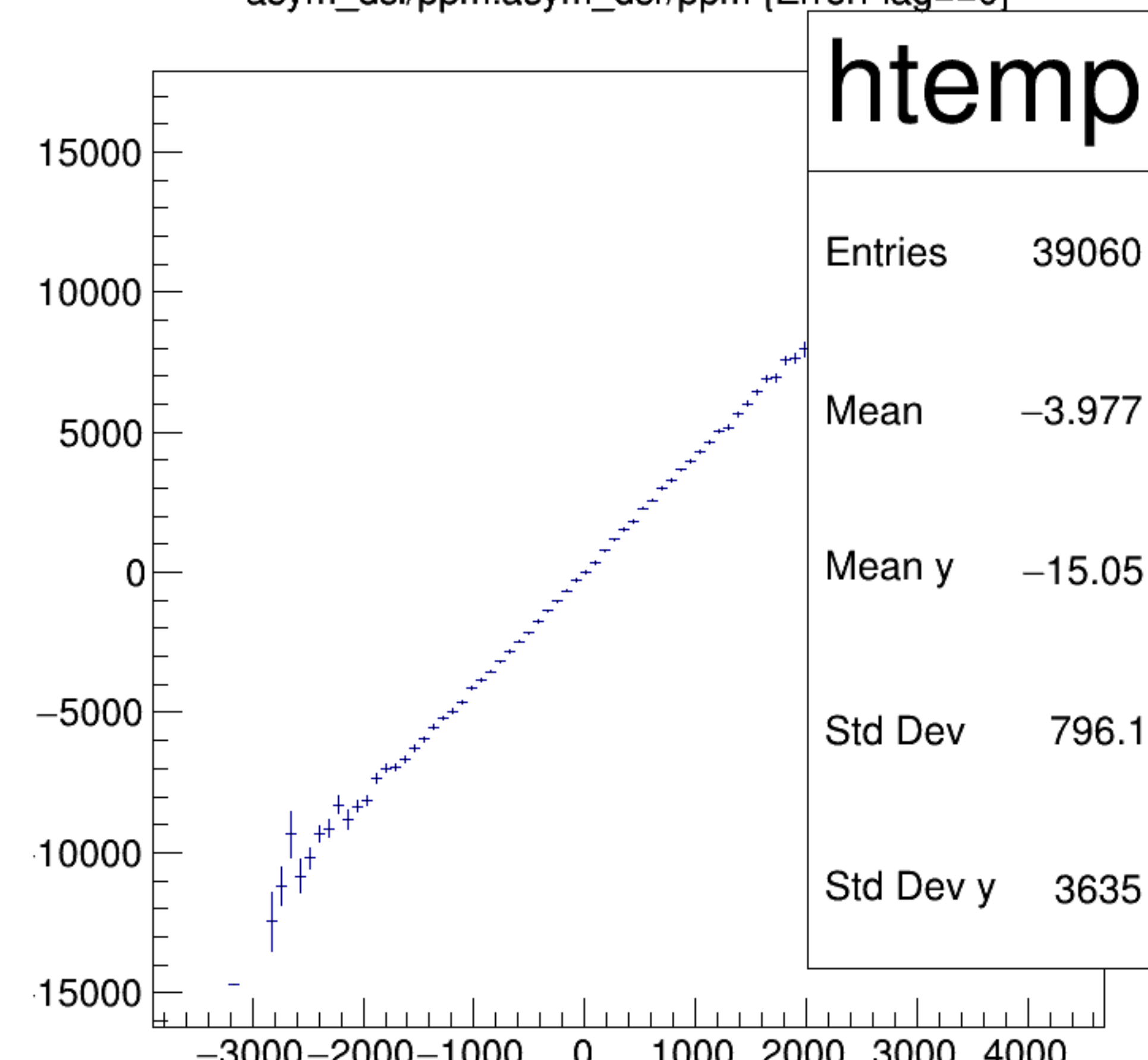
asym_dsl/ppm:asym_dsr/ppm {ErrorFlag==0}
