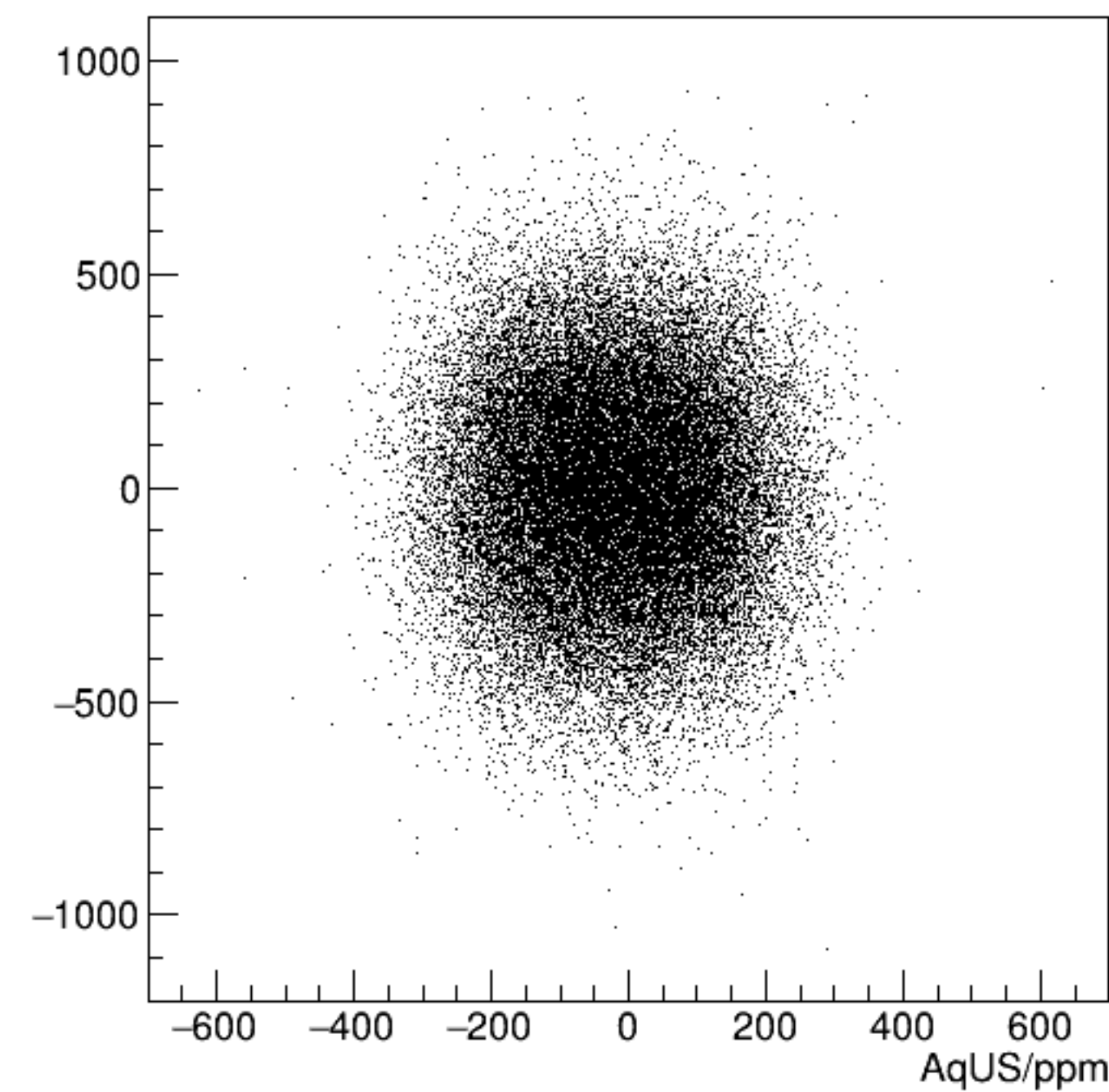
cor_usr/ppm:AqUS/ppm {ErrorFlag==0}
