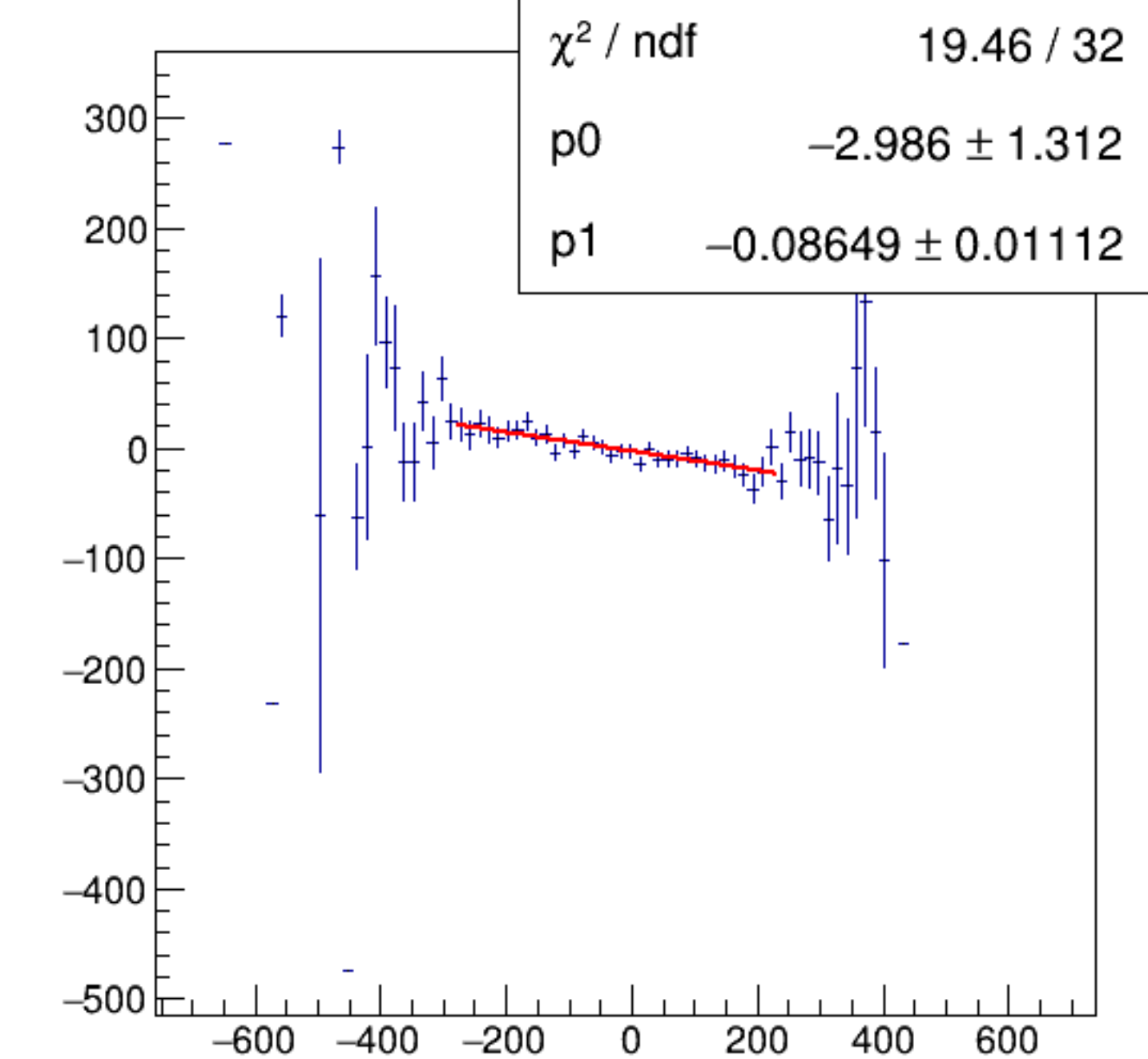
cor_dsr/ppm:AqDS/ppm {ErrorFlag==0}
