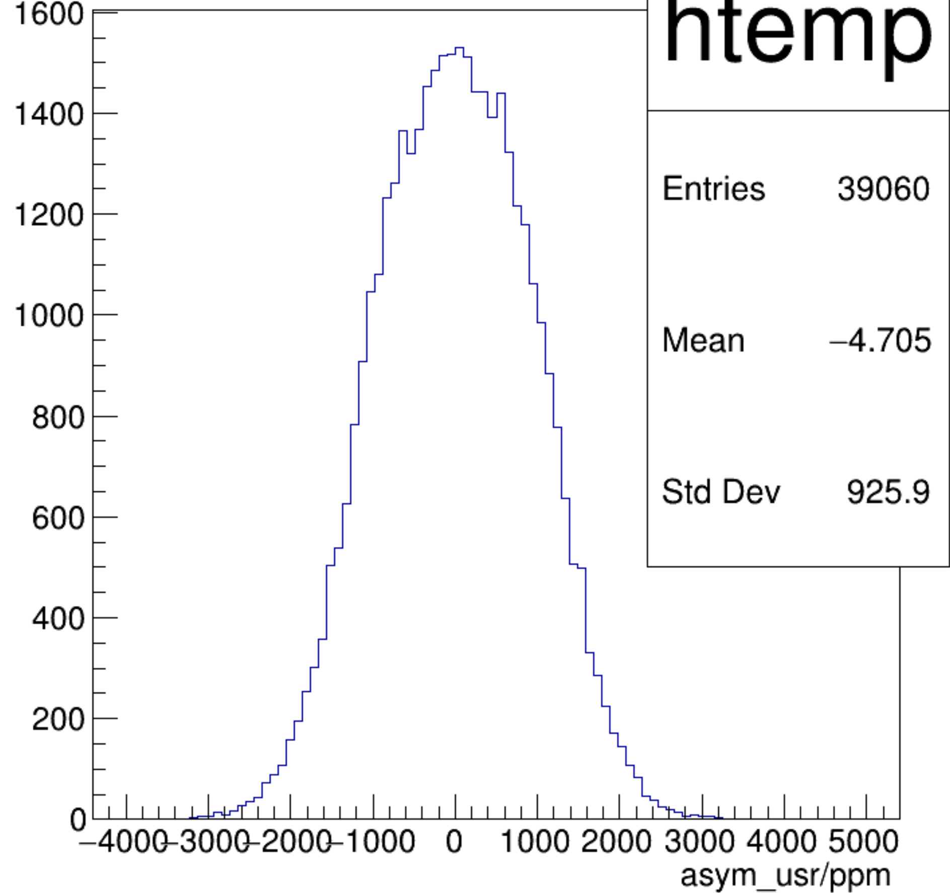
asym_usr/ppm {ErrorFlag==0}
