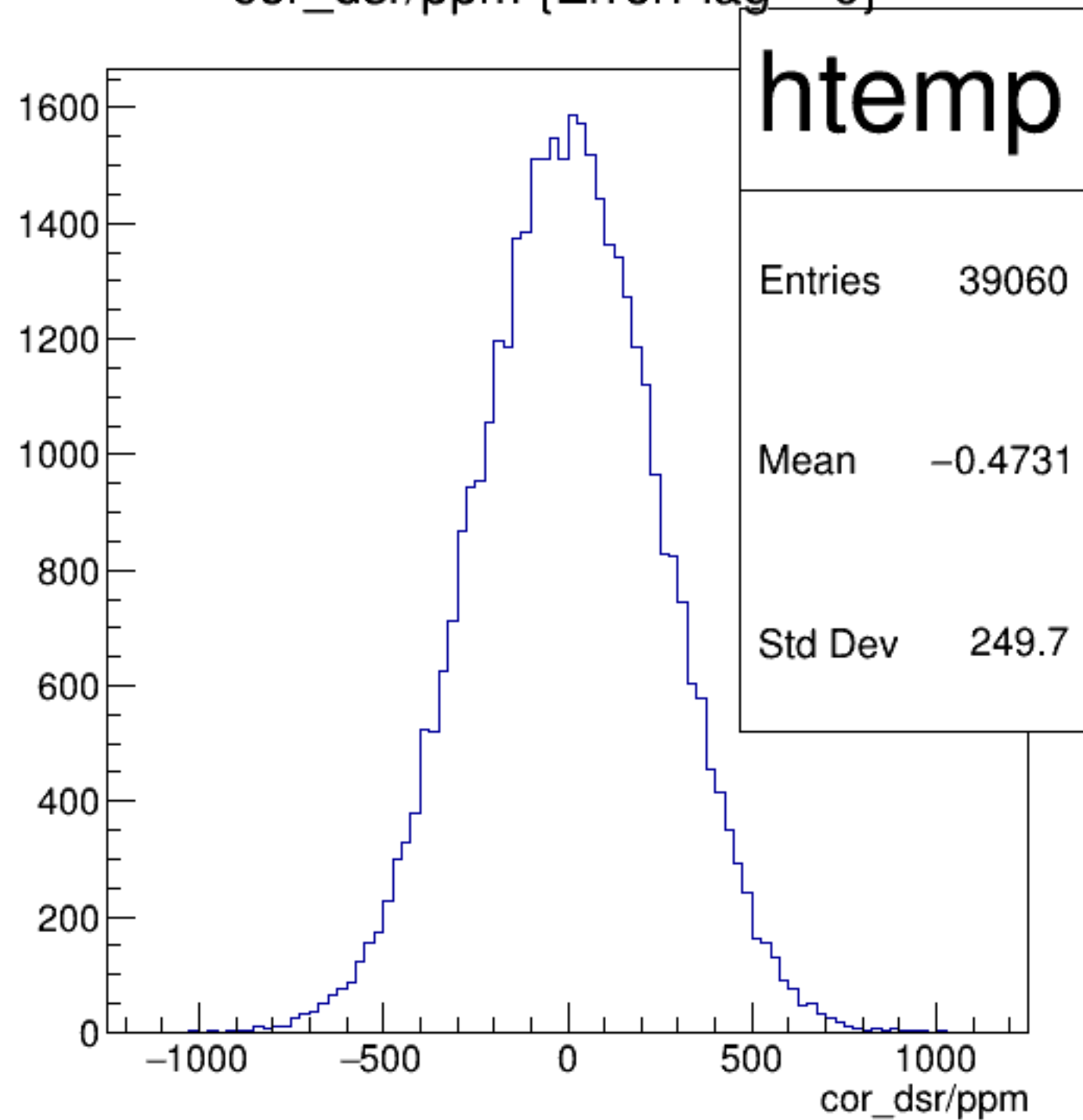
cor_dsr/ppm {ErrorFlag==0}
