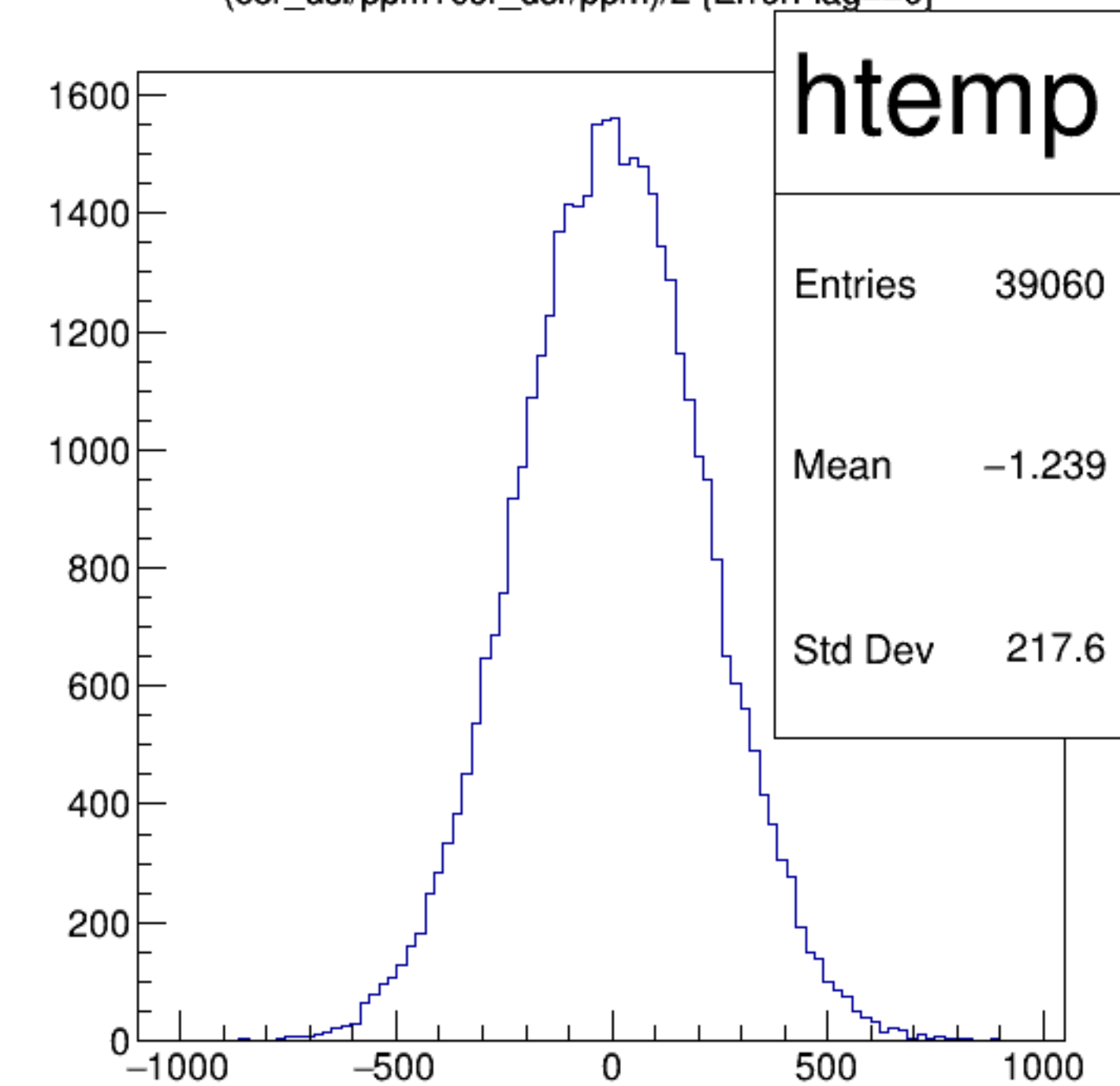
(cor_dsl/ppm+cor_dsr/ppm)/2 {ErrorFlag==0}
