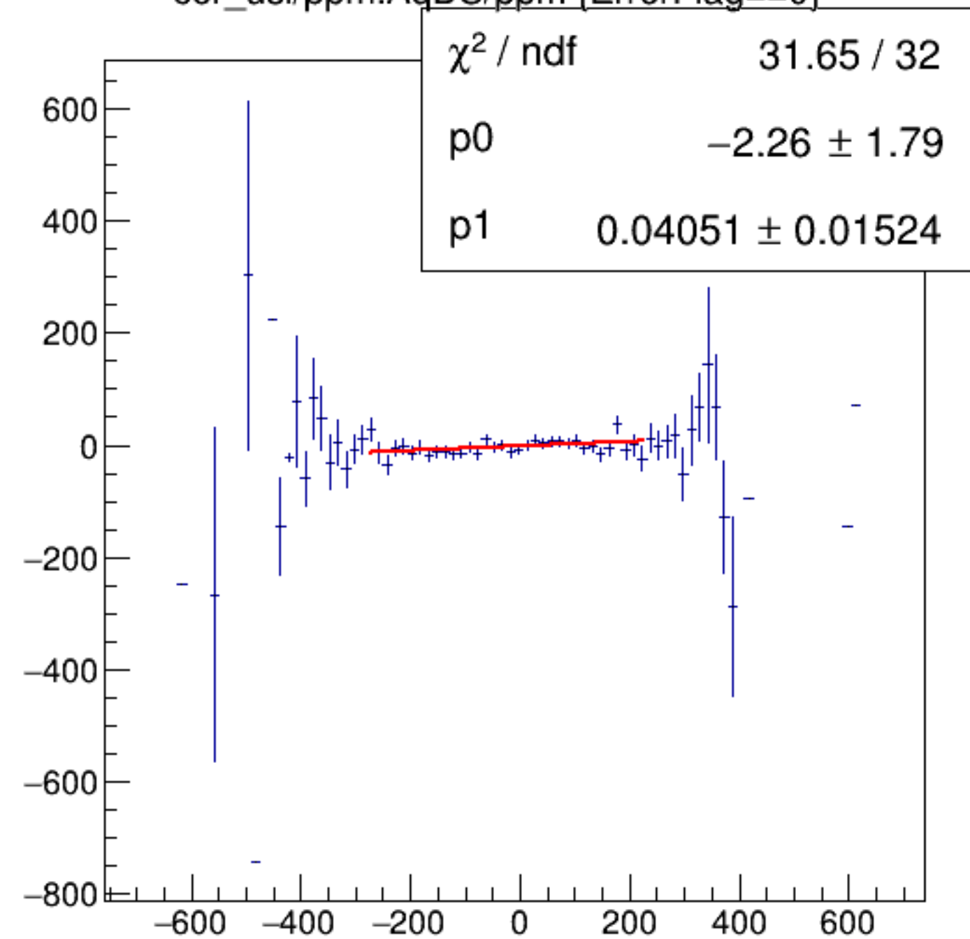
cor_usl/ppm:AqDS/ppm {ErrorFlag==0}
