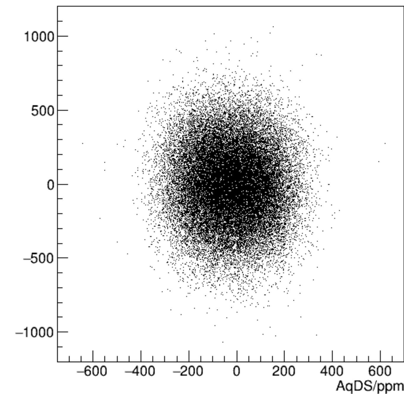
cor_dsr/ppm:AqDS/ppm {ErrorFlag==0}
