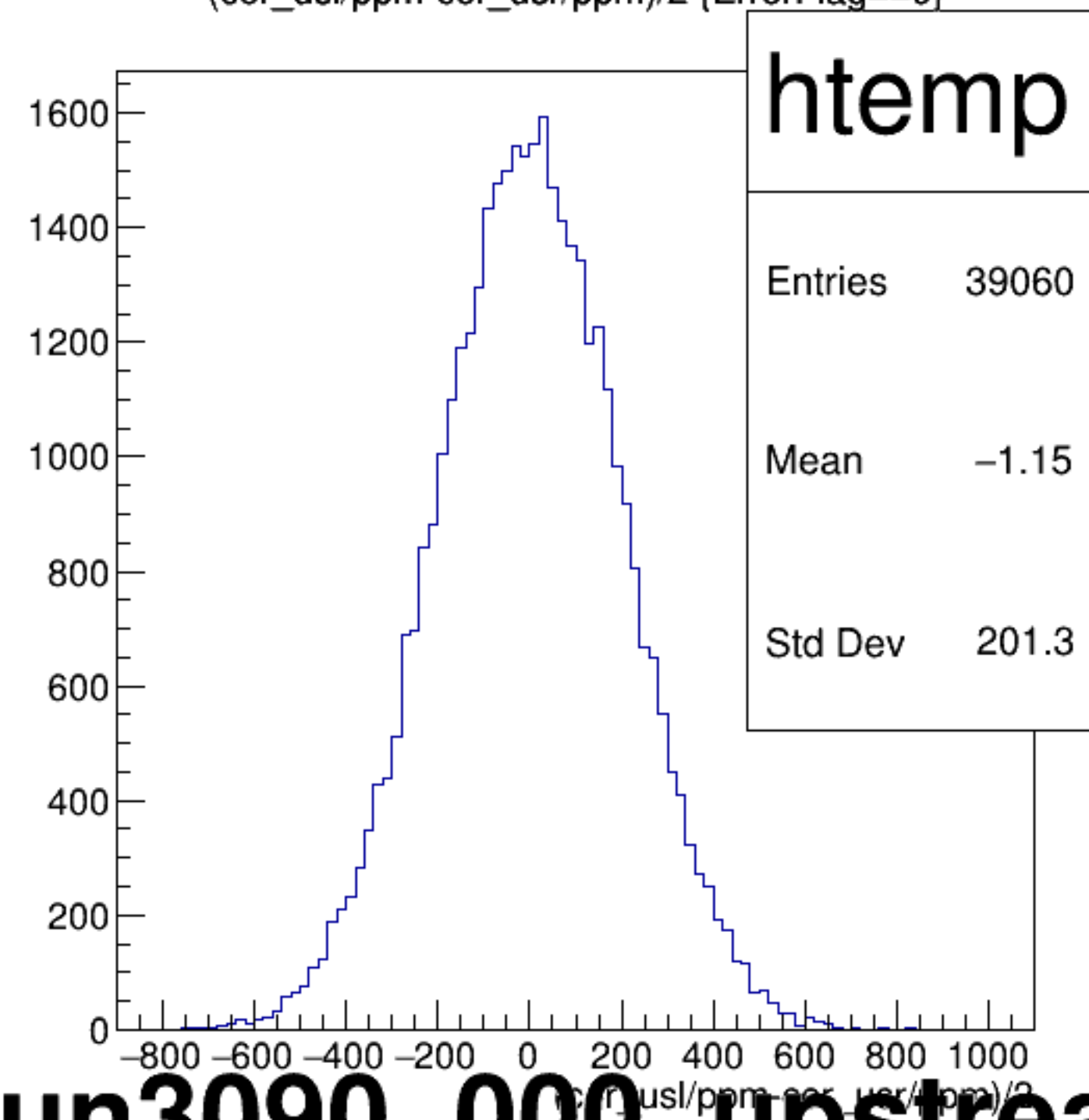
(cor_usl/ppm-cor_usr/ppm)/2 {ErrorFlag==0}
