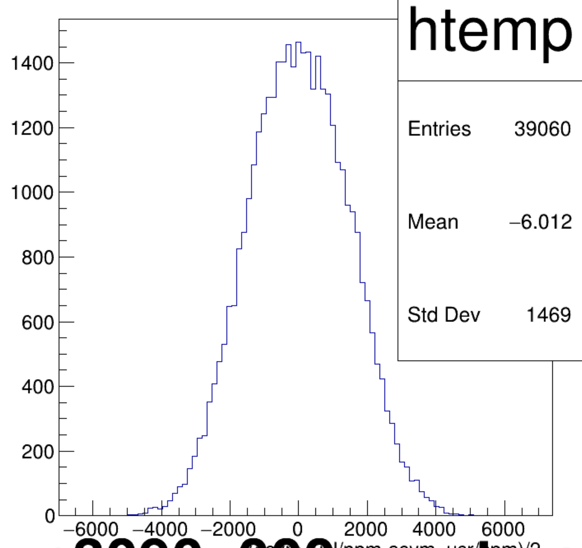
(asym_usl/ppm-asym_usr/ppm)/2 {ErrorFlag==0}
