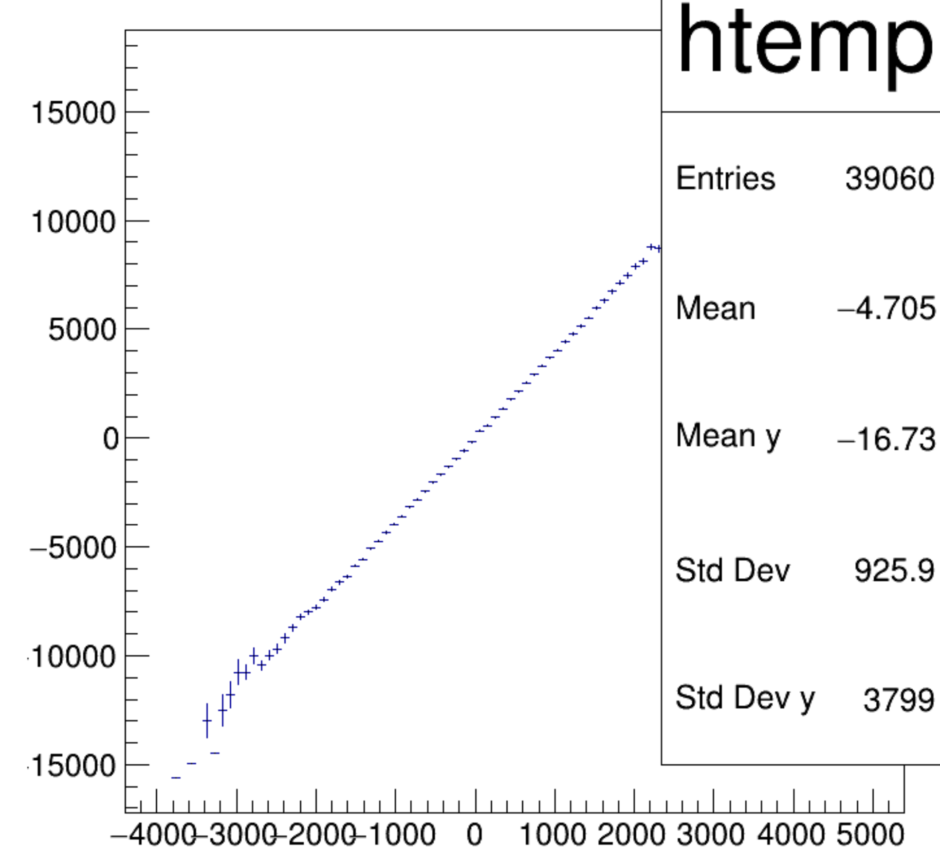
asym_usl/ppm:asym_usr/ppm {ErrorFlag==0}
