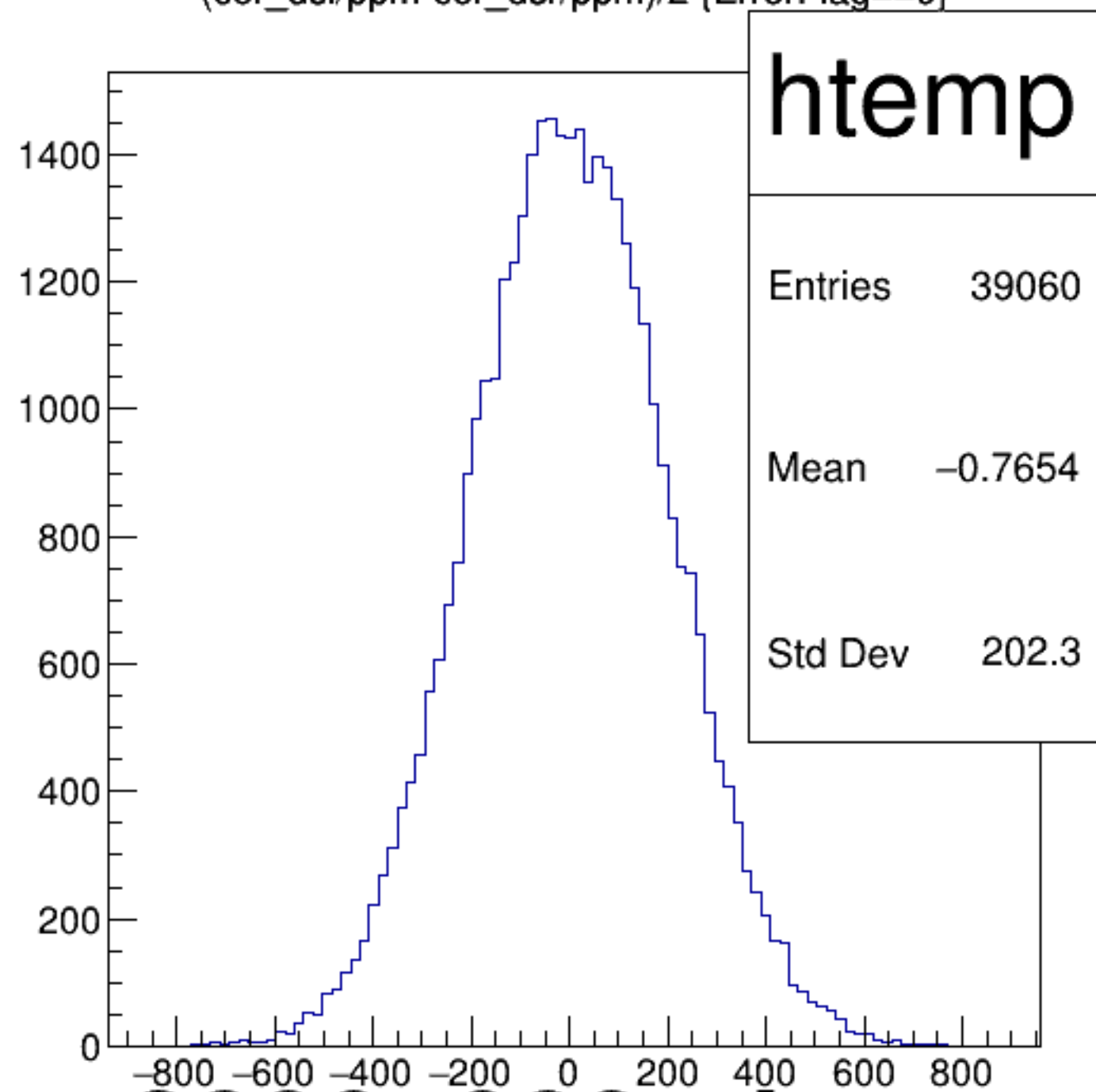
(cor_dsl/ppm-cor_dsr/ppm)/2 {ErrorFlag==0}
