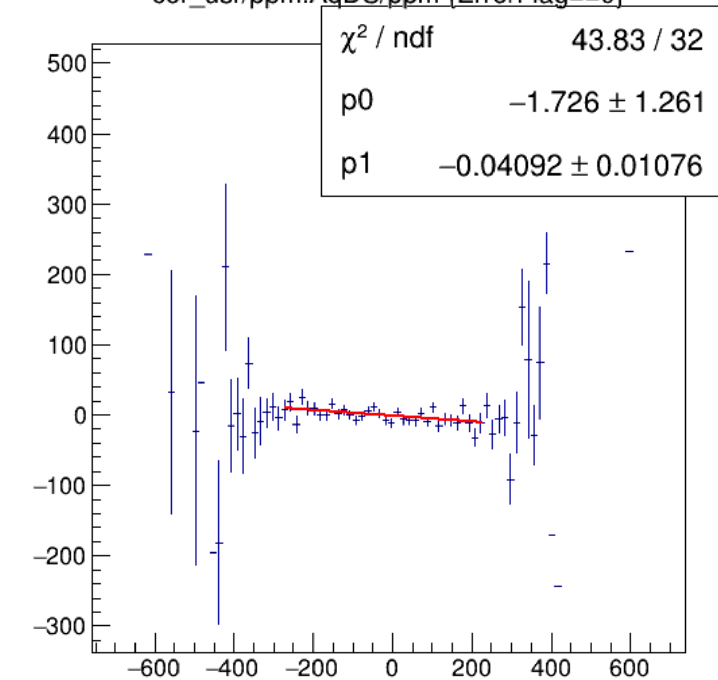
cor_usr/ppm:AqDS/ppm {ErrorFlag==0}
