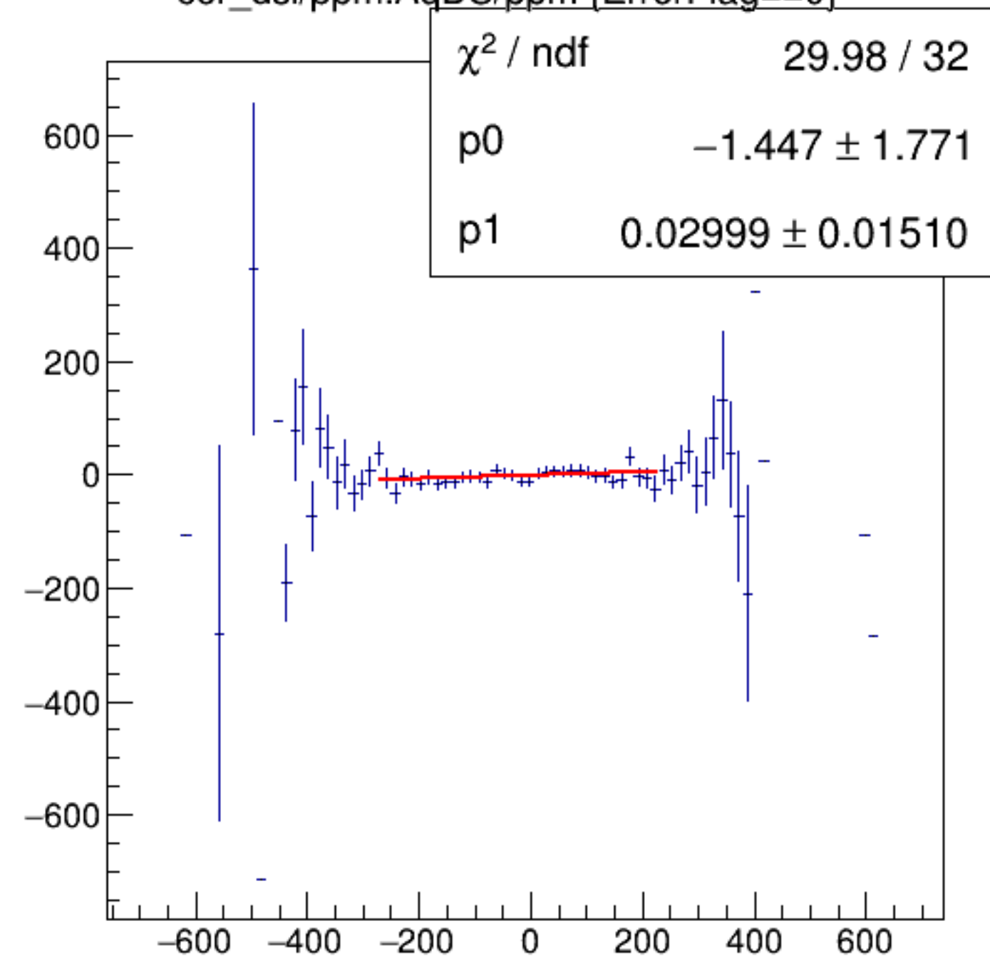
cor_dsl/ppm:AqDS/ppm {ErrorFlag==0}
