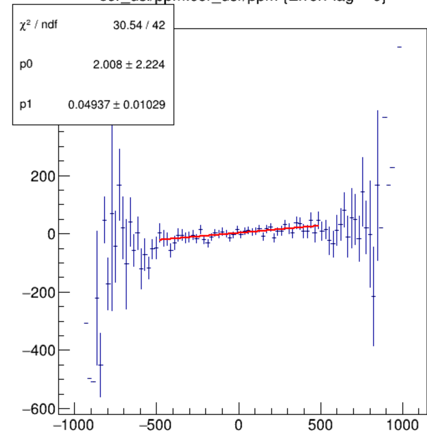
cor_dsl/ppm:cor_dsr/ppm {ErrorFlag==0}
