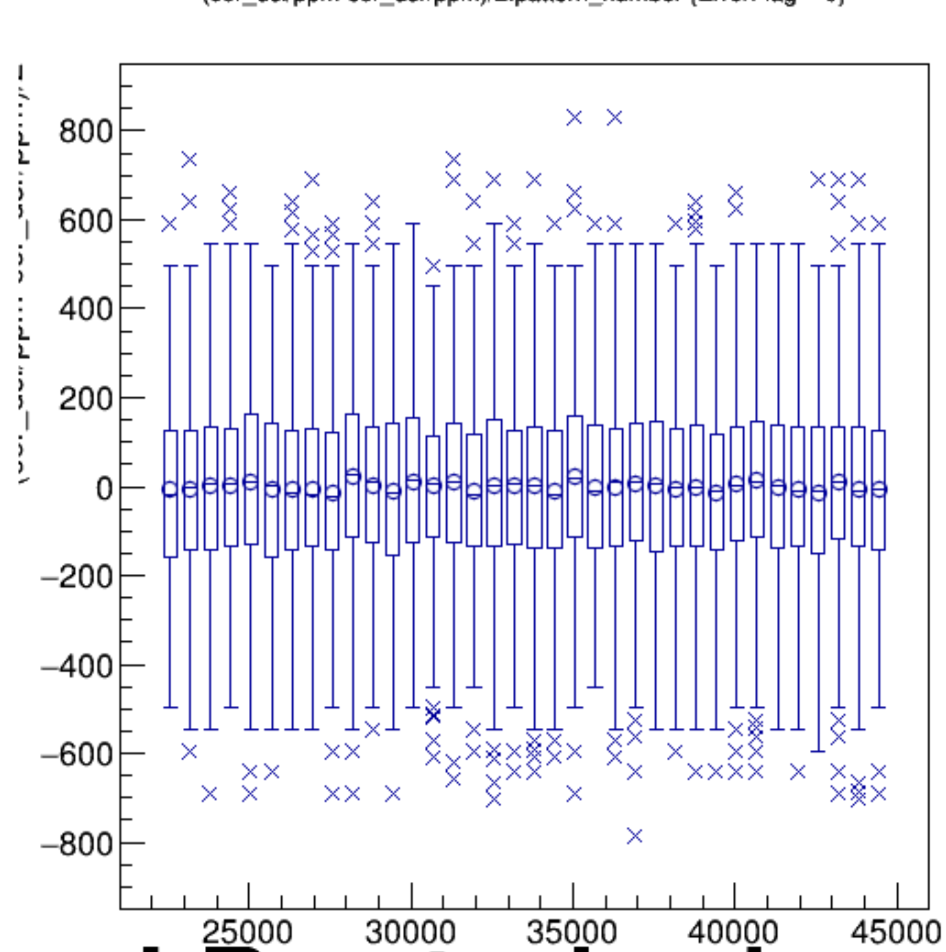
(cor_dsl/ppm-cor_dsr/ppm)/2:pattern_number {ErrorFlag==0}
