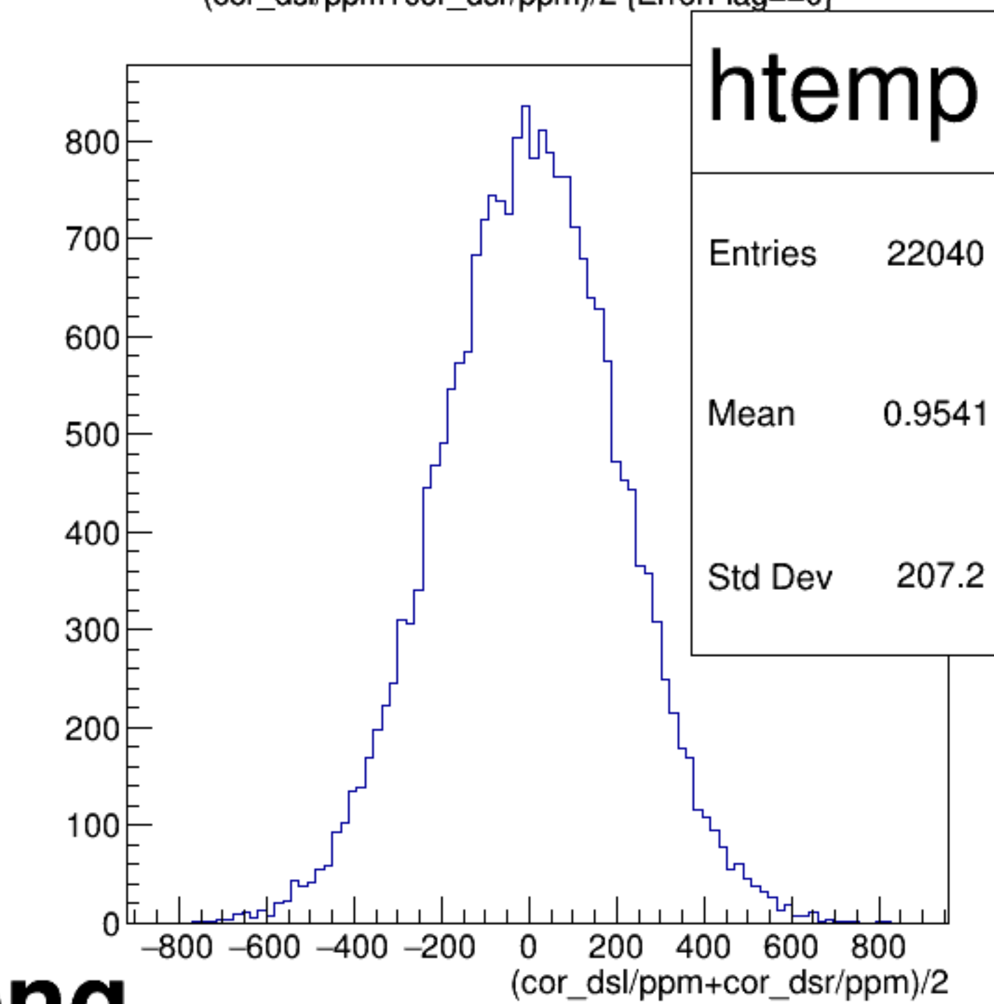
(cor_dsl/ppm+cor_dsr/ppm)/2 {ErrorFlag==0}
