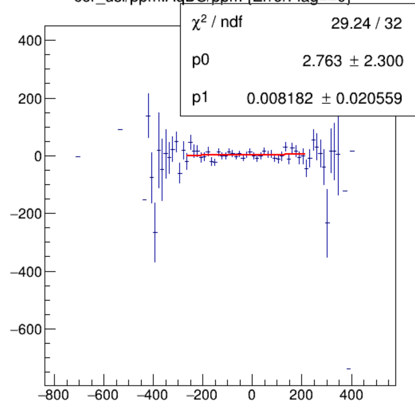
cor_usl/ppm:AqDS/ppm {ErrorFlag==0}
