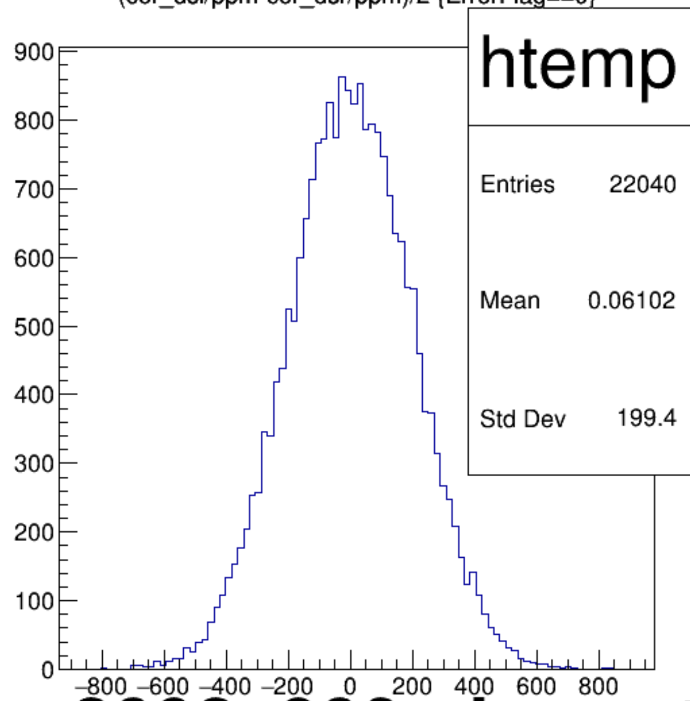
(cor_dsl/ppm-cor_dsr/ppm)/2 {ErrorFlag==0}
