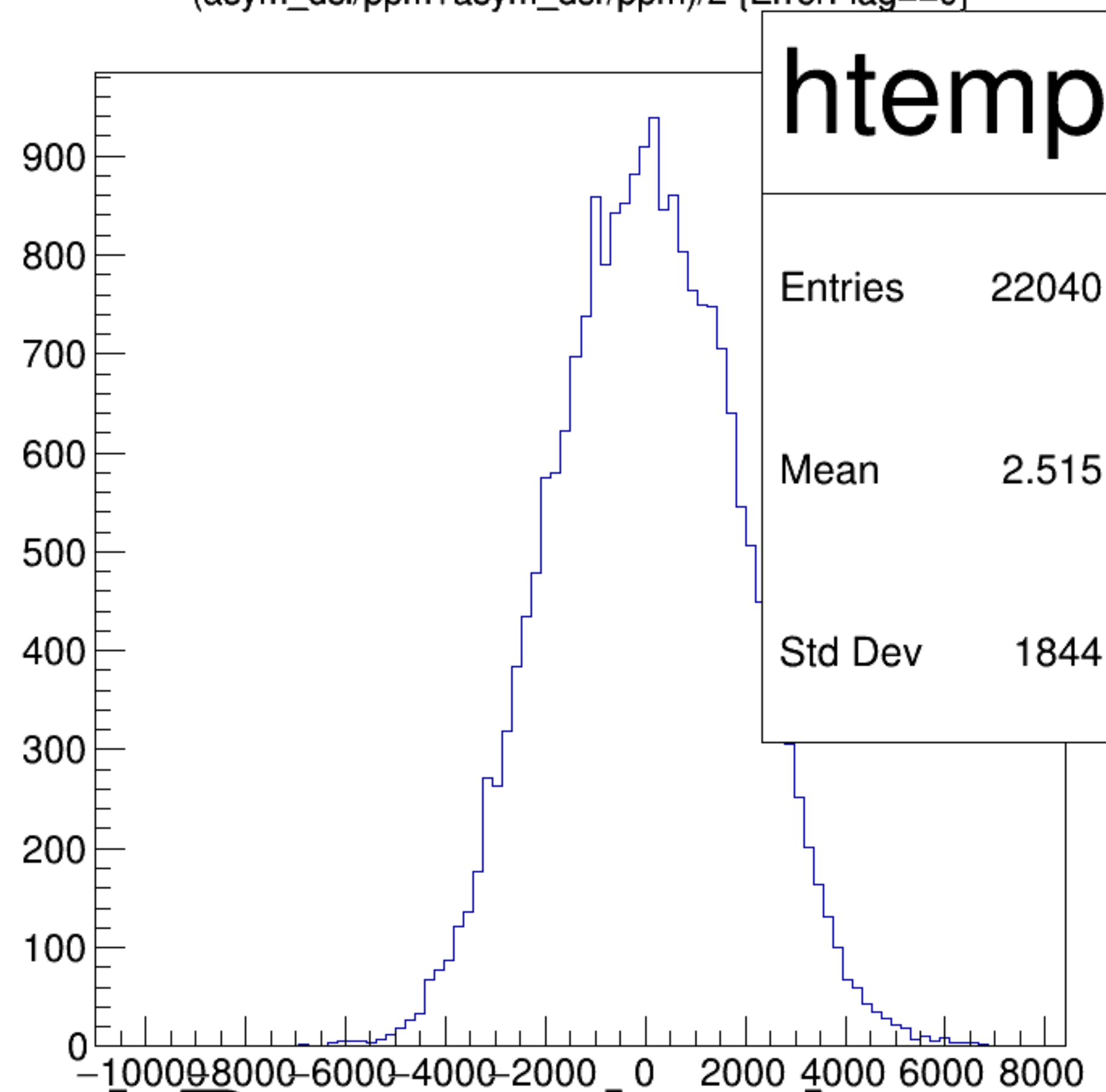
(asym_dsl/ppm+asym_dsr/ppm)/2 {ErrorFlag==0}
