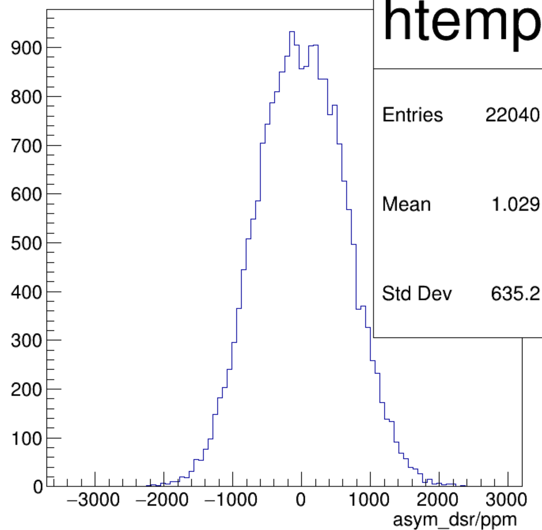
asym_dsr/ppm {ErrorFlag==0}
