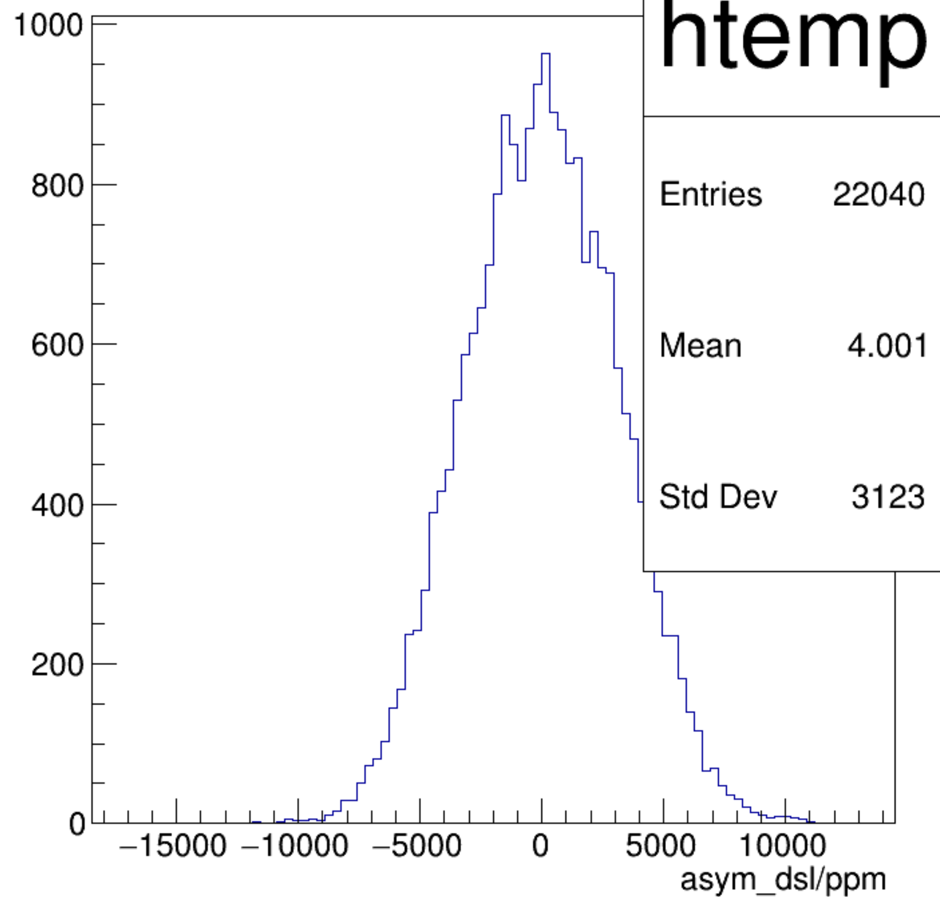
asym_dsl/ppm {ErrorFlag==0}
