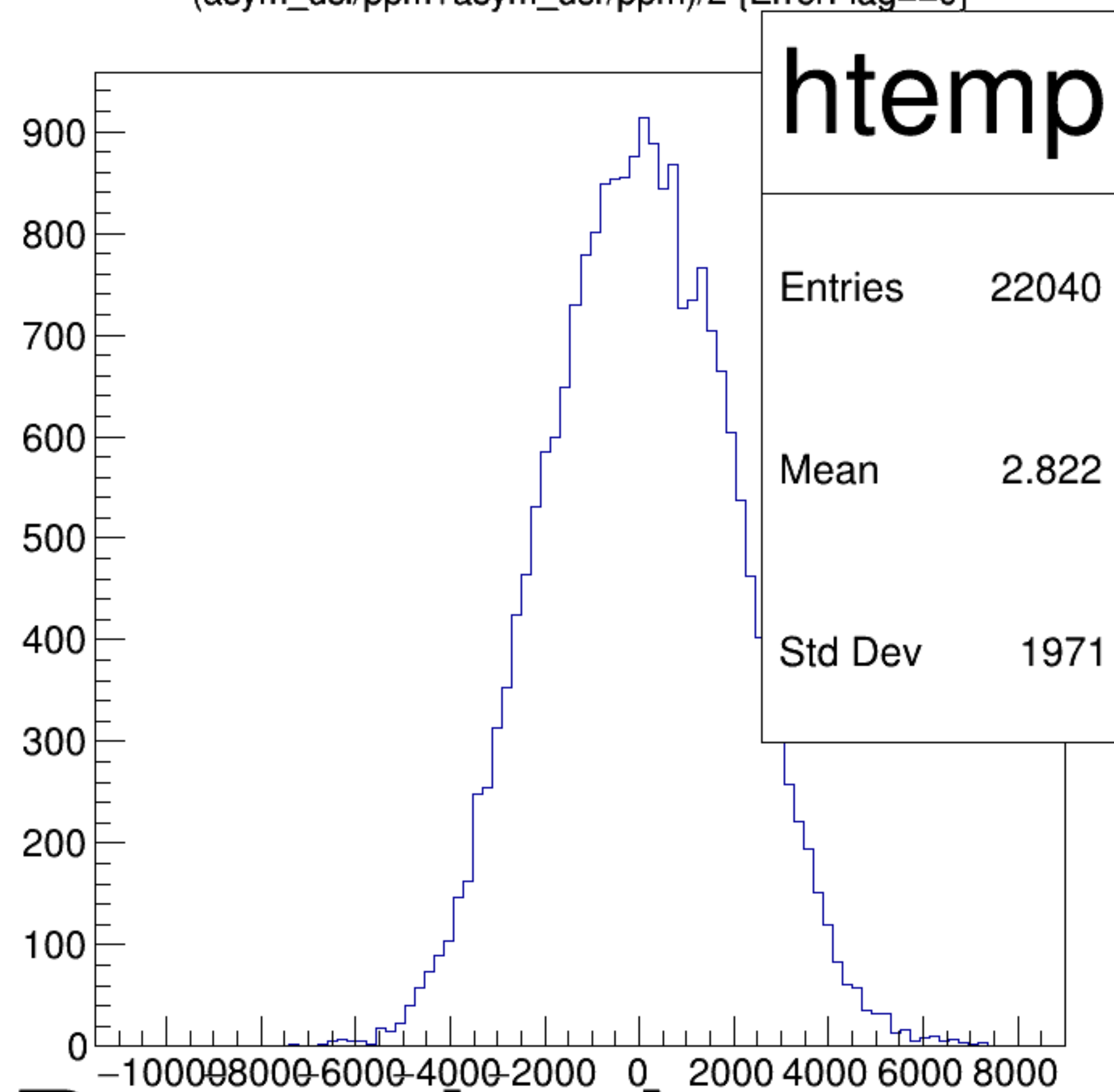
(asym_usl/ppm+asym_usr/ppm)/2 {ErrorFlag==0}
