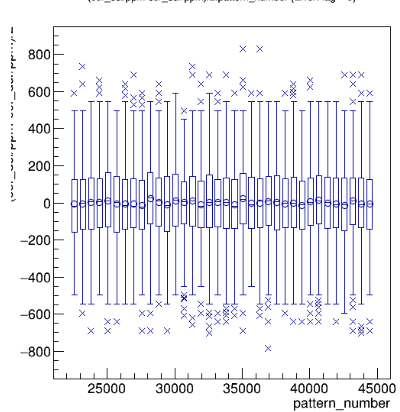
(cor_dsl/ppm+cor_dsr/ppm)/2:pattern_number {ErrorFlag==0}
