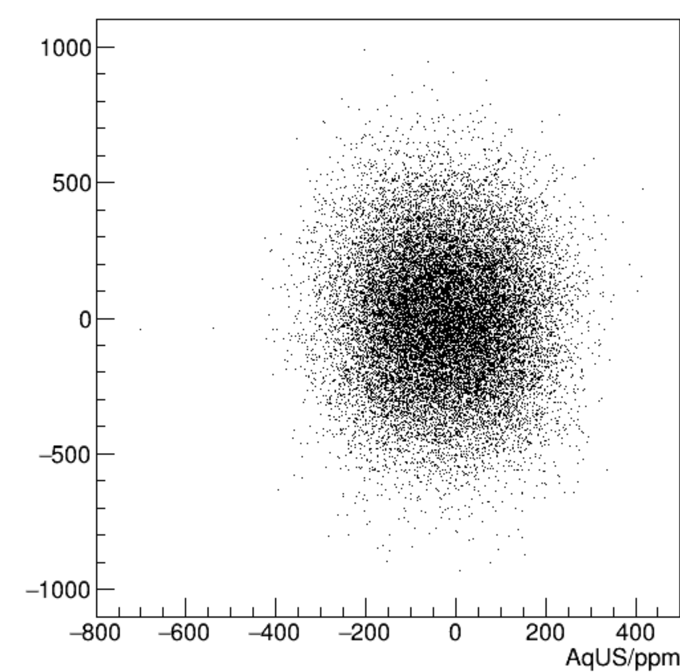
cor_dsr/ppm:AqUS/ppm {ErrorFlag==0}
