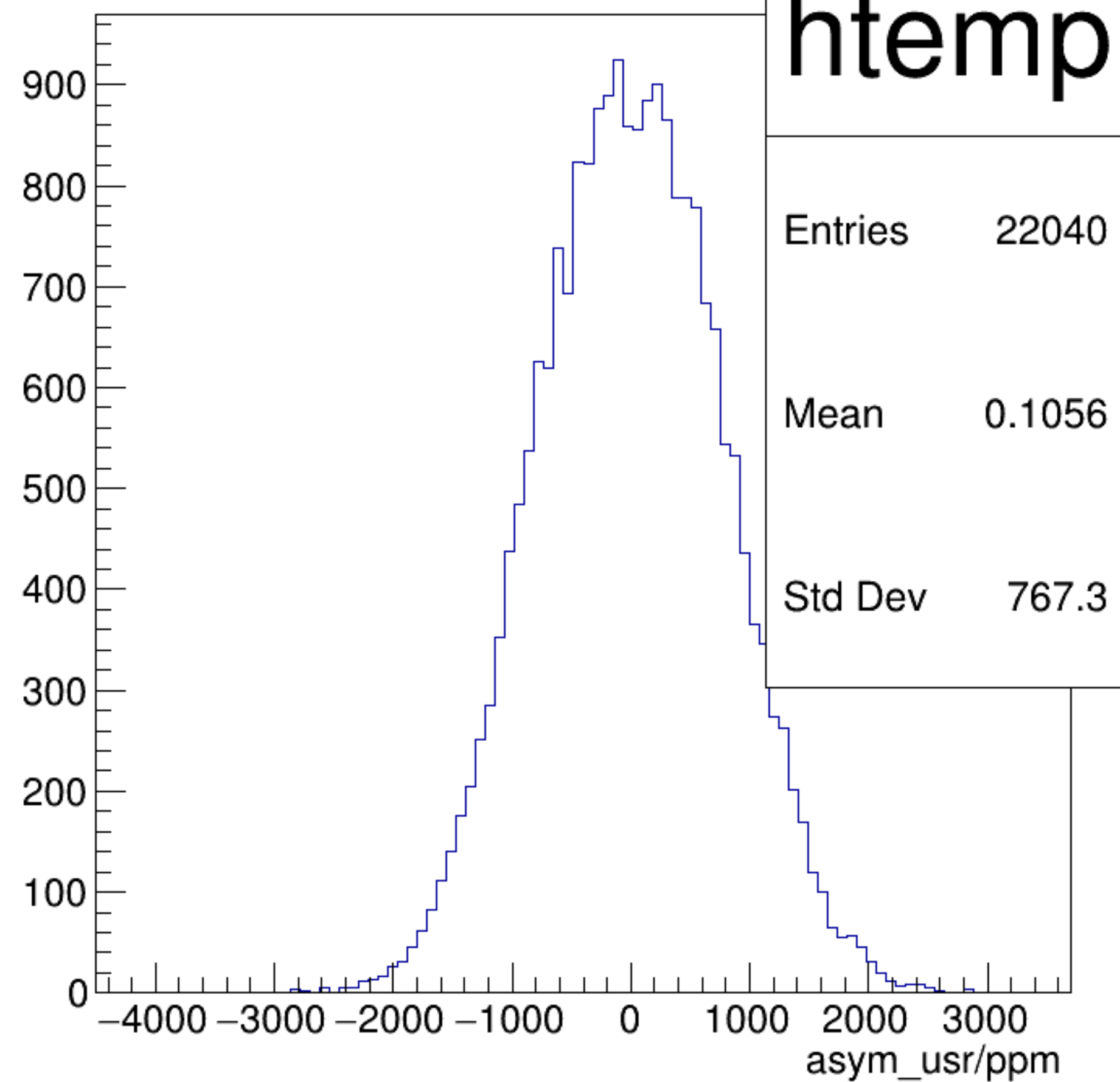
asym_usr/ppm {ErrorFlag==0}
