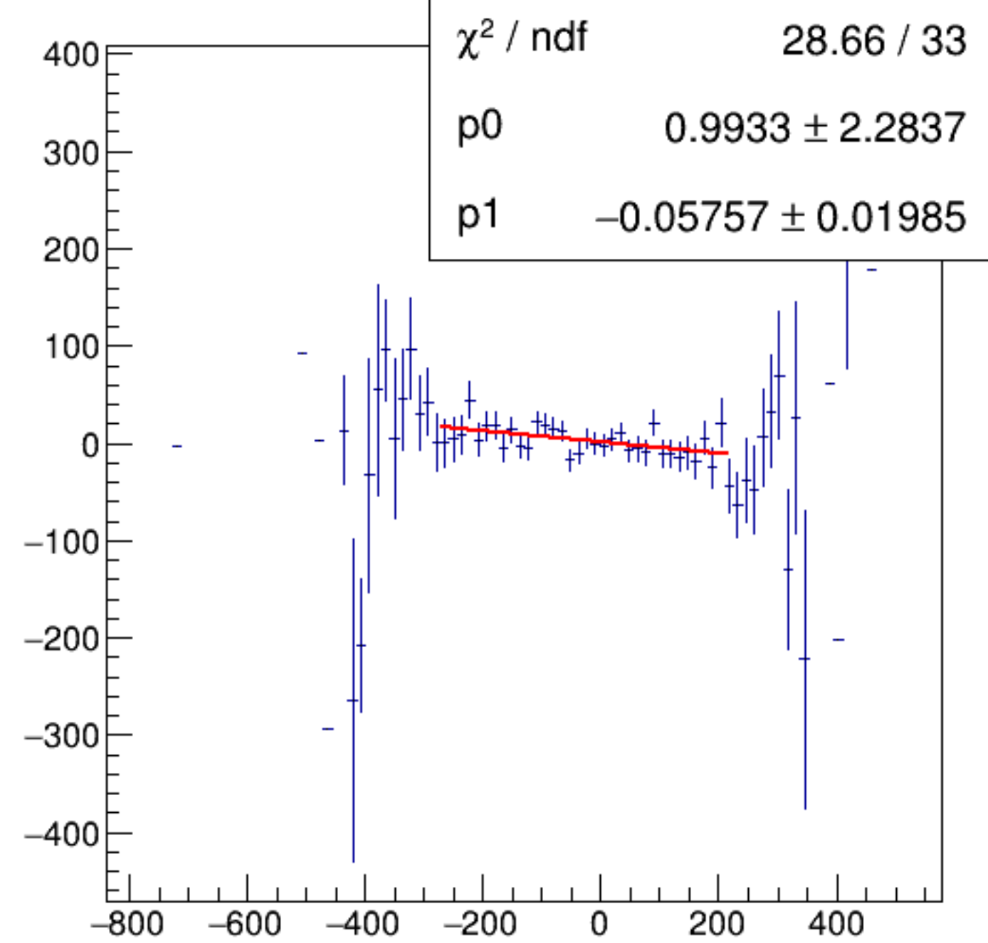
cor_usl/ppm:AqDS/ppm {ErrorFlag==0}
