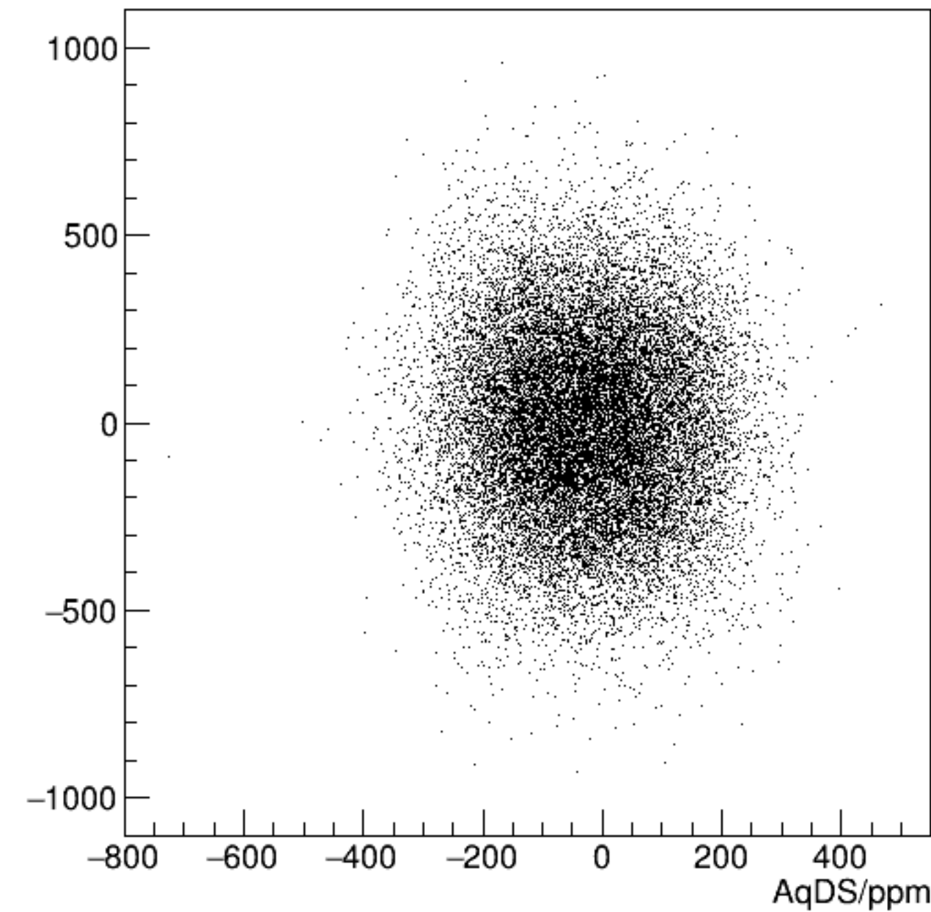
cor_usr/ppm:AqDS/ppm {ErrorFlag==0}
