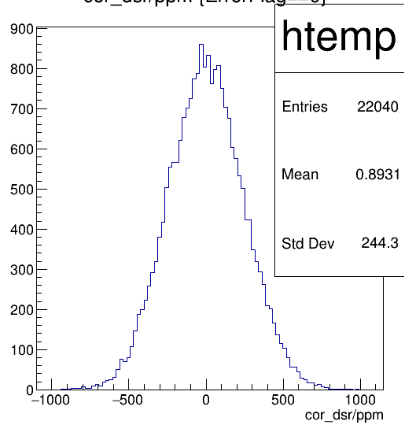
cor_dsr/ppm {ErrorFlag==0}
