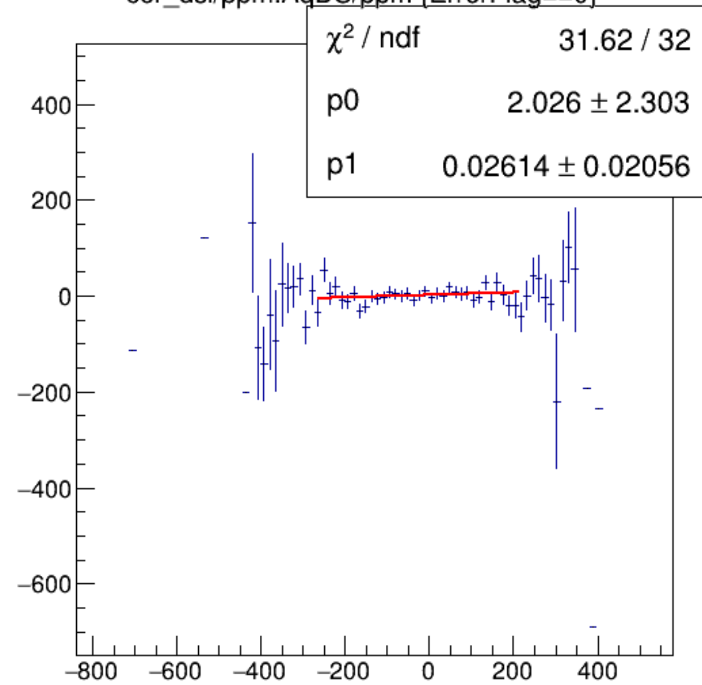
cor_dsl/ppm:AqDS/ppm {ErrorFlag==0}
