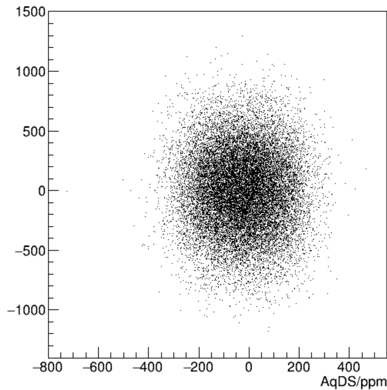
cor_usl/ppm:AqDS/ppm {ErrorFlag==0}
