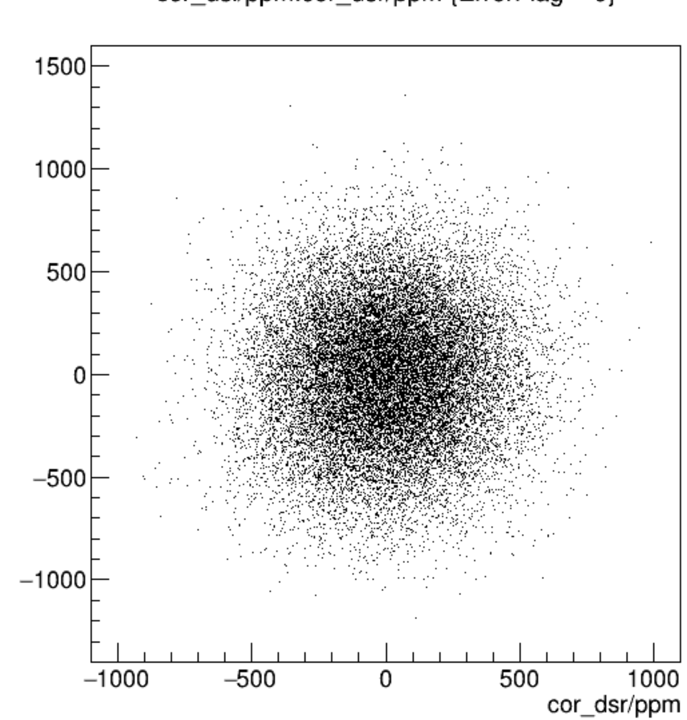
cor_dsl/ppm:cor_dsr/ppm {ErrorFlag==0}
