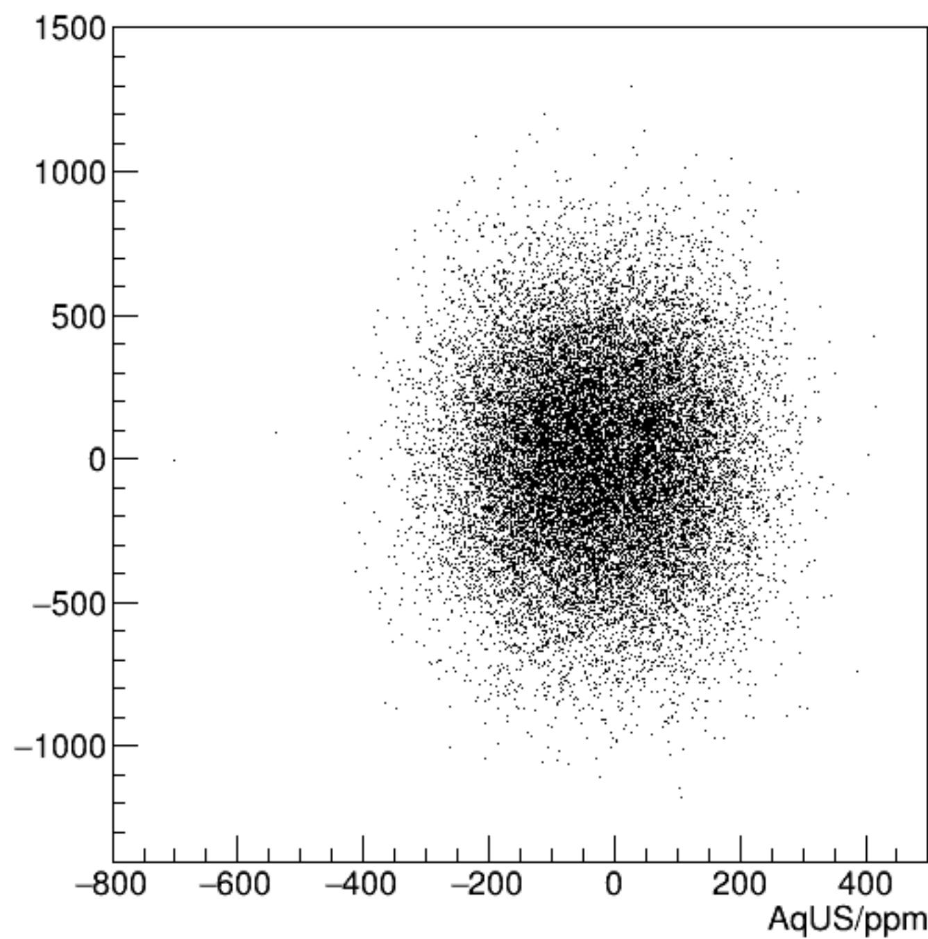
cor_usl/ppm:AqUS/ppm {ErrorFlag==0}
