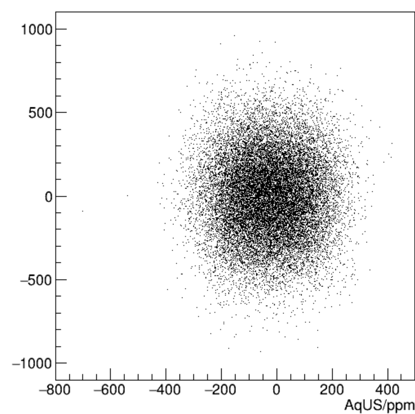
cor_usr/ppm:AqUS/ppm {ErrorFlag==0}
