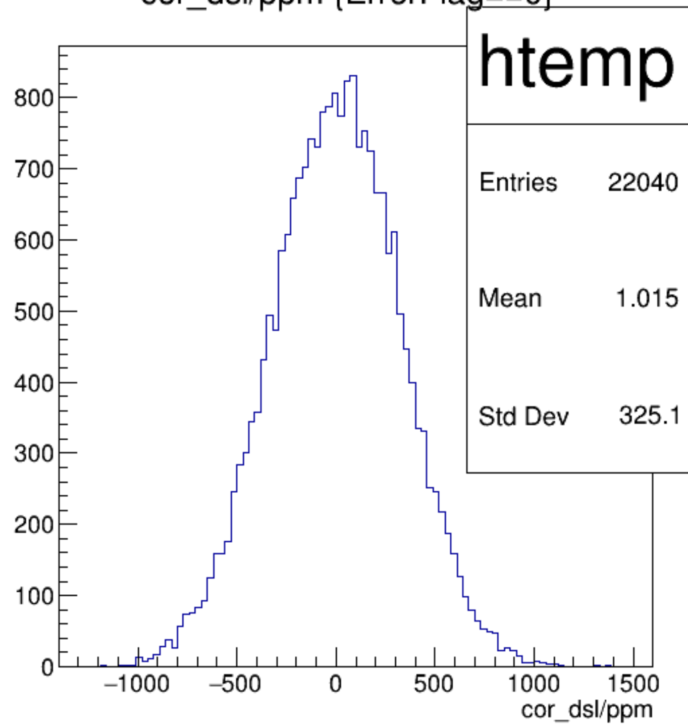
cor_dsl/ppm {ErrorFlag==0}
