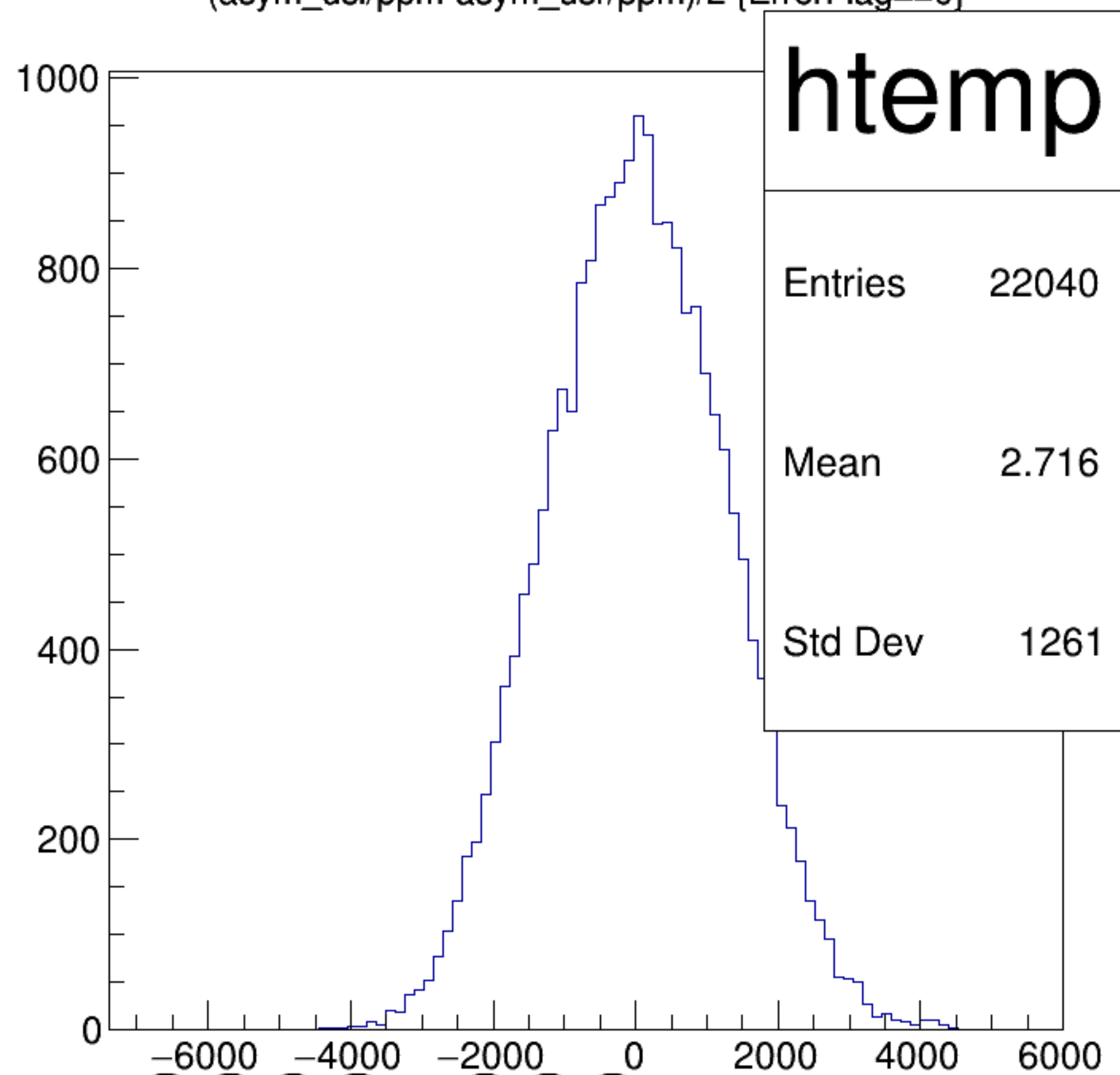
(asym_usl/ppm-asym_usr/ppm)/2 {ErrorFlag==0}
