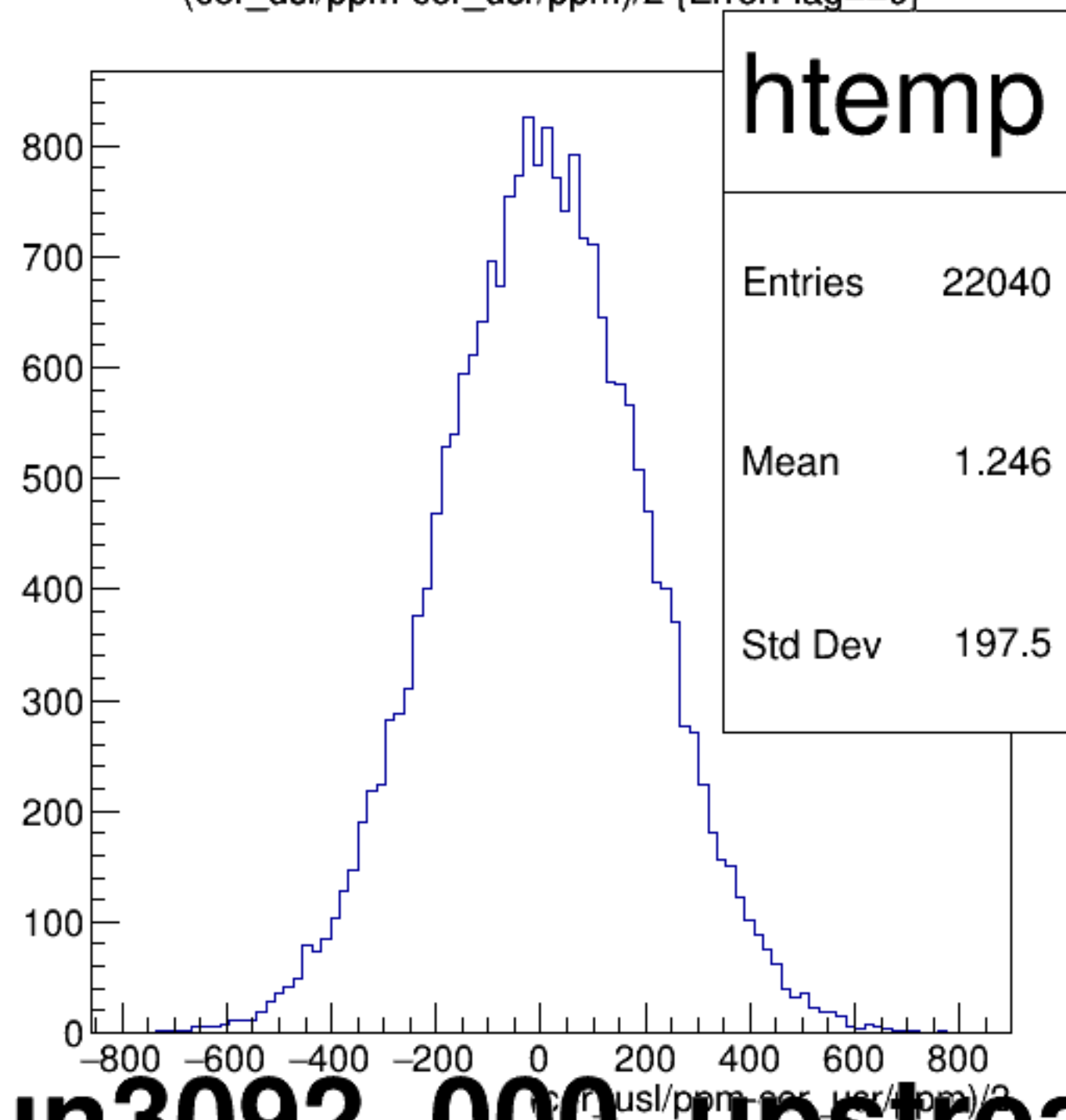
(cor_usl/ppm-cor_usr/ppm)/2 {ErrorFlag==0}
