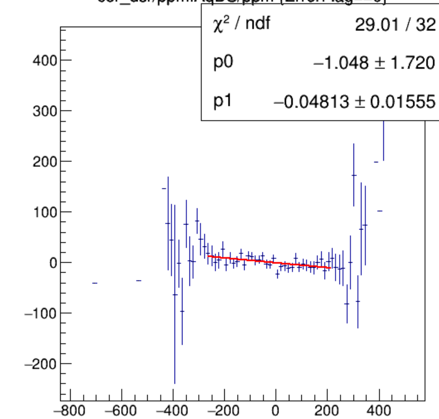
cor_dsr/ppm:AqDS/ppm {ErrorFlag==0}
