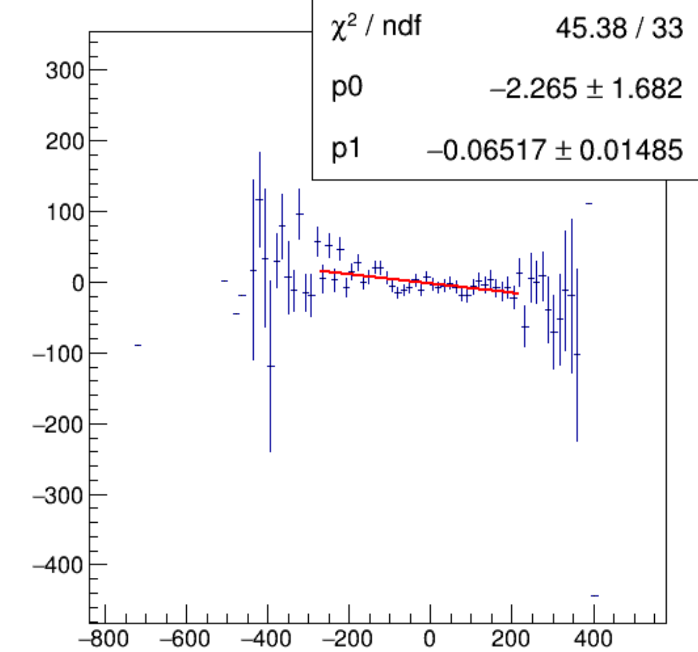
cor_usr/ppm:AqDS/ppm {ErrorFlag==0}
