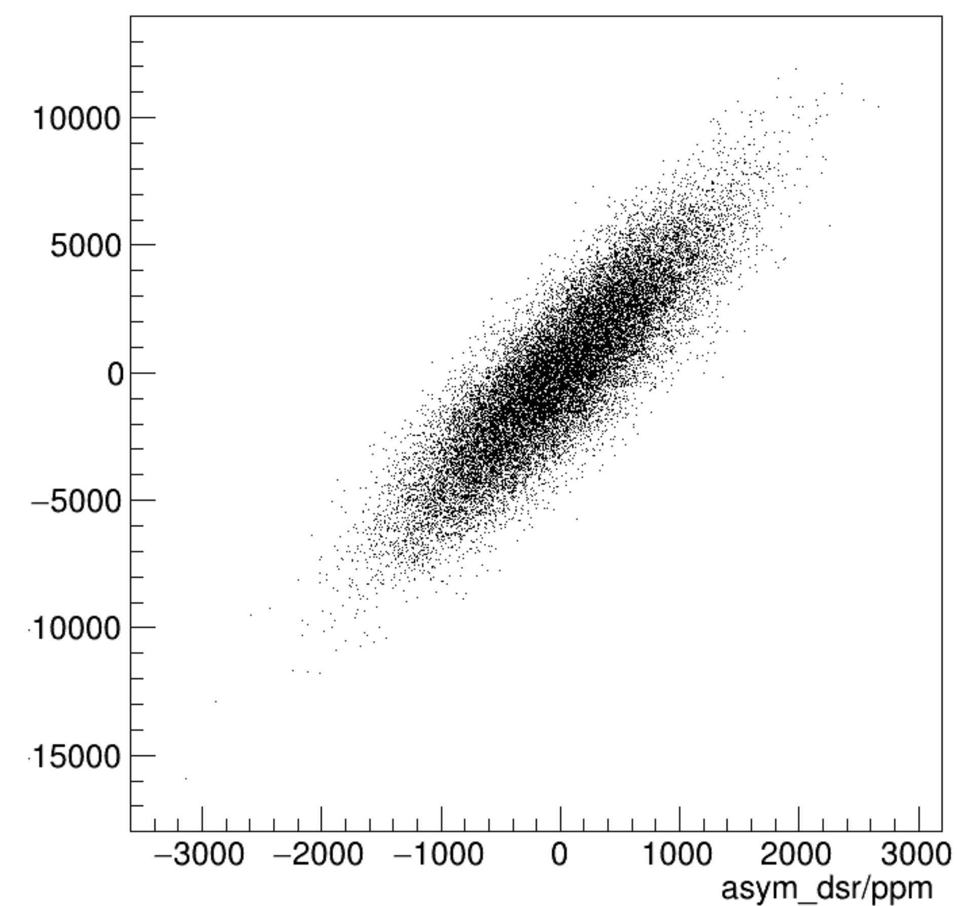
asym_dsl/ppm:asym_dsr/ppm {ErrorFlag==0}
