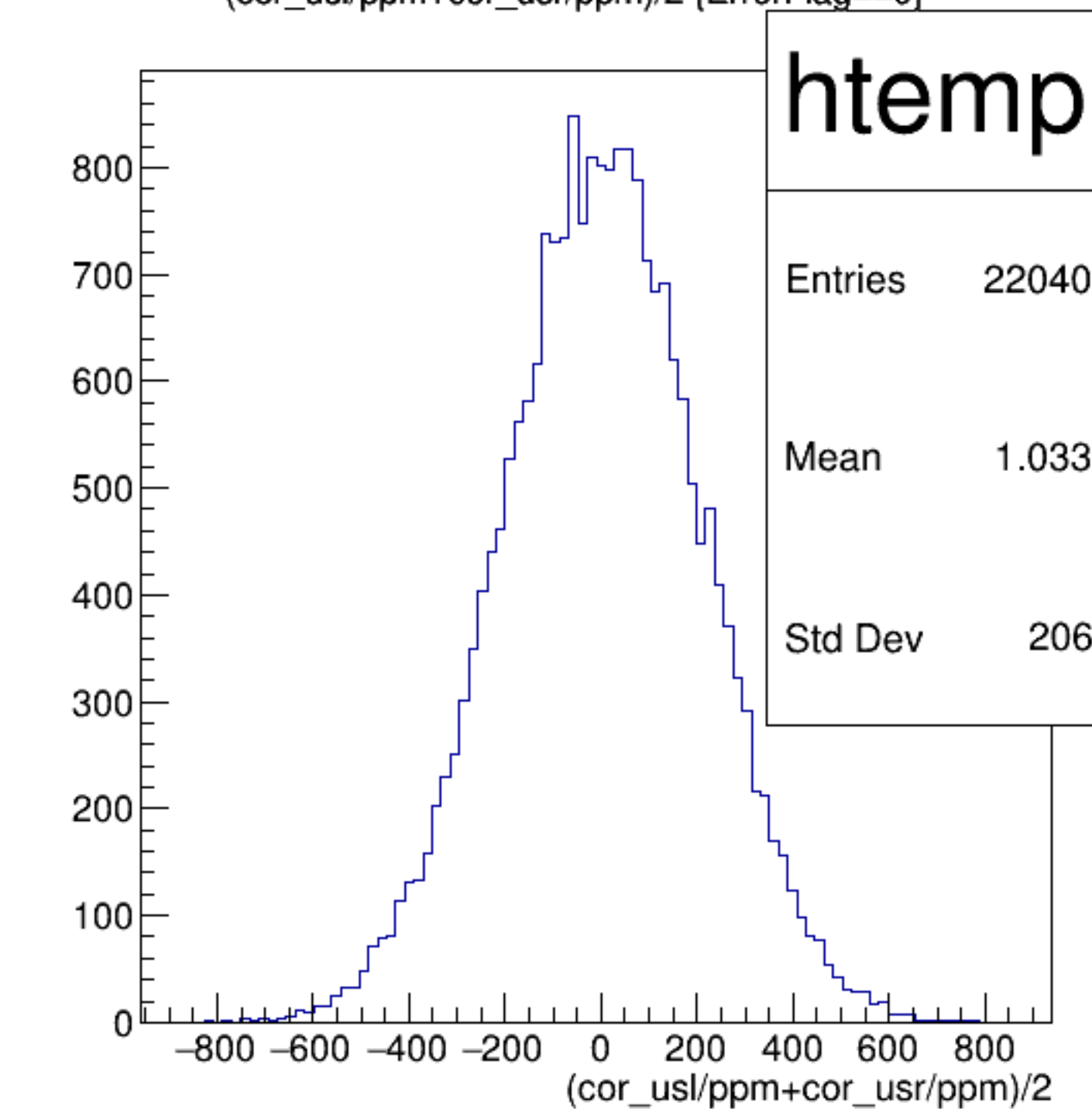
(cor_usl/ppm+cor_usr/ppm)/2 {ErrorFlag==0}
