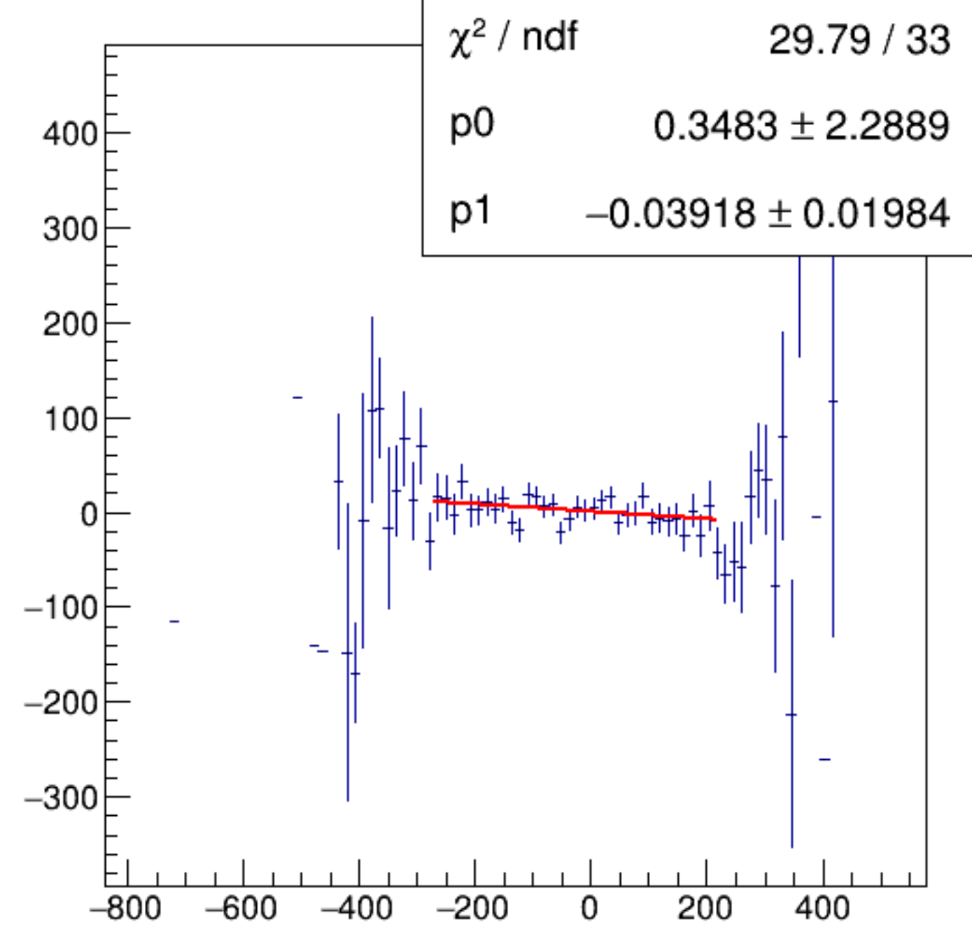
cor_dsl/ppm:AqDS/ppm {ErrorFlag==0}
