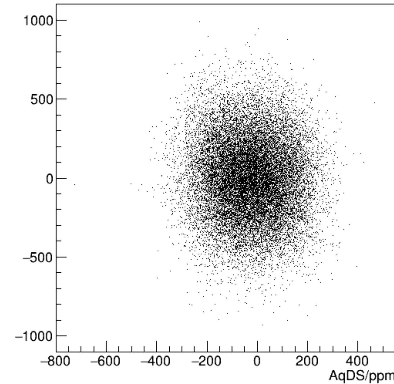
cor_dsr/ppm:AqDS/ppm {ErrorFlag==0}
