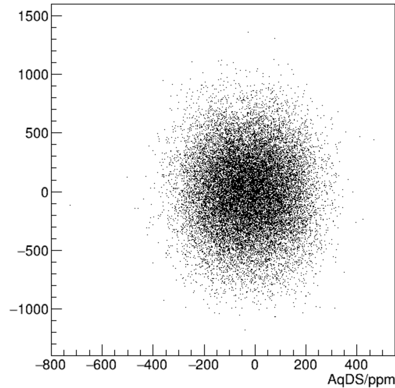
cor_dsl/ppm:AqDS/ppm {ErrorFlag==0}
