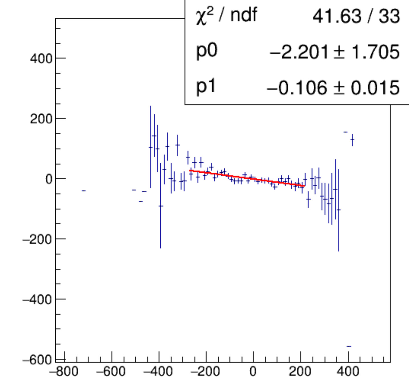
cor_dsr/ppm:AqDS/ppm {ErrorFlag==0}
