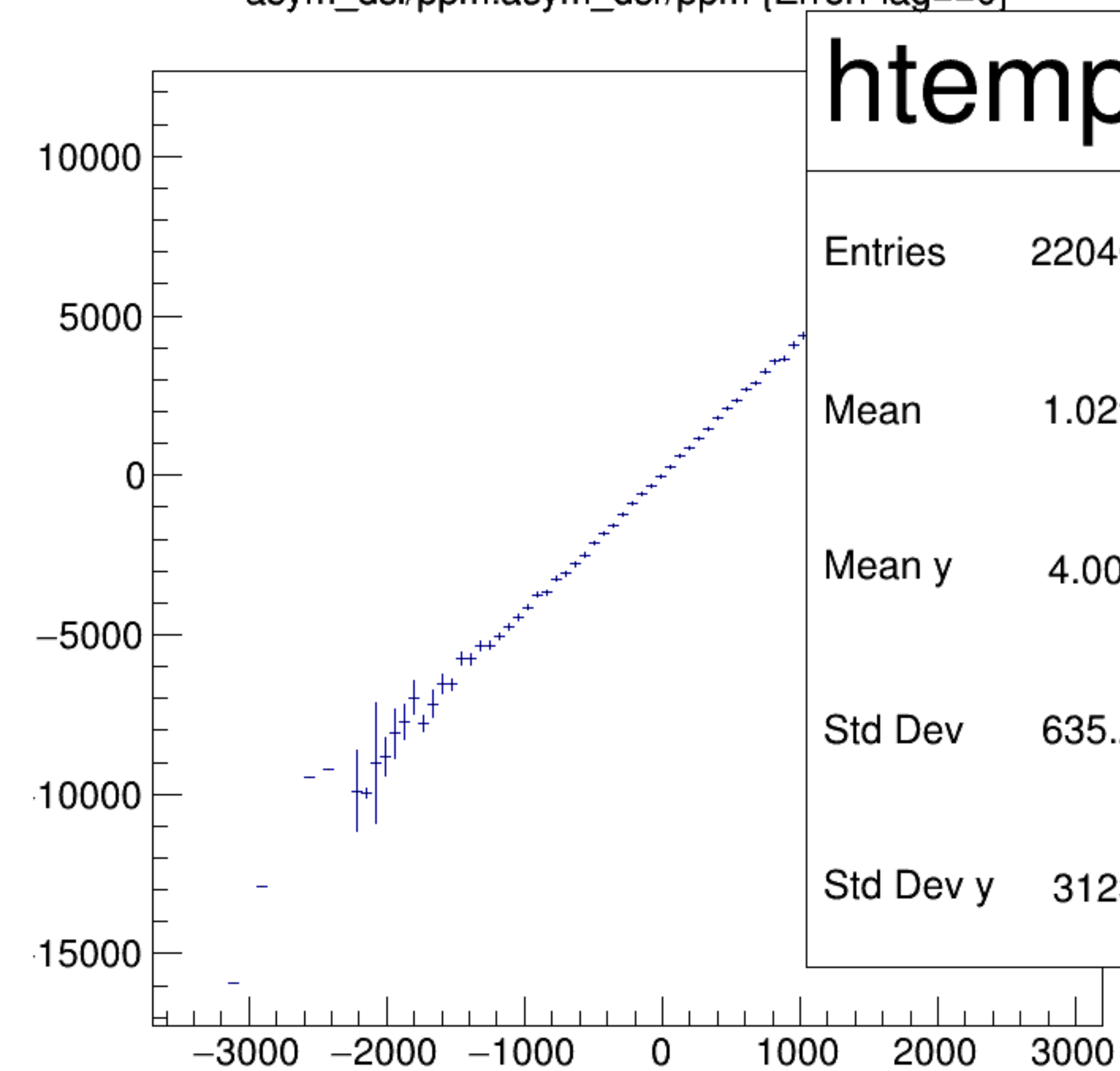
asym_dsl/ppm:asym_dsr/ppm {ErrorFlag==0}
