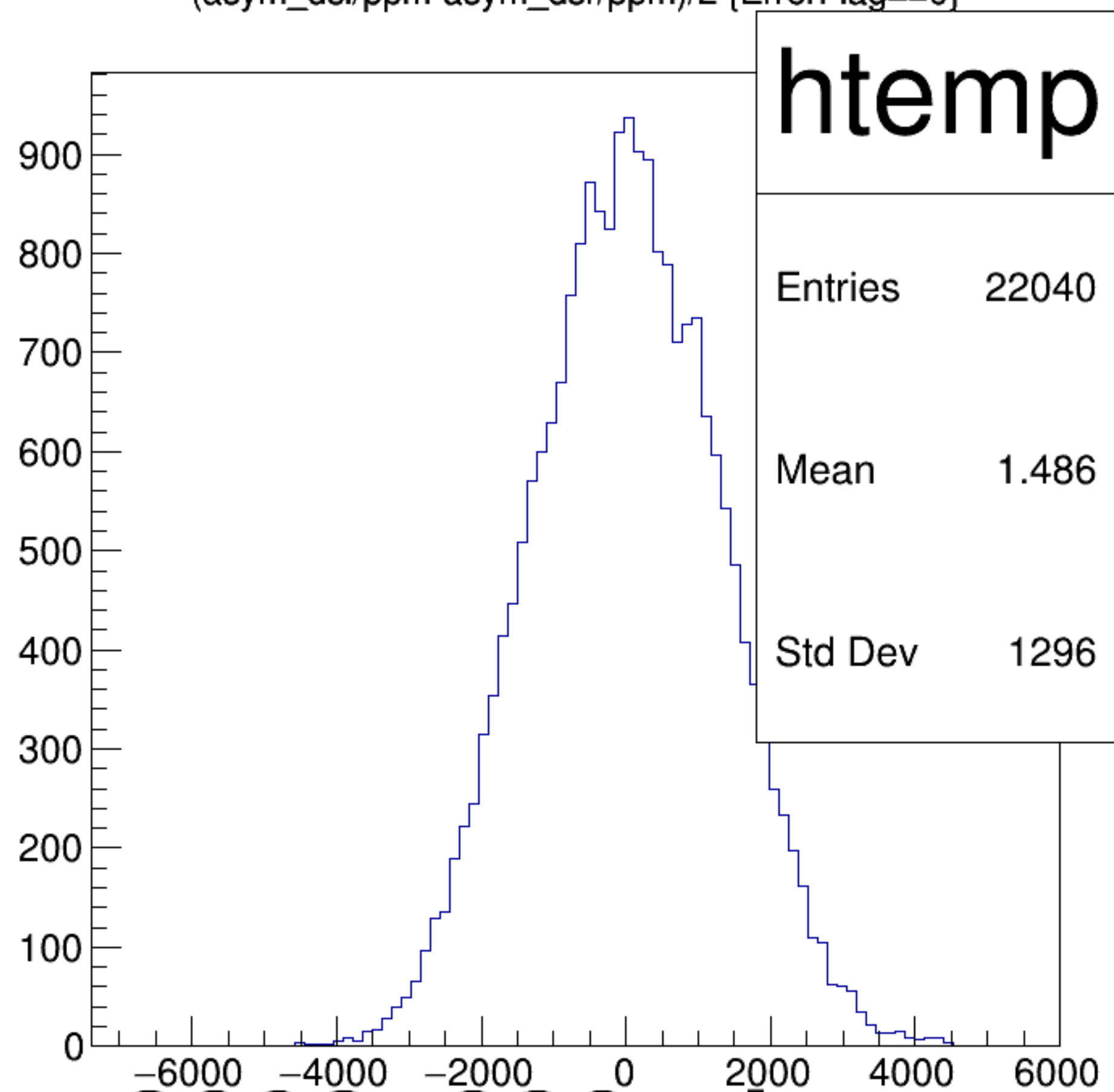
(asym_dsl/ppm-asym_dsr/ppm)/2 {ErrorFlag==0}
