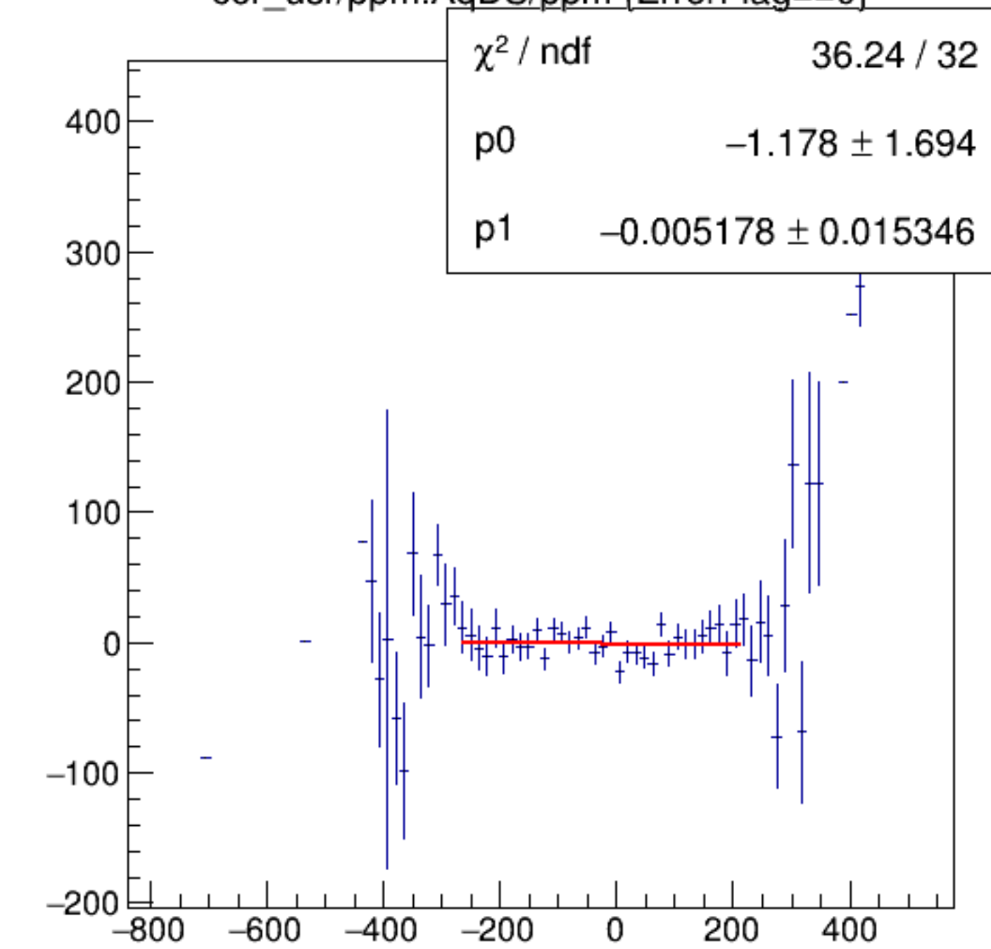
cor_usr/ppm:AqDS/ppm {ErrorFlag==0}
