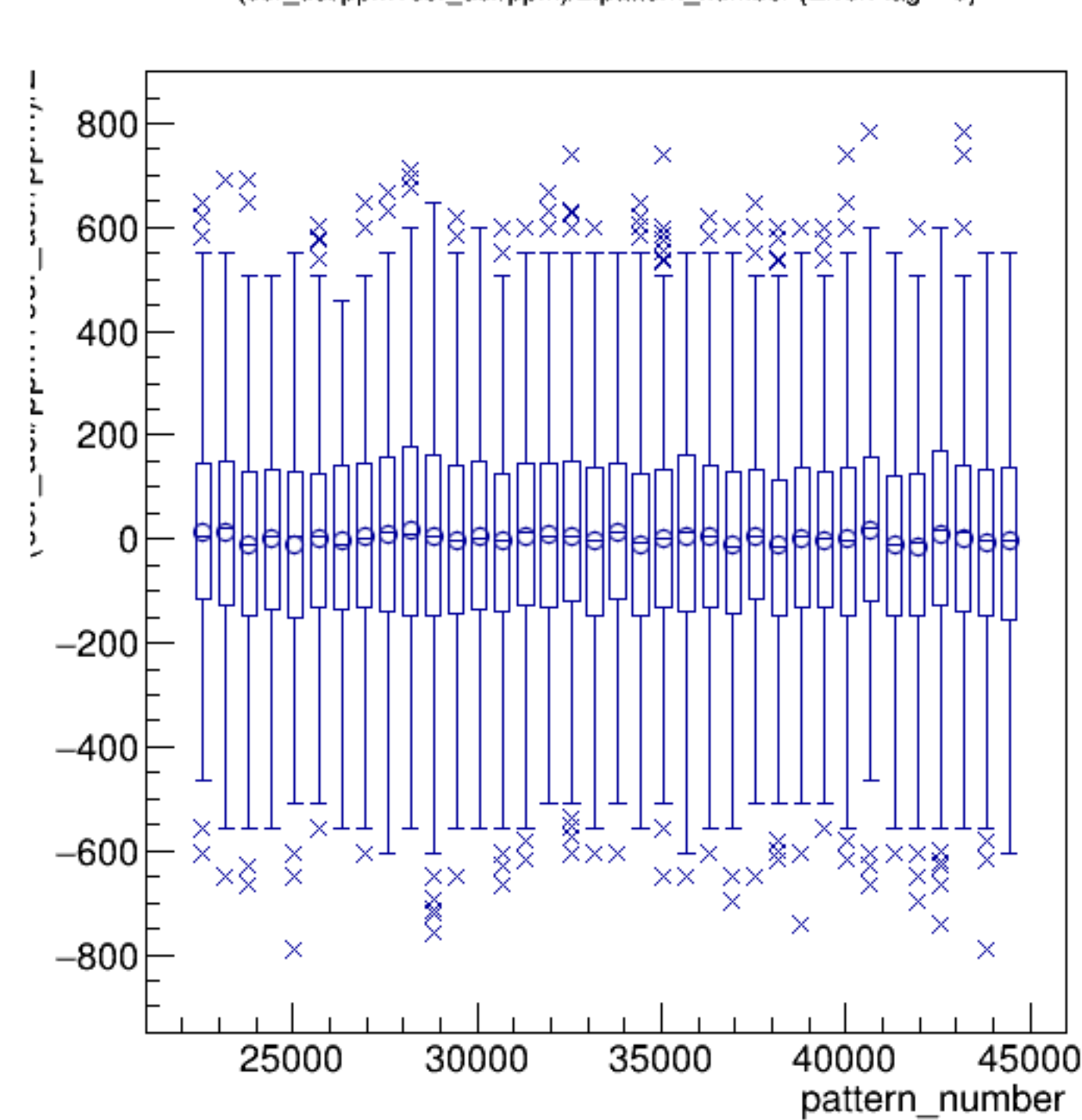
(cor_usl/ppm+cor_usr/ppm)/2:pattern_number {ErrorFlag==0}
