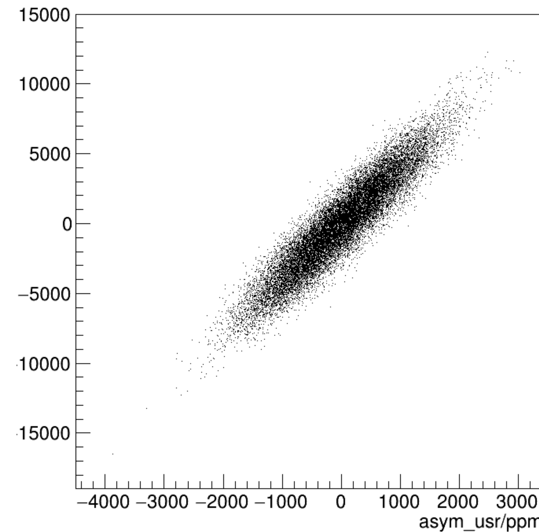
asym_usl/ppm:asym_usr/ppm {ErrorFlag==0}
