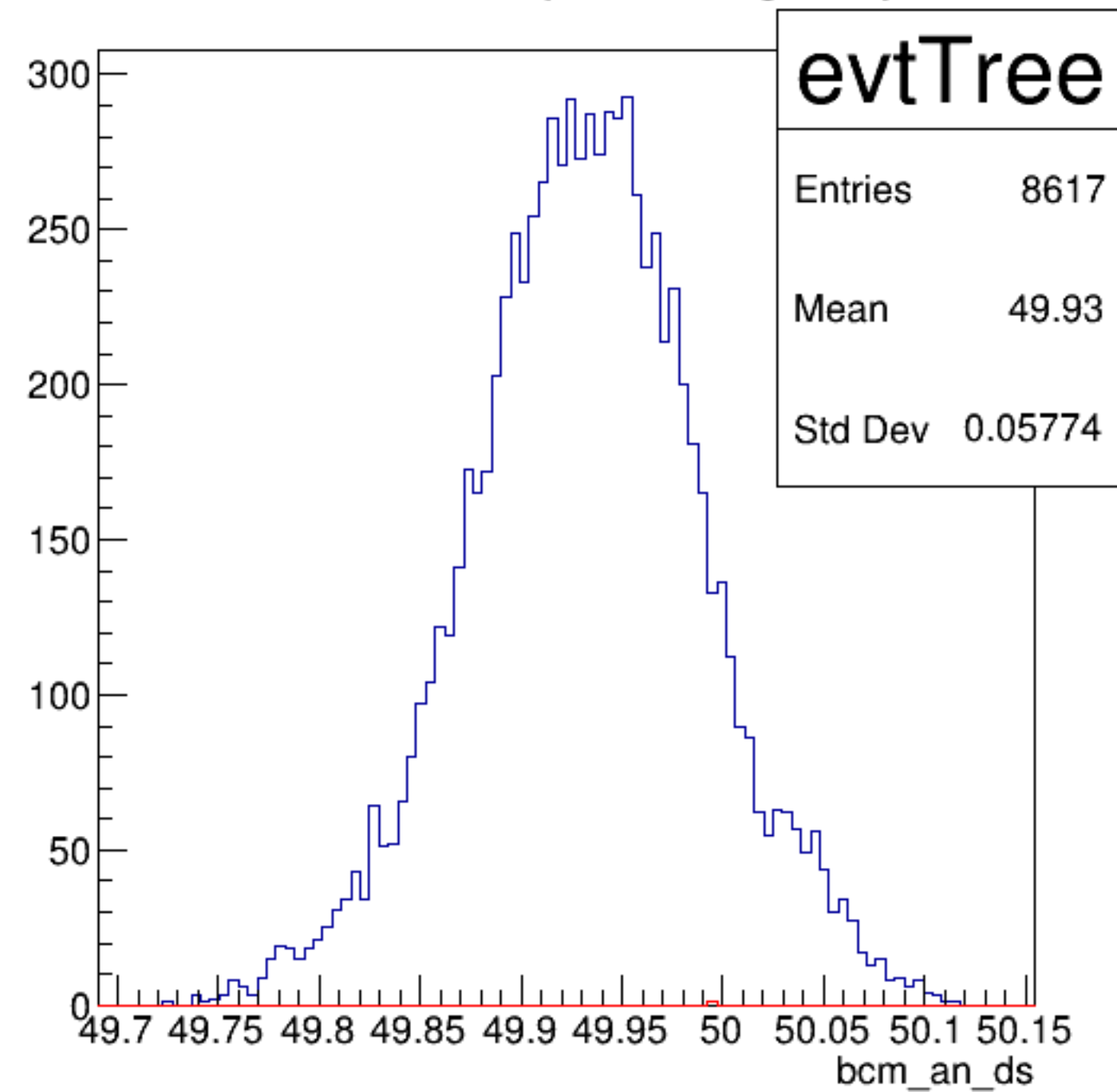
bcm_an_ds {ErrorFlag==0}
