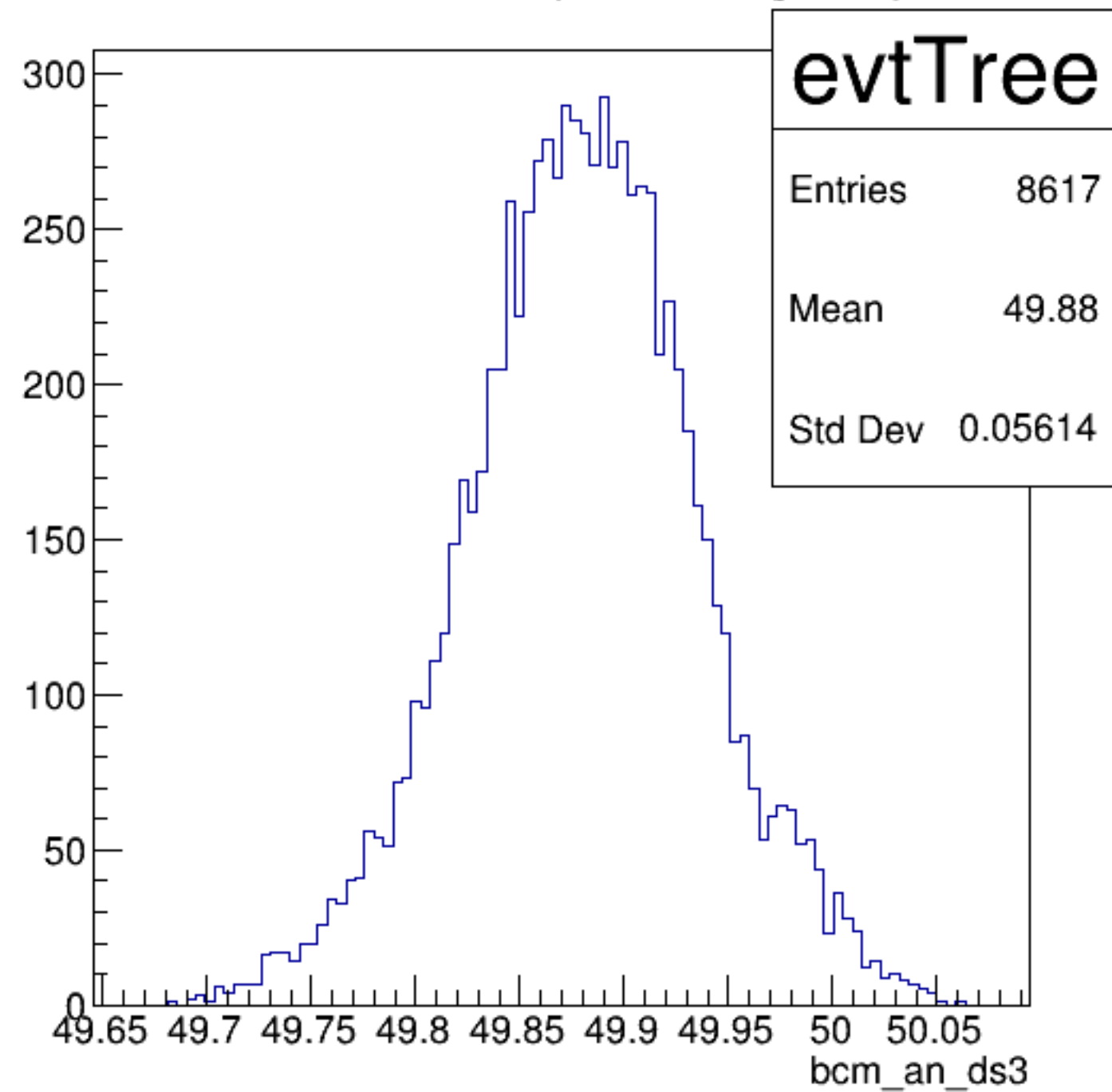
bcm_an_ds3 {ErrorFlag==0}
