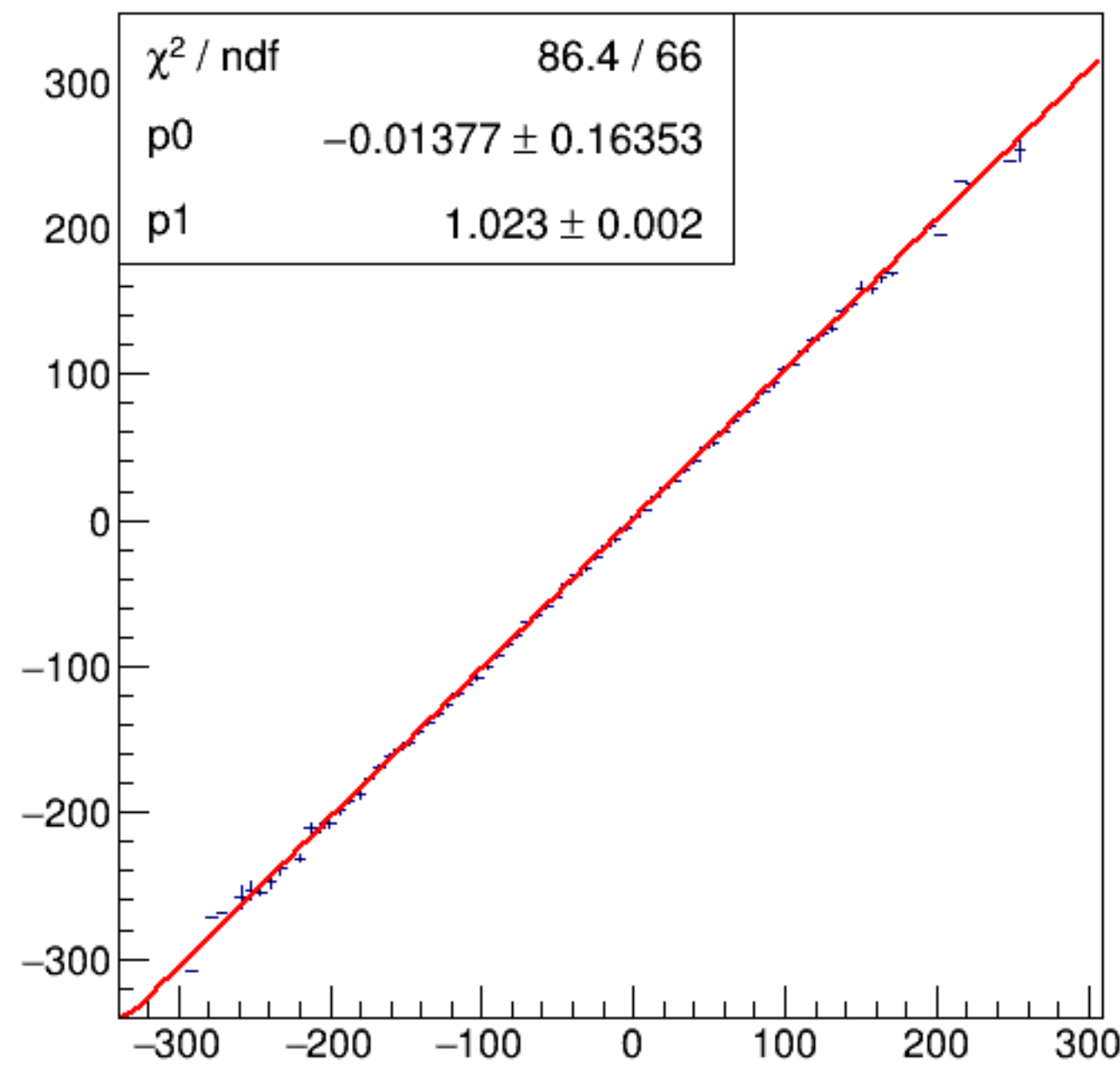
run3115_000_asym_bcm_an_ds_vs_asym_bcm_an_ds3.png
