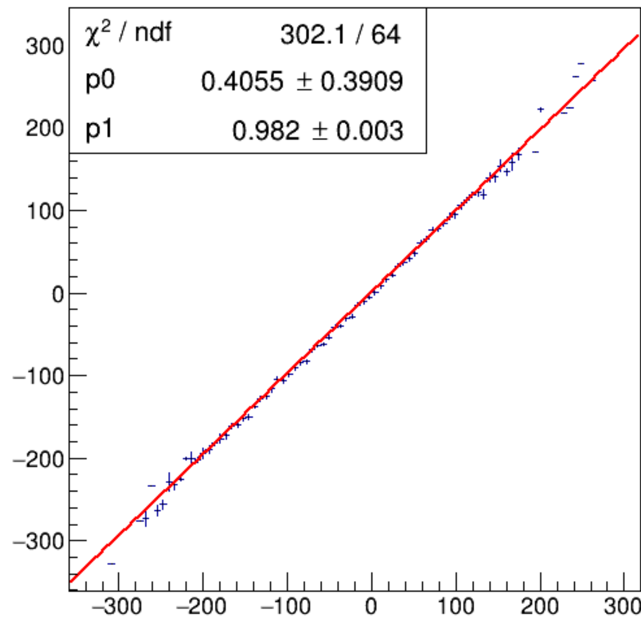
run3115_000_asym_bcm_an_us_vs_asym_bcm_an_ds.png
