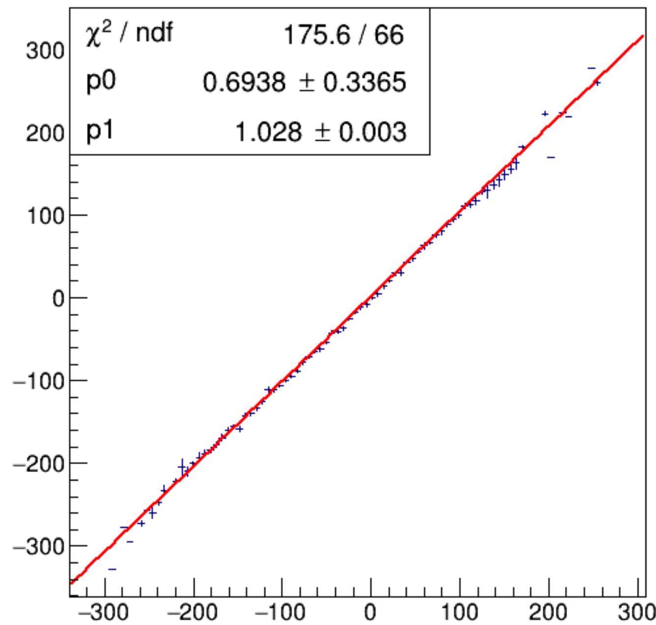
run3115_000_asym_bcm_an_us_vs_asym_bcm_an_ds3.png
