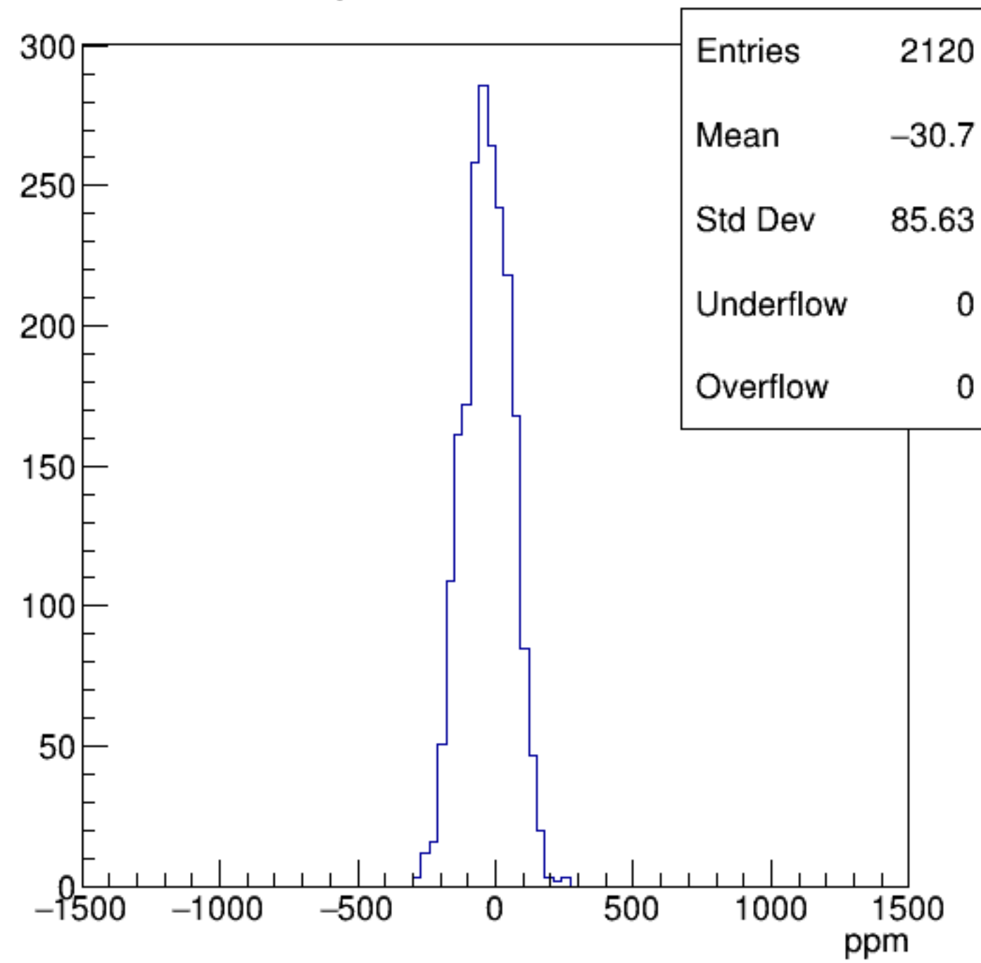
asym_bcm_an_ds3
