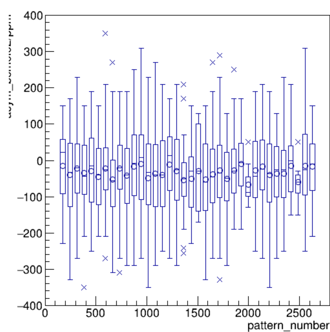
asym_bcm0l02/ppm:pattern_number {ErrorFlag==0}
