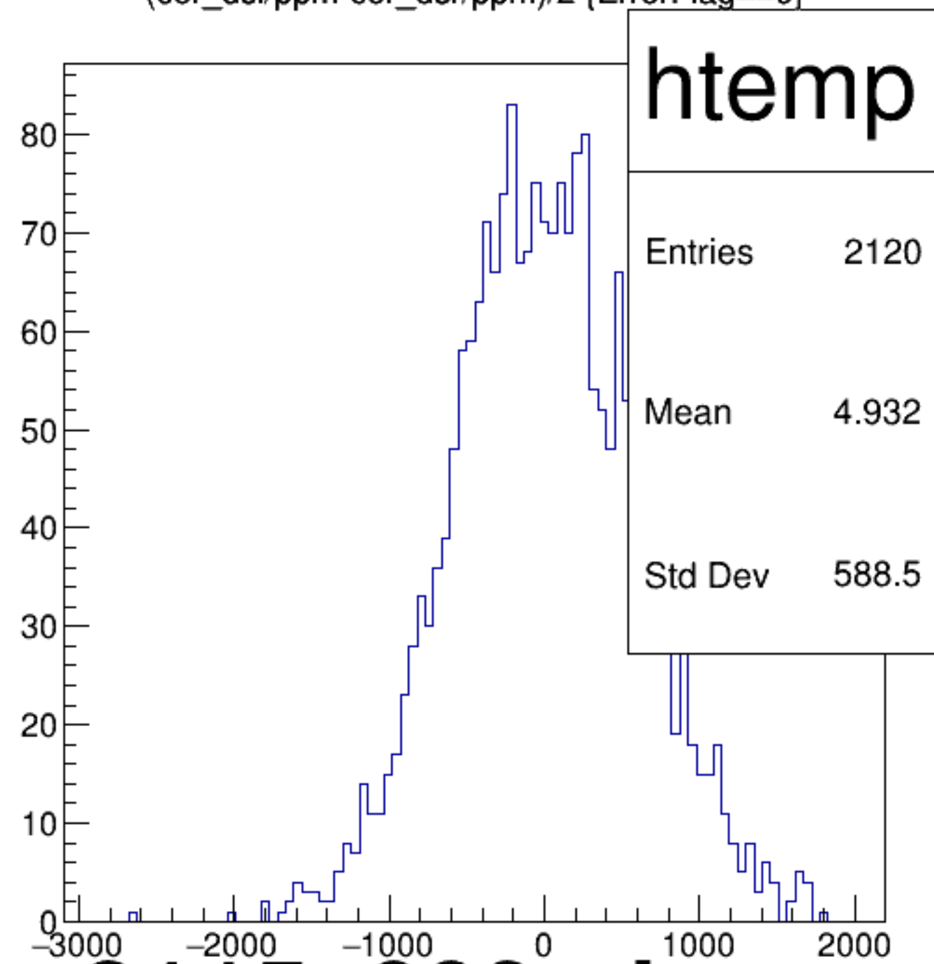
(cor_dsl/ppm-cor_dsr/ppm)/2 {ErrorFlag==0}
