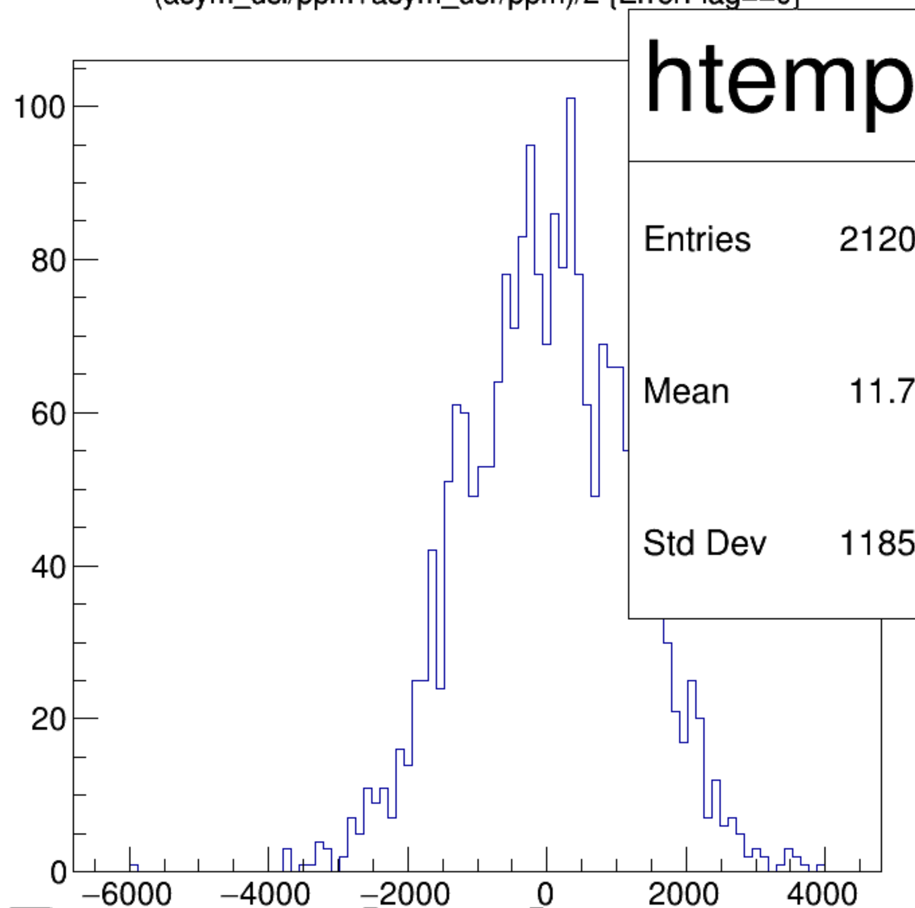
(asym_usl/ppm+asym_usr/ppm)/2 {ErrorFlag==0}
