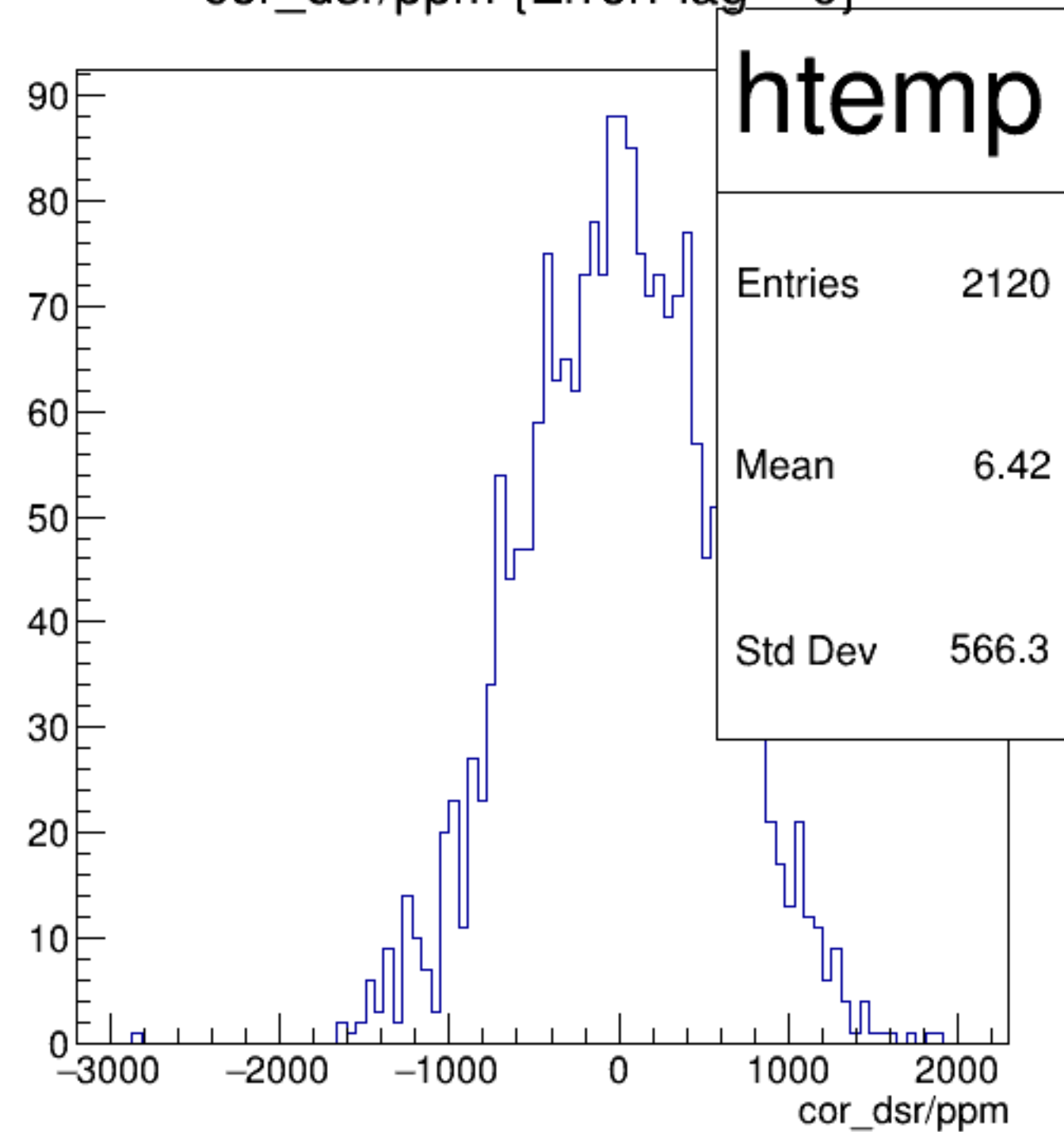
cor_dsr/ppm {ErrorFlag==0}
