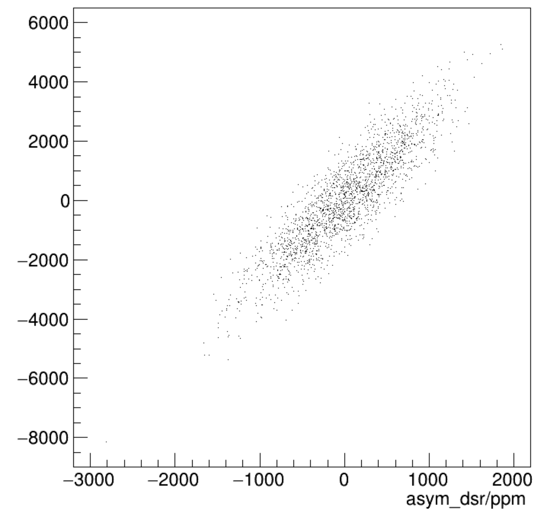
asym_dsl/ppm:asym_dsr/ppm {ErrorFlag==0}
