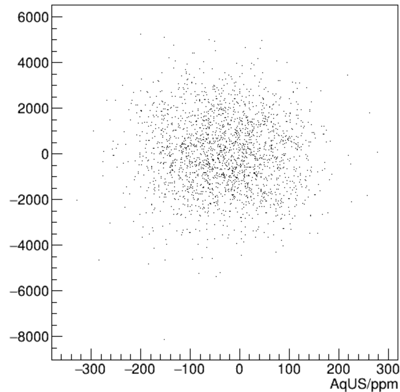
cor_dsl/ppm:AqUS/ppm {ErrorFlag==0}
