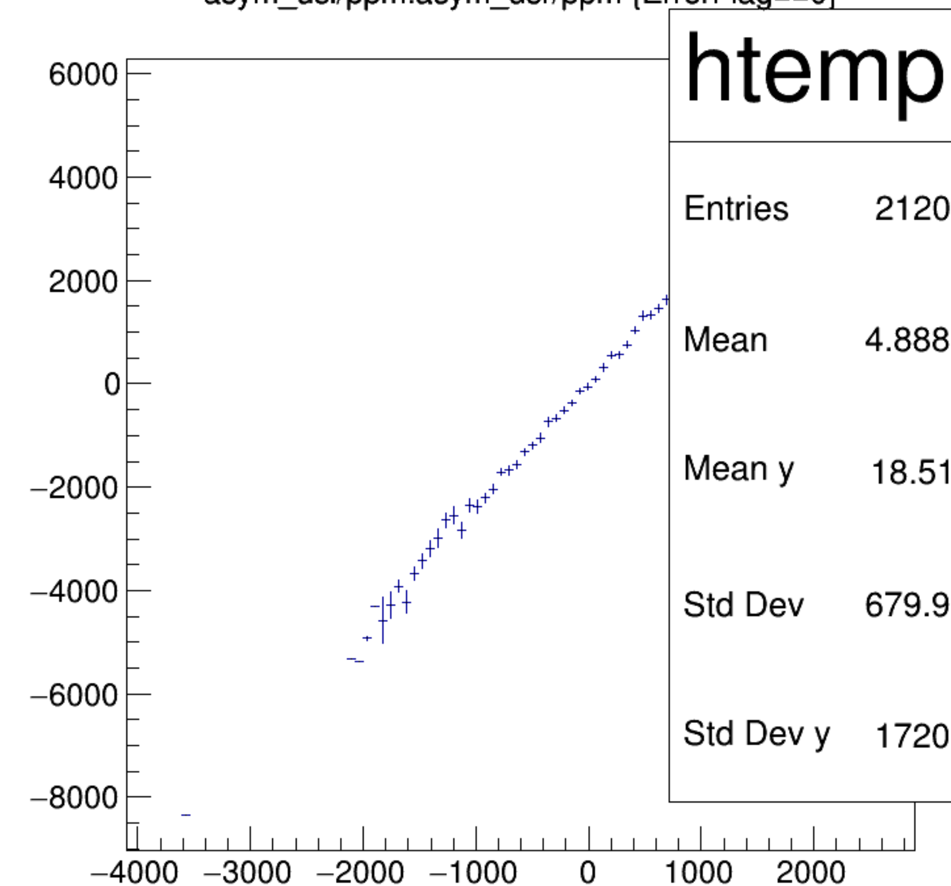
asym_usl/ppm:asym_usr/ppm {ErrorFlag==0}
