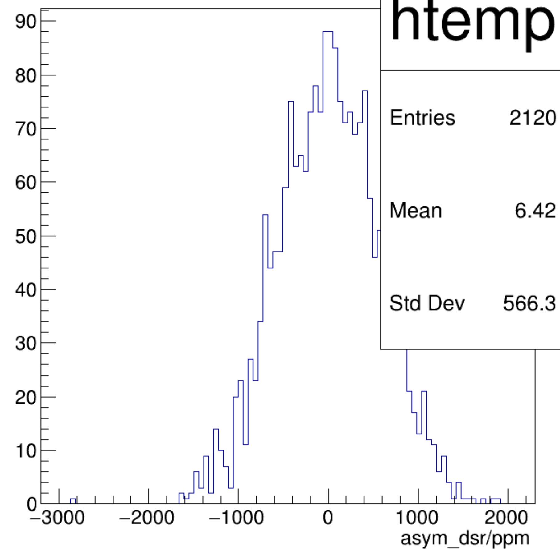
asym_dsr/ppm {ErrorFlag==0}
