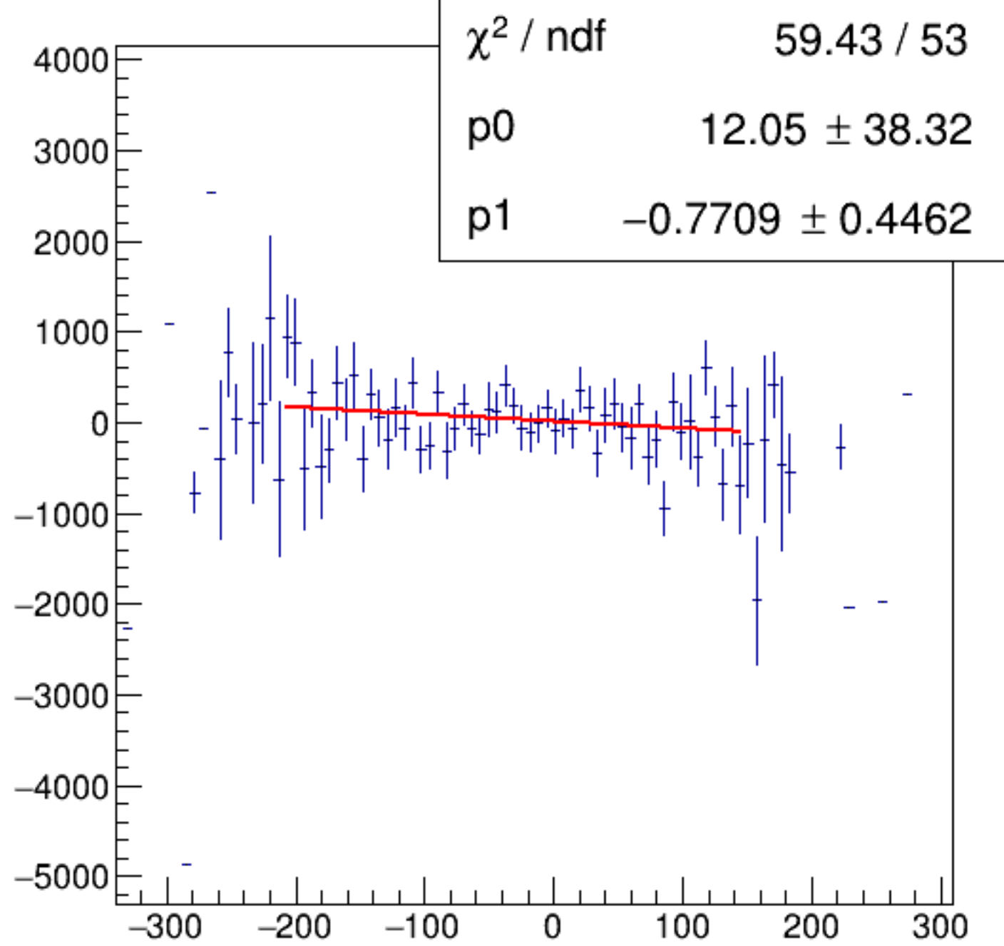
cor_usl/ppm:AqDS/ppm {ErrorFlag==0}
