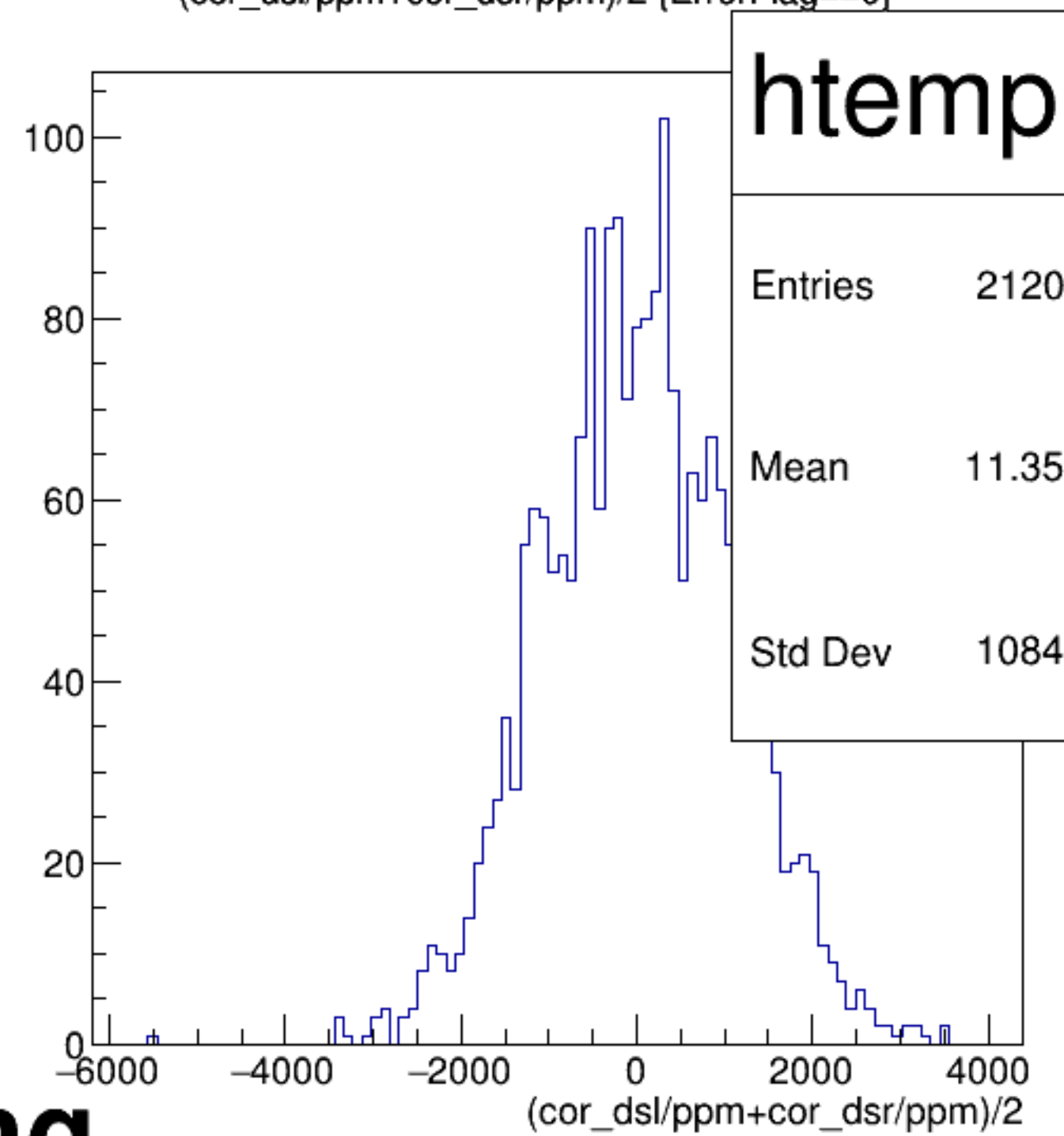
(cor_dsl/ppm+cor_dsr/ppm)/2 {ErrorFlag==0}
