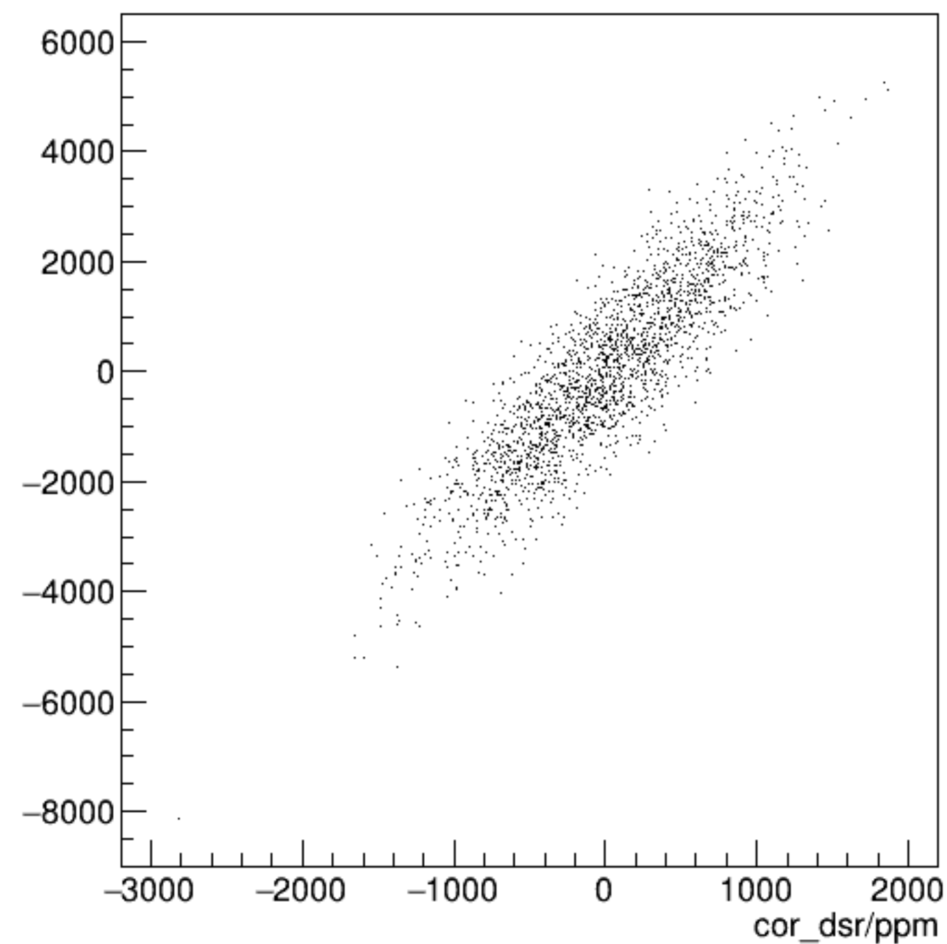
cor_dsl/ppm:cor_dsr/ppm {ErrorFlag==0}
