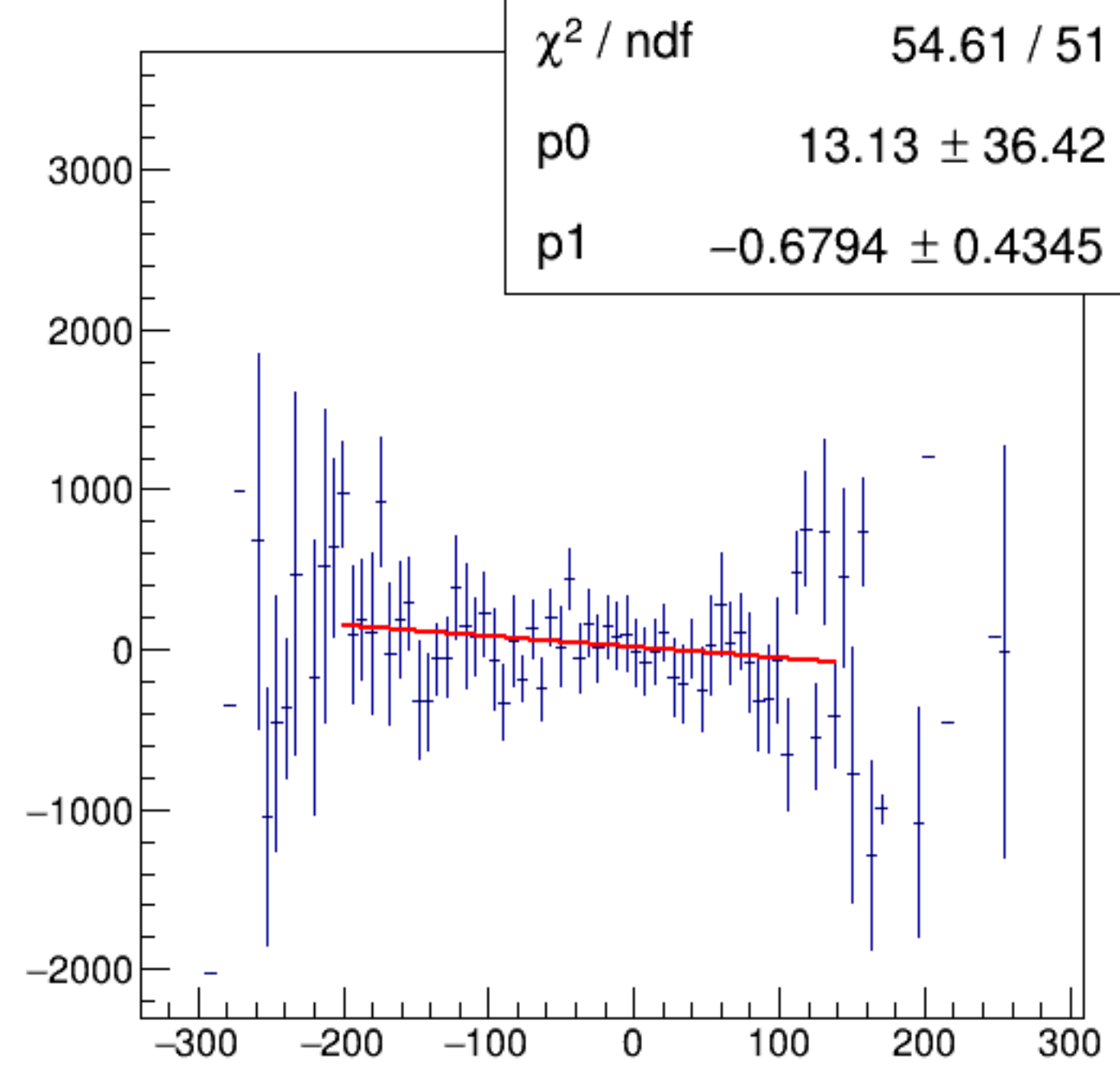
cor_dsl/ppm:AqDS/ppm {ErrorFlag==0}
