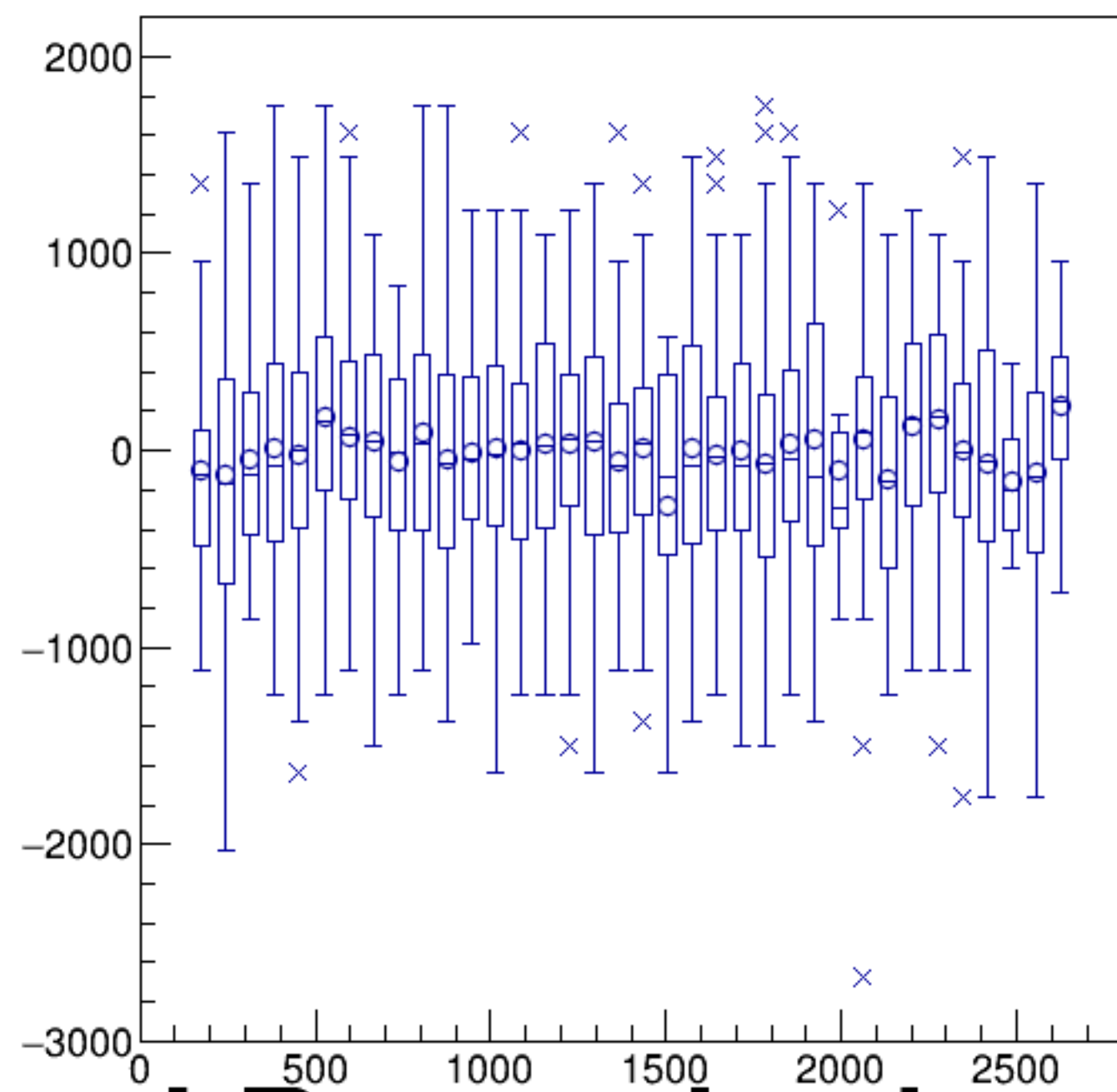
(cor_dsl/ppm-cor_dsr/ppm)/2:pattern_number {ErrorFlag==0}
