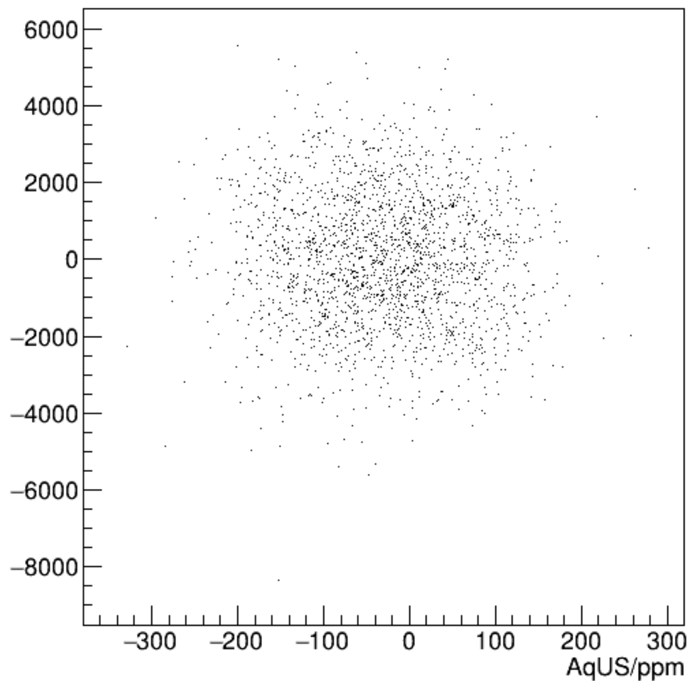
cor_usl/ppm:AqUS/ppm {ErrorFlag==0}
