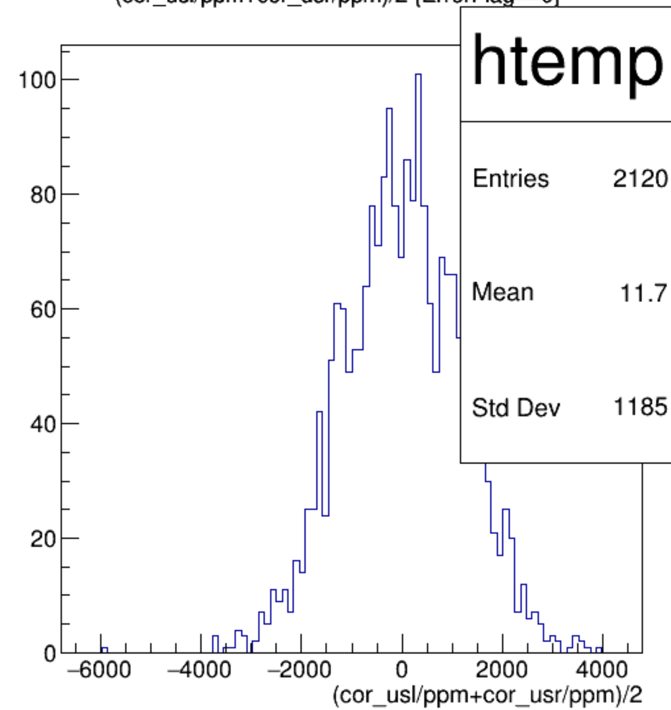
(cor_usr/ppm+cor_usr/ppm)/2 {ErrorFlag==0}
