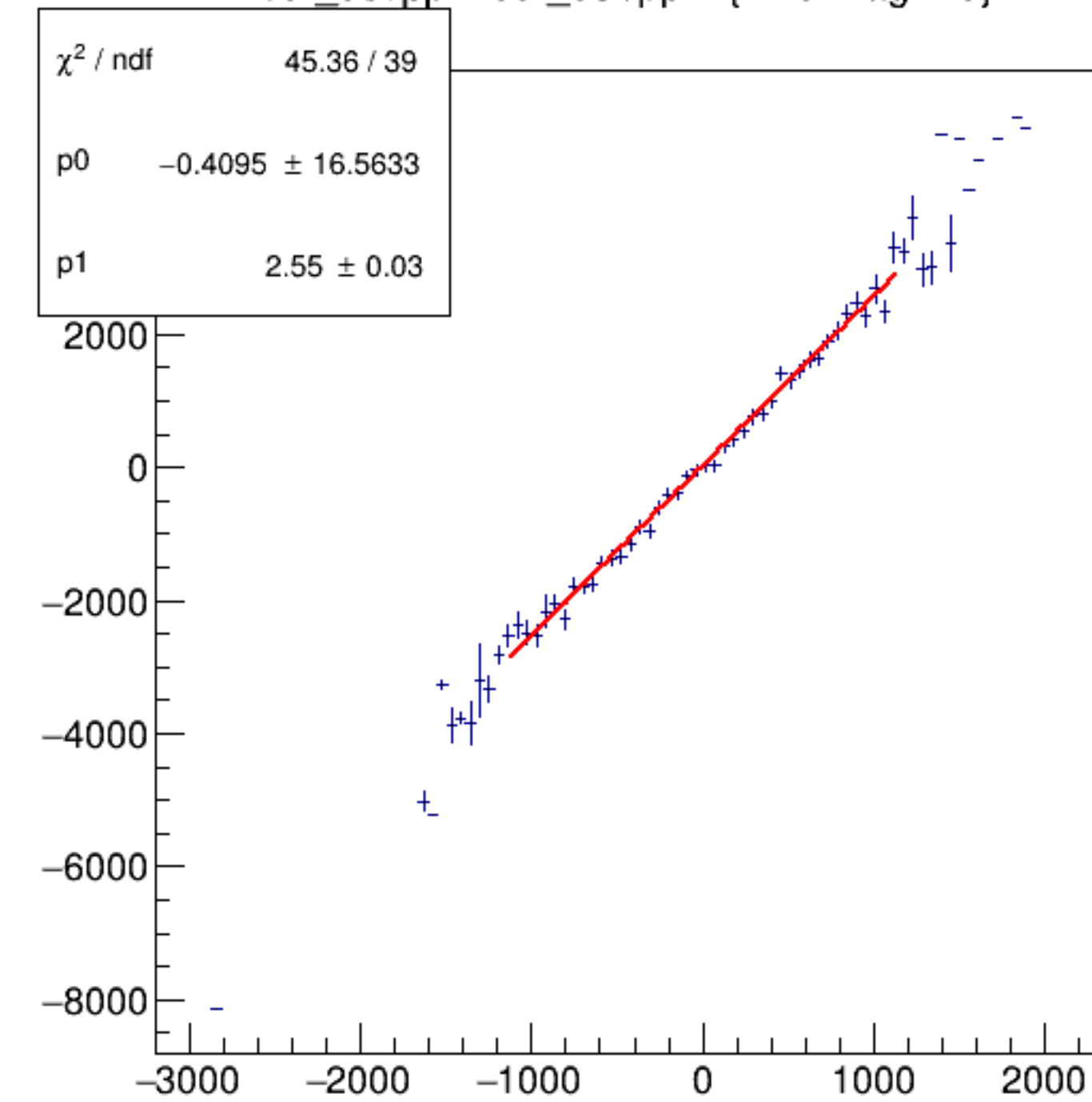
cor_dsl/ppm:cor_dsr/ppm {ErrorFlag==0}
