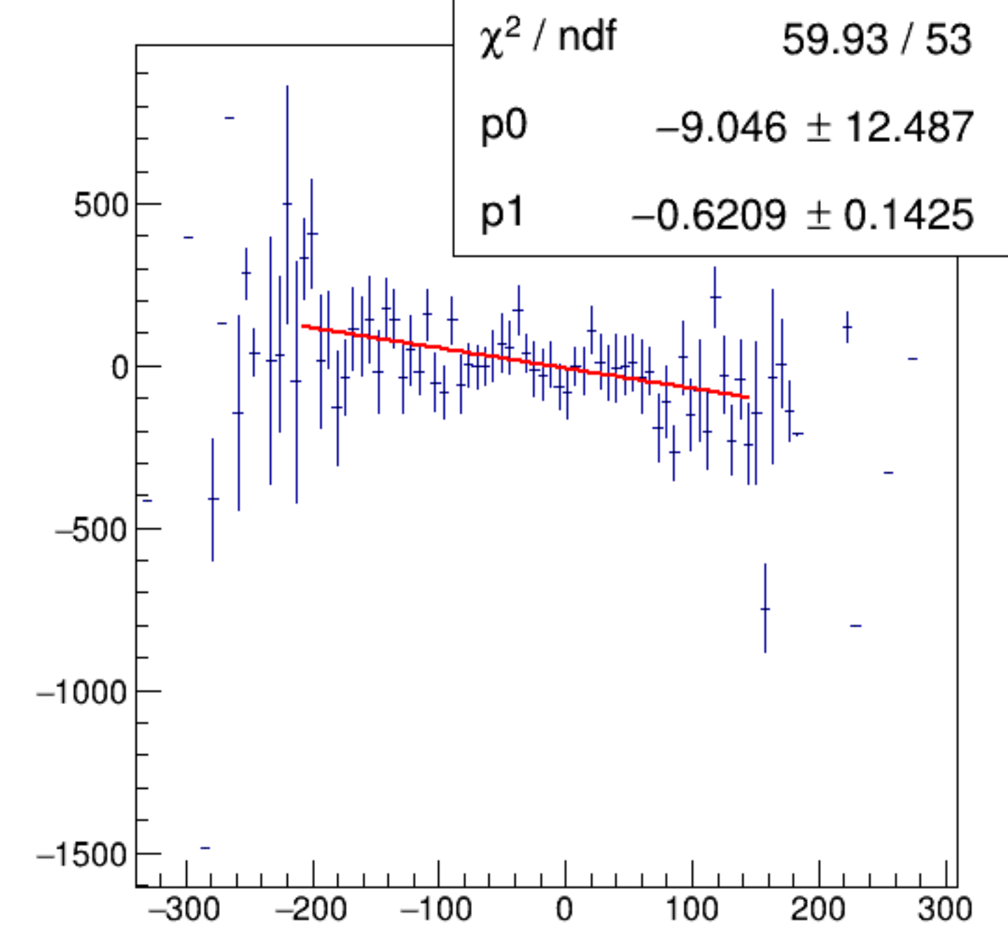
cor_dsr/ppm:AqDS/ppm {ErrorFlag==0}
