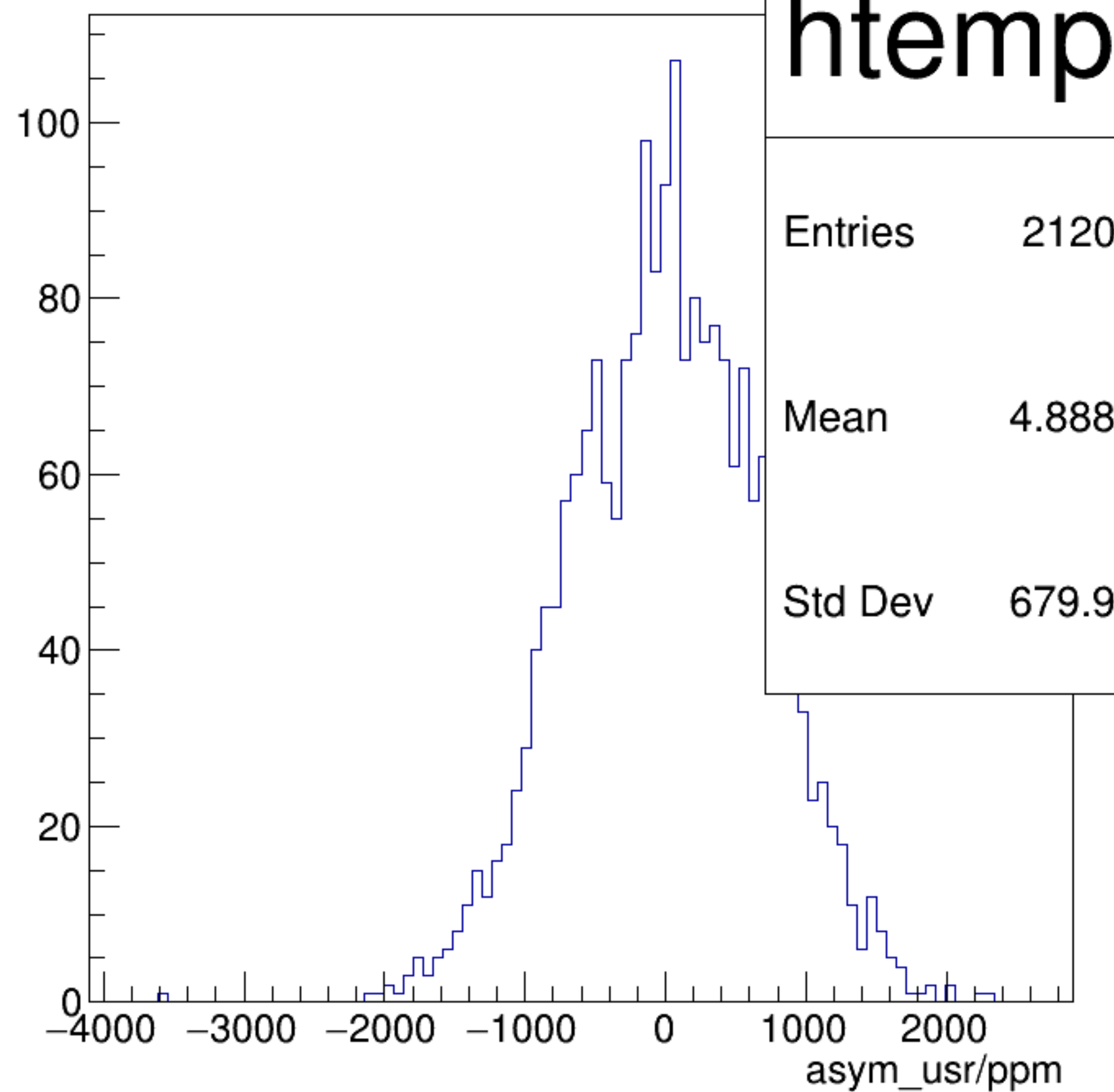
asym_usr/ppm {ErrorFlag==0}
