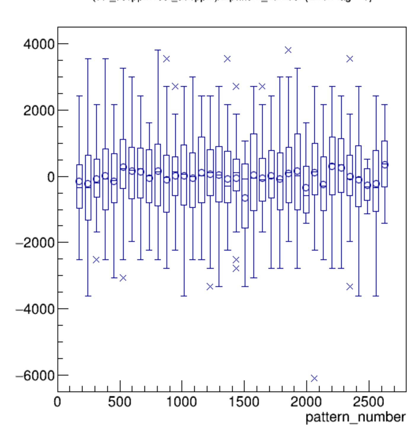
(cor_usr/ppm+cor_usr/ppm)/2:pattern_number {ErrorFlag==0}
