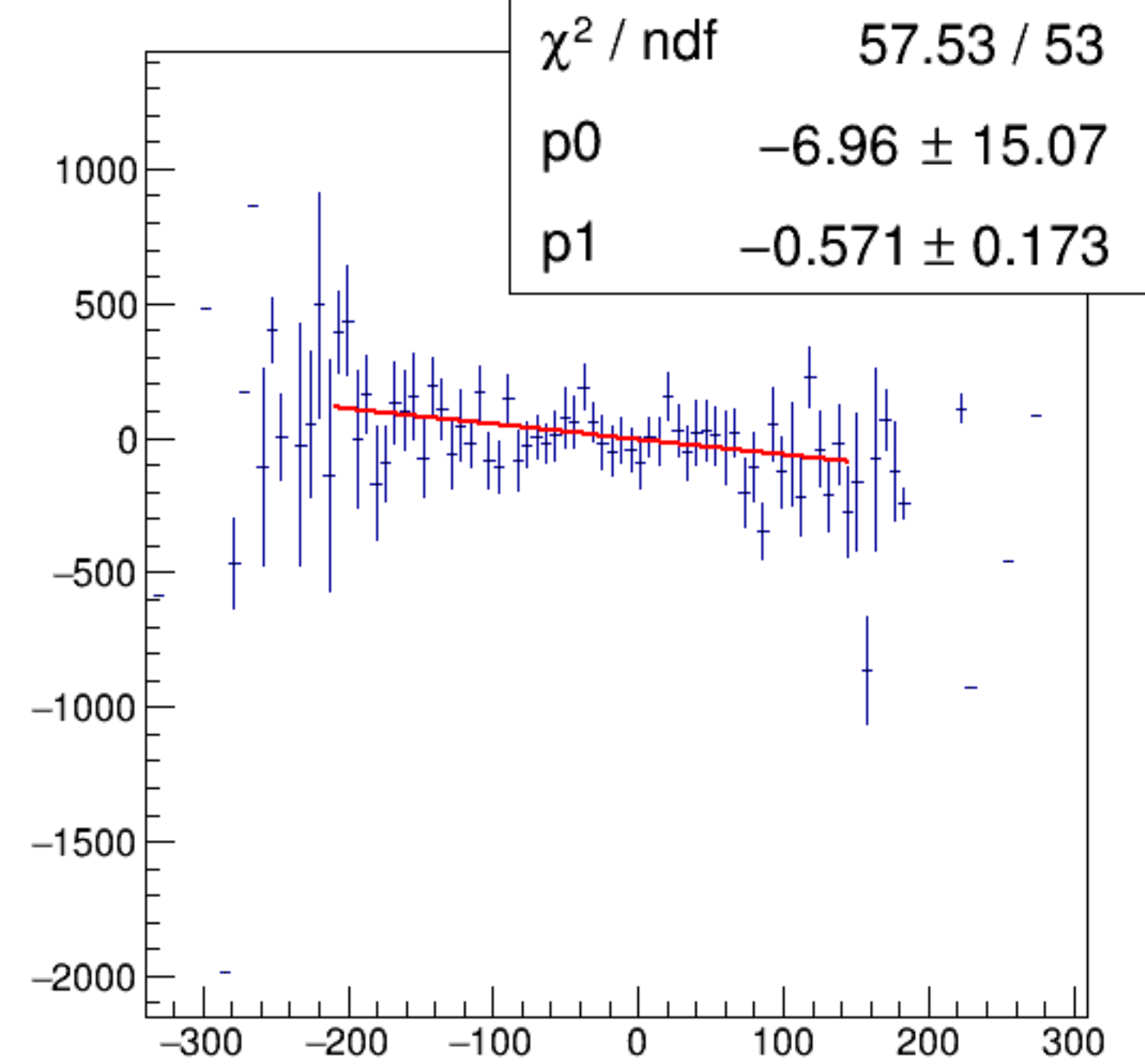
cor_usr/ppm:AqDS/ppm {ErrorFlag==0}
