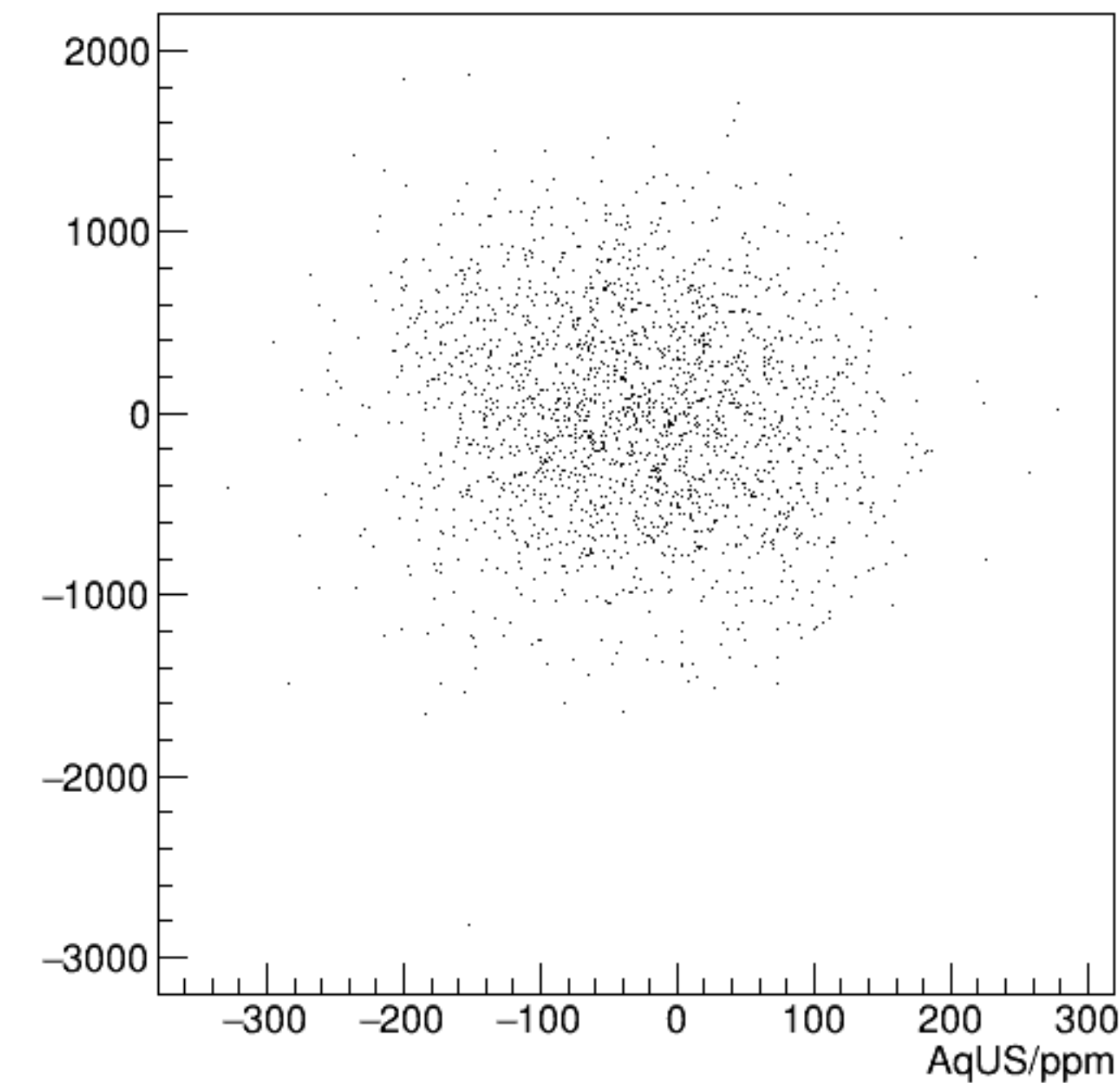
cor_dsr/ppm:AqUS/ppm {ErrorFlag==0}
