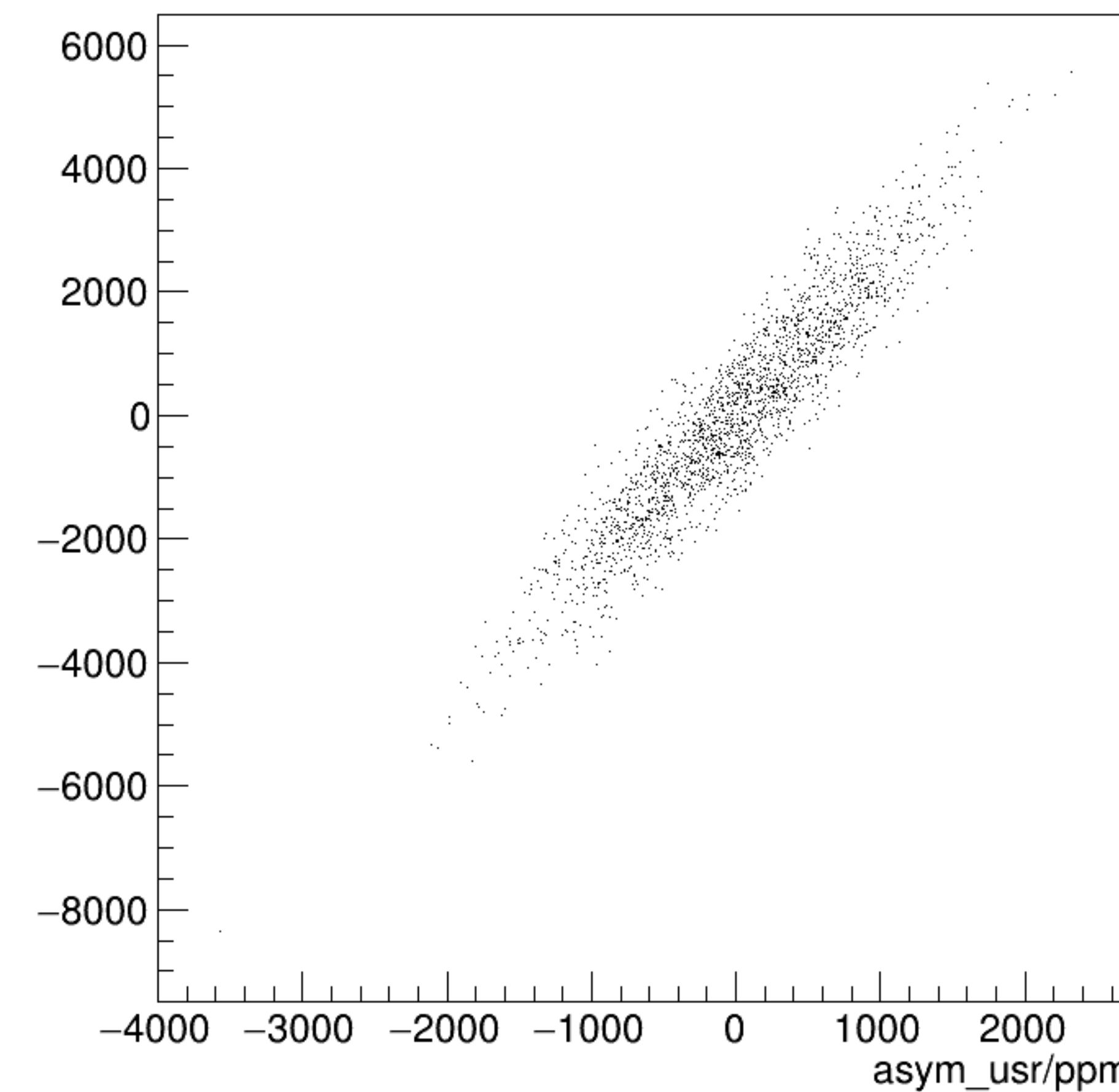
asym_usl/ppm:asym_usr/ppm {ErrorFlag==0}
