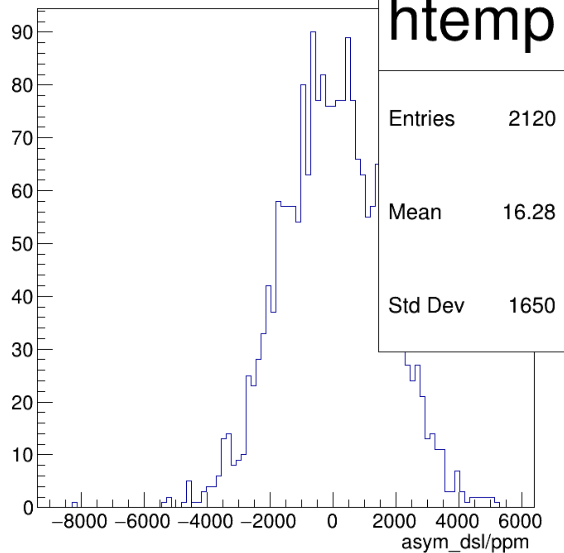
asym_dsl/ppm {ErrorFlag==0}
