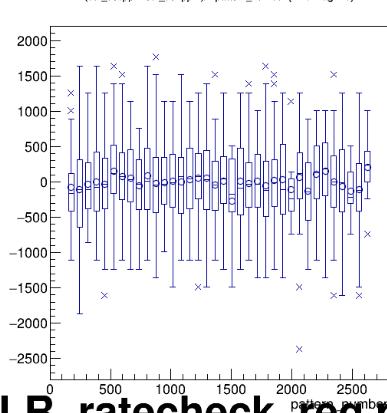
(cor_usr/ppm-cor_usr/ppm)/2:pattern_number {ErrorFlag==0}
