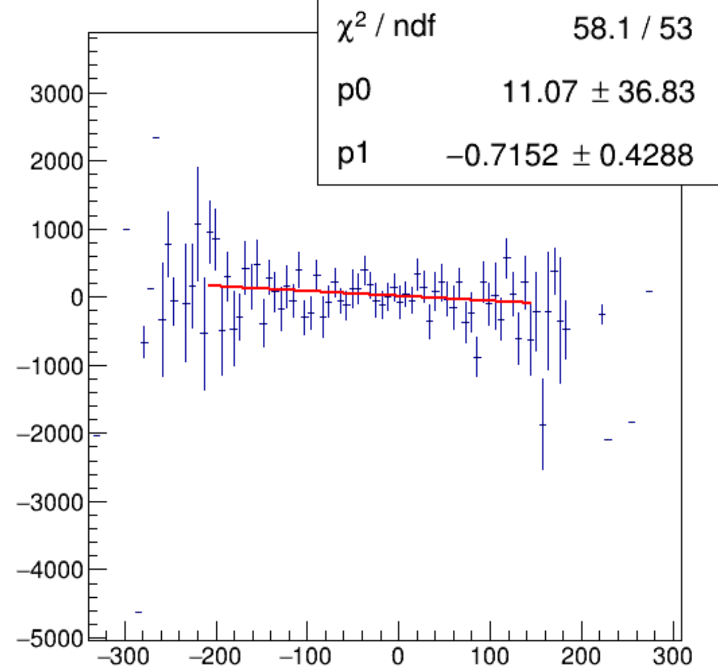
cor_dsl/ppm:AqDS/ppm {ErrorFlag==0}
