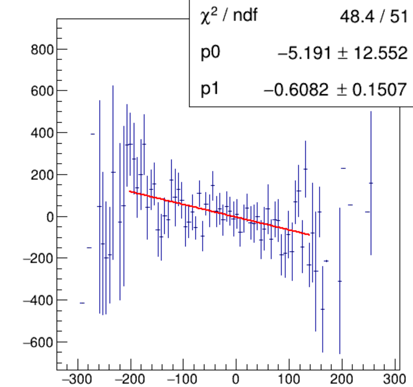
cor_dsr/ppm:AqDS/ppm {ErrorFlag==0}
