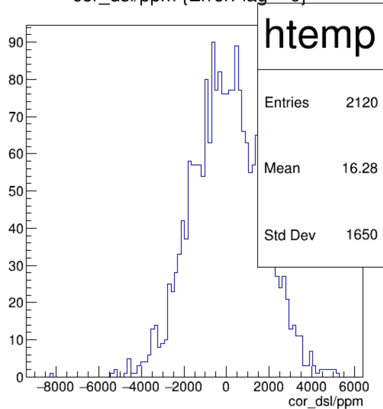
cor_dsl/ppm {ErrorFlag==0}
