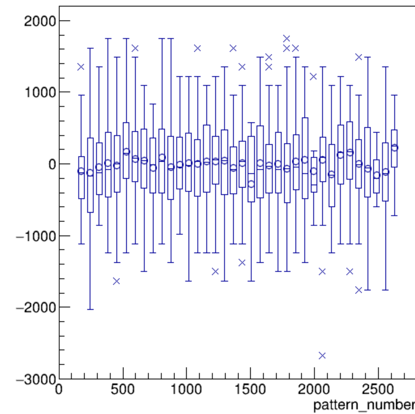
(cor_dsl/ppm-cor_dsr/ppm)/2:pattern_number {ErrorFlag==0}
