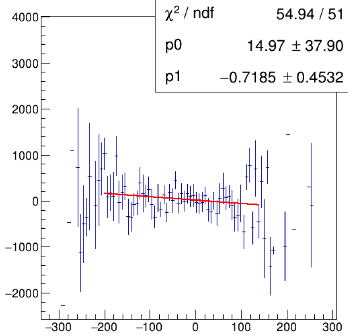
cor_usr/ppm:AqDS/ppm {ErrorFlag==0}
