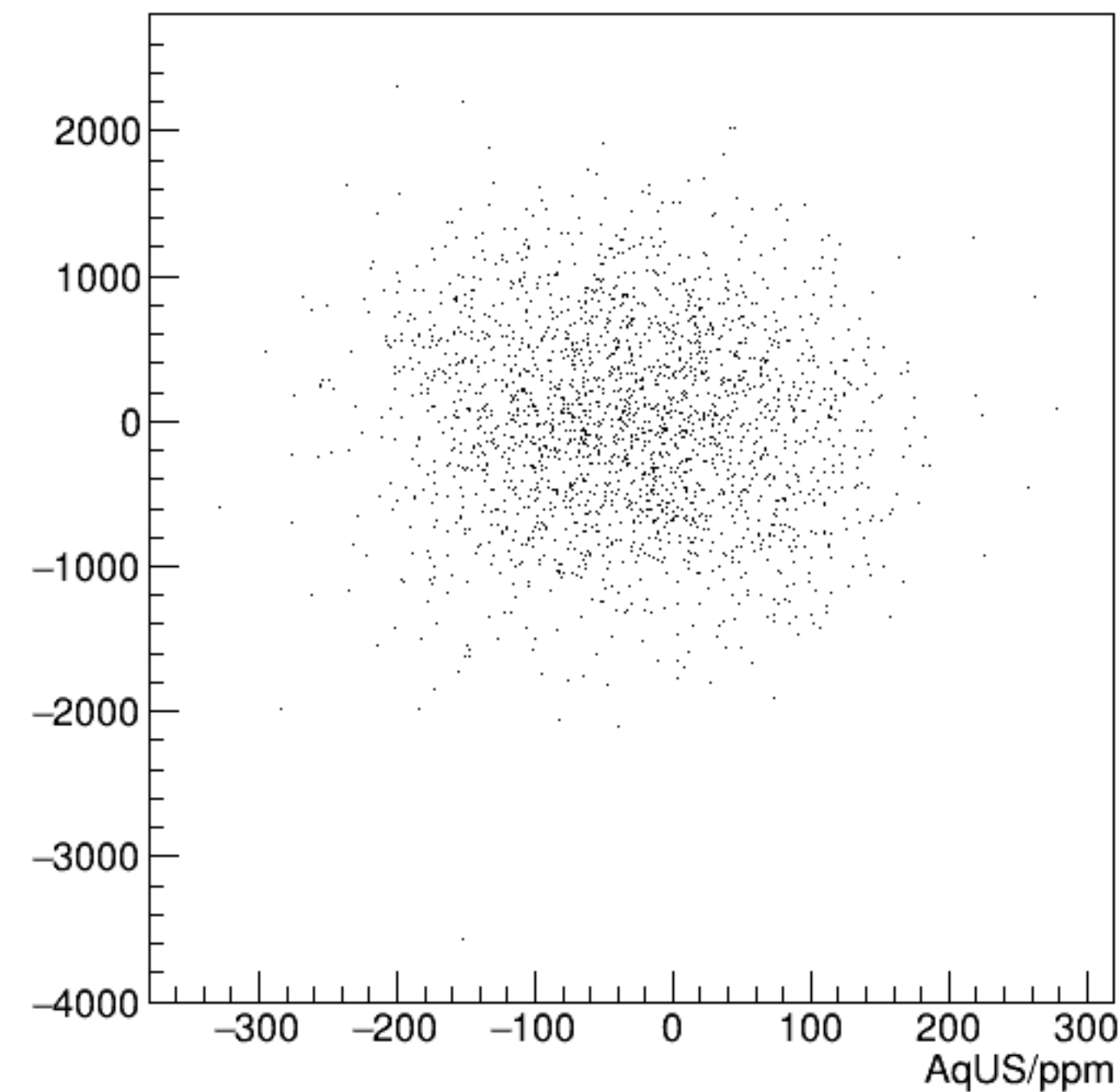
cor_usr/ppm:AqUS/ppm {ErrorFlag==0}
