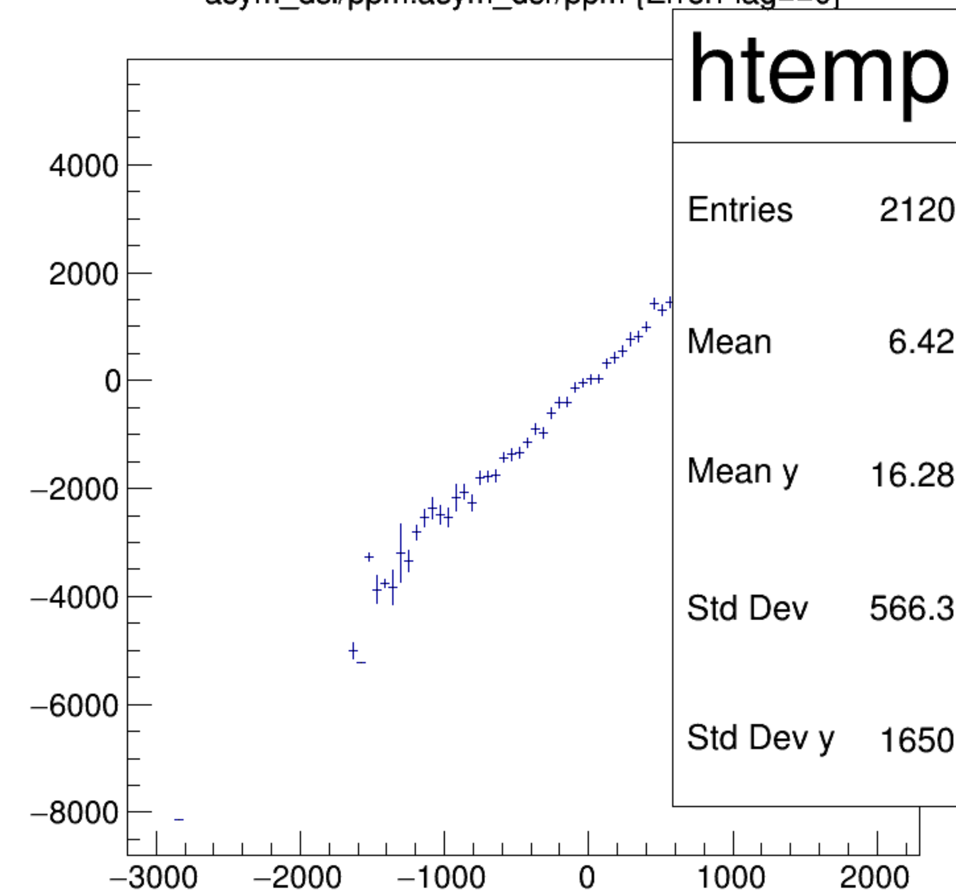
asym_dsl/ppm:asym_dsr/ppm {ErrorFlag==0}
