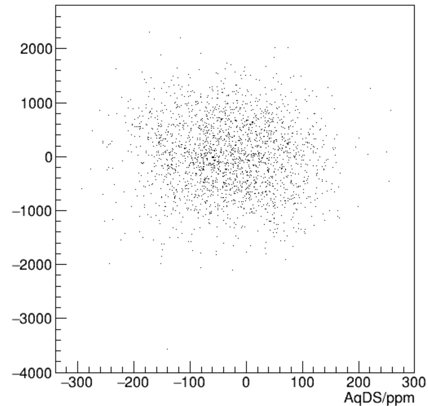
cor_usr/ppm:AqDS/ppm {ErrorFlag==0}
