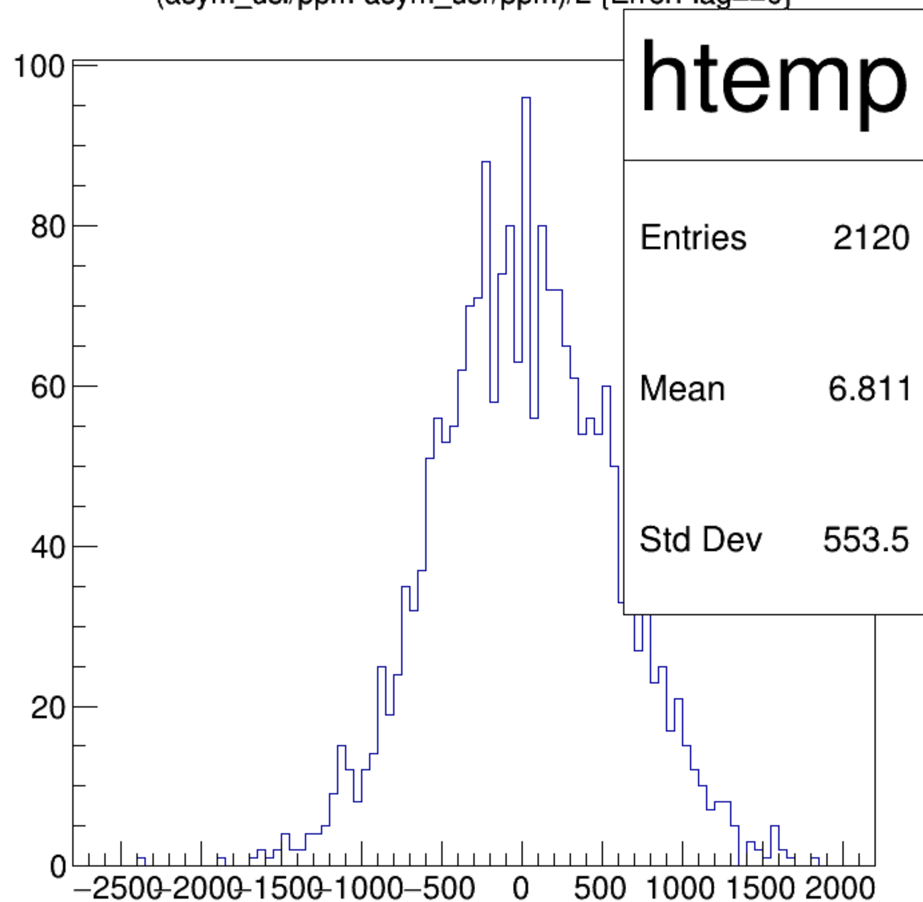
(asym_usl/ppm-asym_usr/ppm)/2 {ErrorFlag==0}
