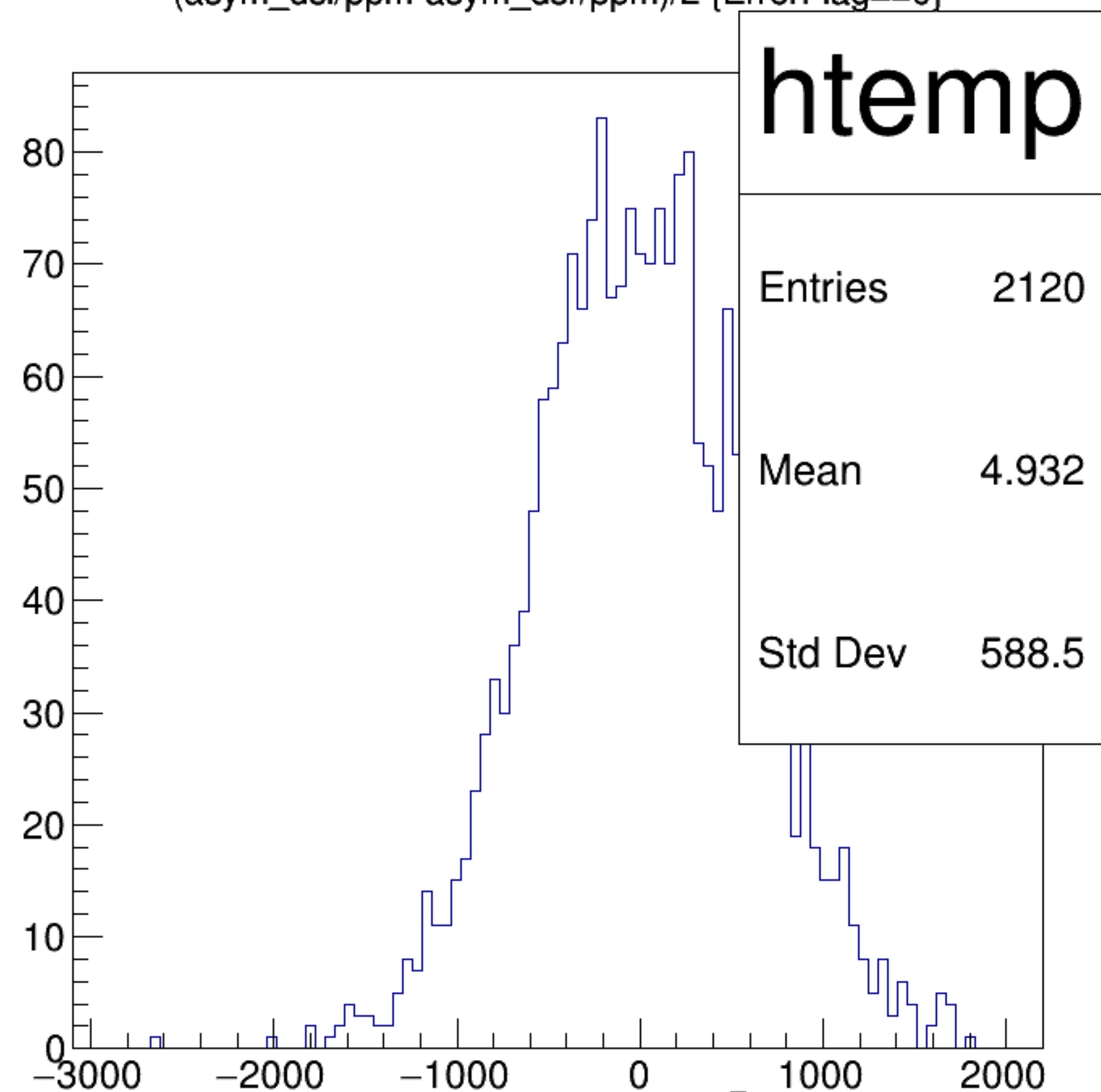
(asym_dsl/ppm-asym_dsr/ppm)/2 {ErrorFlag==0}
