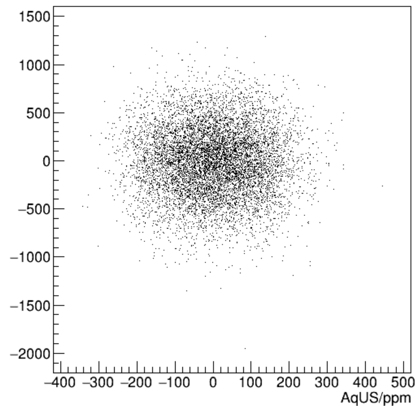
cor_sam5/ppm:AqUS/ppm {ErrorFlag==0}
