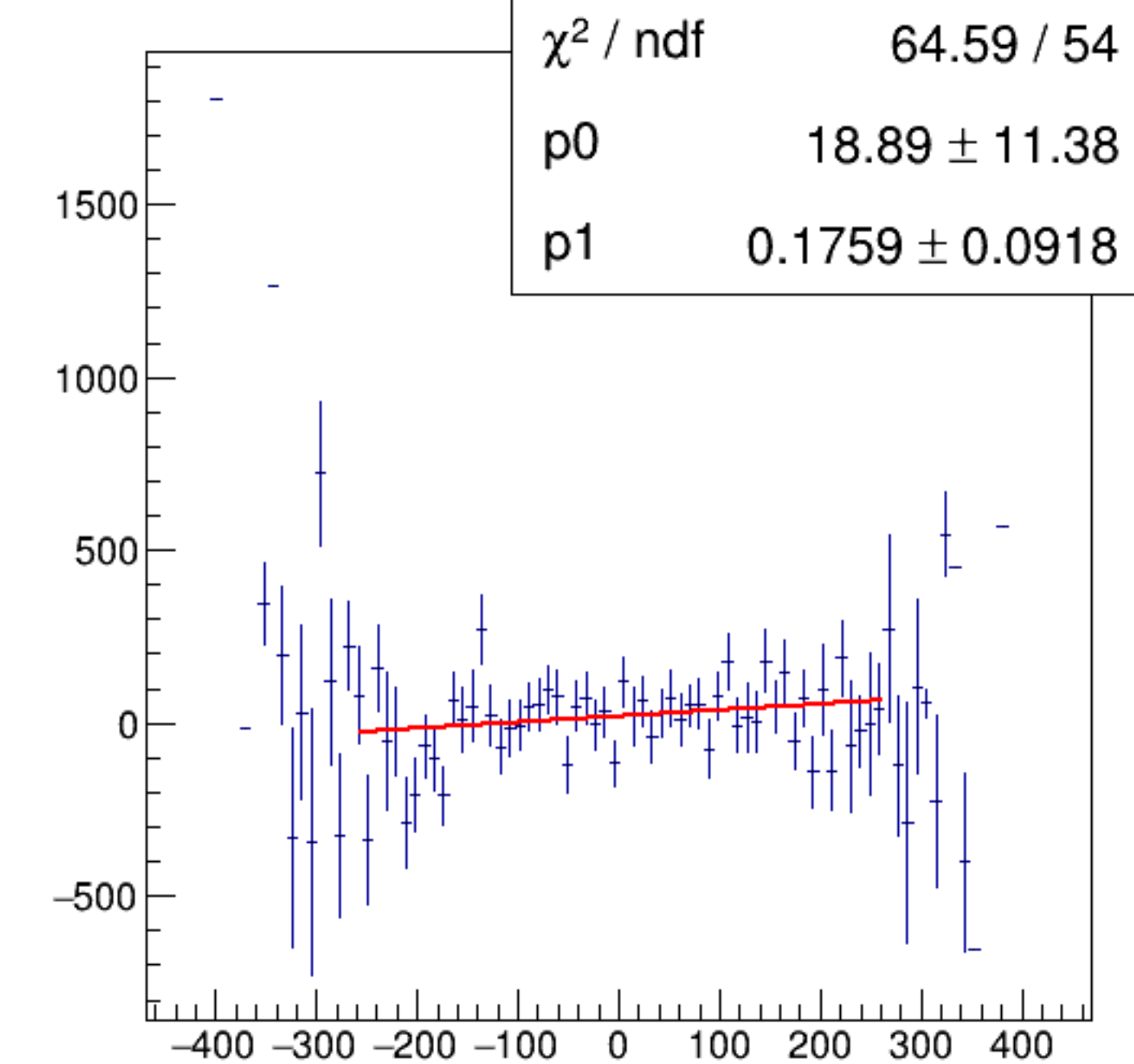
cor_sam3/ppm:AqDS/ppm {ErrorFlag==0}
