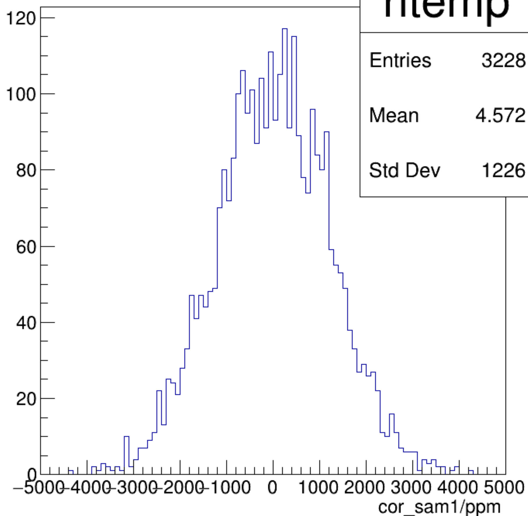
cor_sam1/ppm {ErrorFlag==0}
