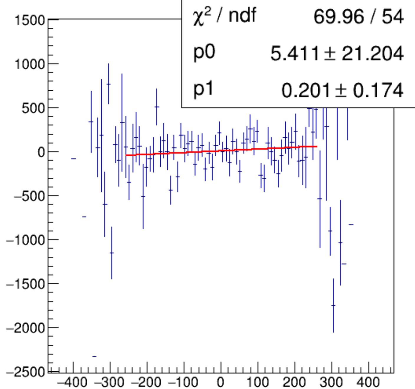
cor_sam1/ppm:AqDS/ppm {ErrorFlag==0}
