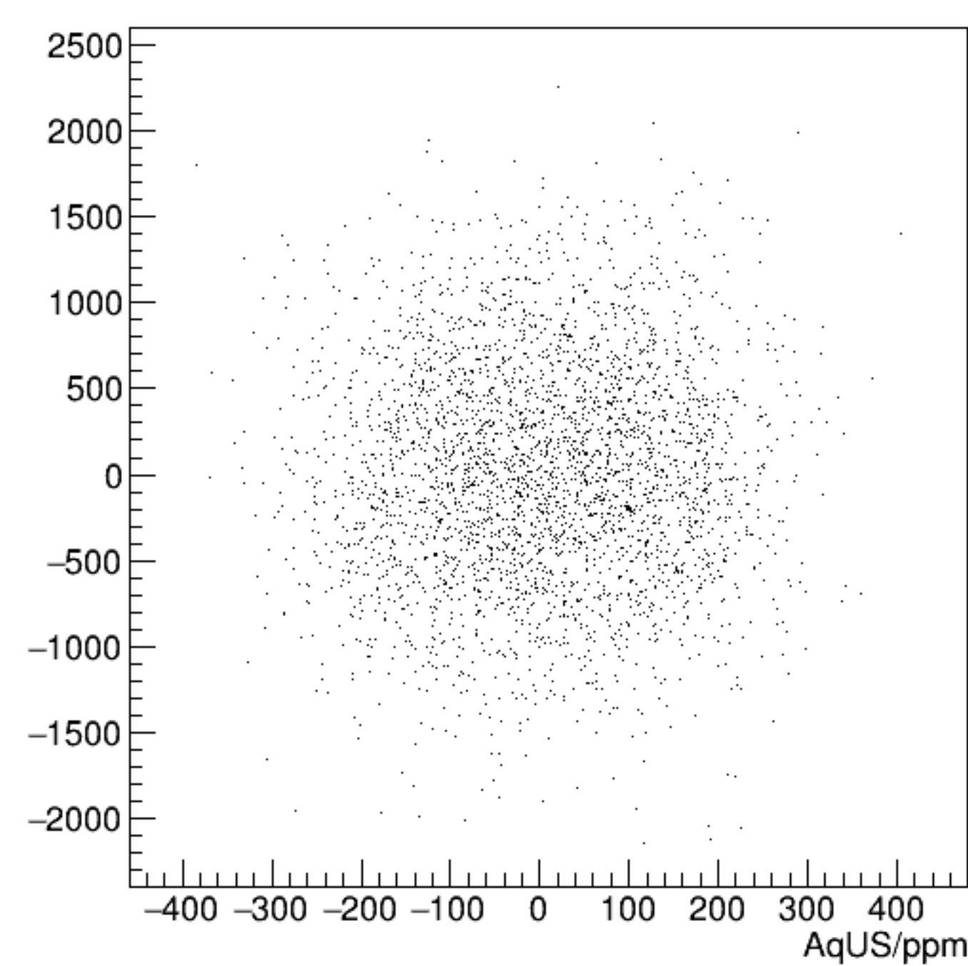
cor_sam3/ppm:AqUS/ppm {ErrorFlag==0}
