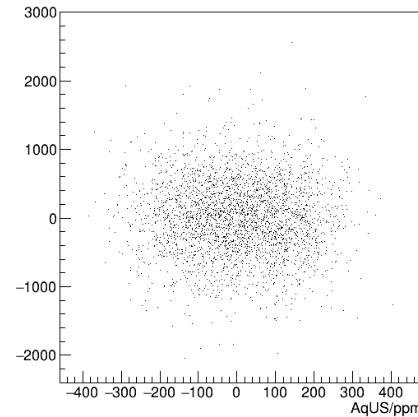
cor_sam7/ppm:AqUS/ppm {ErrorFlag==0}
