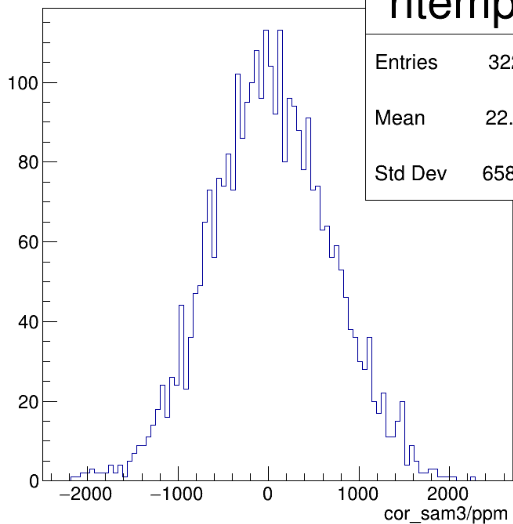
cor_sam3/ppm {ErrorFlag==0}
