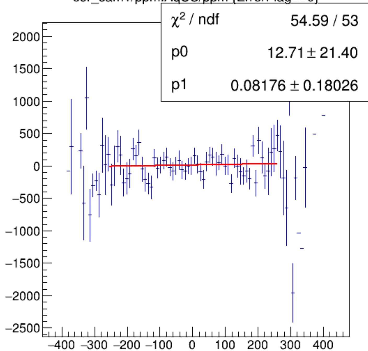
cor_sam1/ppm:AqUS/ppm {ErrorFlag==0}
