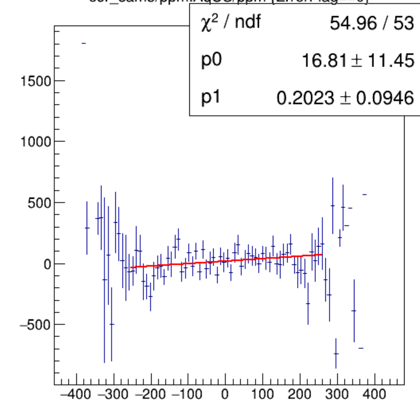
cor_sam3/ppm:AqUS/ppm {ErrorFlag==0}
