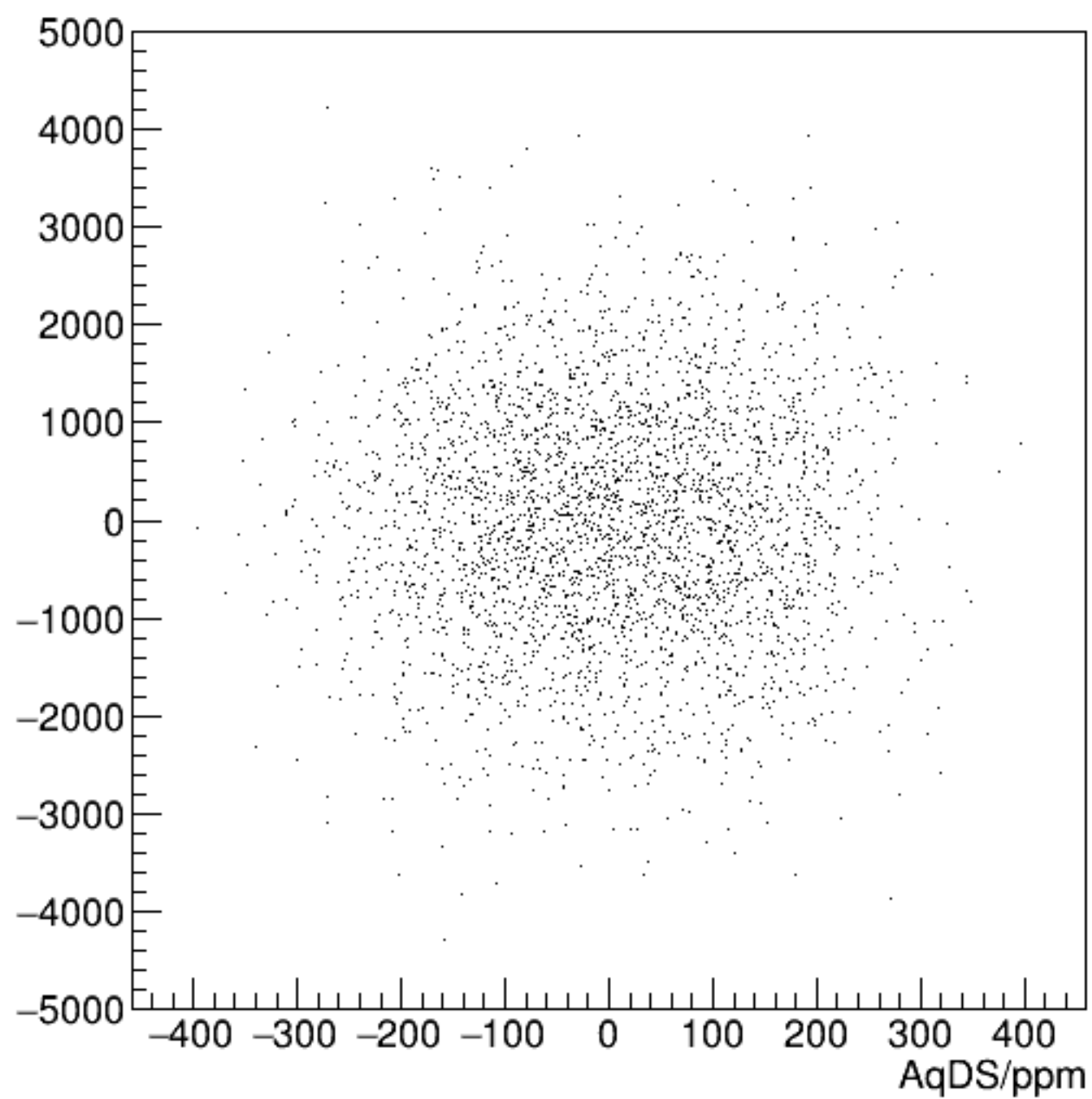
cor_sam1/ppm:AqDS/ppm {ErrorFlag==0}
