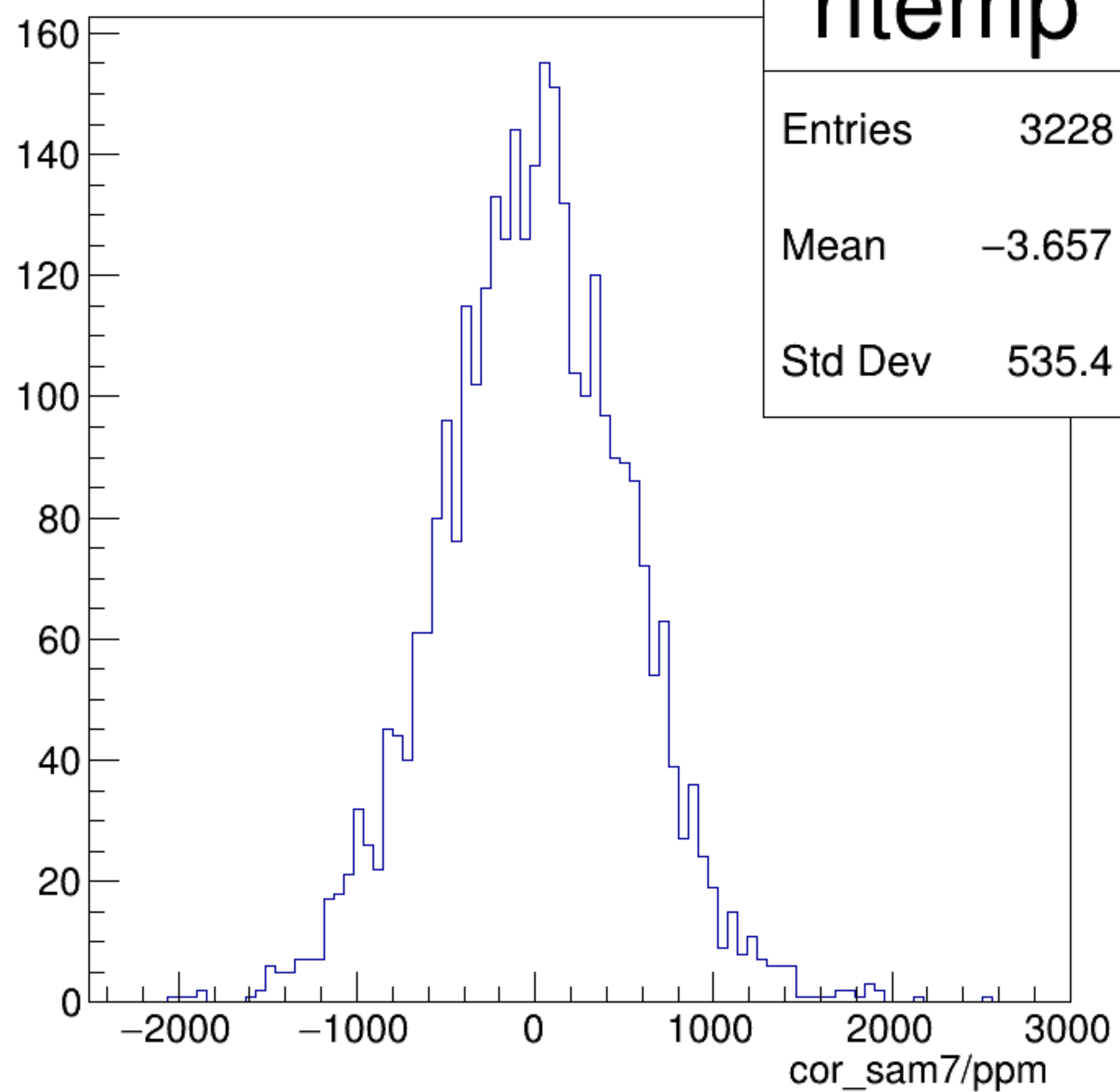
cor_sam7/ppm {ErrorFlag==0}
