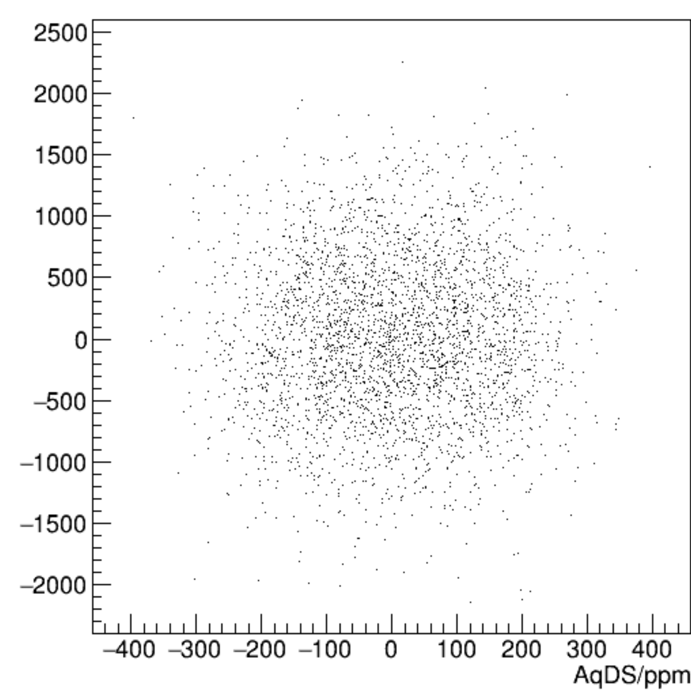
cor_sam3/ppm:AqDS/ppm {ErrorFlag==0}
