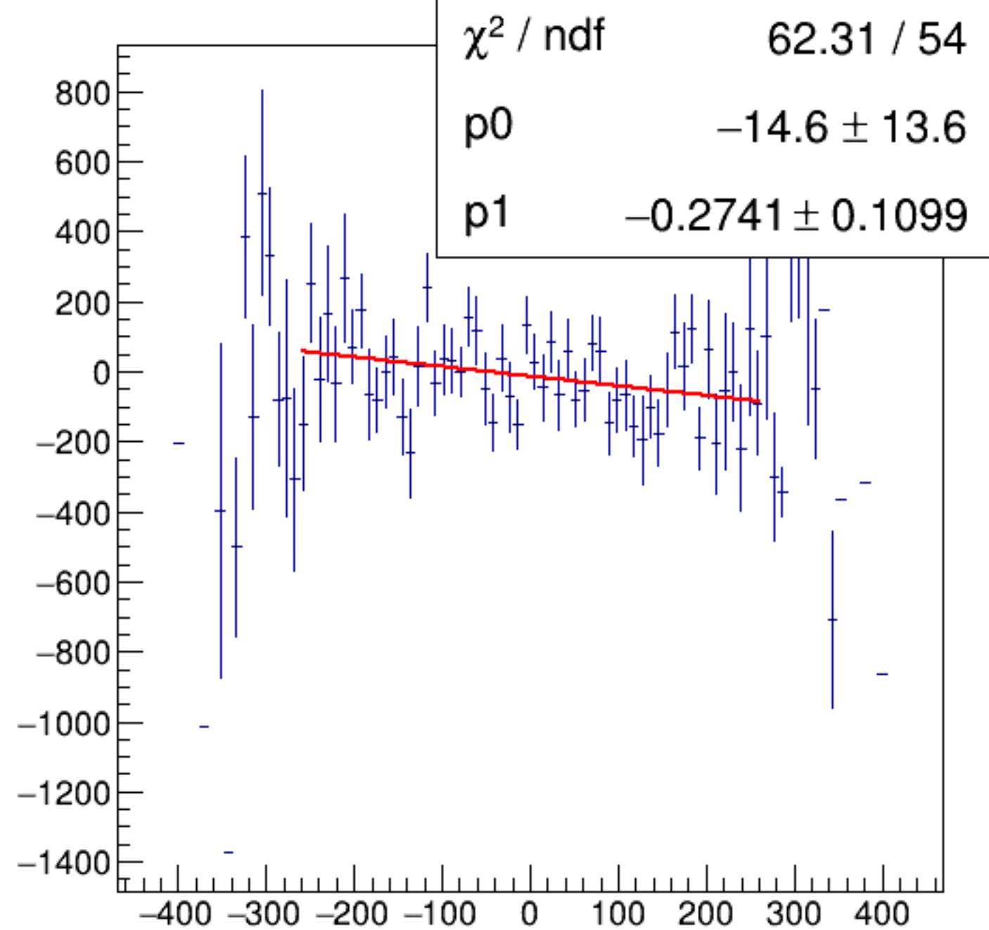
cor_sam5/ppm:AqDS/ppm {ErrorFlag==0}
