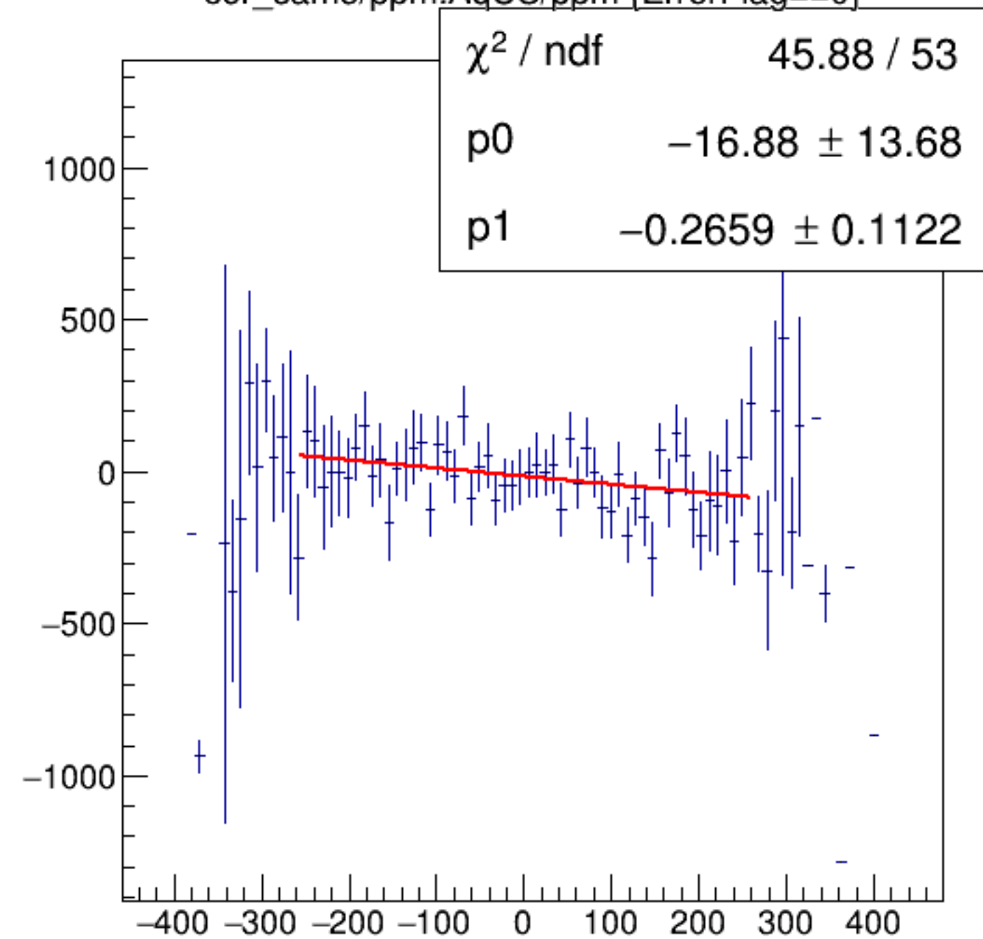
cor_sam5/ppm:AqUS/ppm {ErrorFlag==0}
