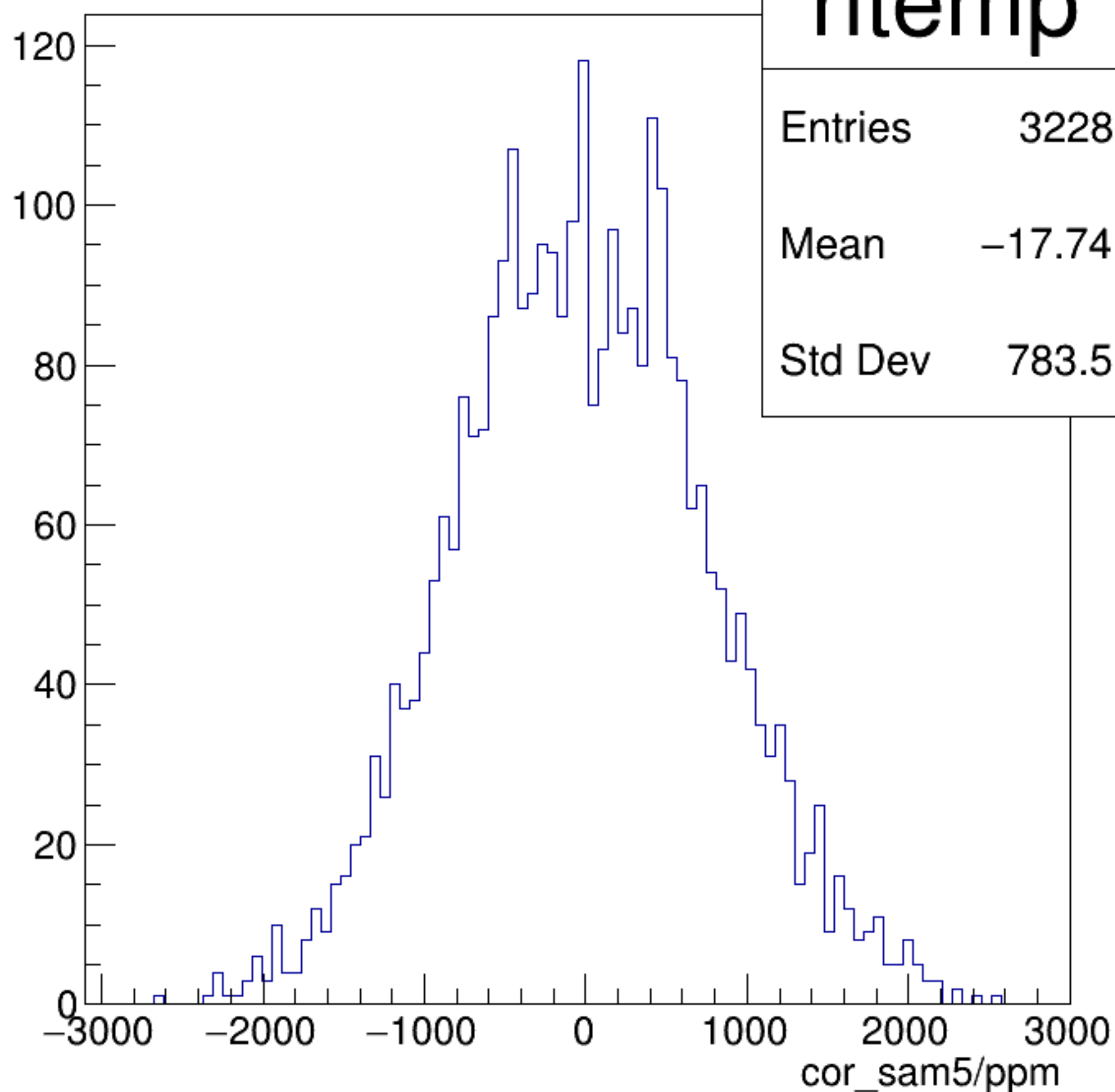
cor_sam5/ppm {ErrorFlag==0}
