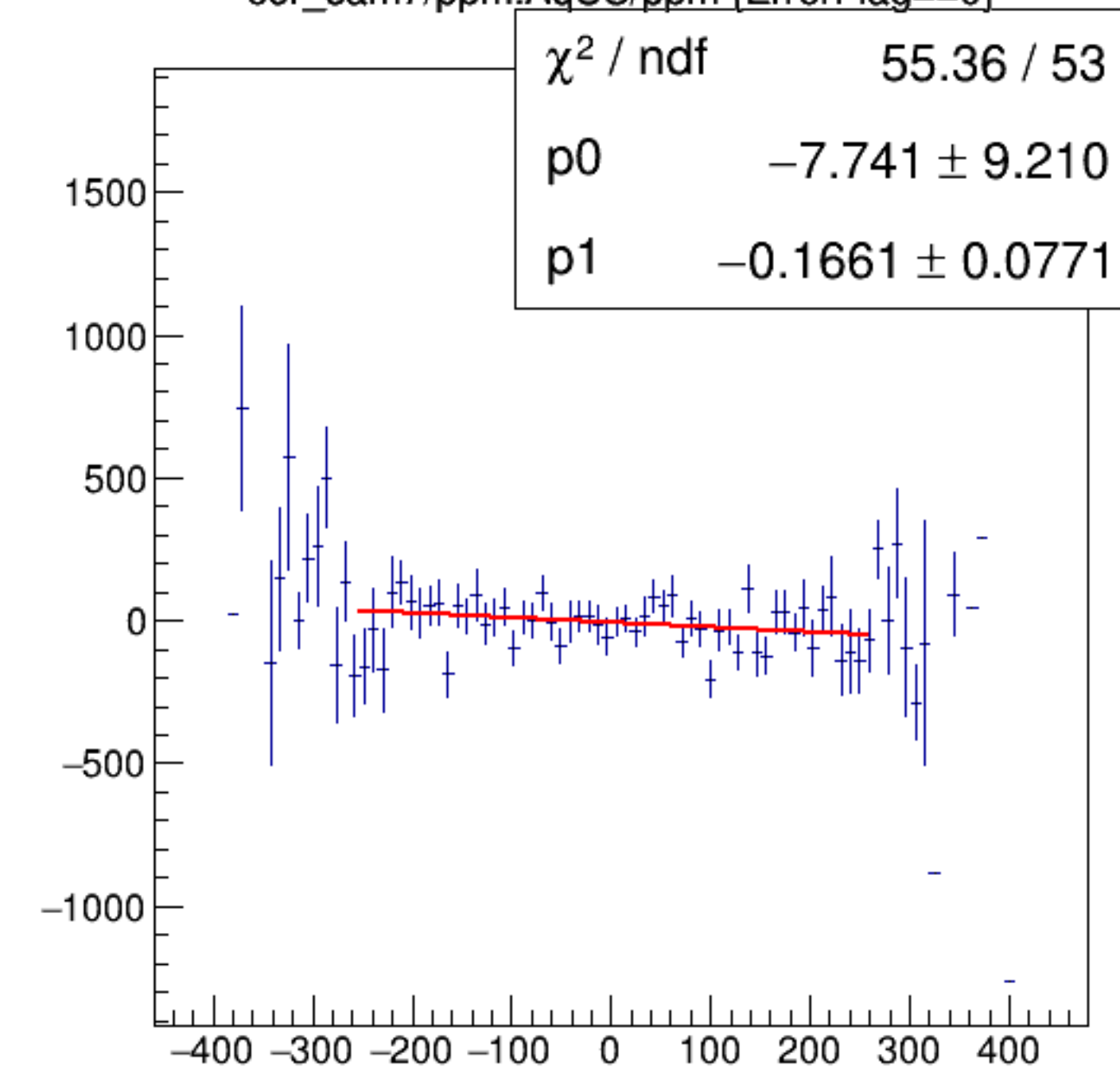
cor_sam7/ppm:AqUS/ppm {ErrorFlag==0}
