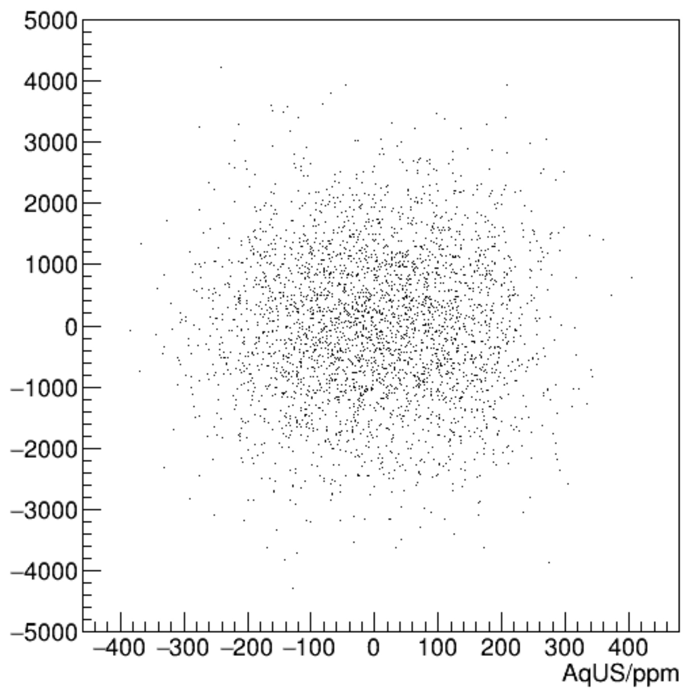
cor_sam1/ppm:AqUS/ppm {ErrorFlag==0}
