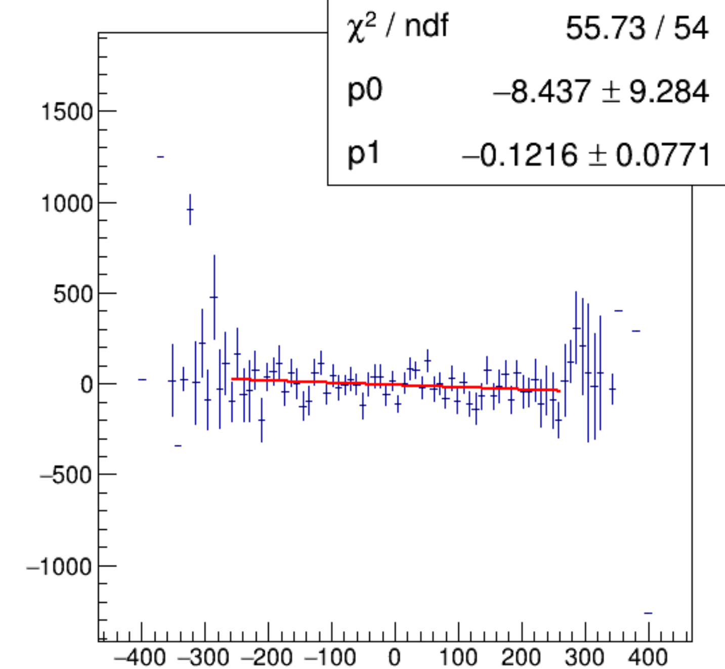
cor_sam7/ppm:AqDS/ppm {ErrorFlag==0}
