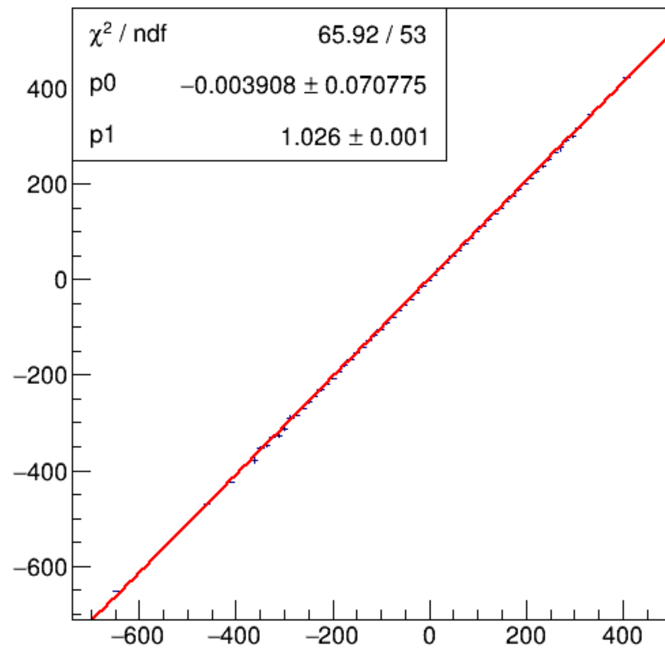
run3132_000_asym_bcm_an_ds_vs_asym_bcm_an_ds3.png
