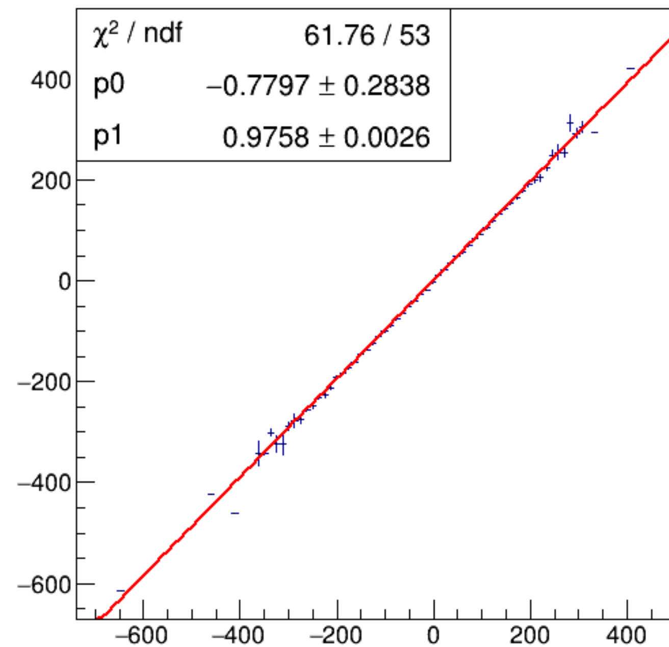
run3132_000_asym_bcm_an_us_vs_asym_bcm_an_ds3.png
