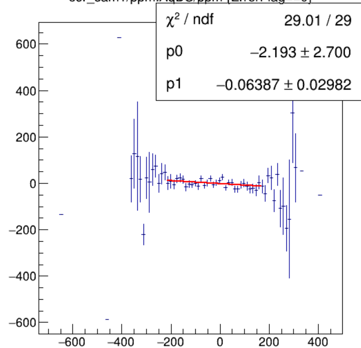
cor_sam1/ppm:AqDS/ppm {ErrorFlag==0}
