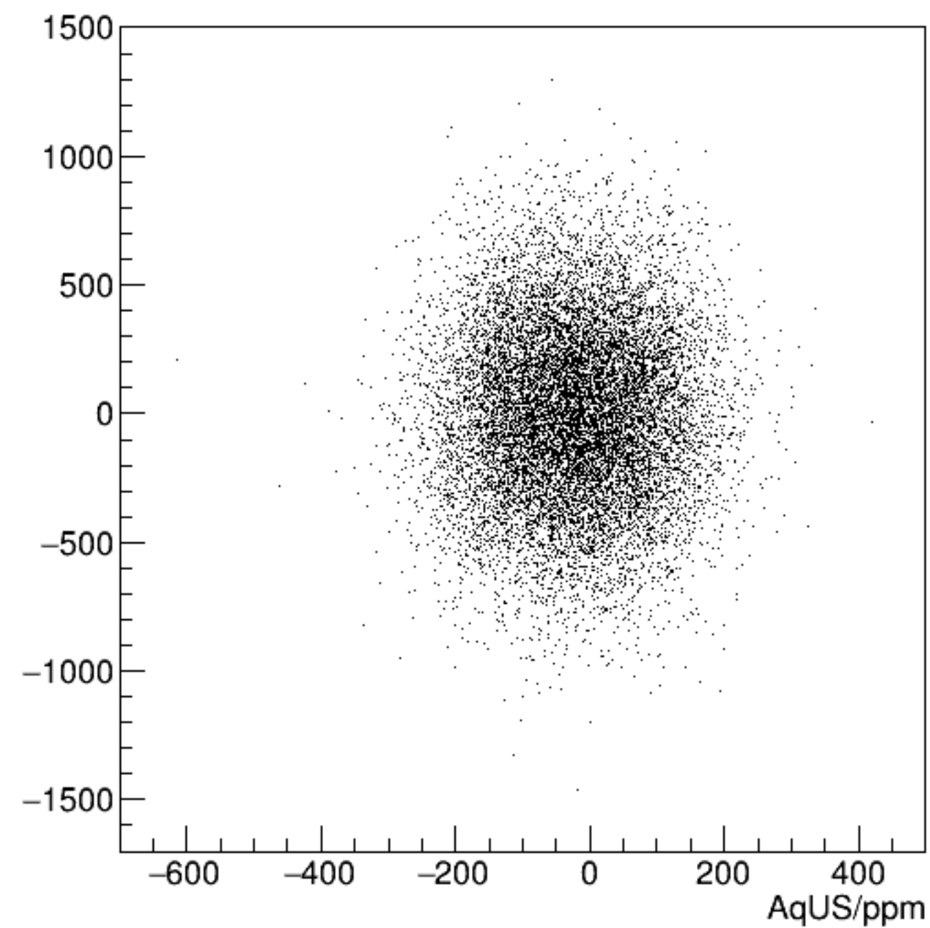
cor_sam5/ppm:AqUS/ppm {ErrorFlag==0}
