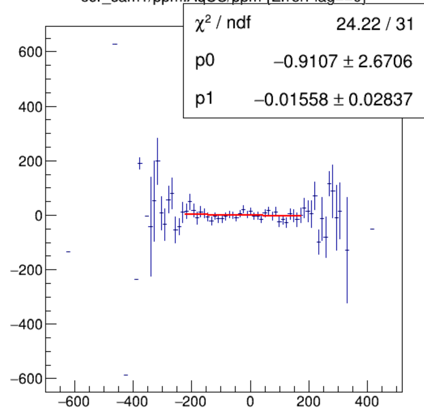
cor_sam1/ppm:AqUS/ppm {ErrorFlag==0}
