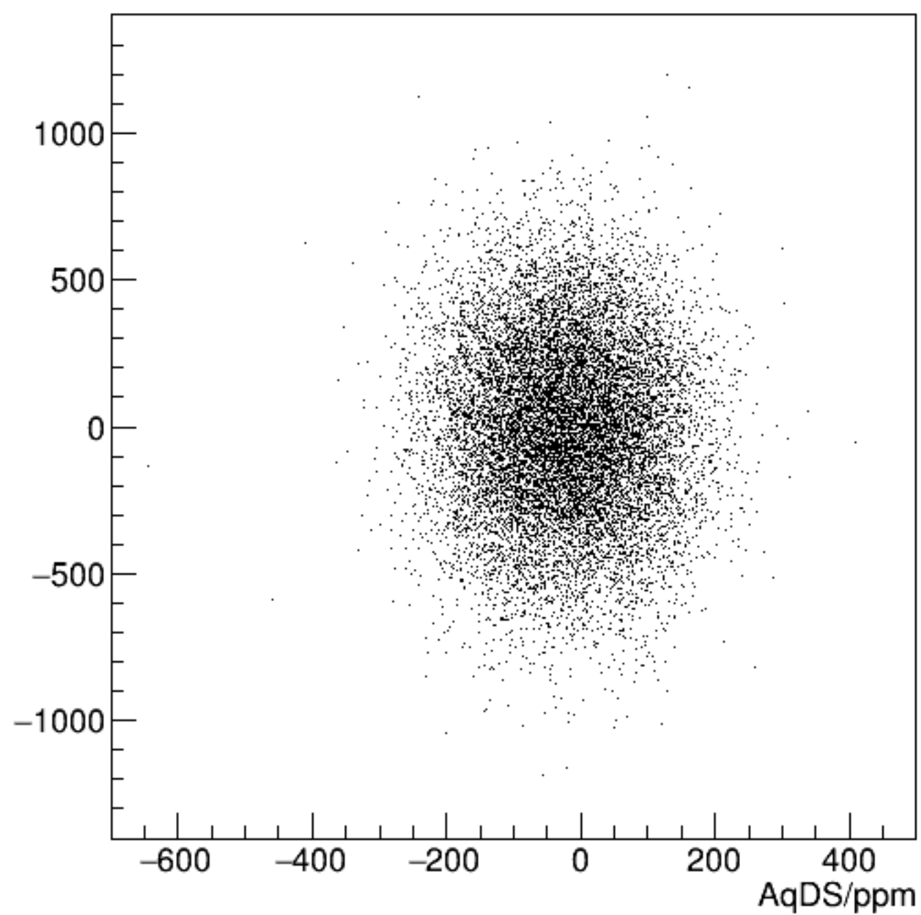
cor_sam1/ppm:AqDS/ppm {ErrorFlag==0}
