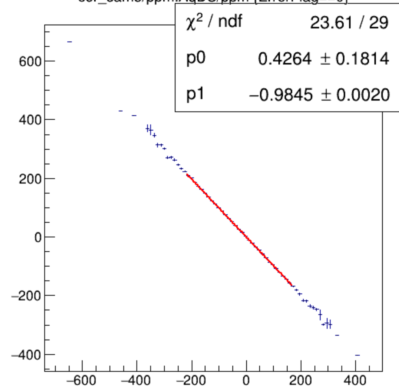
cor_sam3/ppm:AqDS/ppm {ErrorFlag==0}
