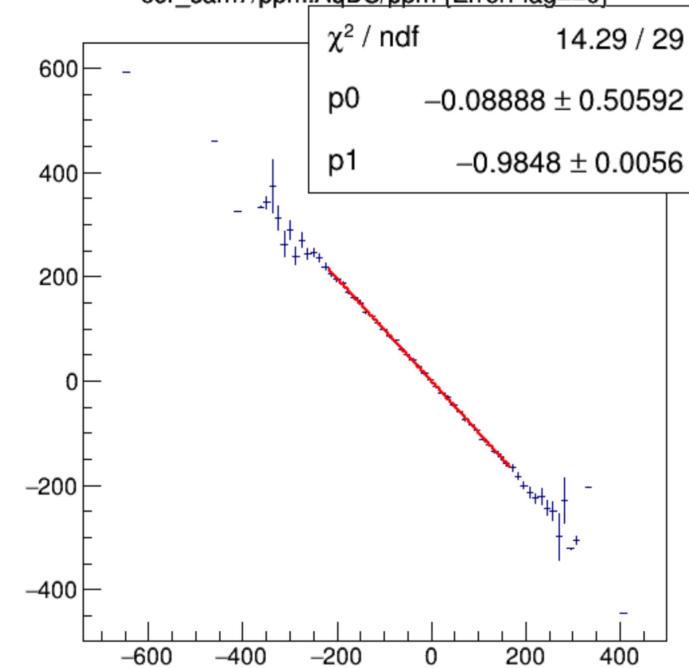
cor_sam7/ppm:AqDS/ppm {ErrorFlag==0}
