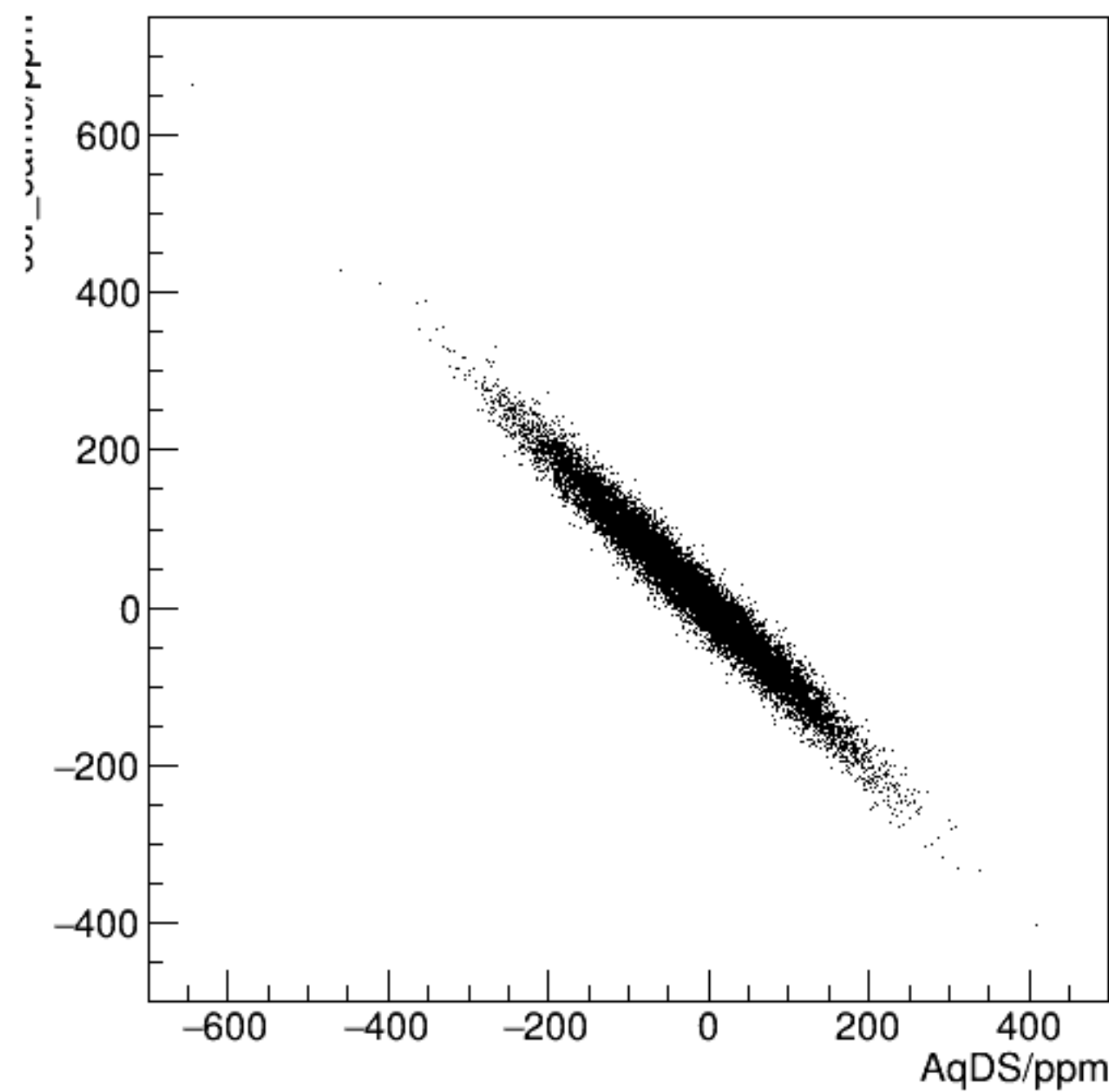
cor_sam3/ppm:AqDS/ppm {ErrorFlag==0}
