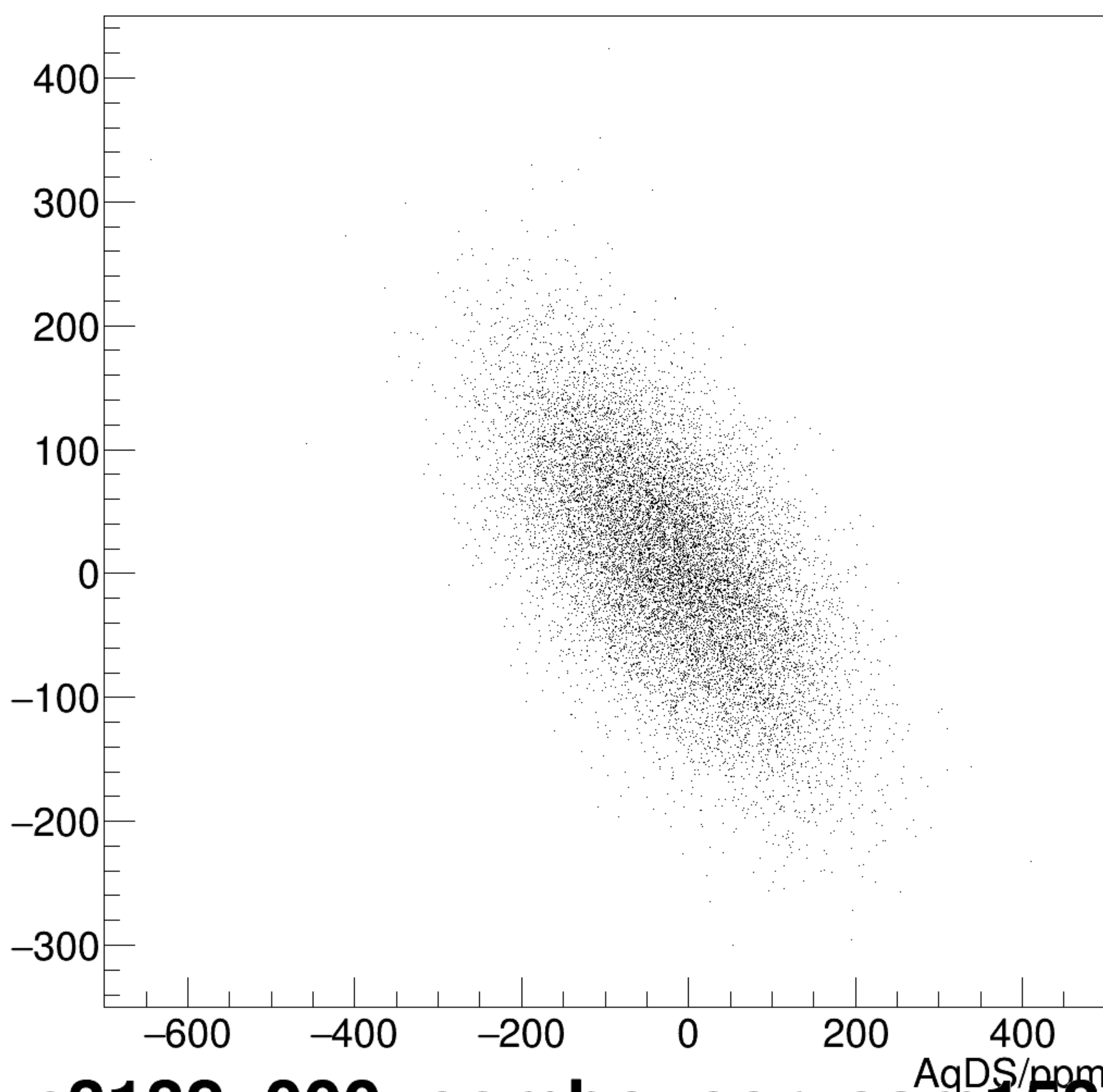
AverageLumi/ppm:AqDS/ppm {ErrorFlag==0}
