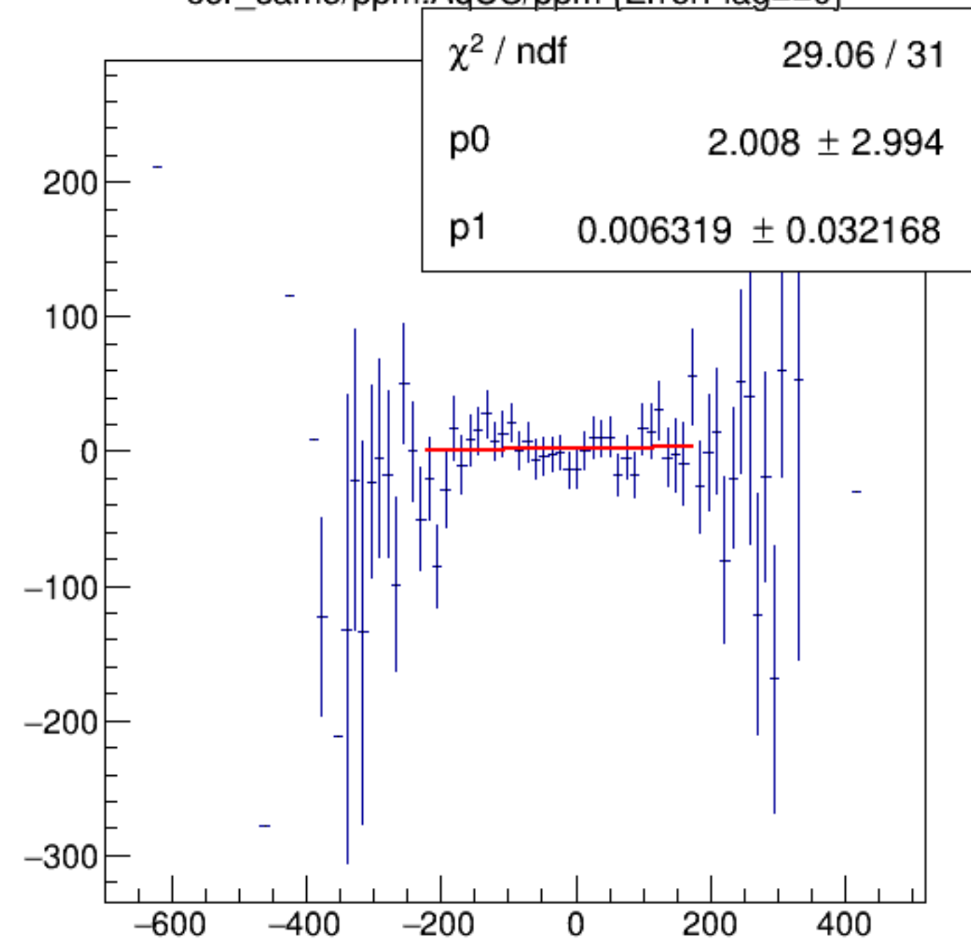
cor_sam5/ppm:AqUS/ppm {ErrorFlag==0}
