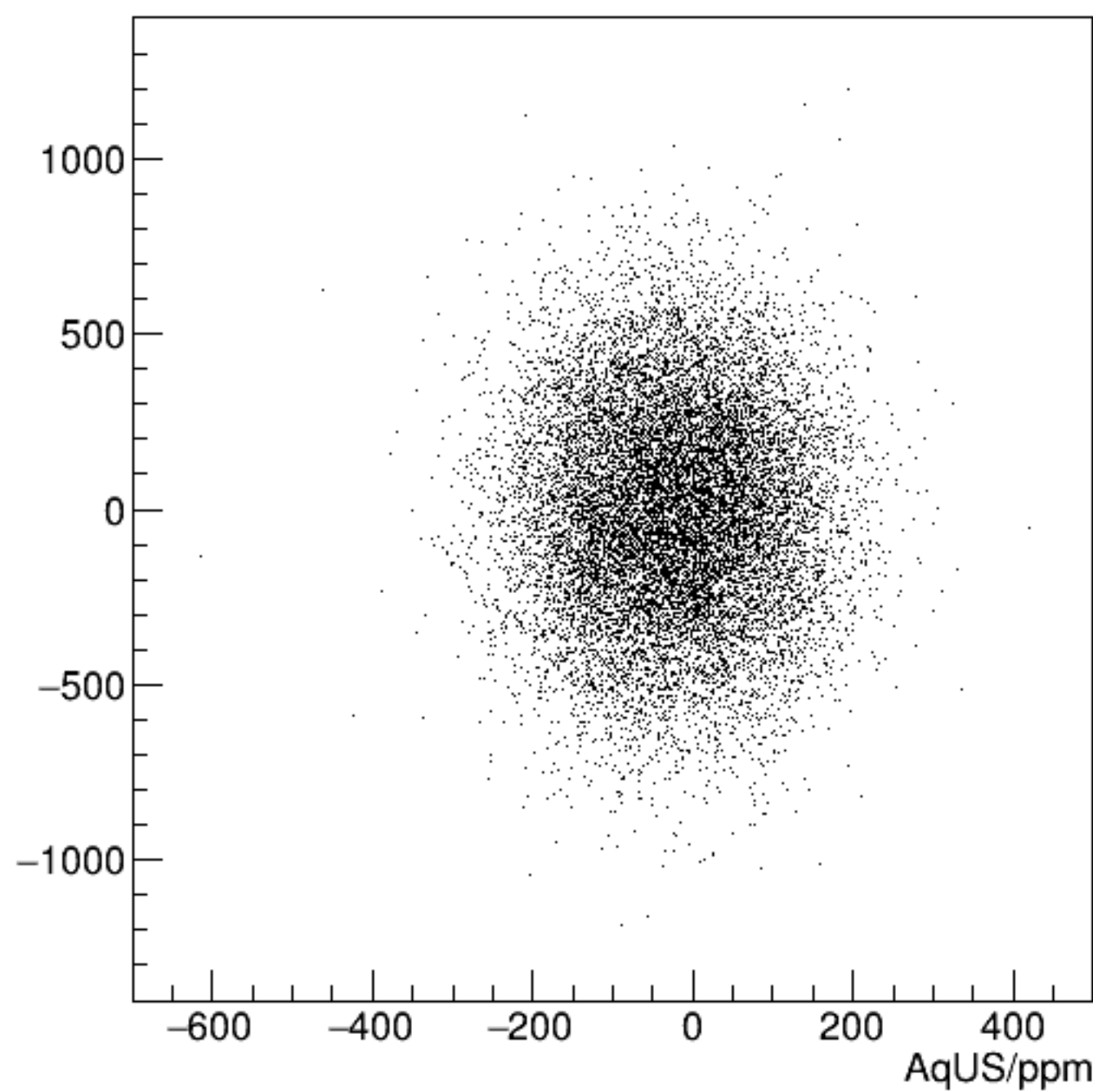
cor_sam1/ppm:AqUS/ppm {ErrorFlag==0}
