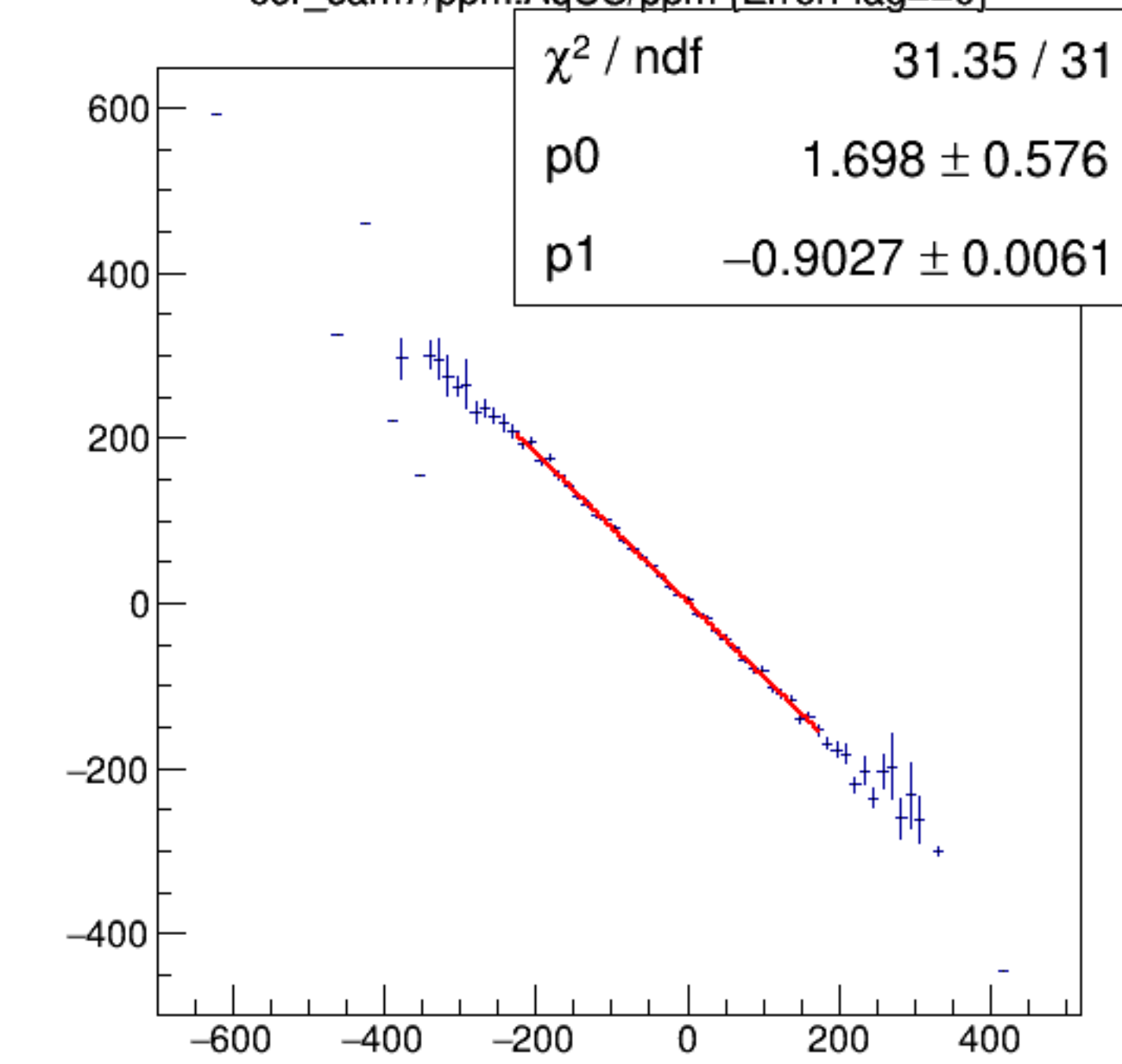
cor_sam7/ppm:AqUS/ppm {ErrorFlag==0}
