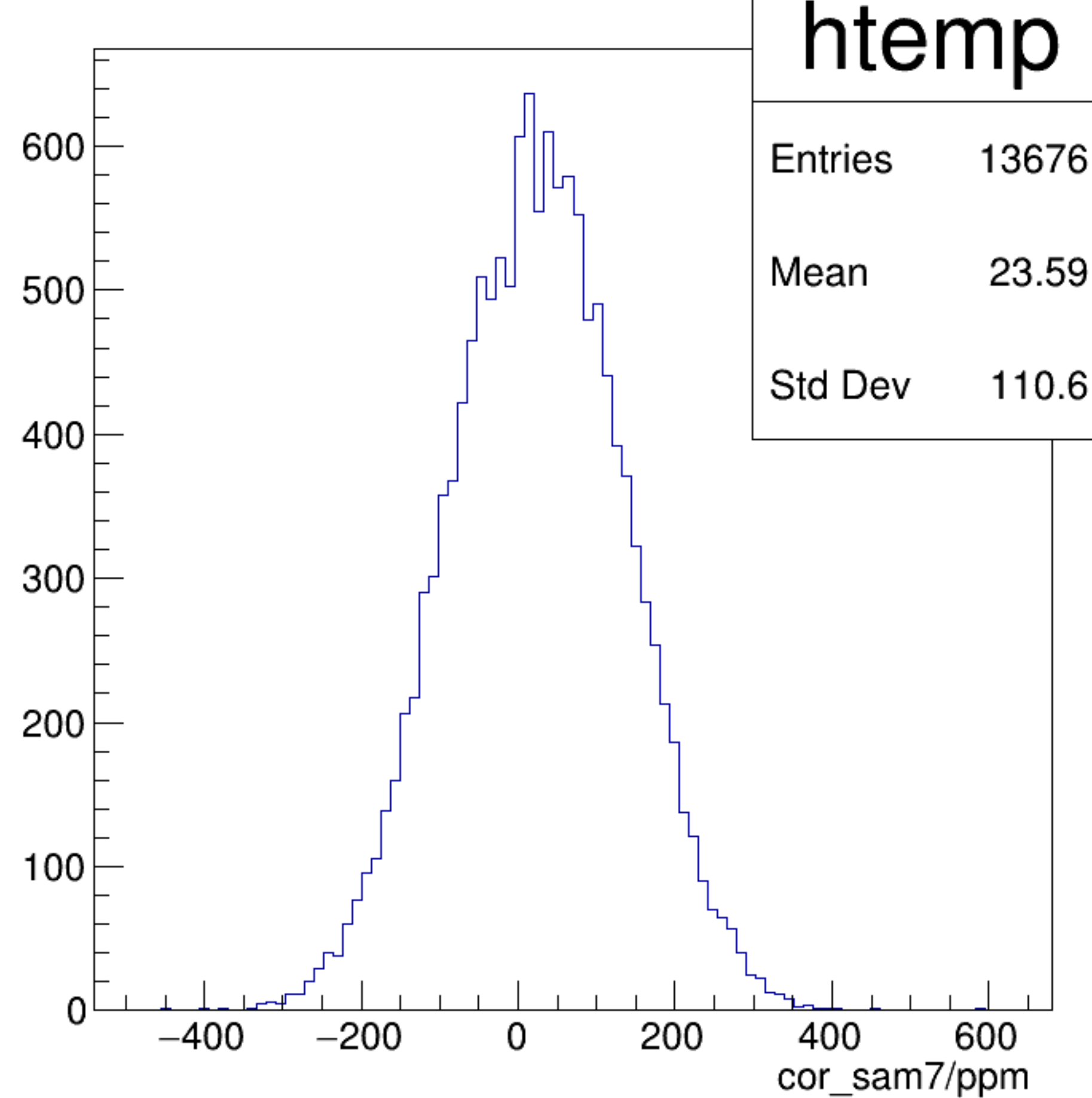
cor_sam7/ppm {ErrorFlag==0}
