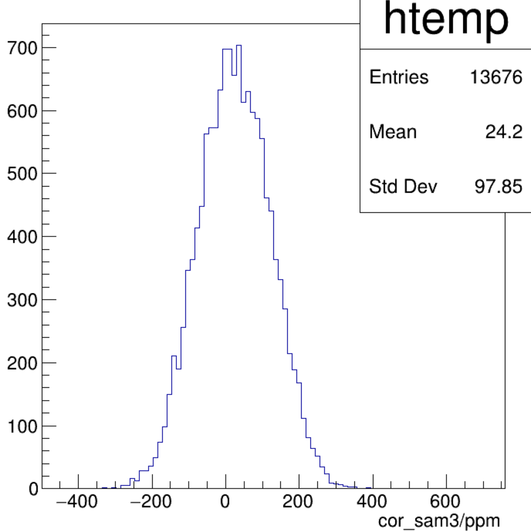
cor_sam3/ppm {ErrorFlag==0}
