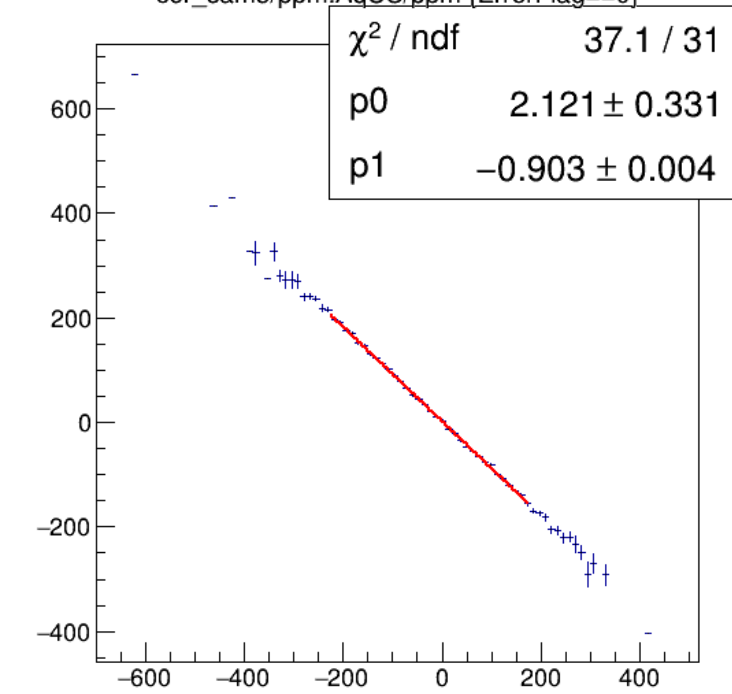
cor_sam3/ppm:AqUS/ppm {ErrorFlag==0}
