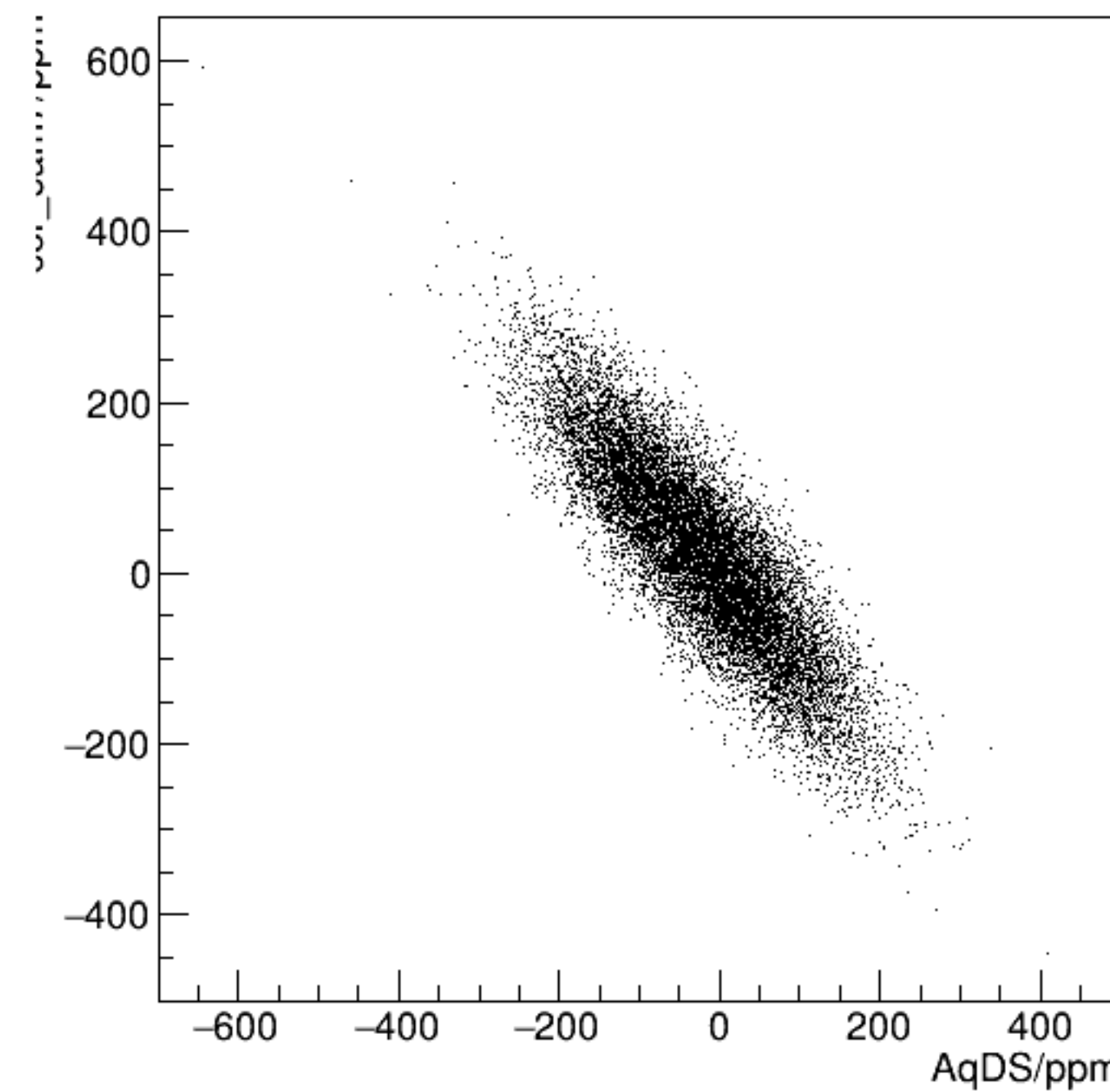
cor_sam7/ppm:AqDS/ppm {ErrorFlag==0}
