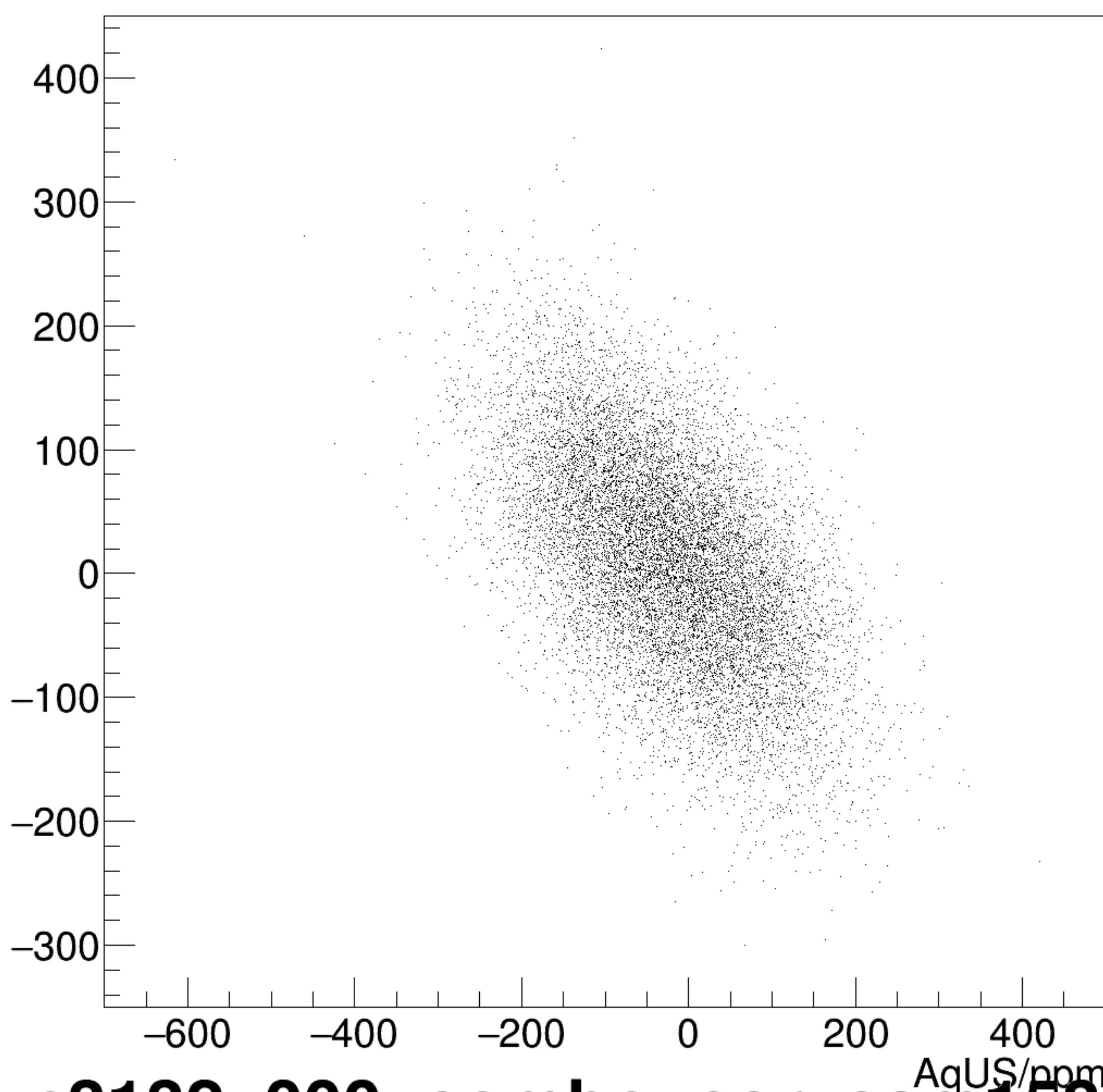
AverageLumi/ppm:AqUS/ppm {ErrorFlag==0}
