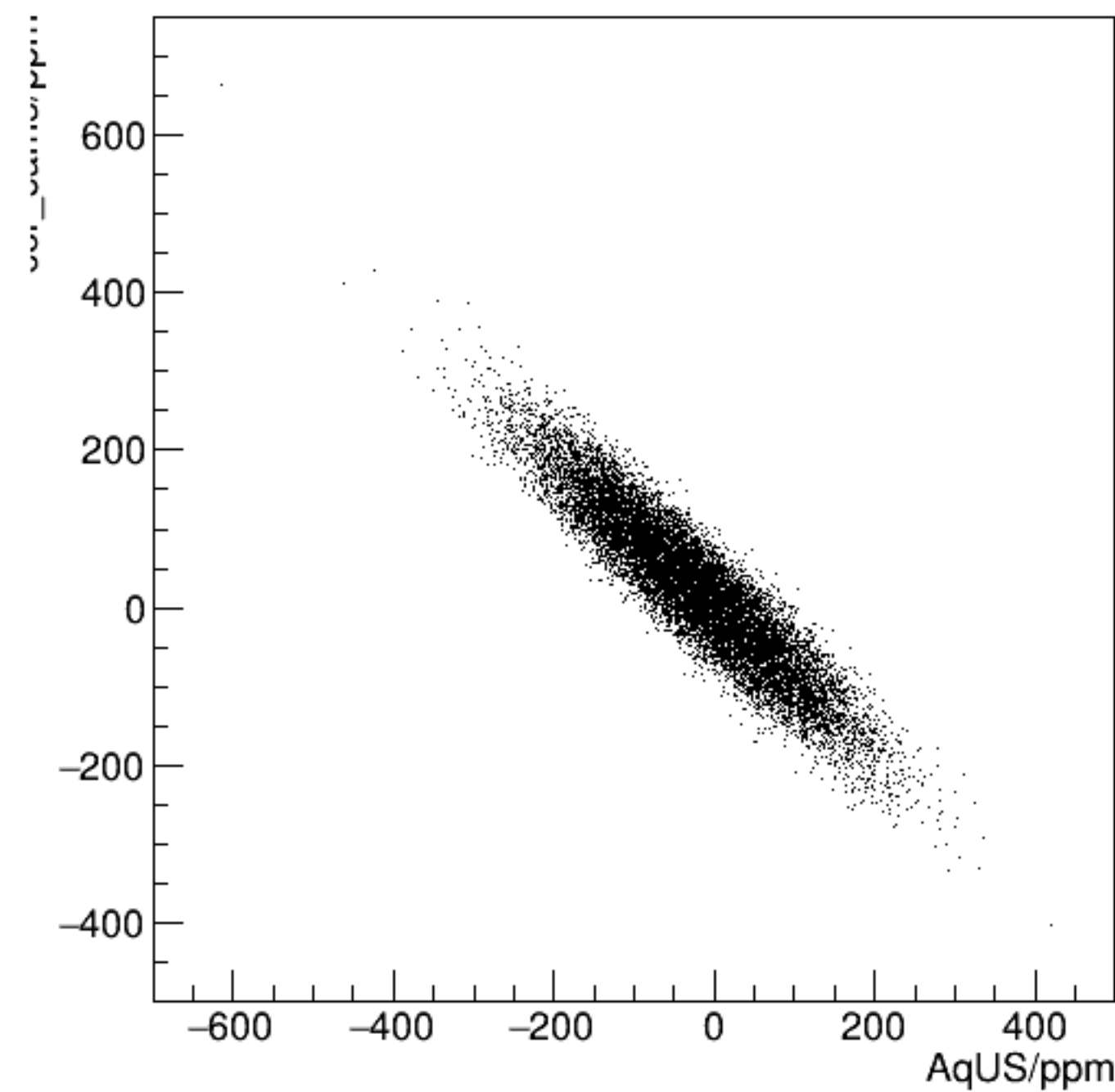
cor_sam3/ppm:AqUS/ppm {ErrorFlag==0}
