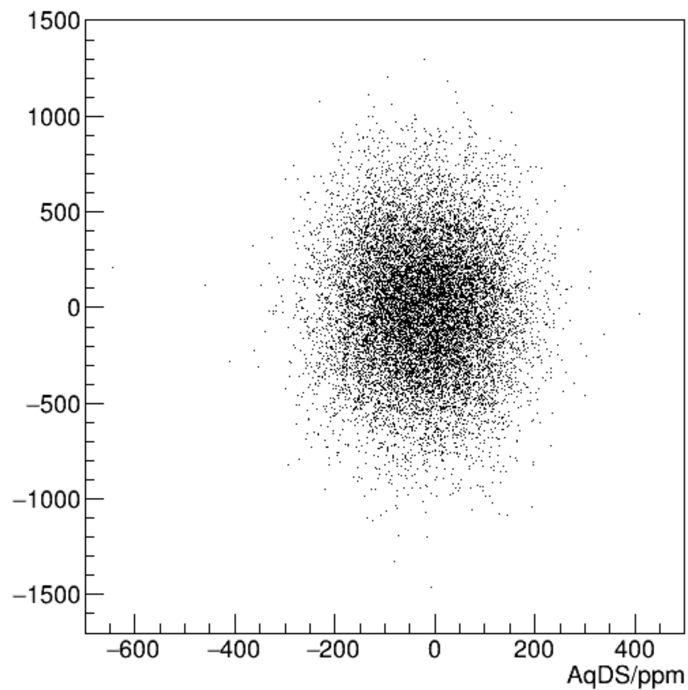
cor_sam5/ppm:AqDS/ppm {ErrorFlag==0}
