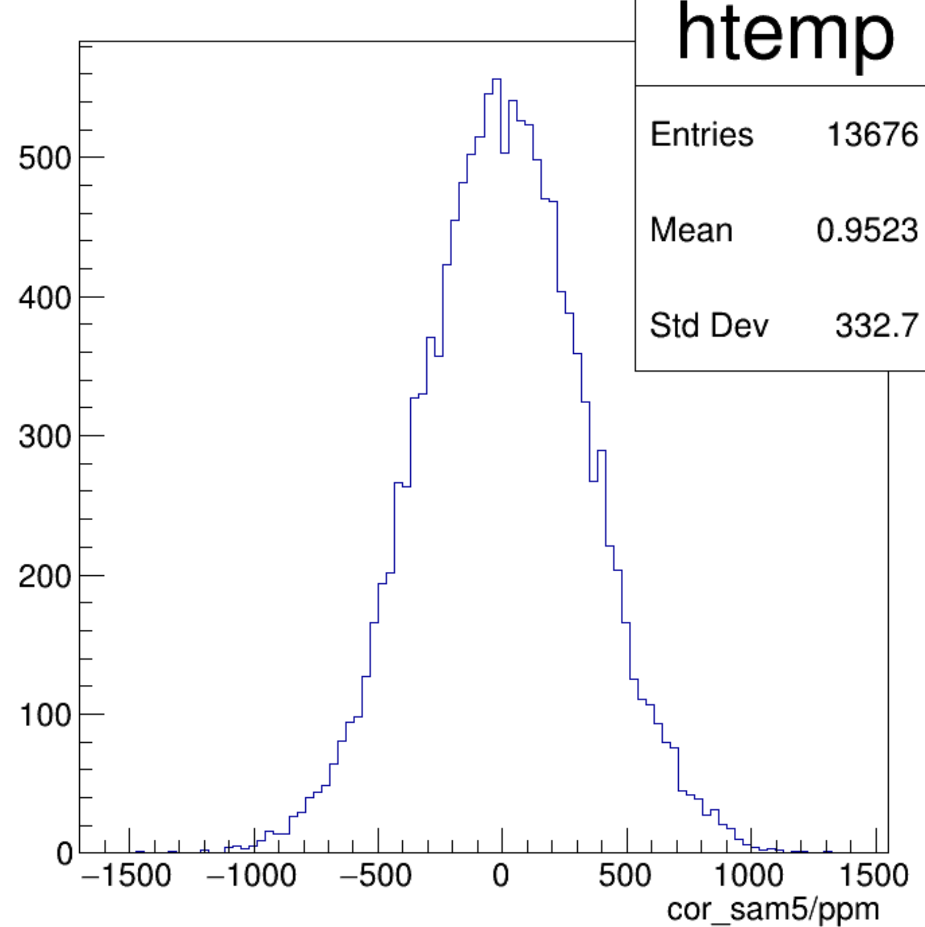
cor_sam5/ppm {ErrorFlag==0}
