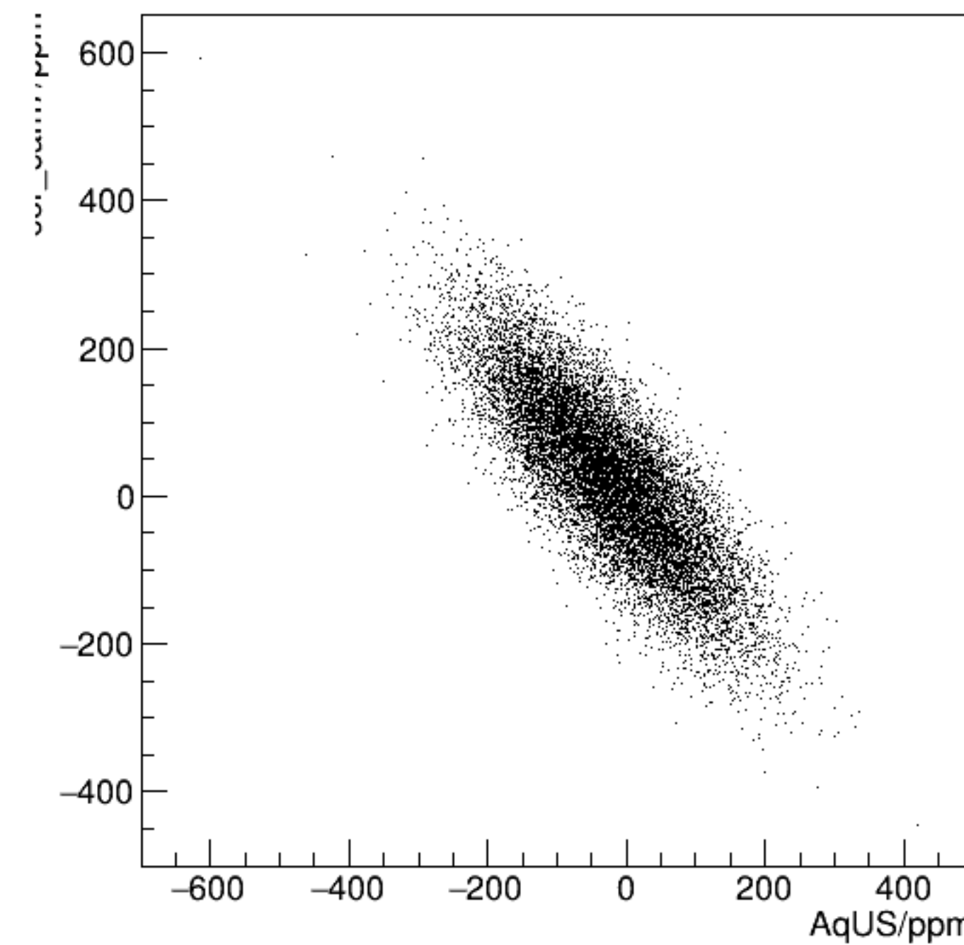
cor_sam7/ppm:AqUS/ppm {ErrorFlag==0}
