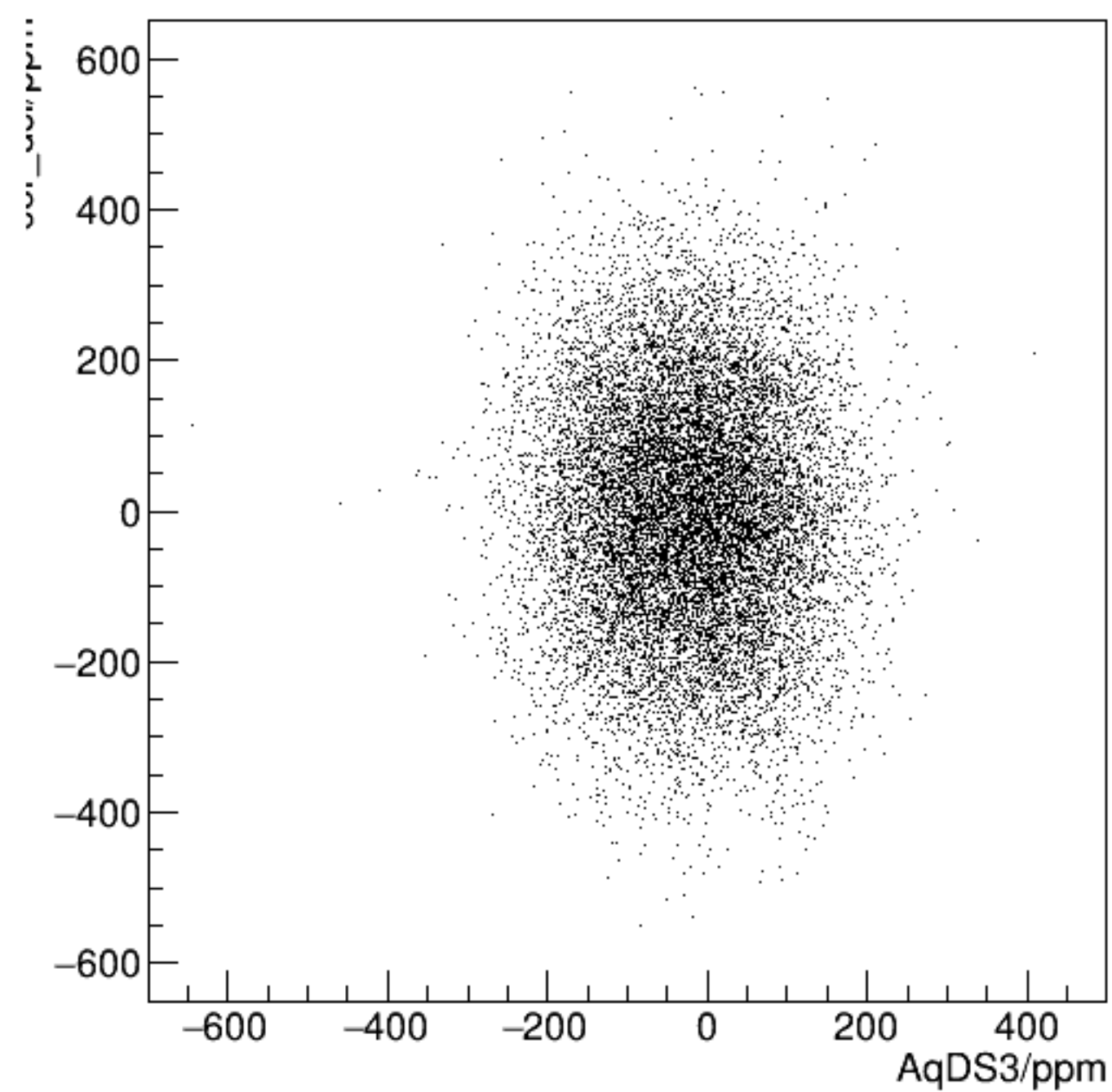
cor_dsl/ppm:AqDS3/ppm {ErrorFlag==0}
