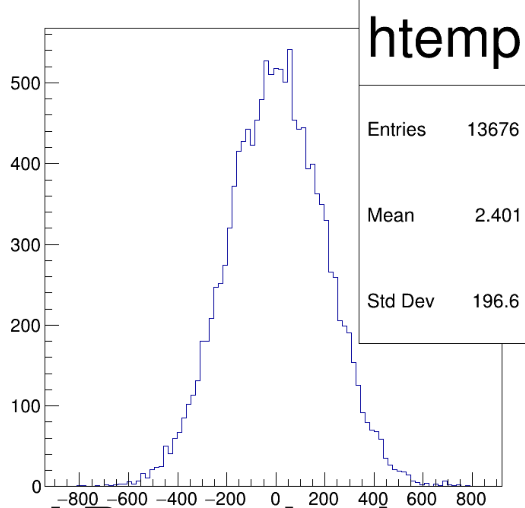
(asym_dsl/ppm+asym_dsr/ppm)/2 {ErrorFlag==0}
