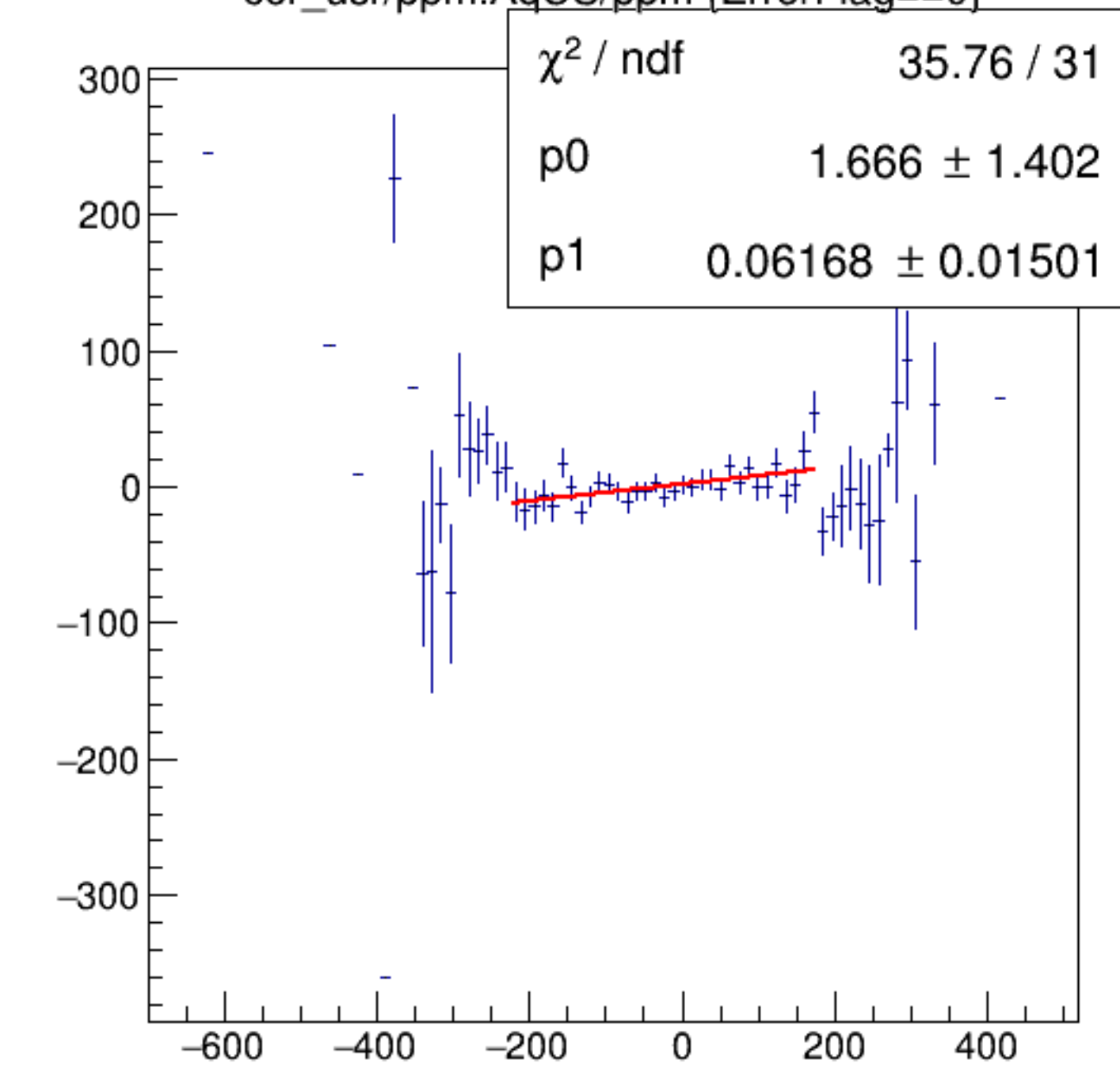
cor_usr/ppm:AqUS/ppm {ErrorFlag==0}
