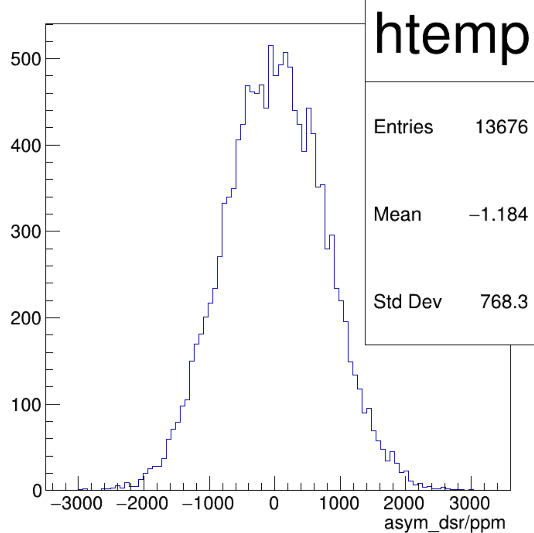
asym_dsr/ppm {ErrorFlag==0}
