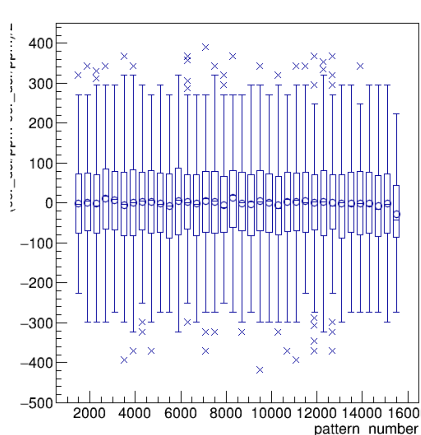
(cor_dsl/ppm+cor_dsr/ppm)/2:pattern_number {ErrorFlag==0}
