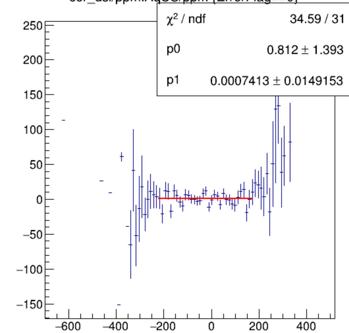
cor_dsl/ppm:AqUS/ppm {ErrorFlag==0}
