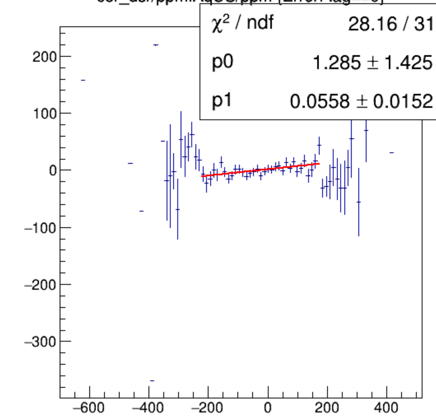
cor_dsr/ppm:AqUS/ppm {ErrorFlag==0}
