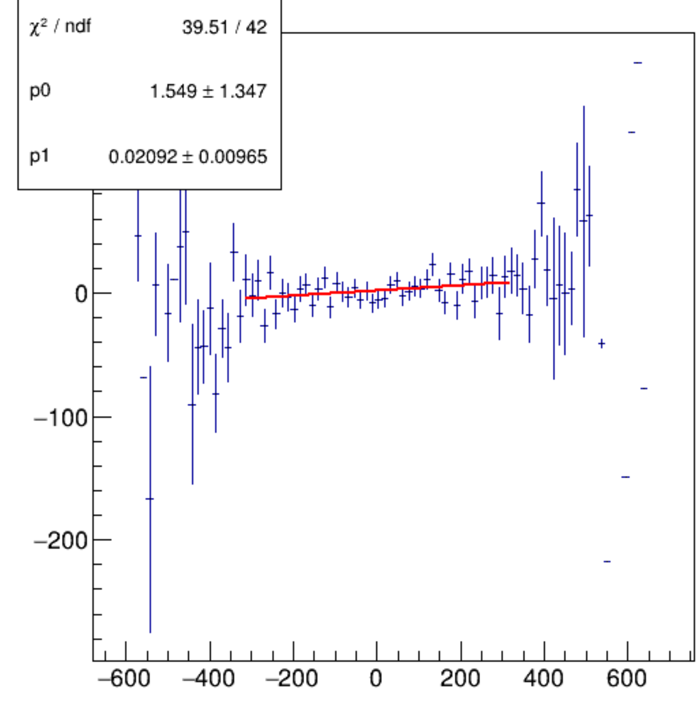
cor_dsl/ppm:cor_dsr/ppm {ErrorFlag==0}
