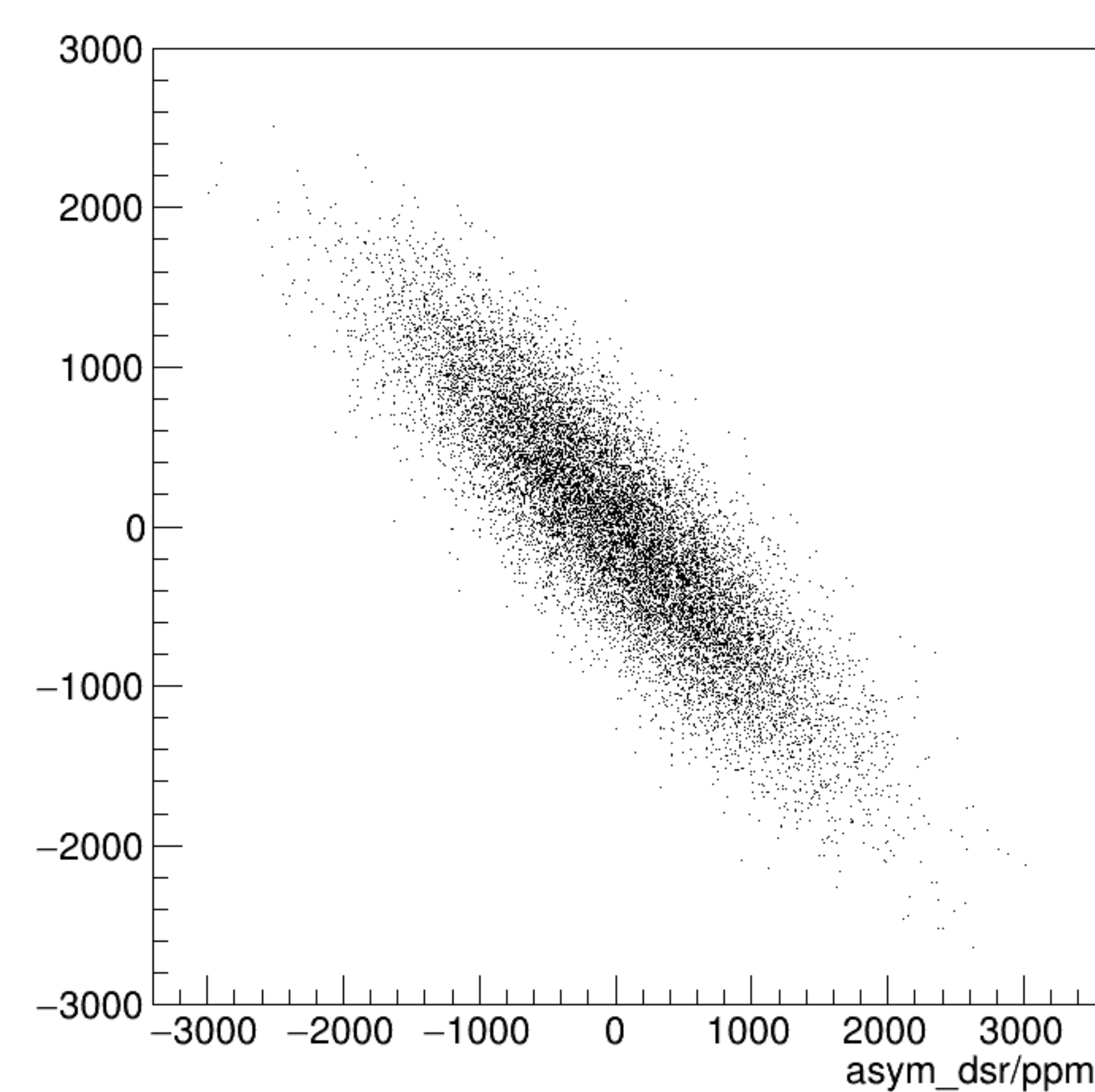
asym_dsl/ppm:asym_dsr/ppm {ErrorFlag==0}
