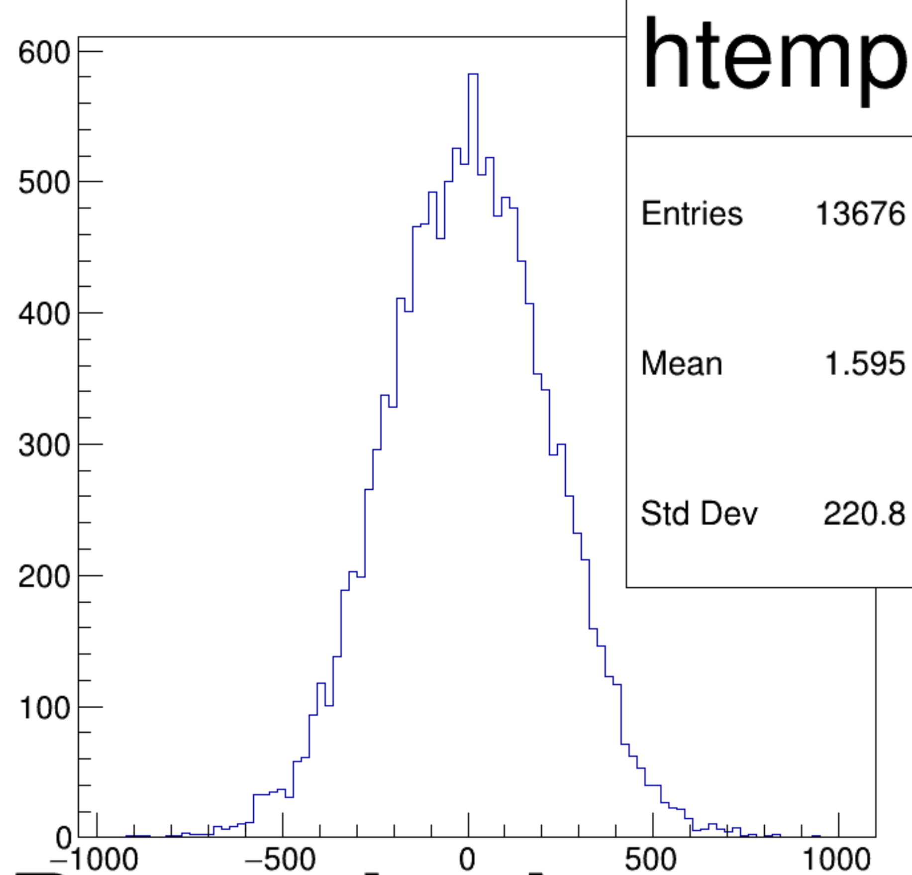
(asym_usr/ppm+asym_usr/ppm)/2 {ErrorFlag==0}
