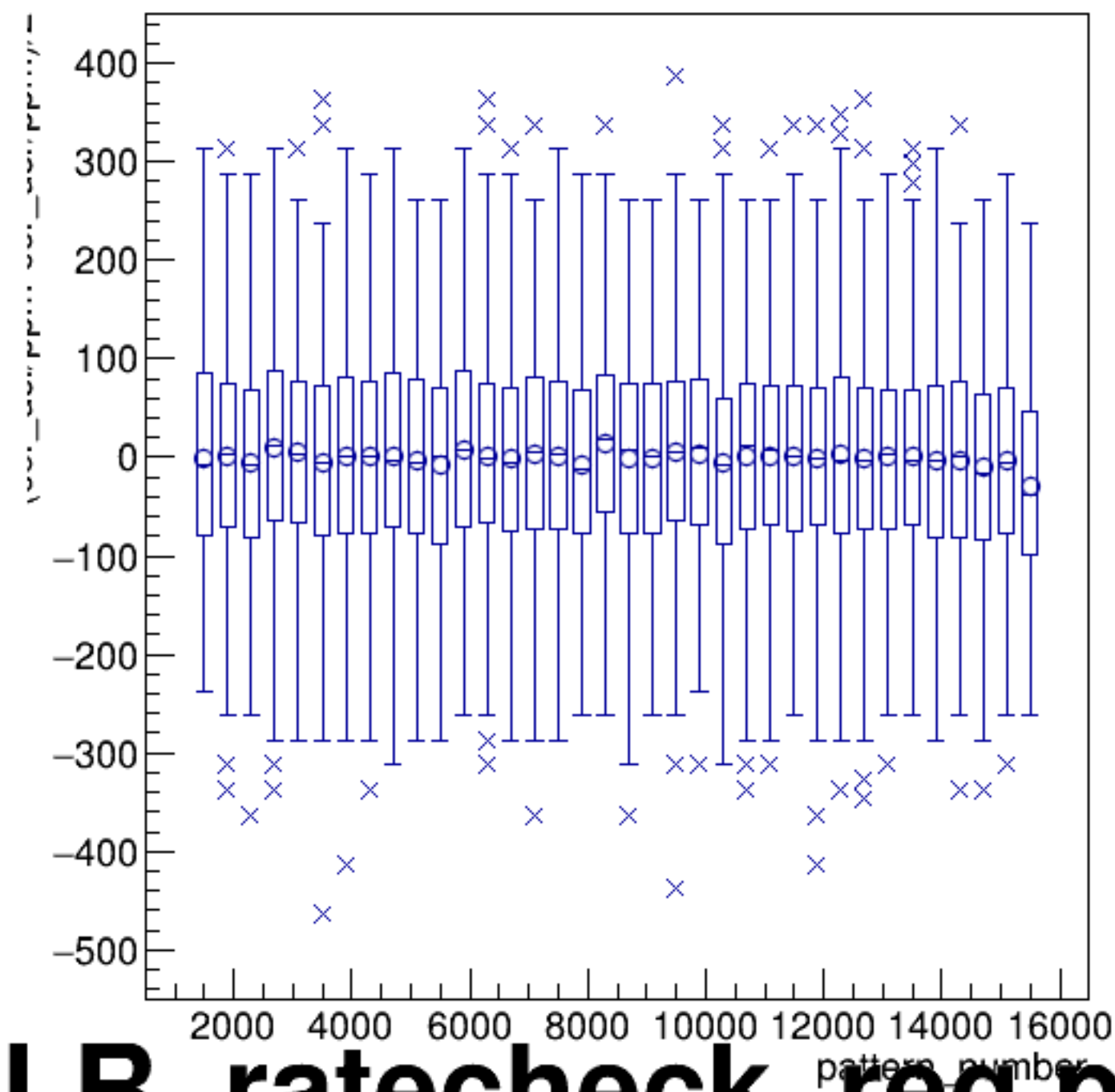
(cor_usl/ppm-cor_usr/ppm)/2:pattern_number {ErrorFlag==0}
