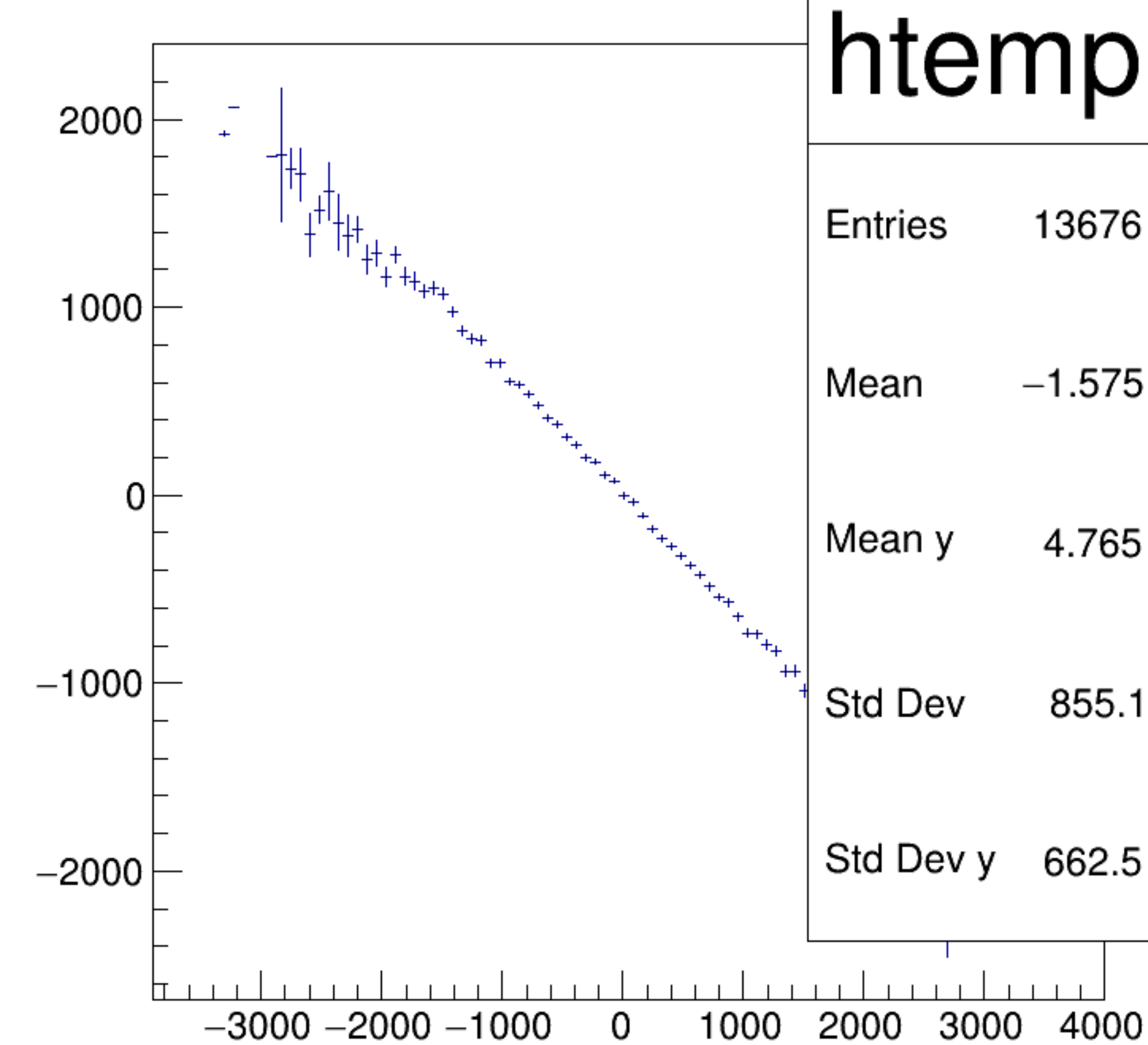
asym_usr/ppm:asym_usr/ppm {ErrorFlag==0}
