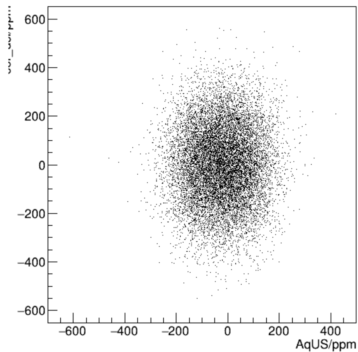
cor_dsl/ppm:AqUS/ppm {ErrorFlag==0}
