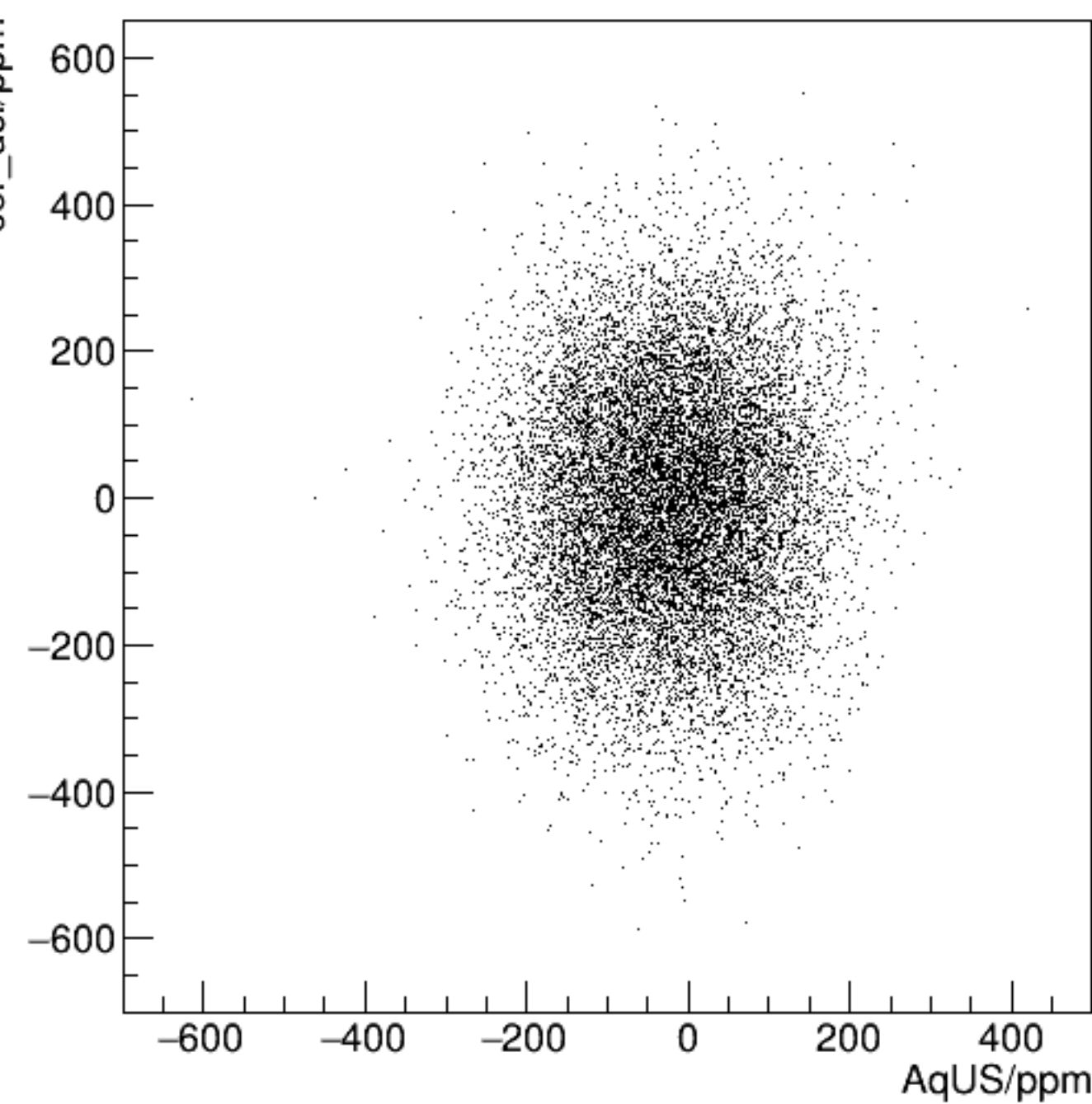
cor_usl/ppm:AqUS/ppm {ErrorFlag==0}
