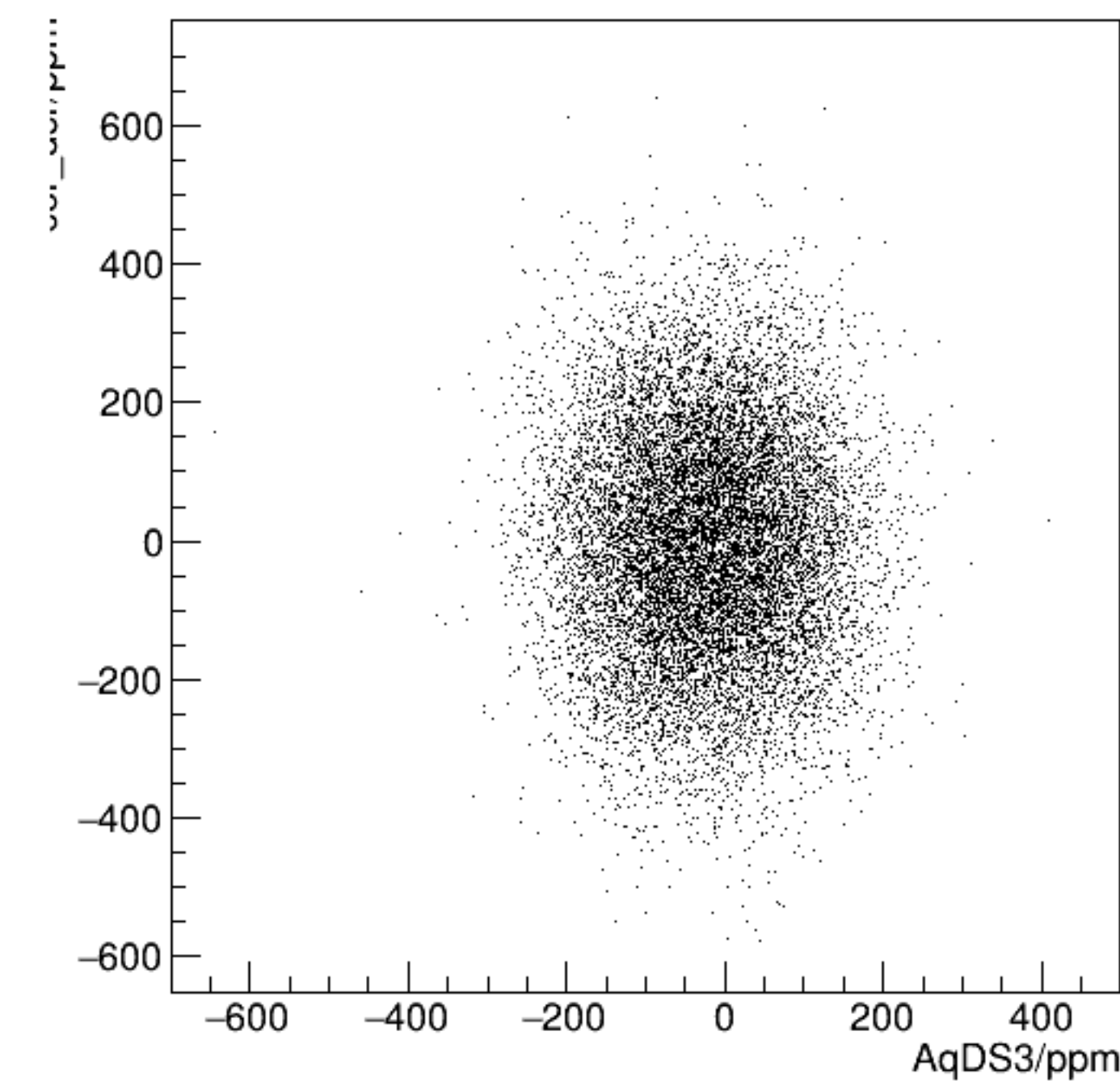
cor_dsr/ppm:AqDS3/ppm {ErrorFlag==0}
