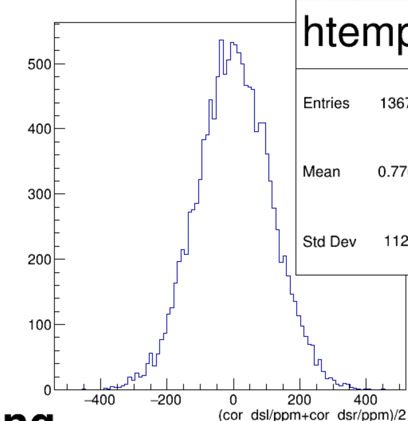
(cor_dsl/ppm+cor_dsr/ppm)/2 {ErrorFlag==0}
