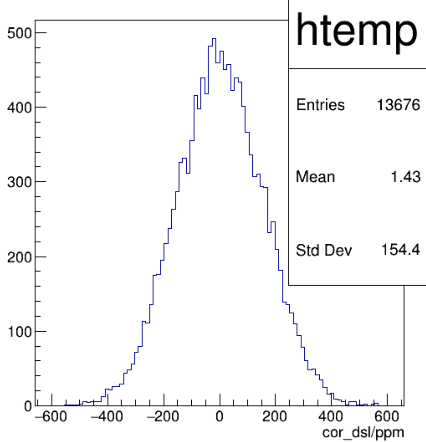
cor_dsl/ppm {ErrorFlag==0}
