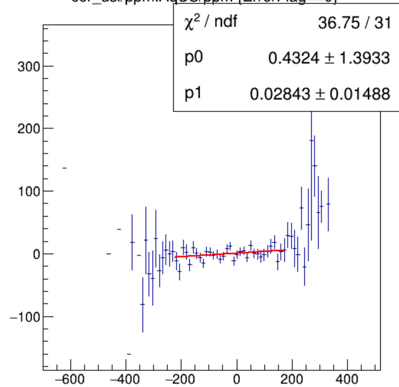
cor_usl/ppm:AqUS/ppm {ErrorFlag==0}
