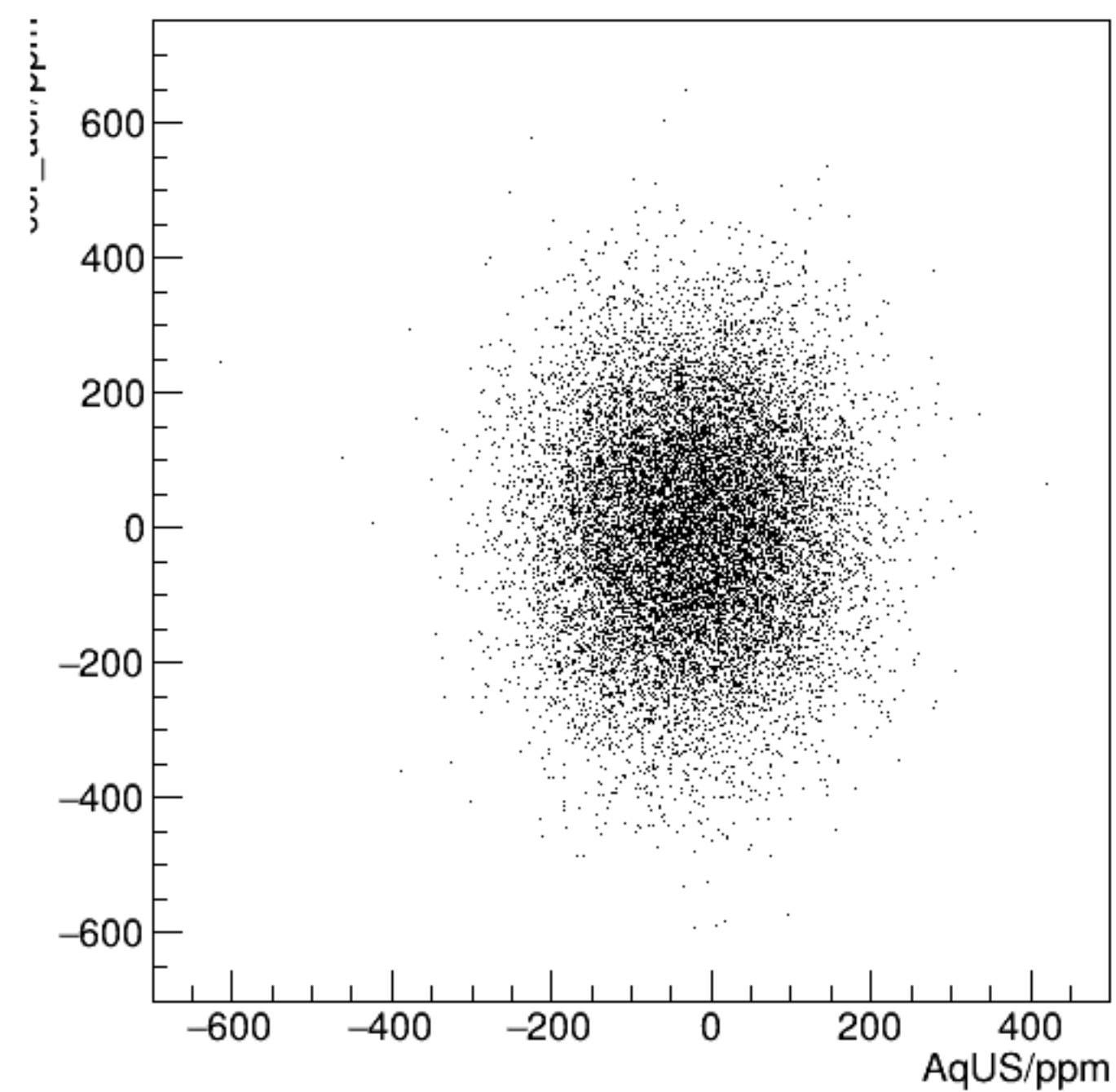
cor_usr/ppm:AqUS/ppm {ErrorFlag==0}
