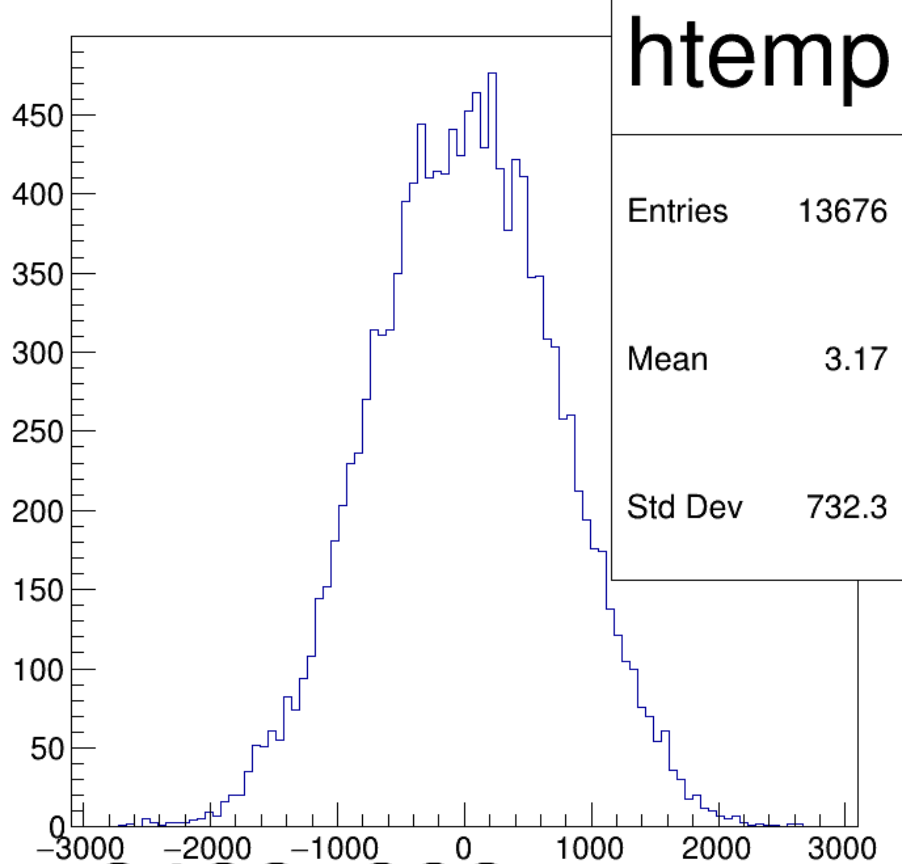
(asym_usr/ppm-asym_usr/ppm)/2 {ErrorFlag==0}
