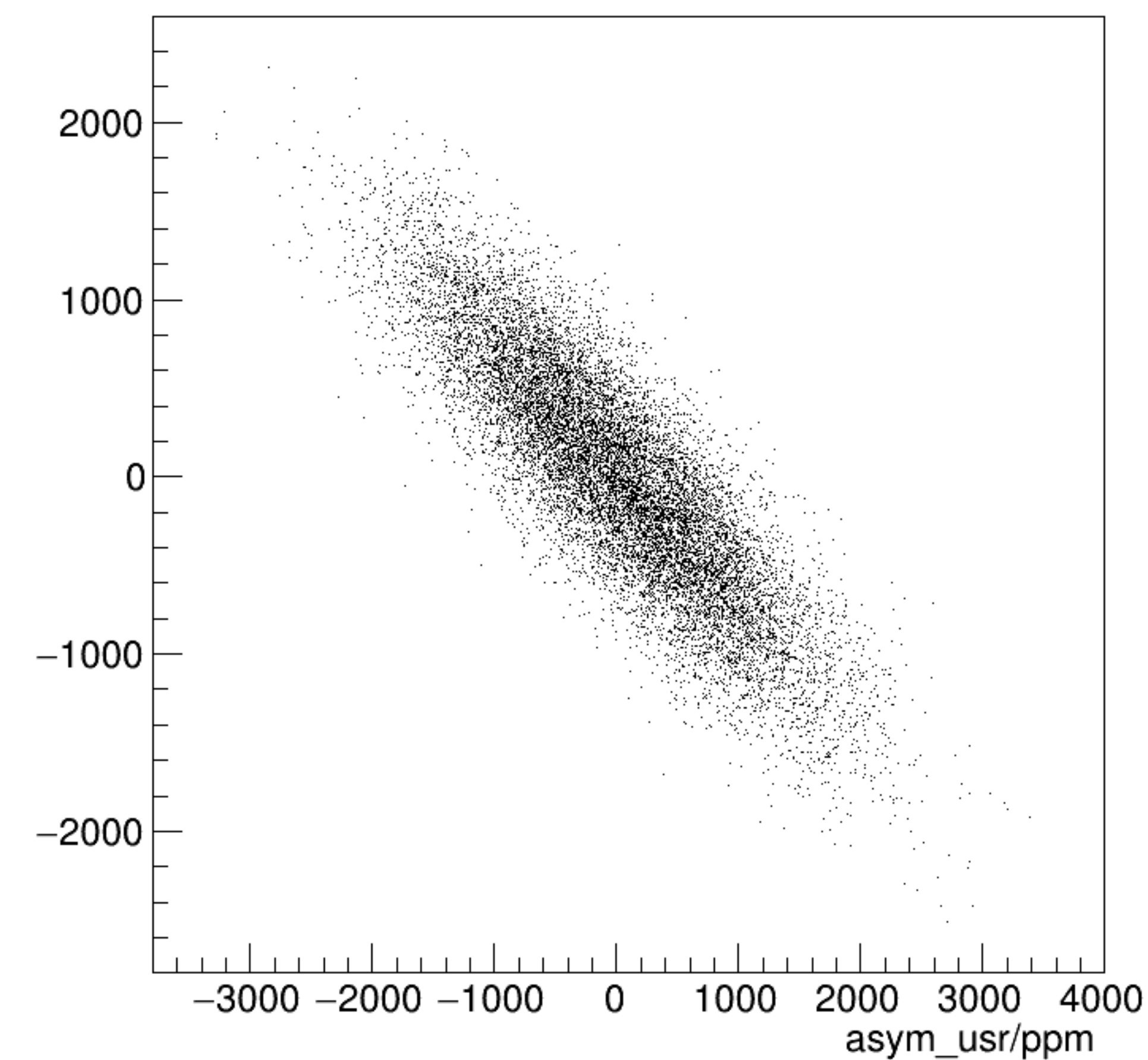
asym_usr/ppm:asym_usr/ppm {ErrorFlag==0}
