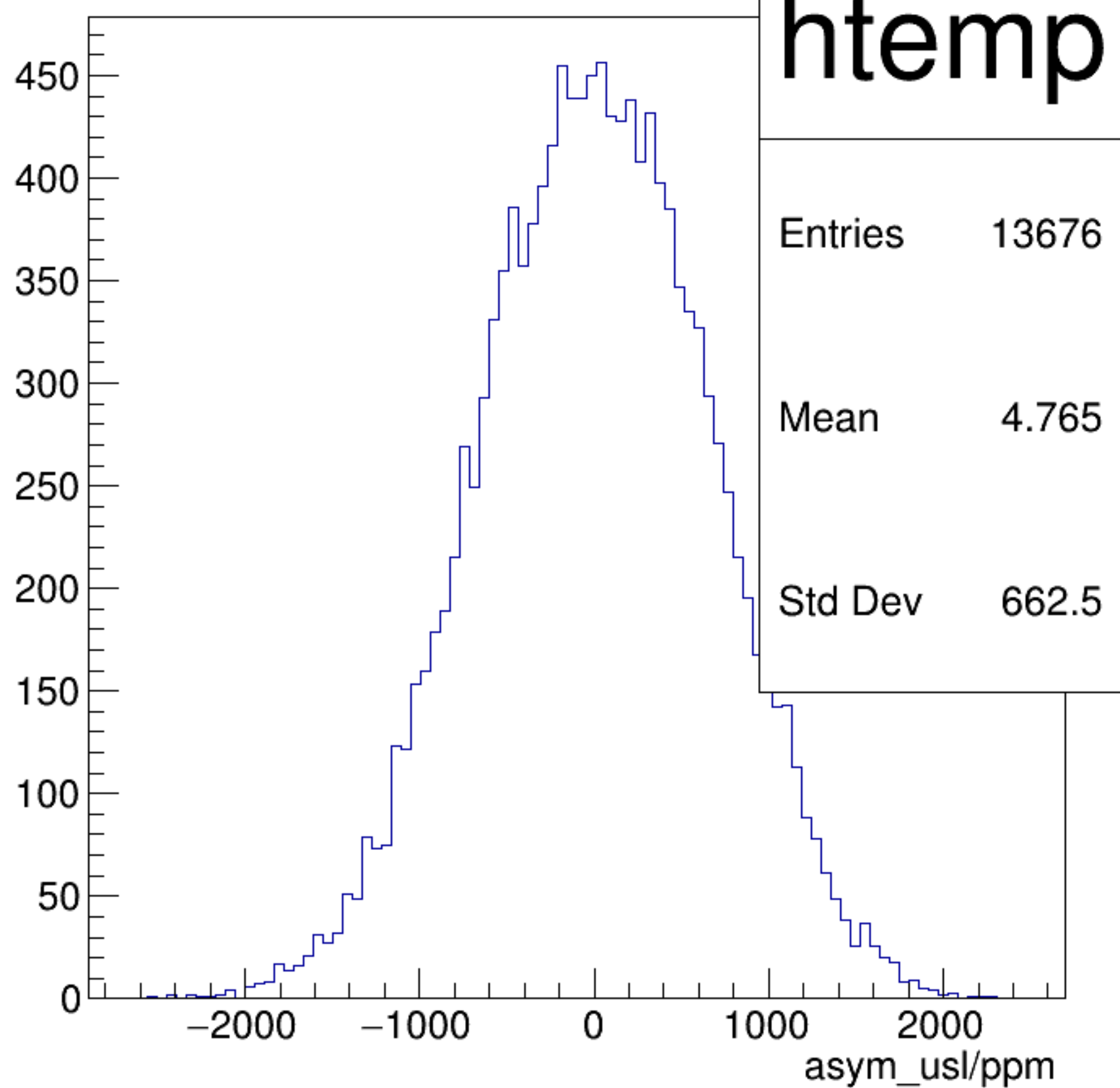
asym_usr/ppm {ErrorFlag==0}
