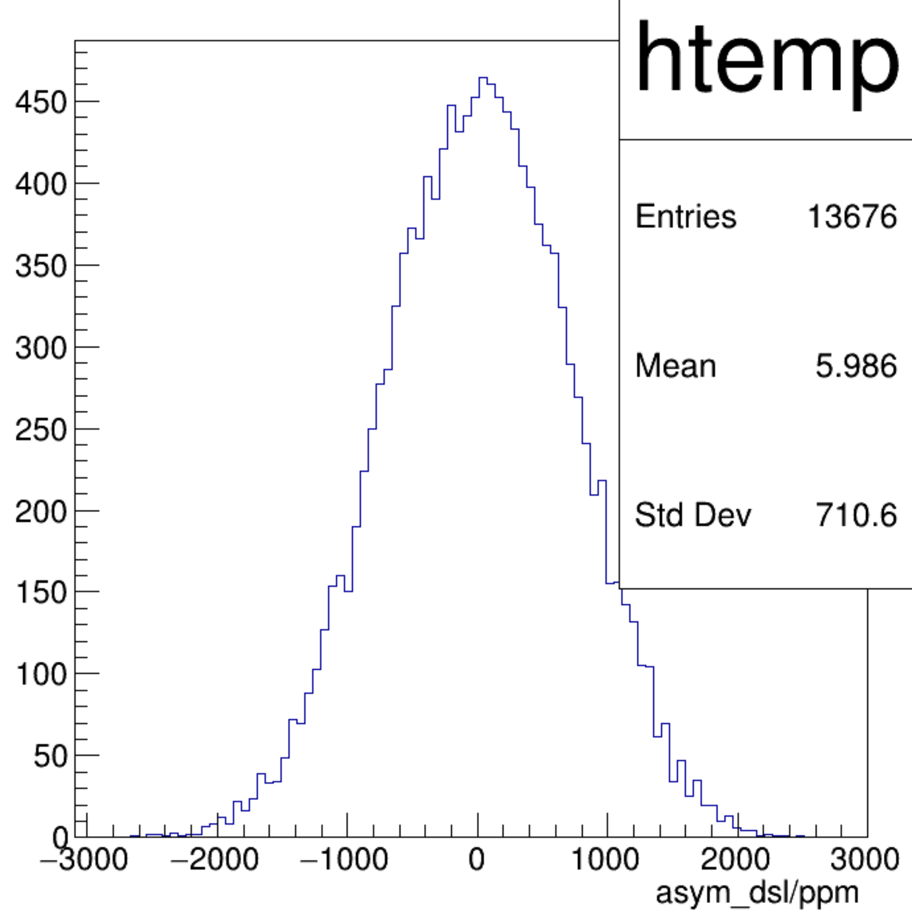
asym_dsl/ppm {ErrorFlag==0}
