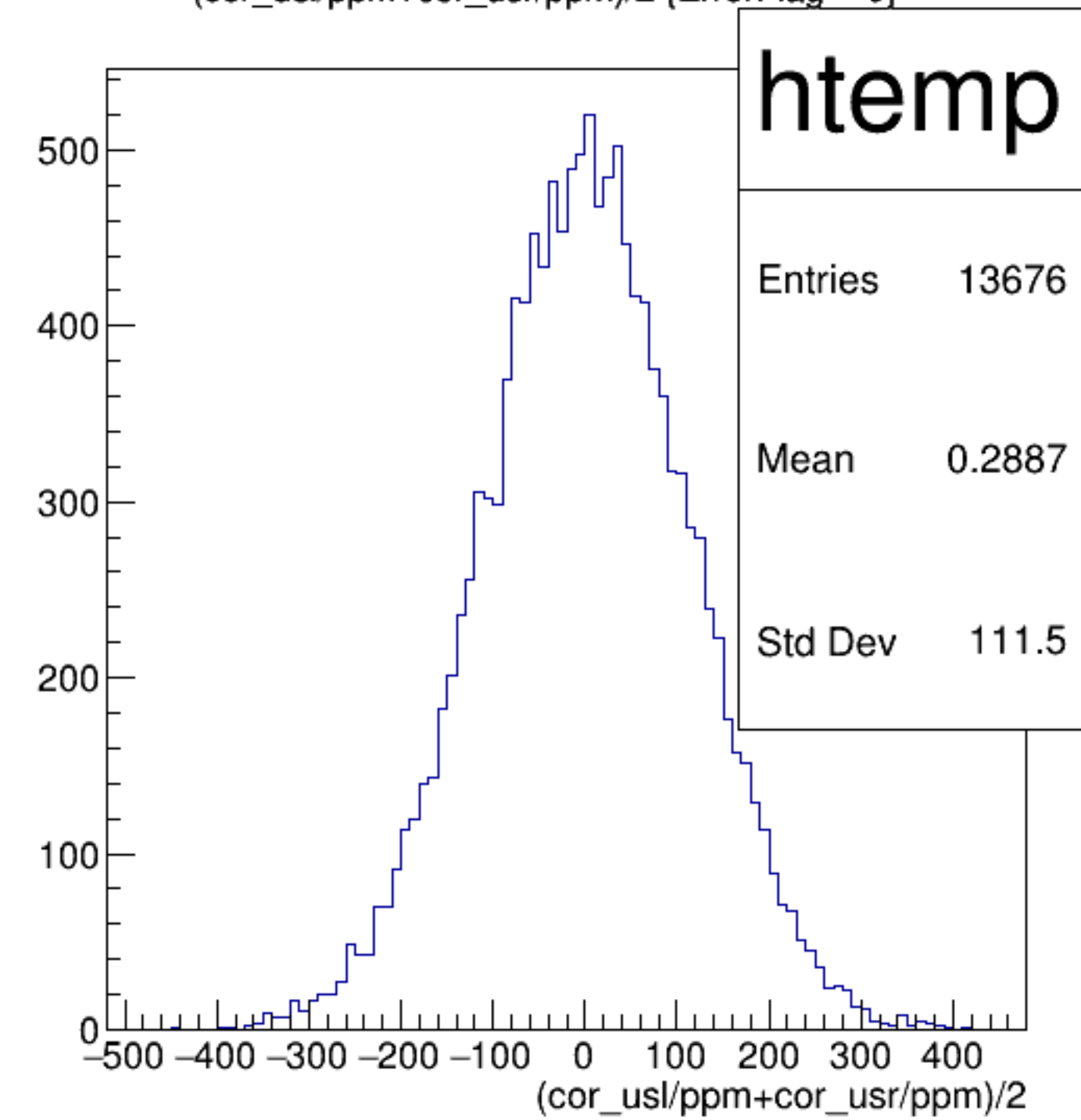
(cor_usl/ppm+cor_usr/ppm)/2 {ErrorFlag==0}
