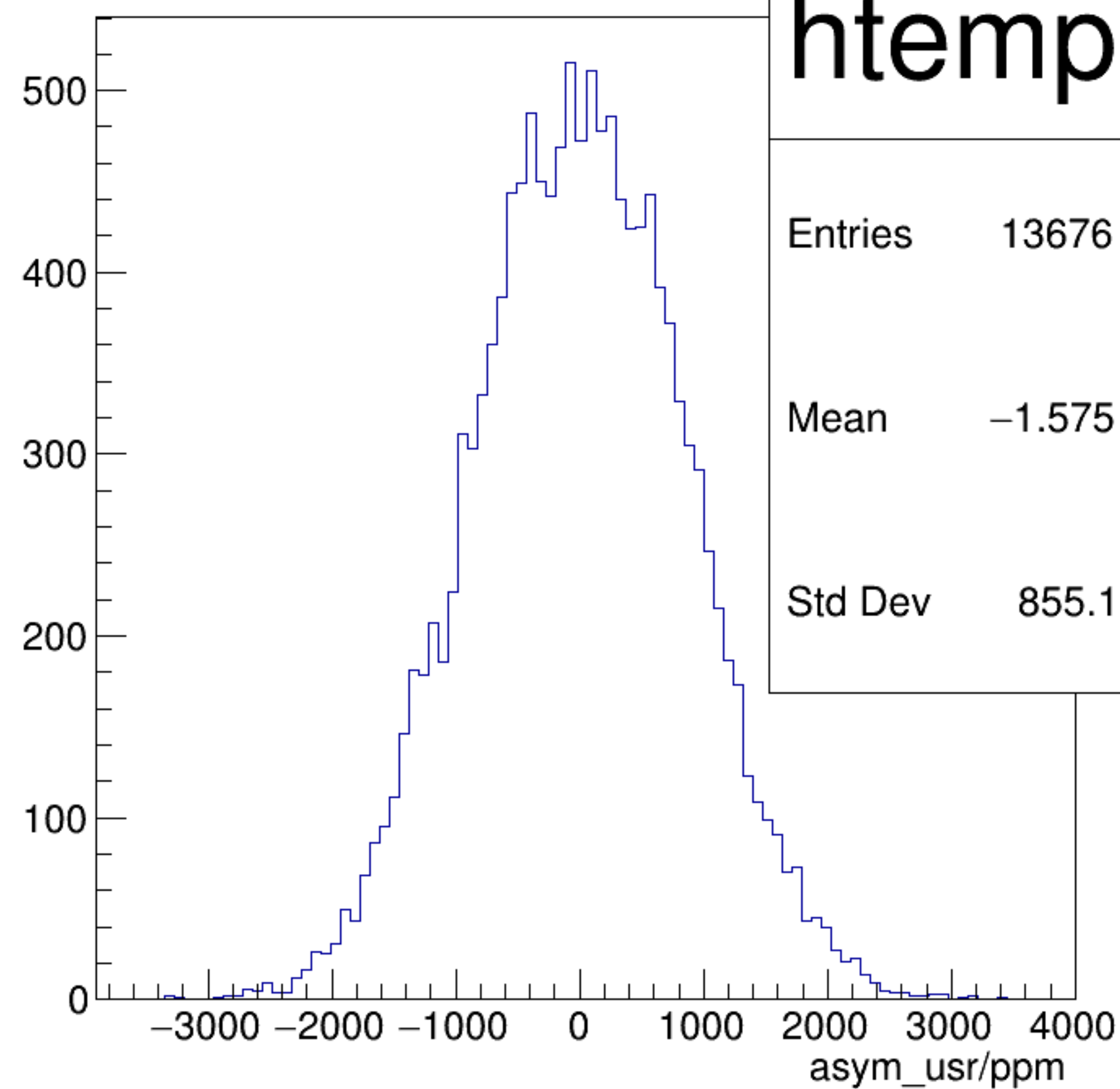
asym_usr/ppm {ErrorFlag==0}
