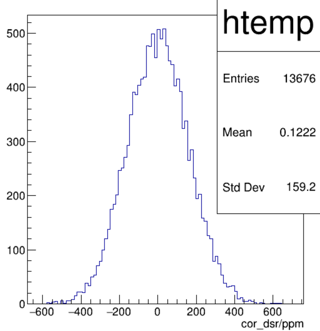
cor_dsr/ppm {ErrorFlag==0}
