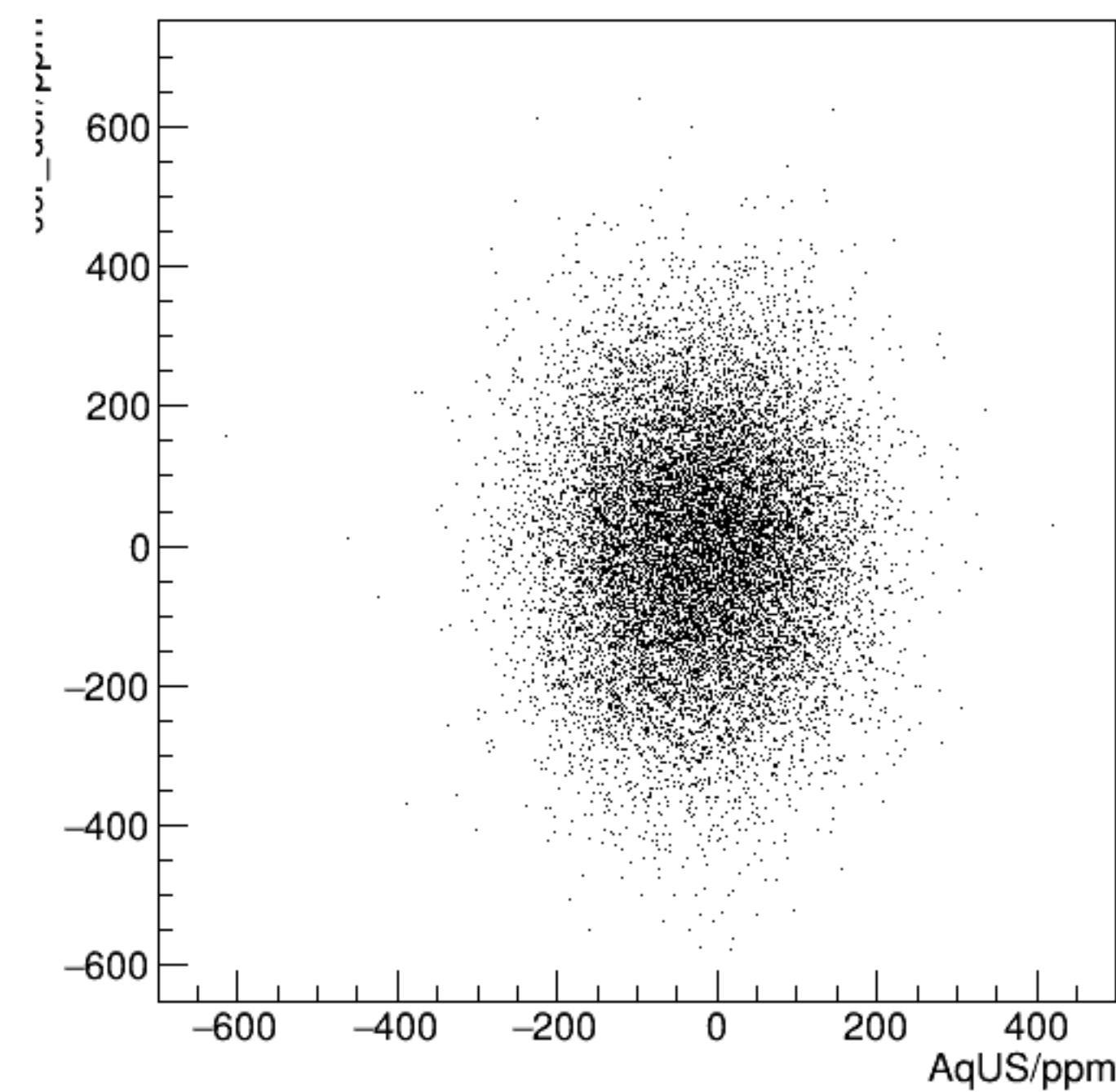
cor_dsr/ppm:AqUS/ppm {ErrorFlag==0}
