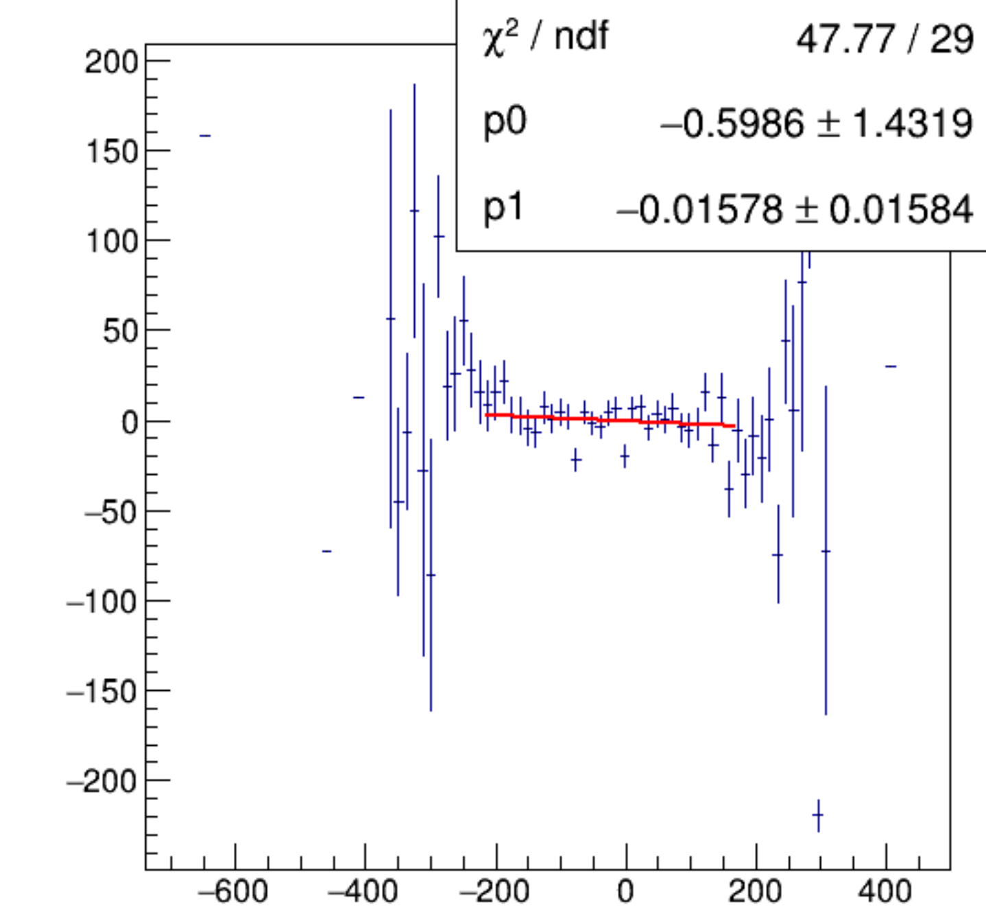
cor_dsr/ppm:AqDS3/ppm {ErrorFlag==0}
