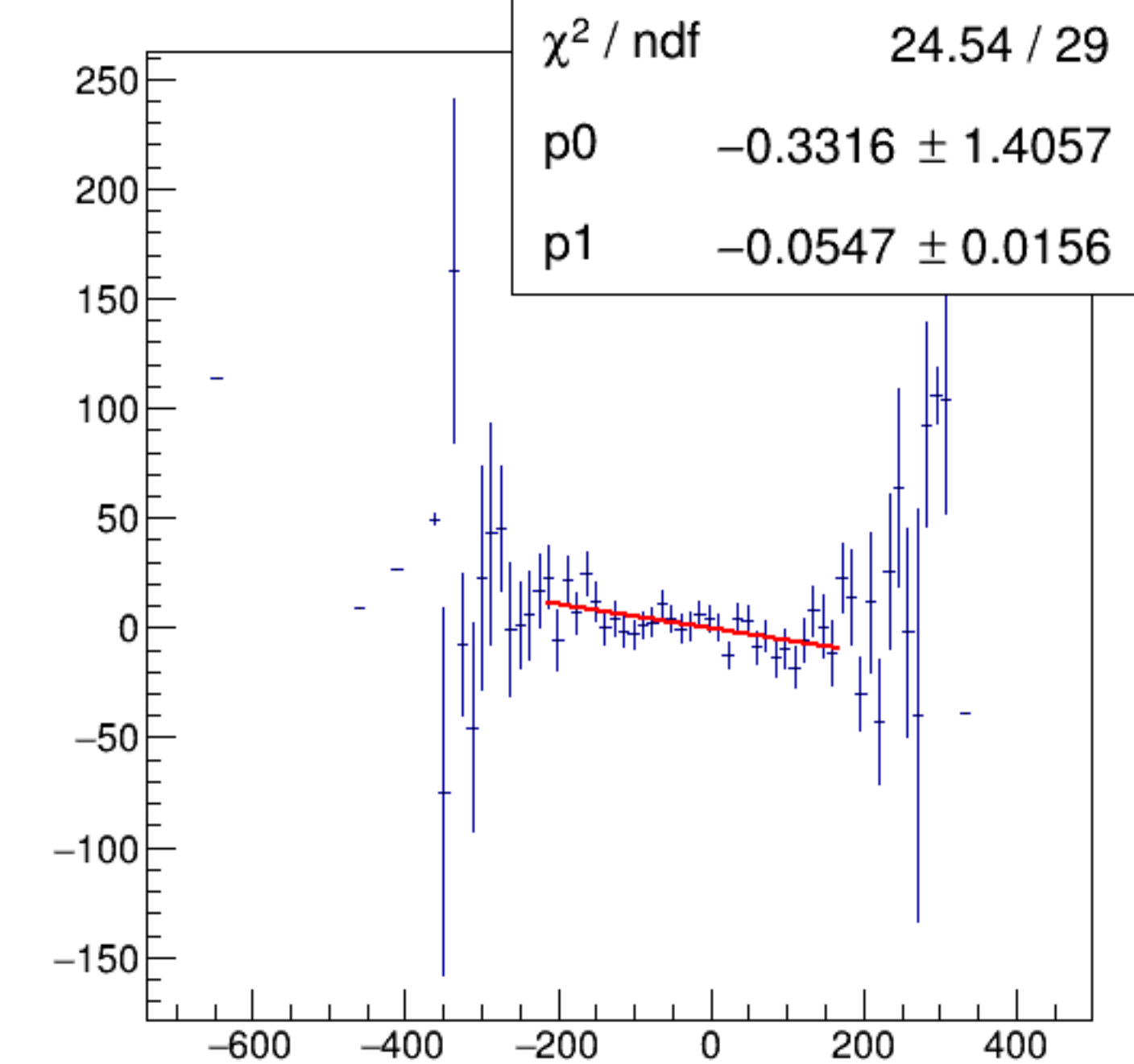
cor_dsl/ppm:AqDS3/ppm {ErrorFlag==0}
