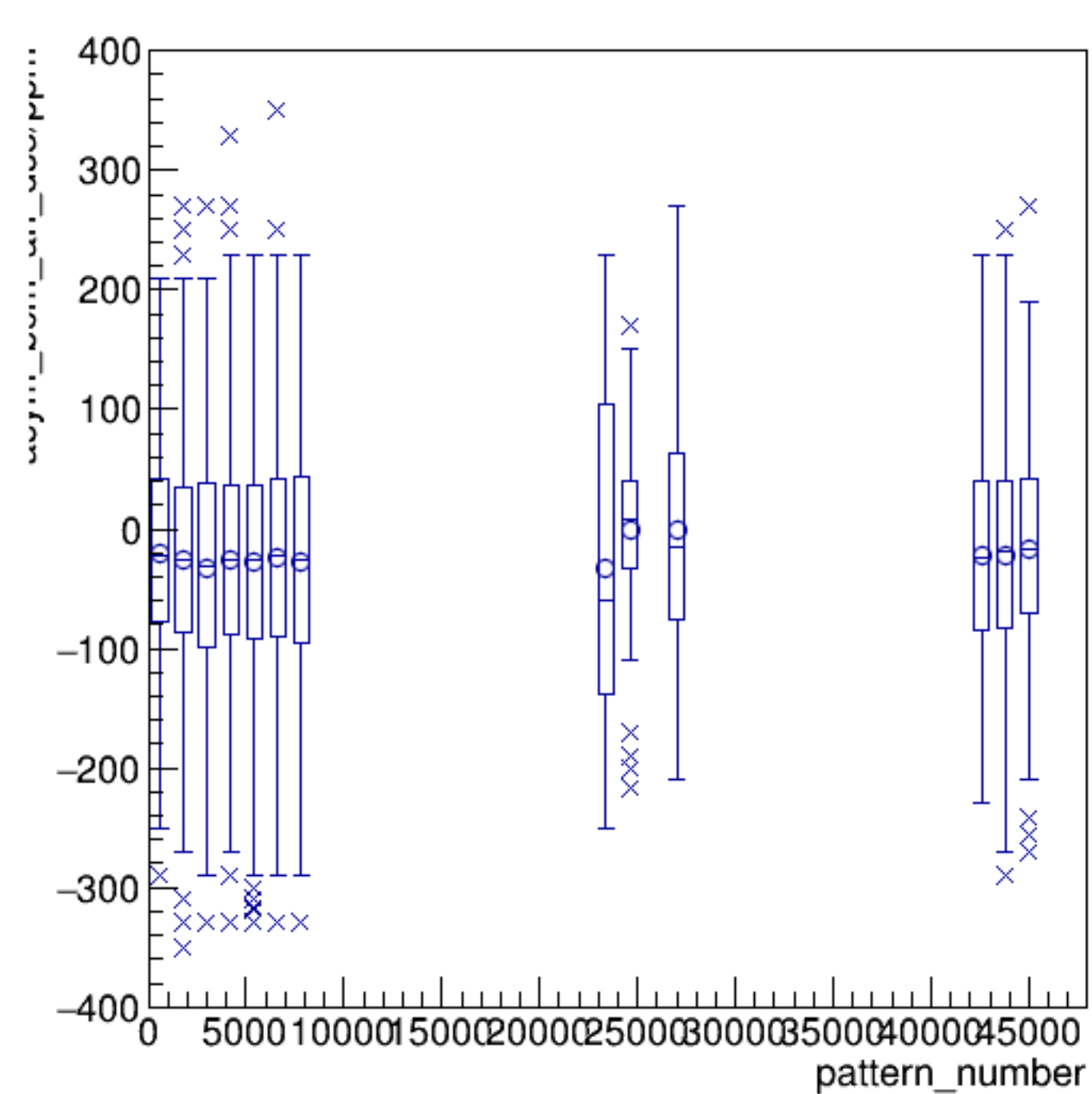
asym_bcm_an_ds3/ppm:pattern_number {ErrorFlag==0}
