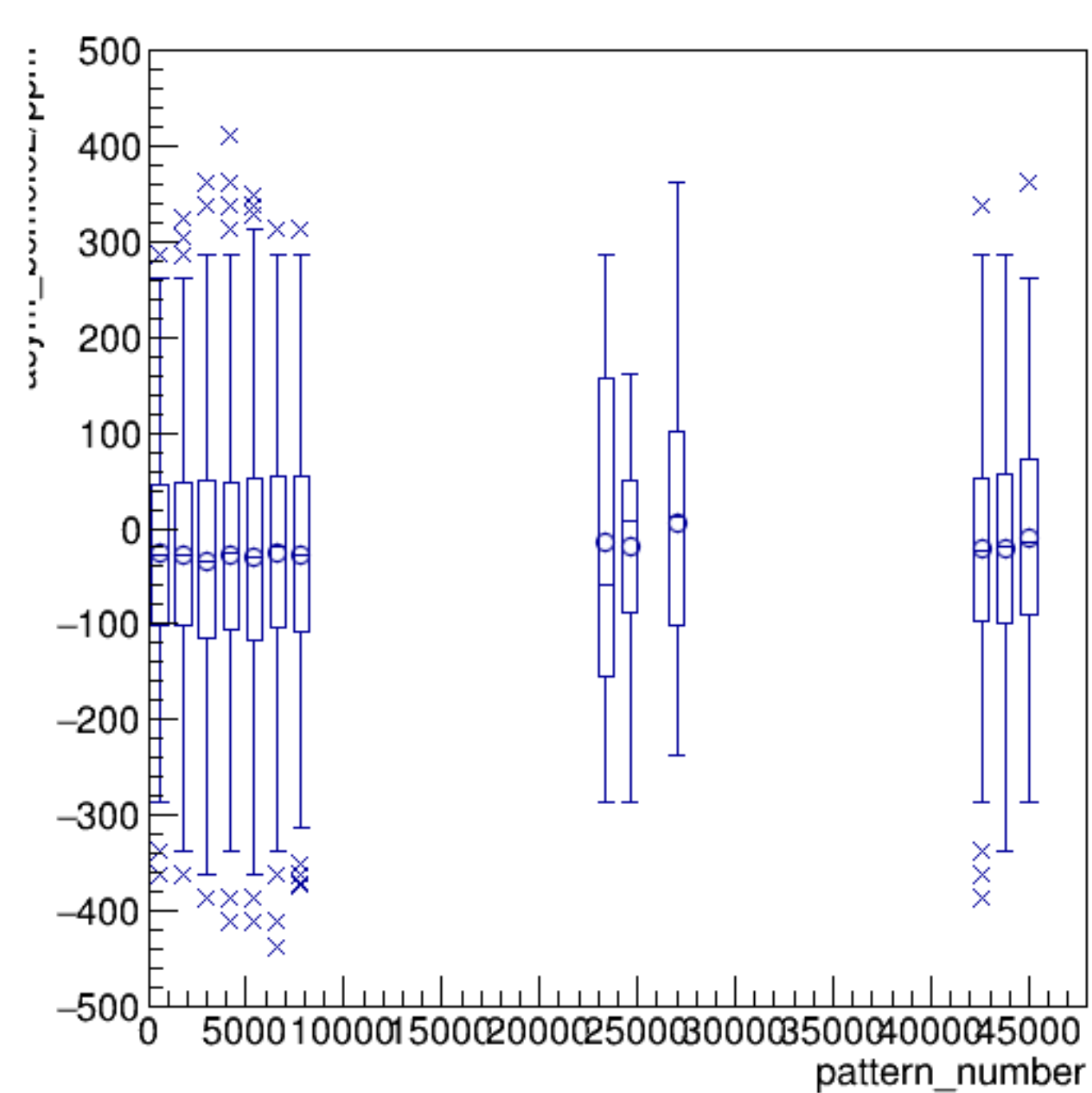
asym_bcm0l02/ppm:pattern_number {ErrorFlag==0}
