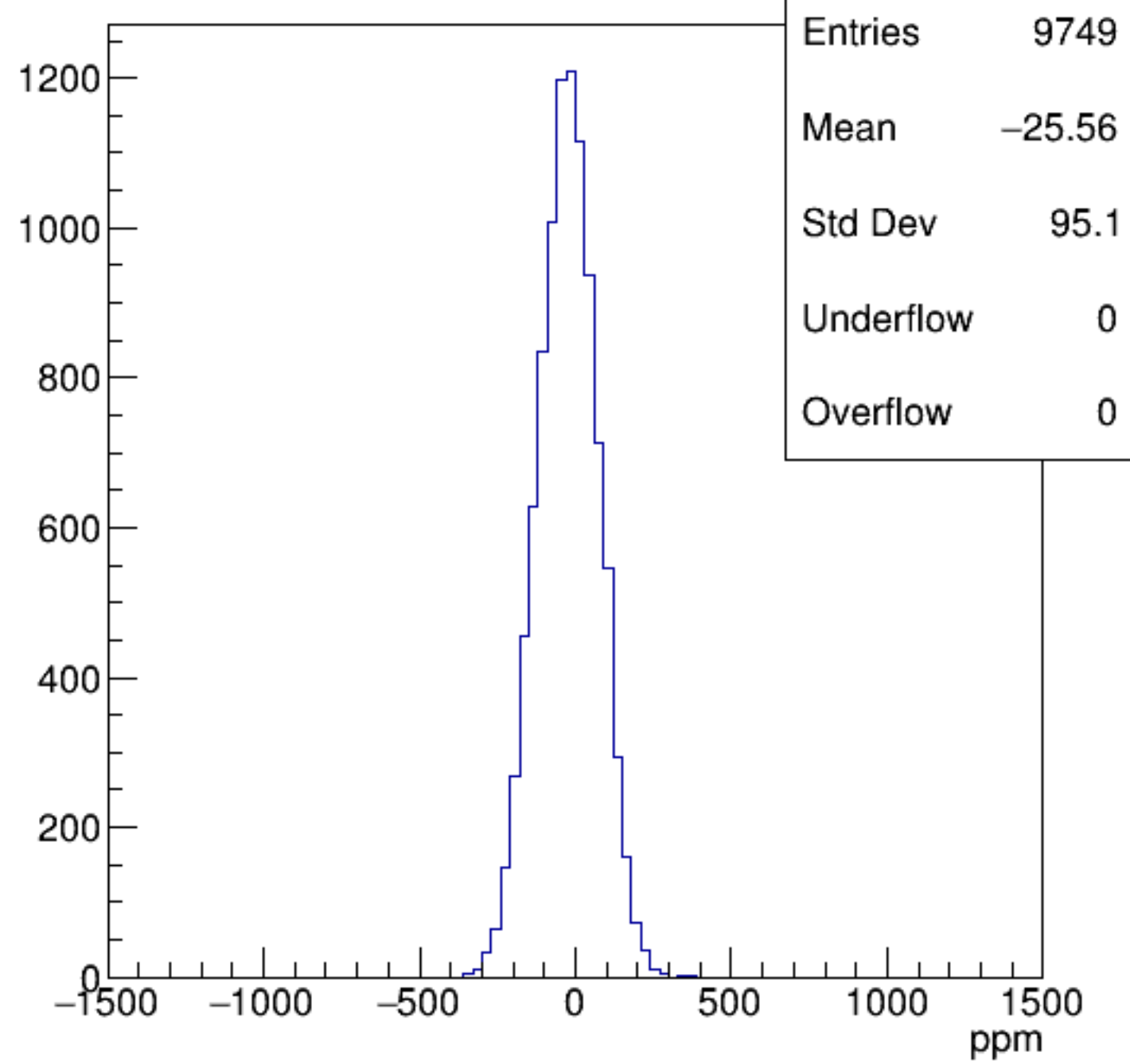
asym_bcm_an_ds
