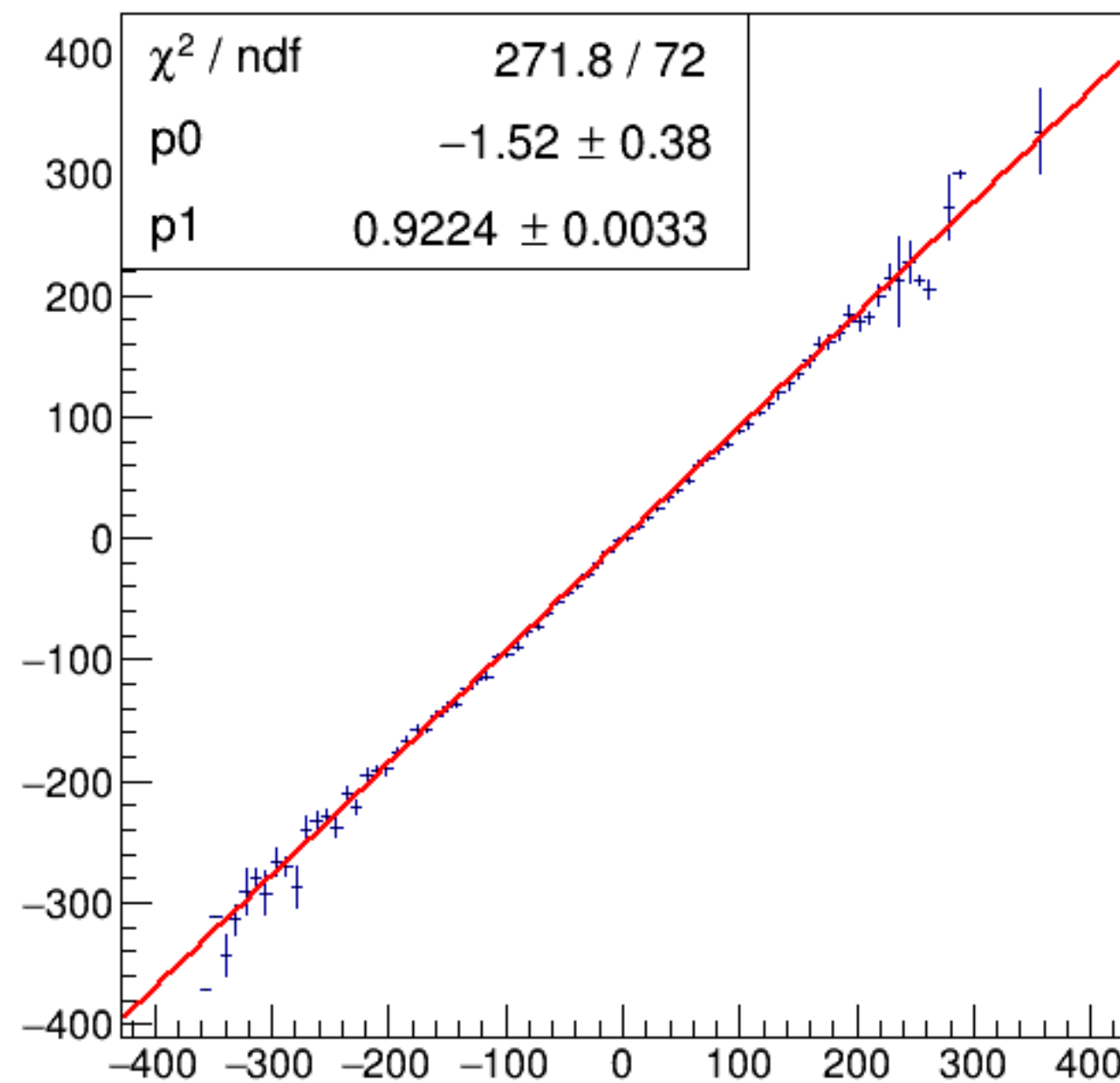
run3133_000_asym_bcm_an_us_vs_asym_bcm_an_ds.png
