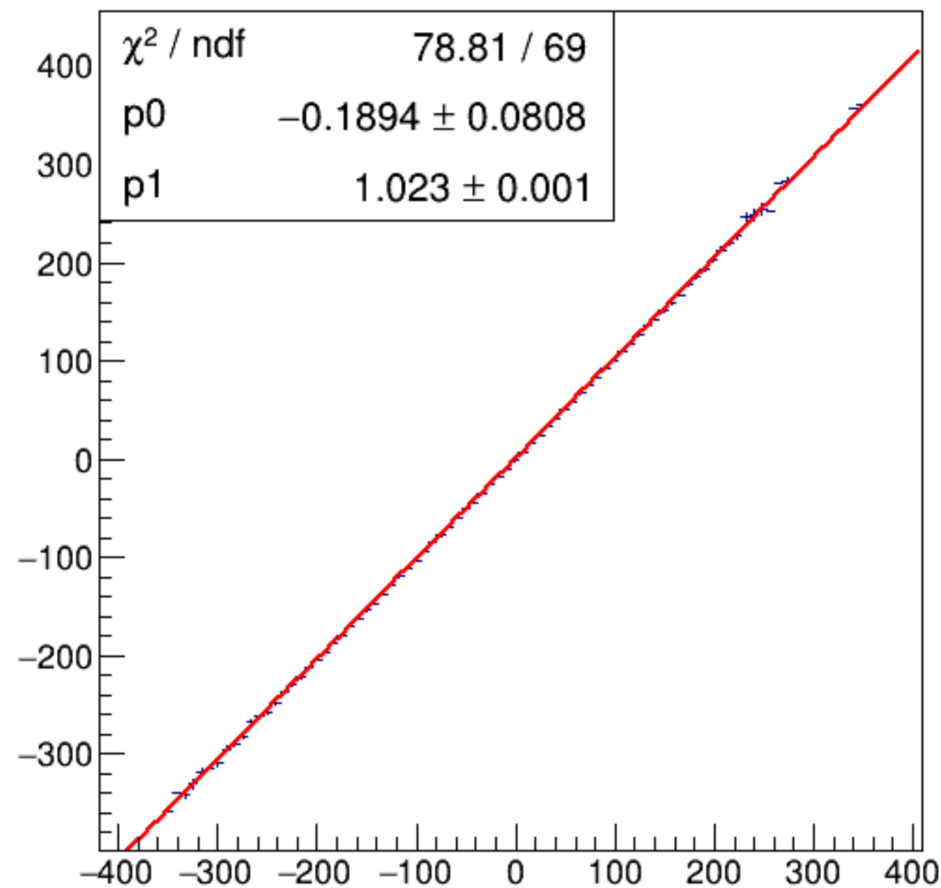
run3133_000_asym_bcm_an_ds_vs_asym_bcm_an_ds3.png
