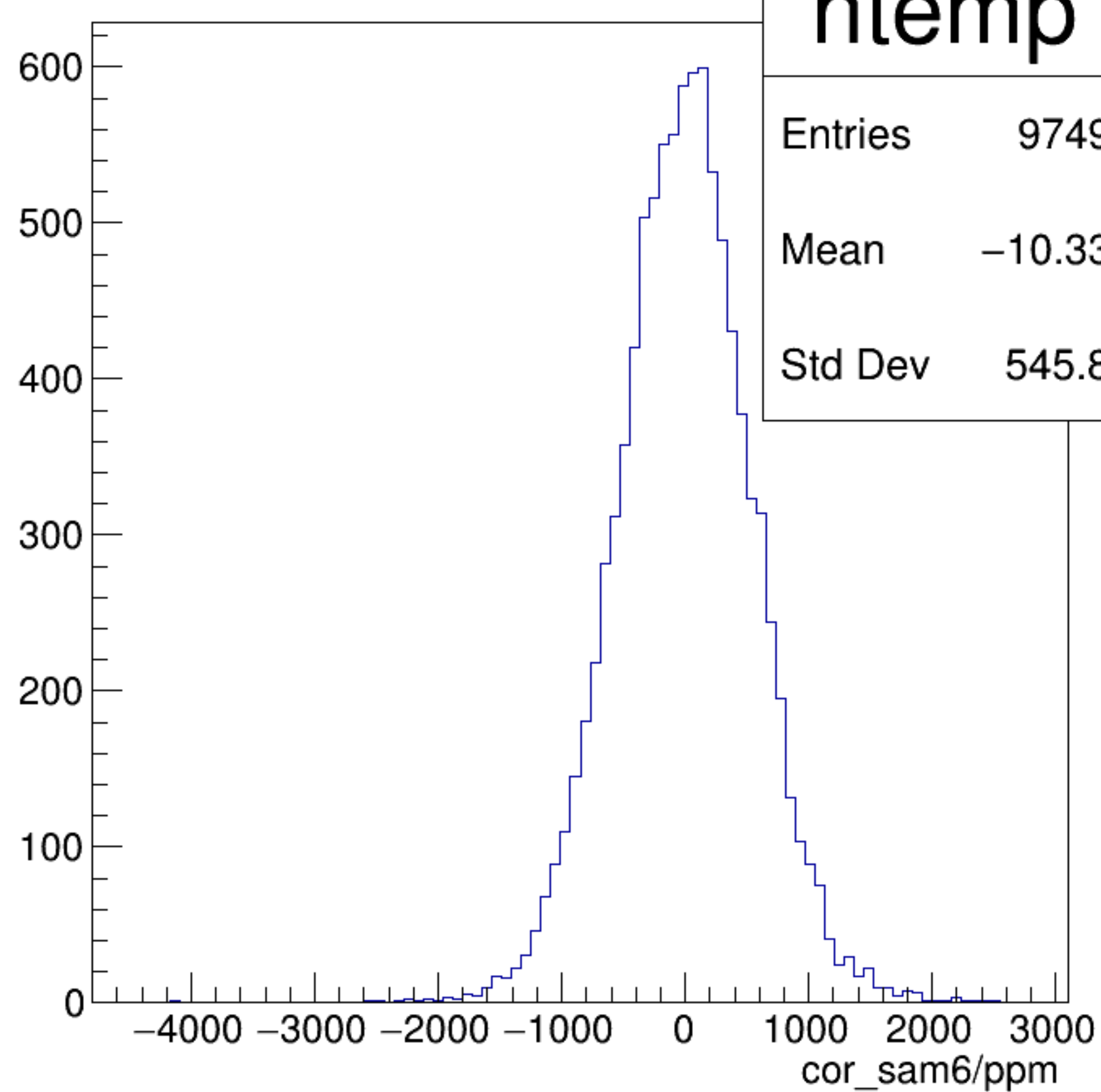
cor_sam6/ppm {ErrorFlag==0}
