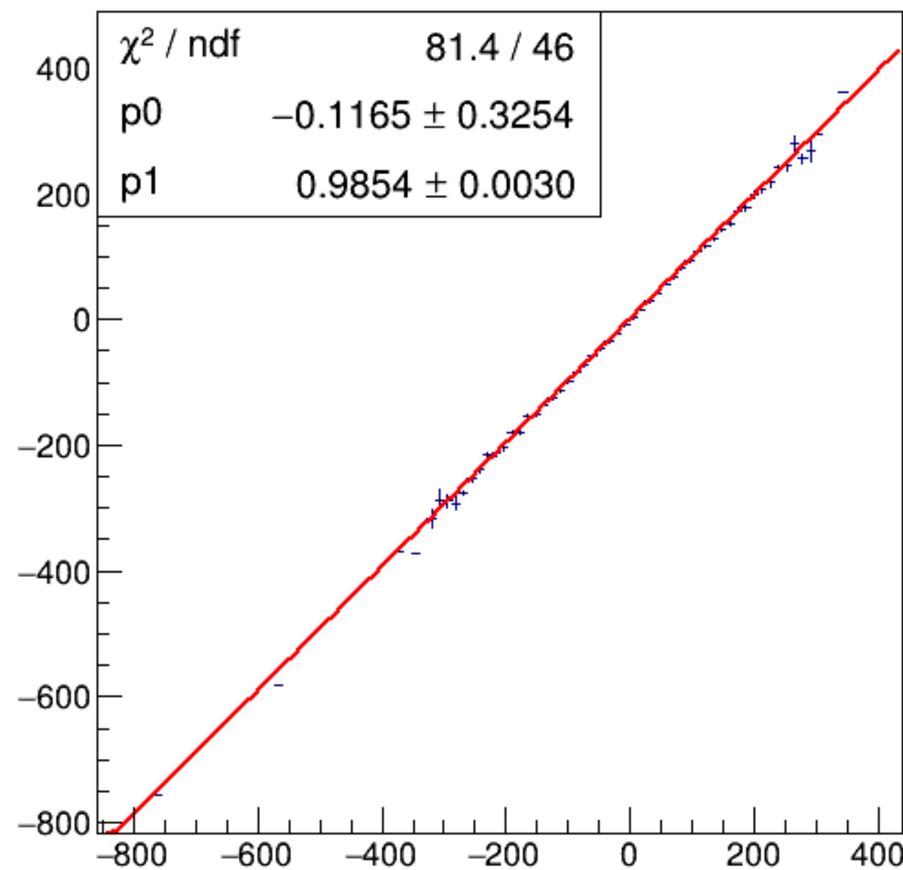
run3137_000_asym_bcm_an_us_vs_asym_bcm_an_ds.png
