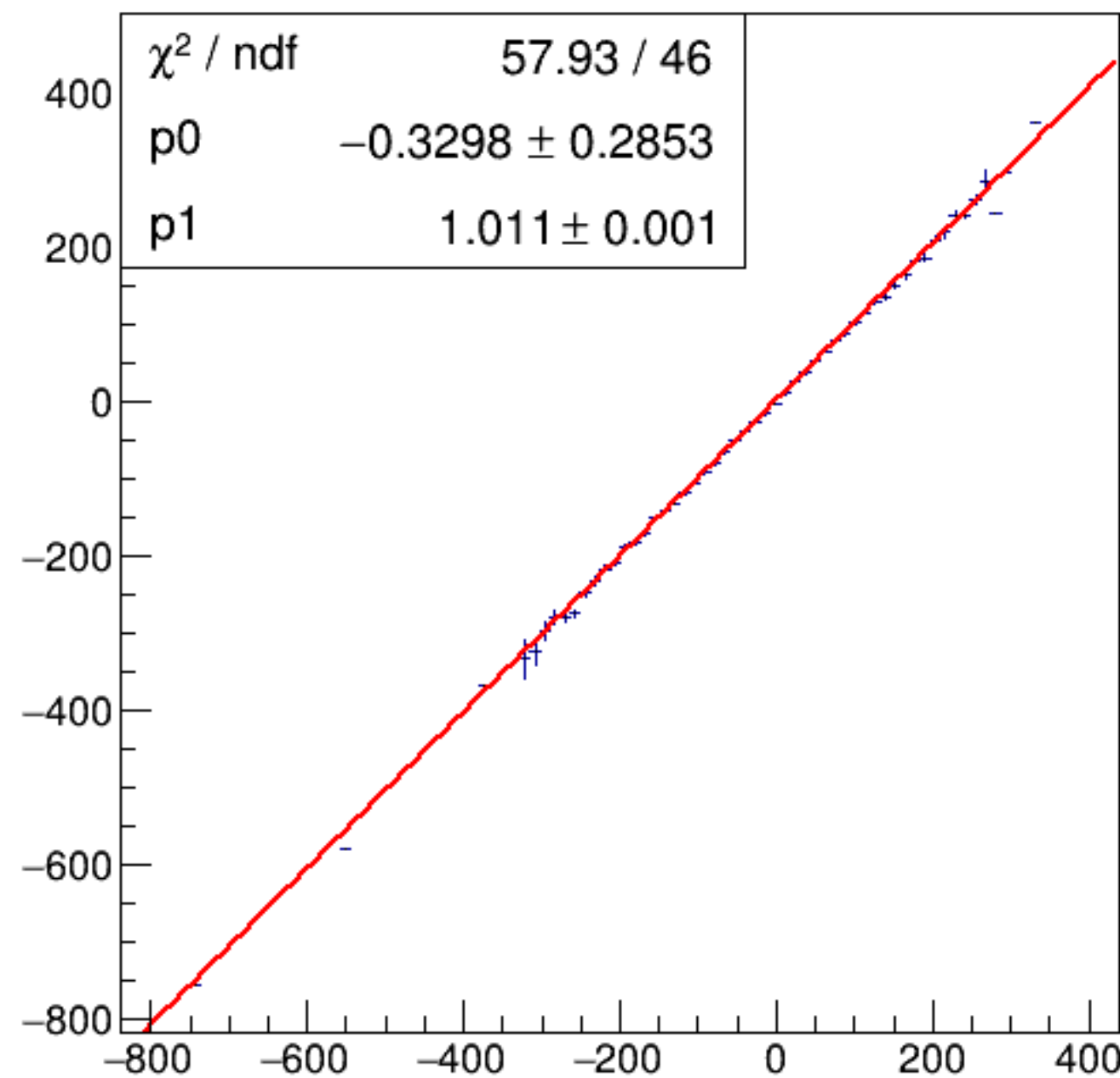
run3137_000_asym_bcm_an_us_vs_asym_bcm_an_ds3.png
