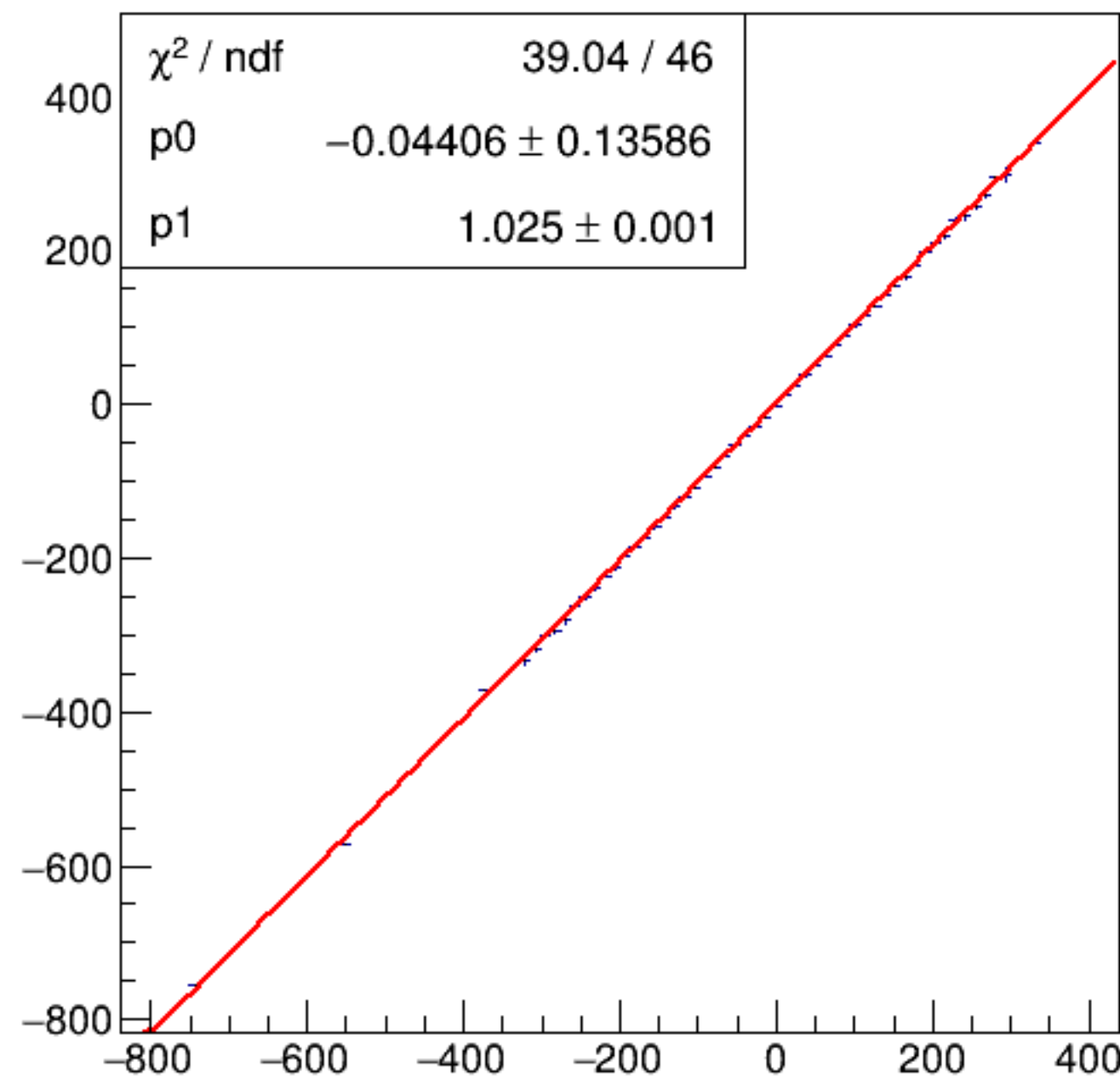
run3137_000_asym_bcm_an_ds_vs_asym_bcm_an_ds3.png
