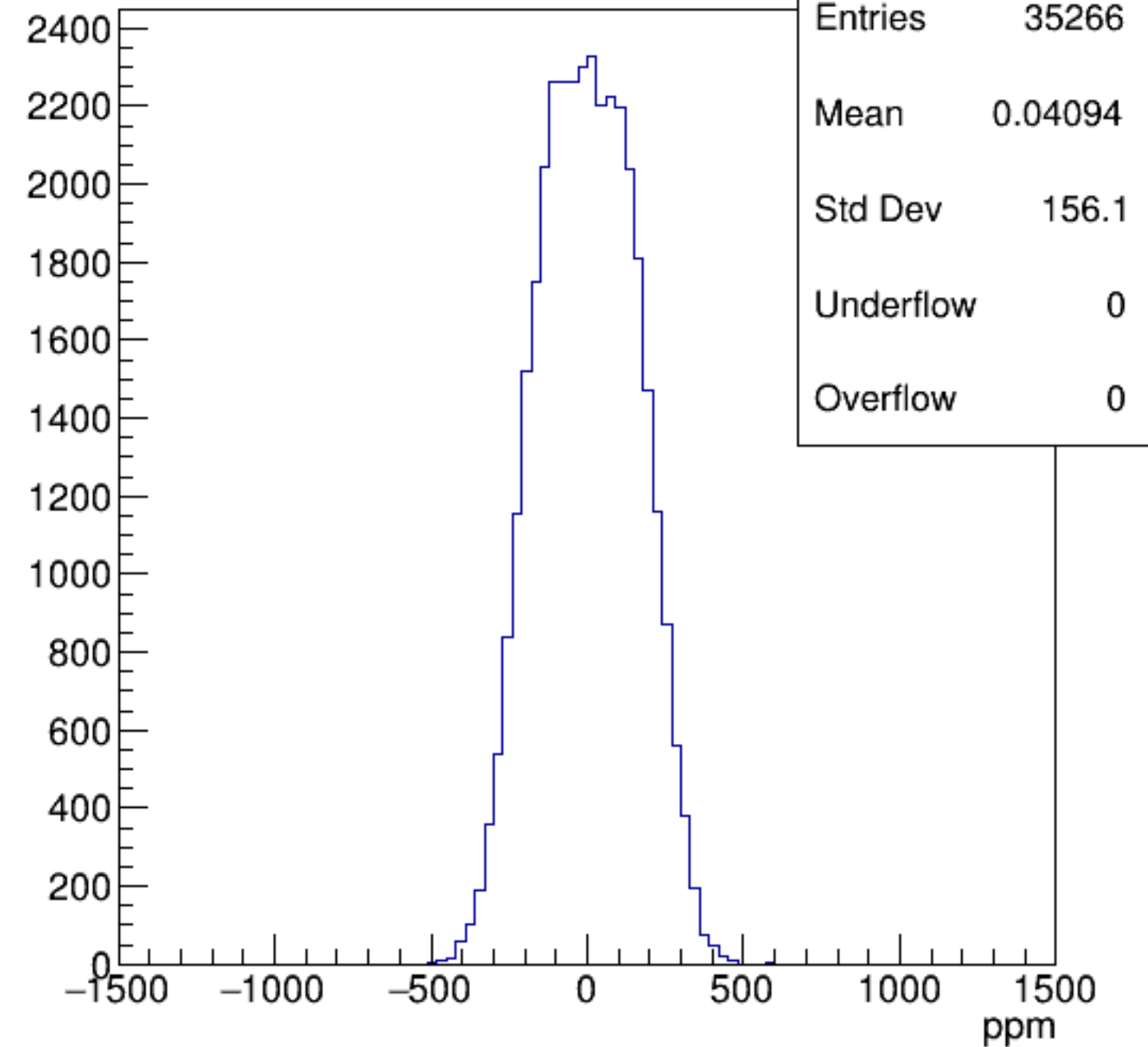
asym_bcm_an_ds3
