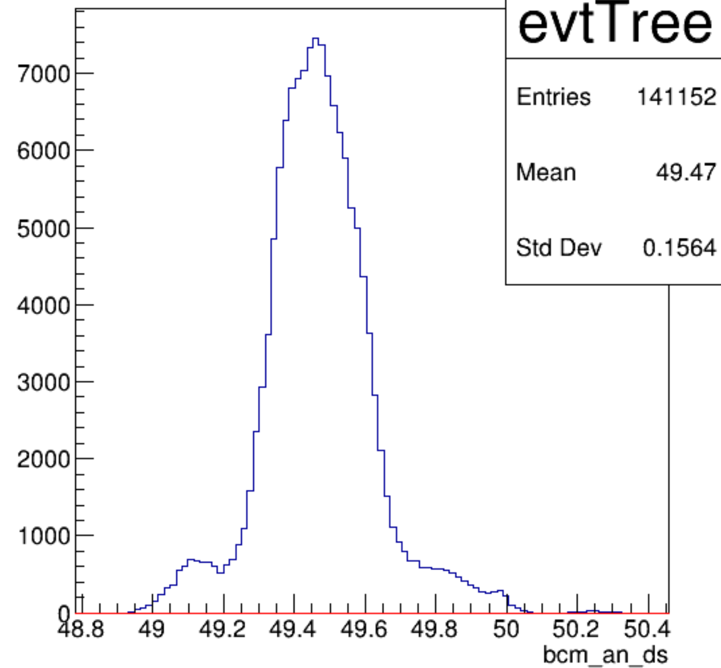
bcm_an_ds {ErrorFlag==0}
