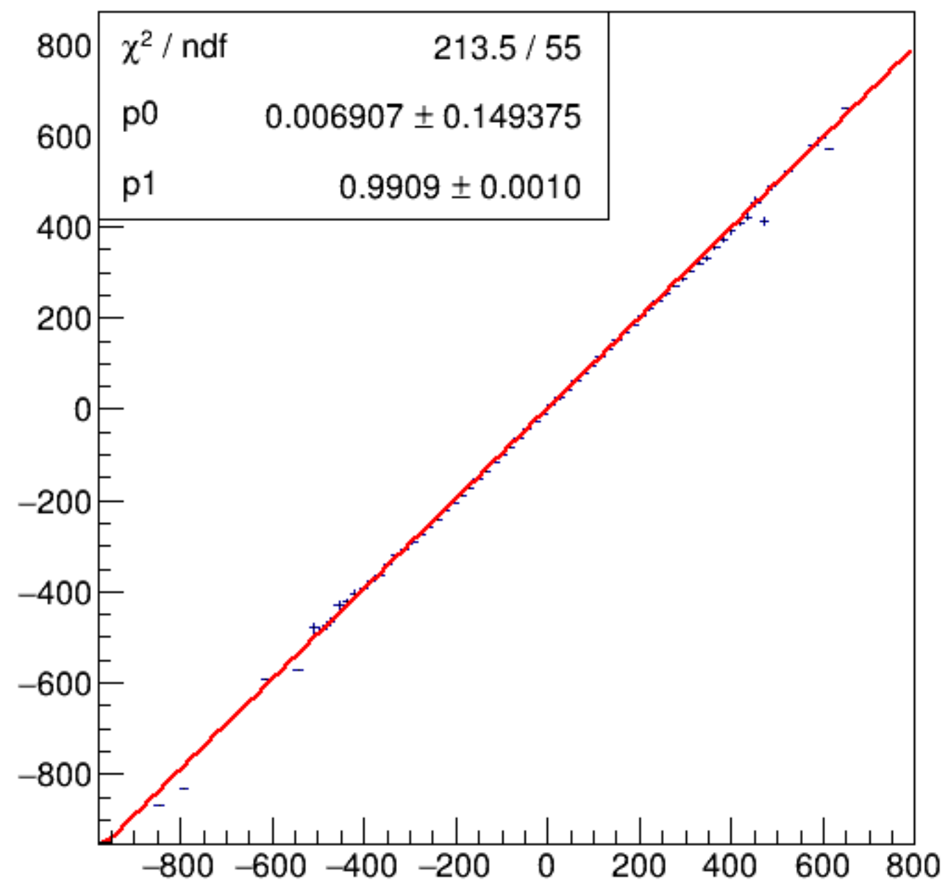
run3140_000_asym_bcm_an_us_vs_asym_bcm_an_ds.png
