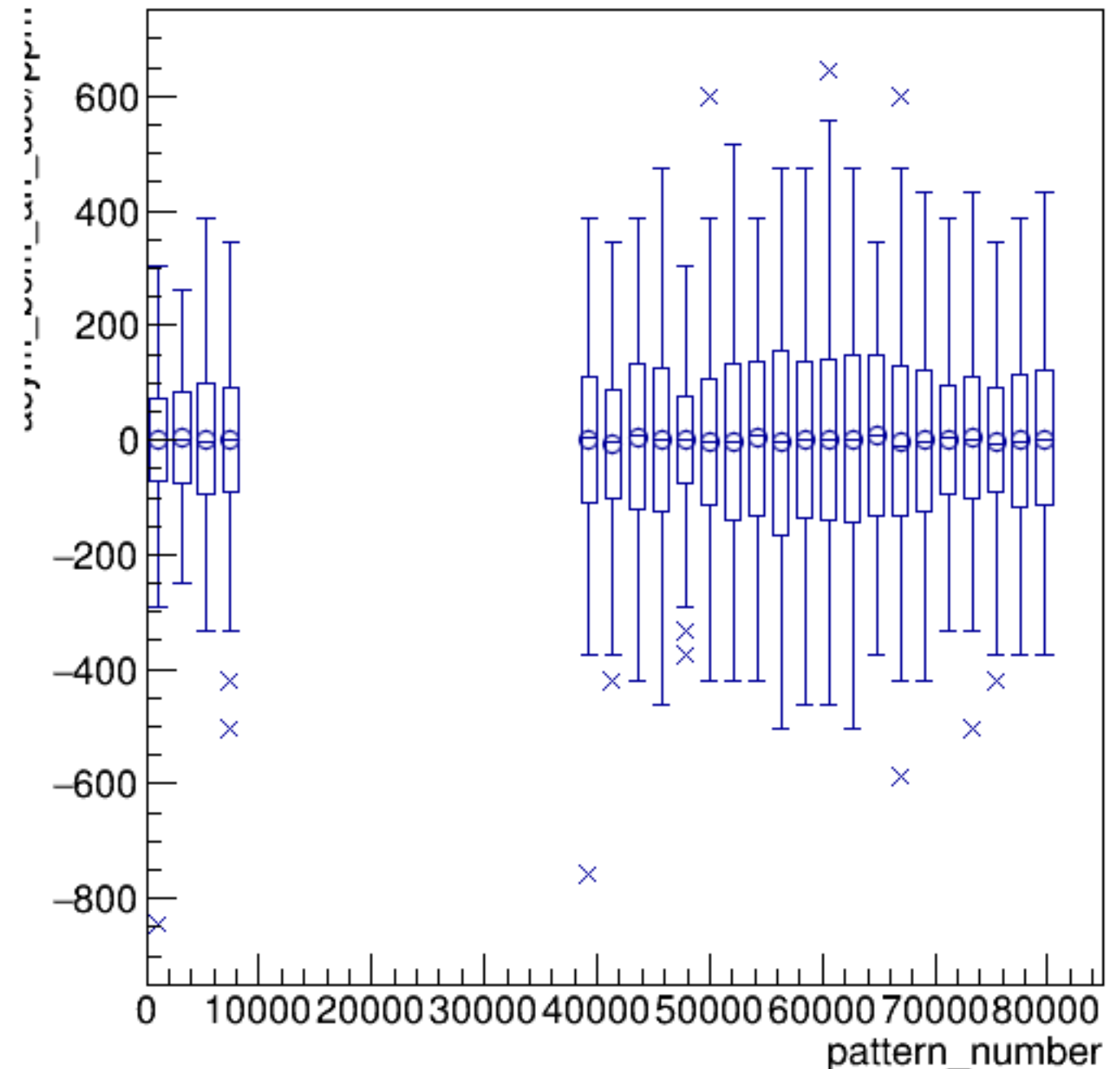
asym_bcm_an_ds3/ppm:pattern_number {ErrorFlag==0}
