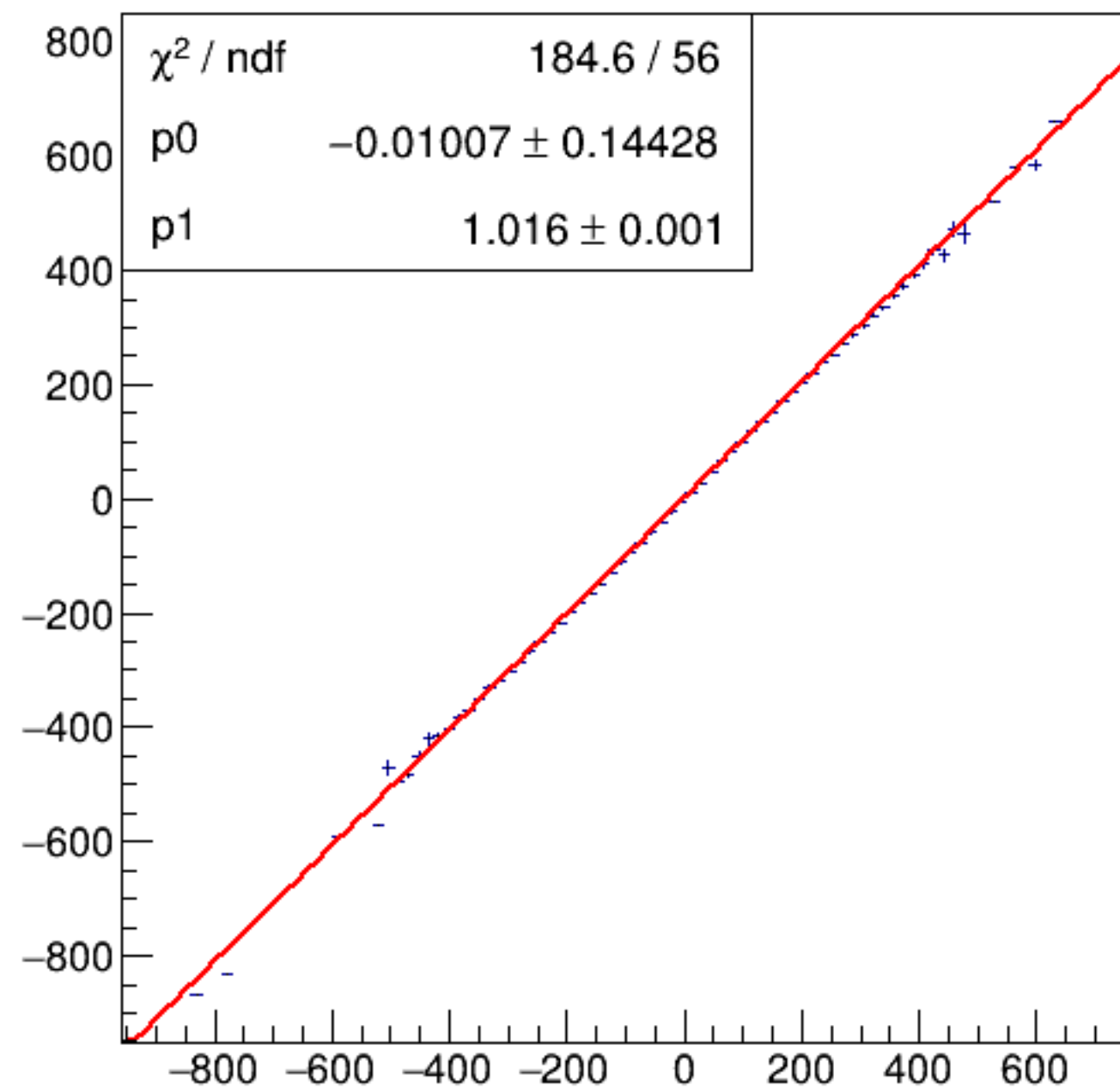
run3140_000_asym_bcm_an_us_vs_asym_bcm_an_ds3.png
