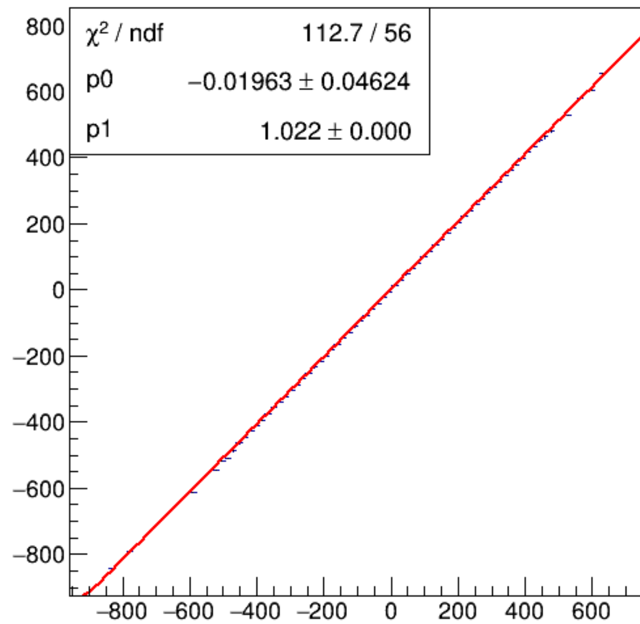
run3140_000_asym_bcm_an_ds_vs_asym_bcm_an_ds3.png
