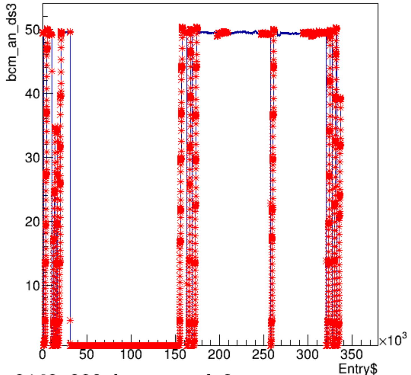
bcm_an_ds3:Entry$
