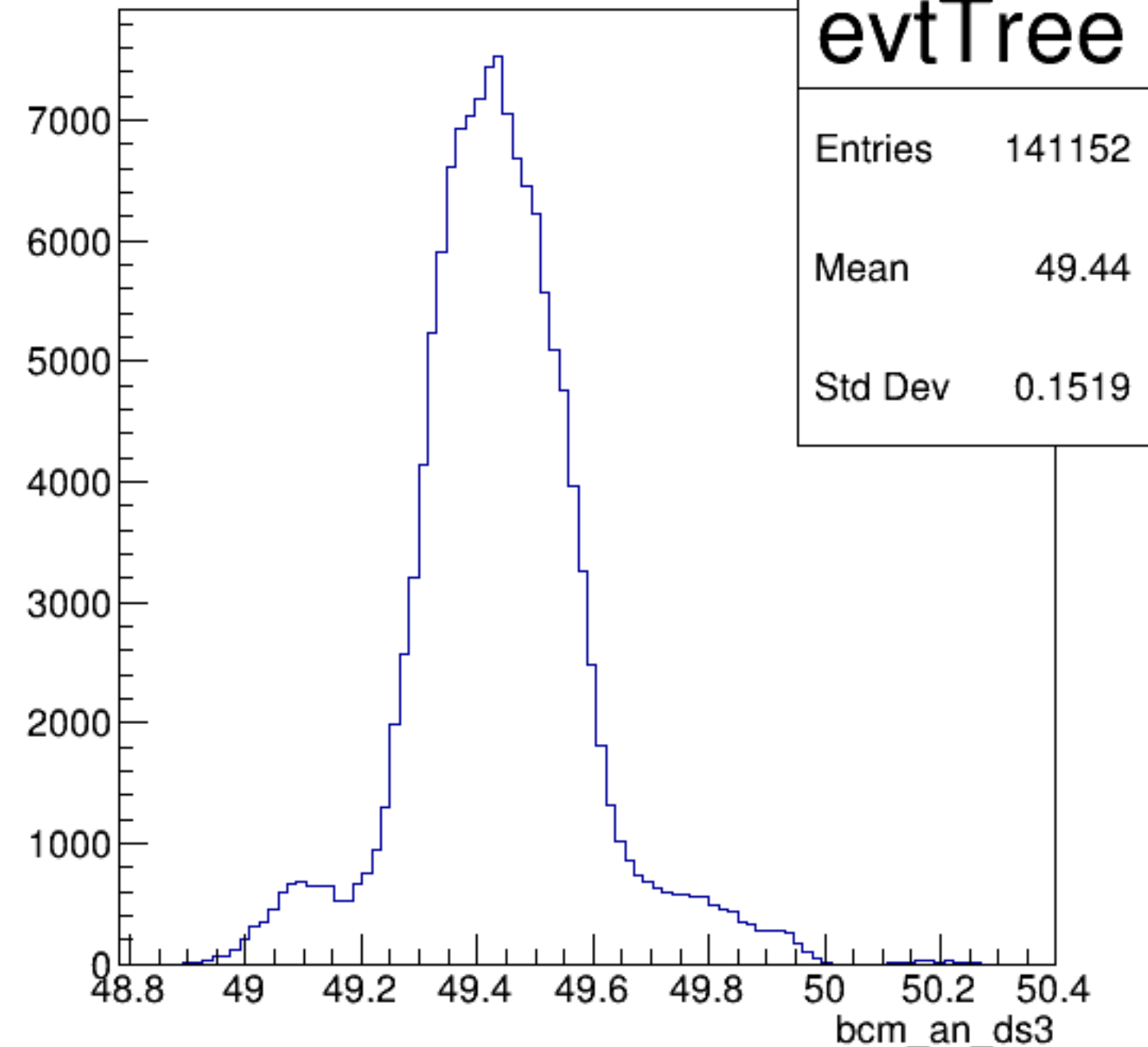
bcm_an_ds3 {ErrorFlag==0}
