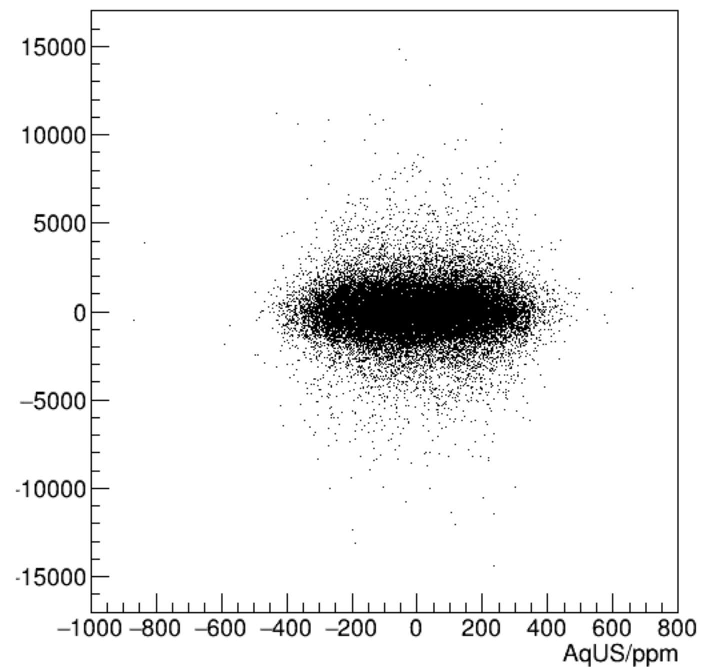
cor_sam6/ppm:AqUS/ppm {ErrorFlag==0}
