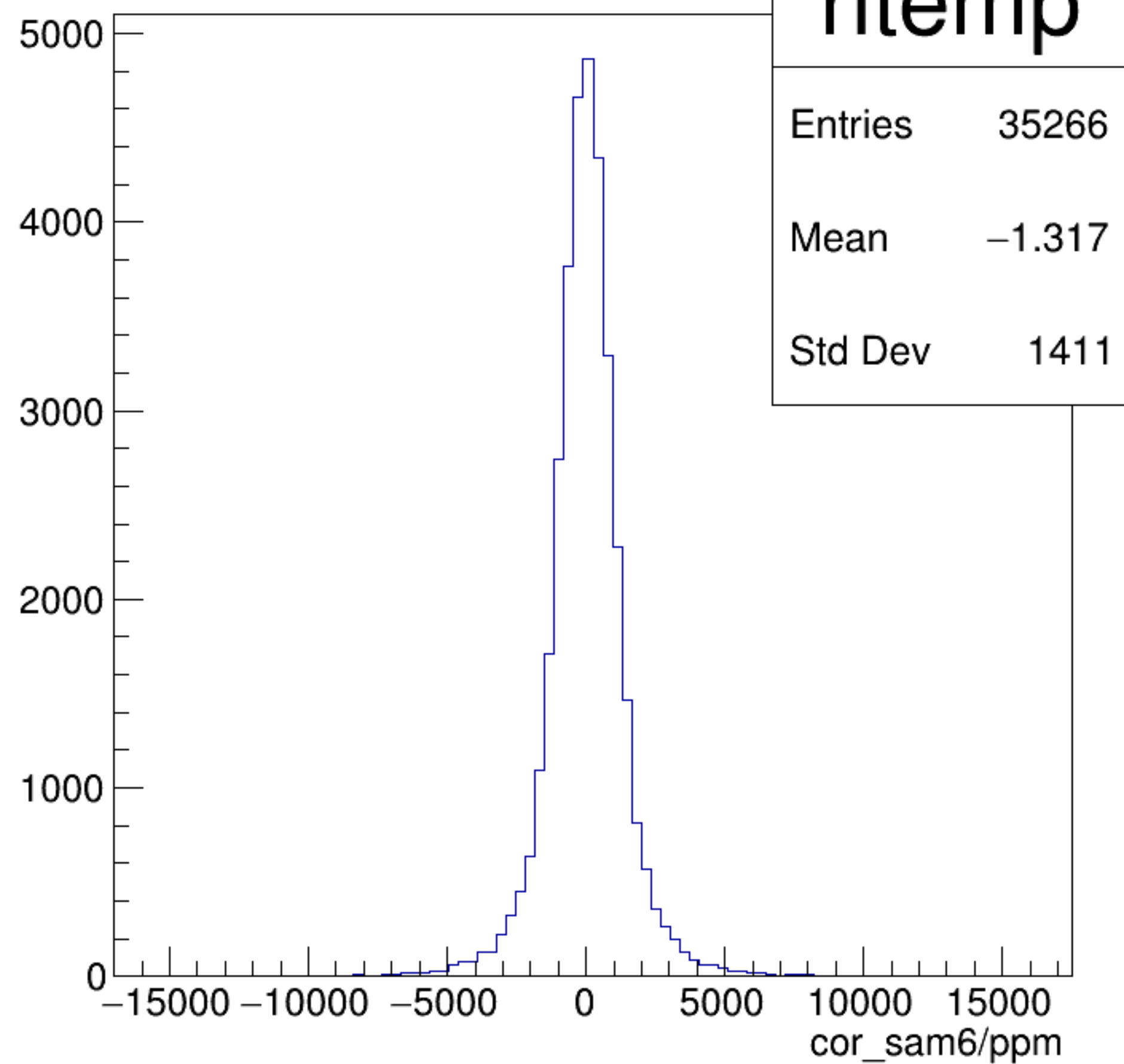
cor_sam6/ppm {ErrorFlag==0}
