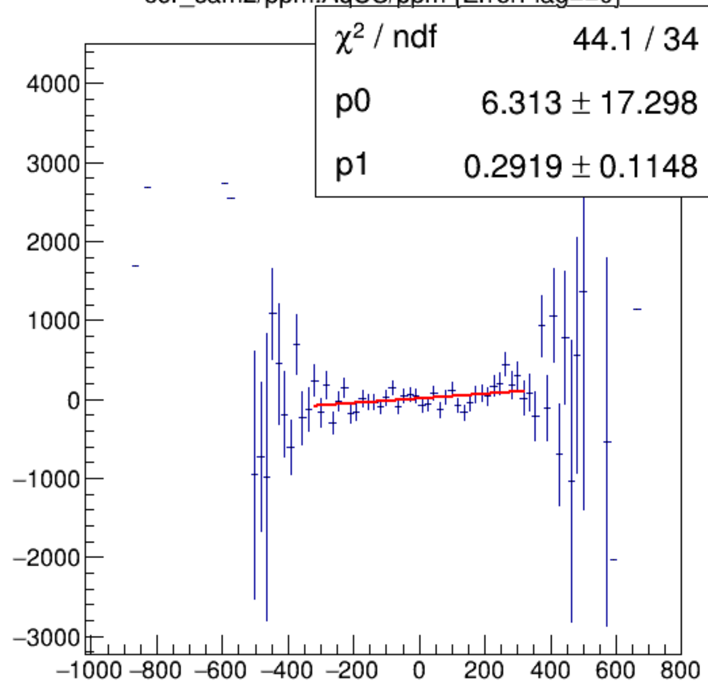
cor_sam2/ppm:AqUS/ppm {ErrorFlag==0}
