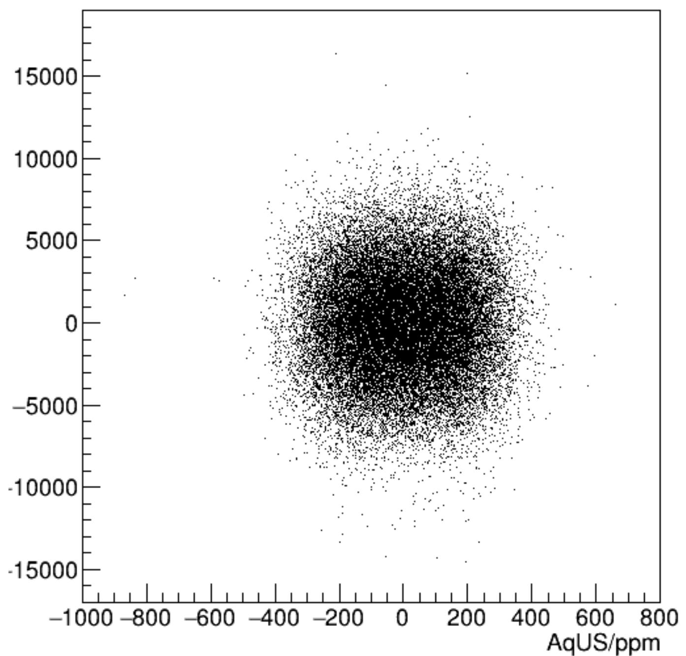
cor_sam2/ppm:AqUS/ppm {ErrorFlag==0}
