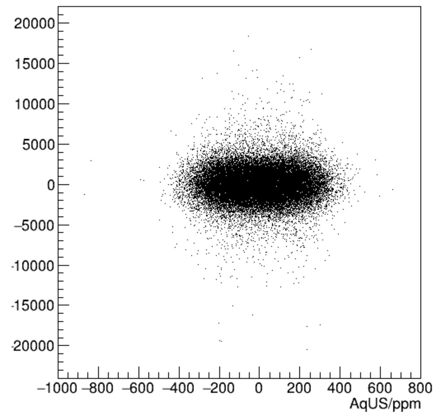
cor_sam4/ppm:AqUS/ppm {ErrorFlag==0}
