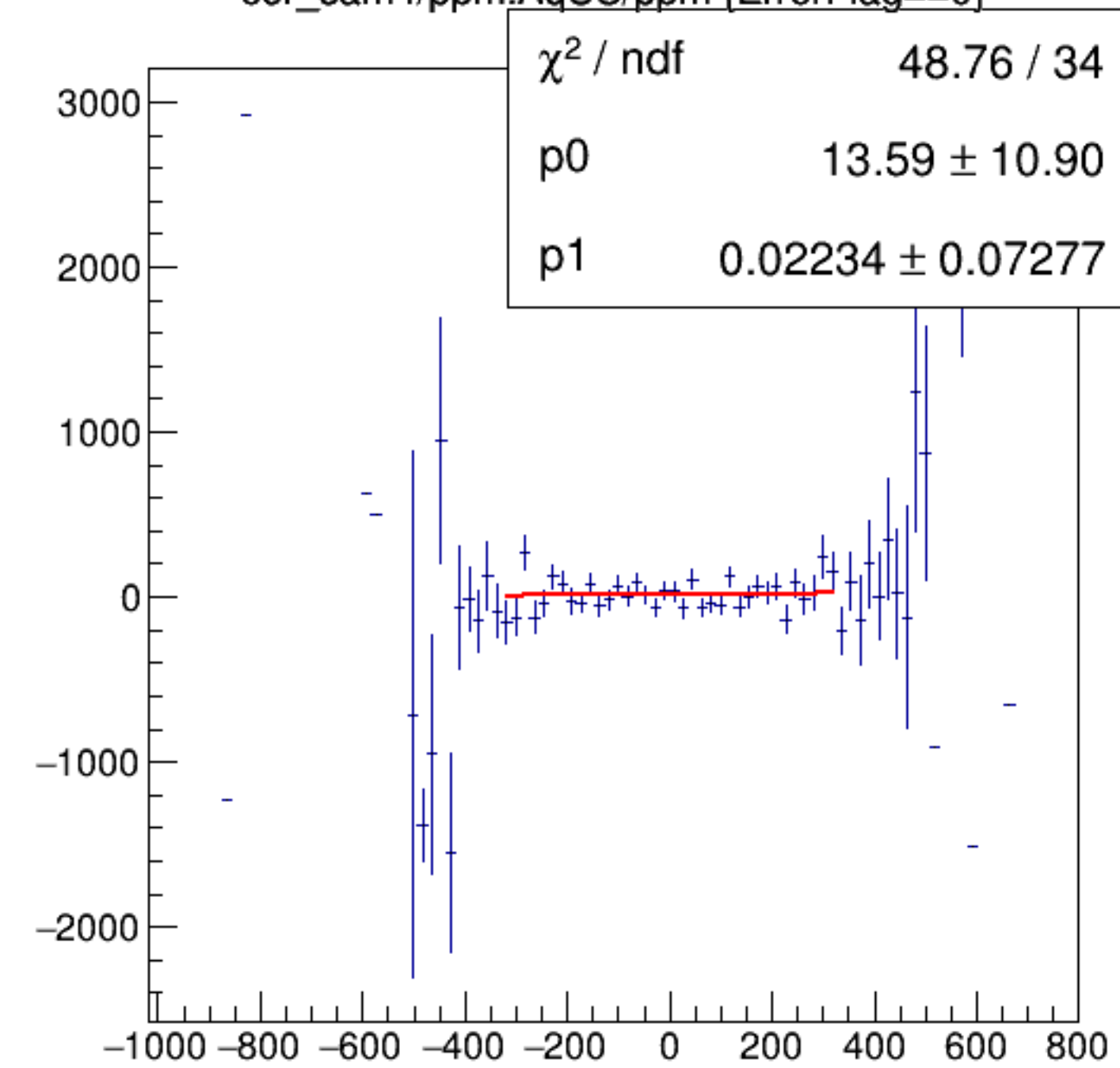
cor_sam4/ppm:AqUS/ppm {ErrorFlag==0}
