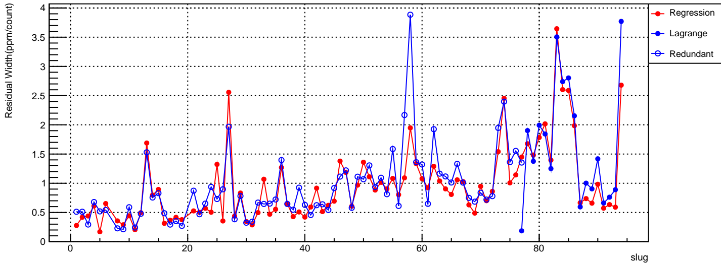
usl vs coil 5 residual Width (ppm/count)
