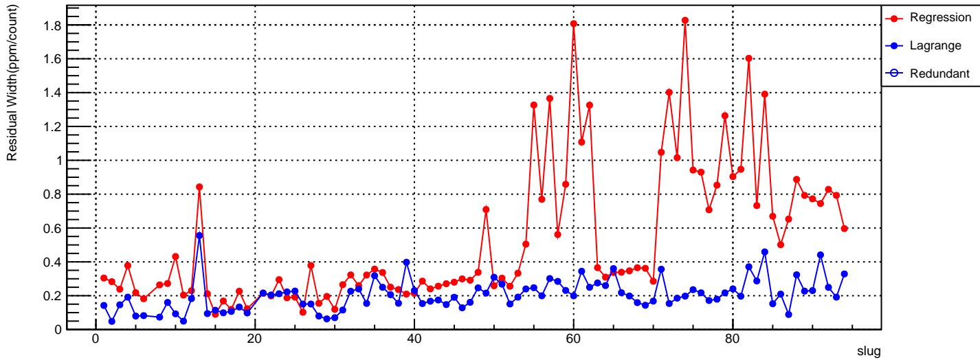
usl vs coil 4 residual Width (ppm/count)
