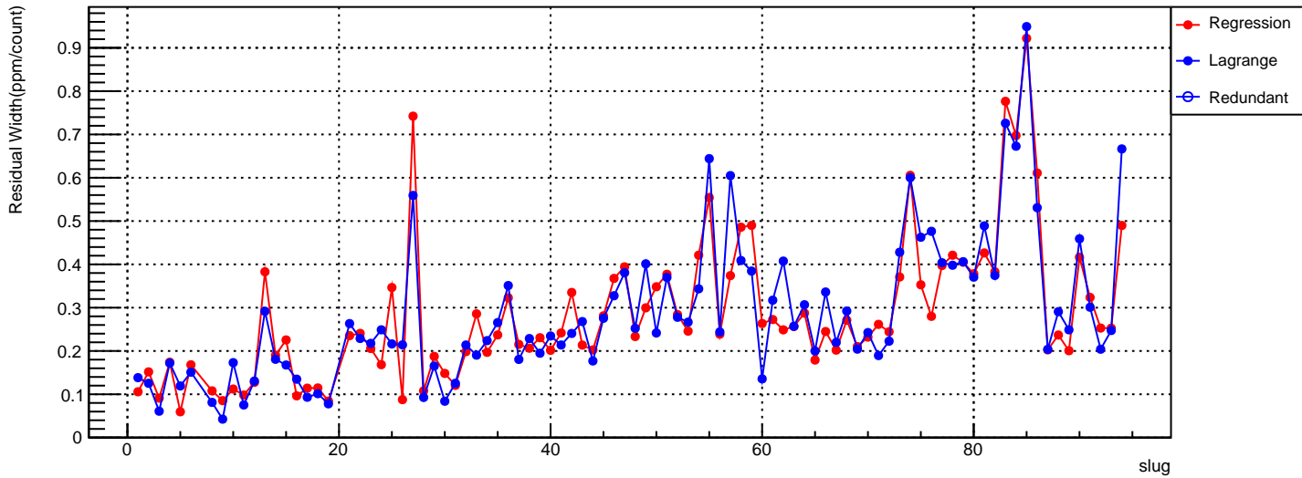
usl vs coil 3 residual Width (ppm/count)
