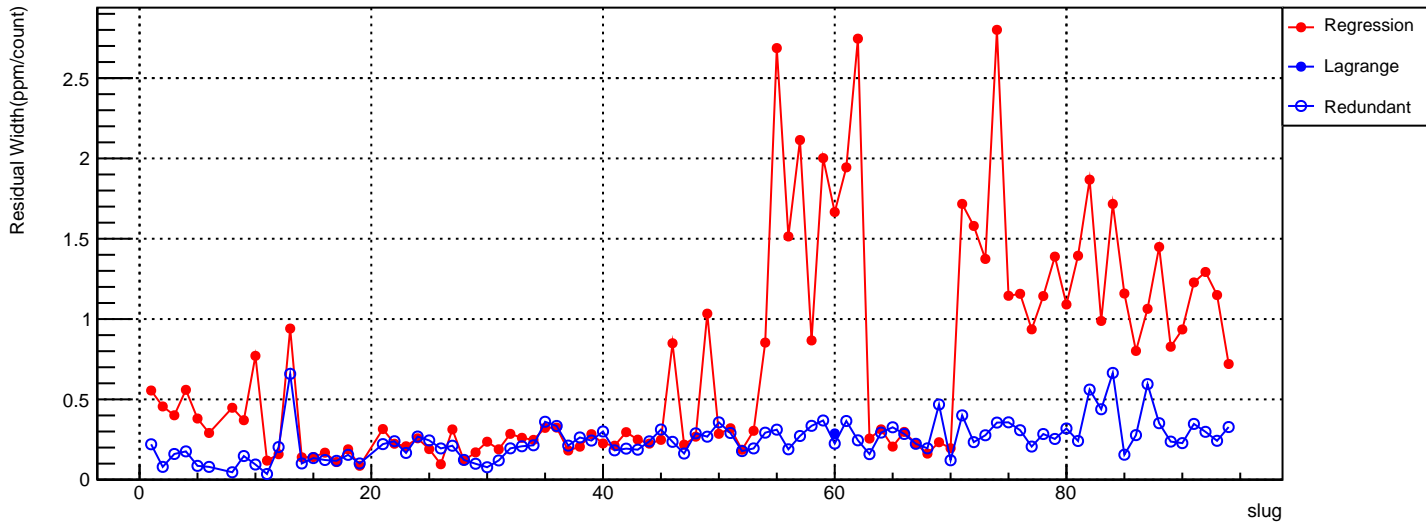
usl vs coil 2 residual Width (ppm/count)
