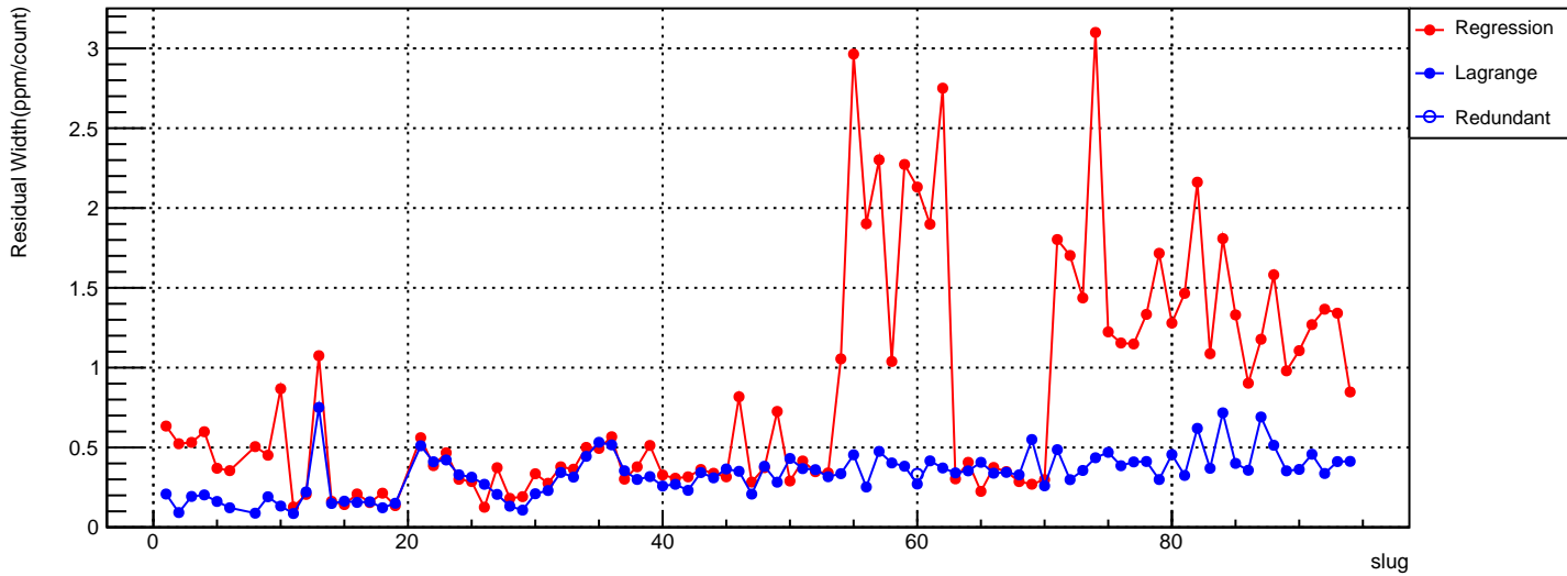
usl vs coil 6 residual Width (ppm/count)
